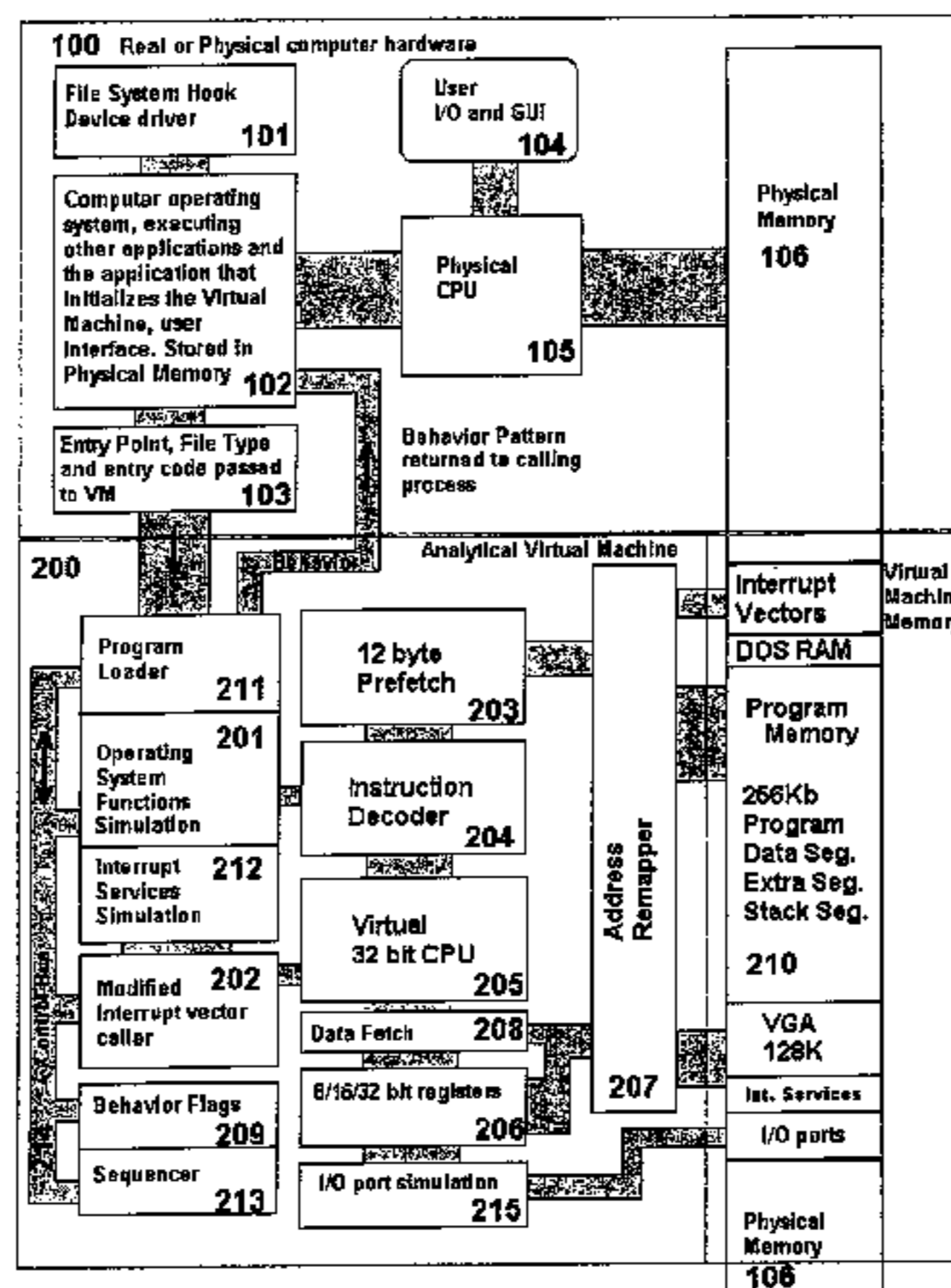
The vCIS Analytical Virtual Machine
