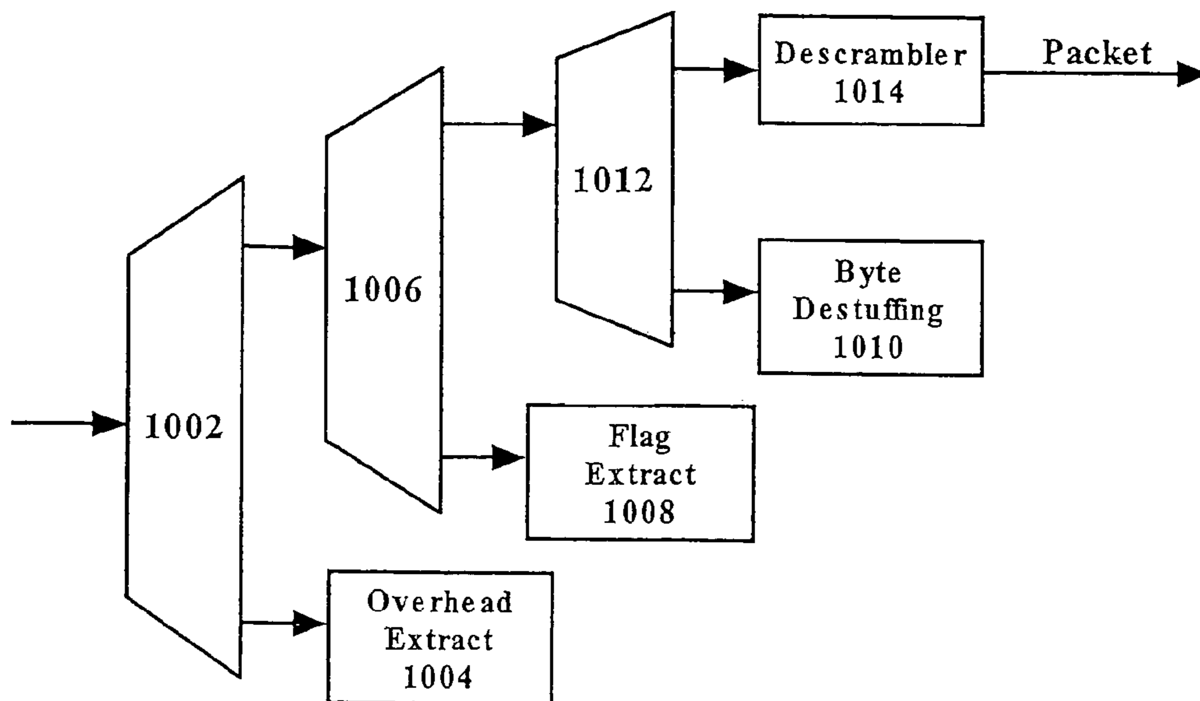
FIG. 10 (PRIOR ART)
