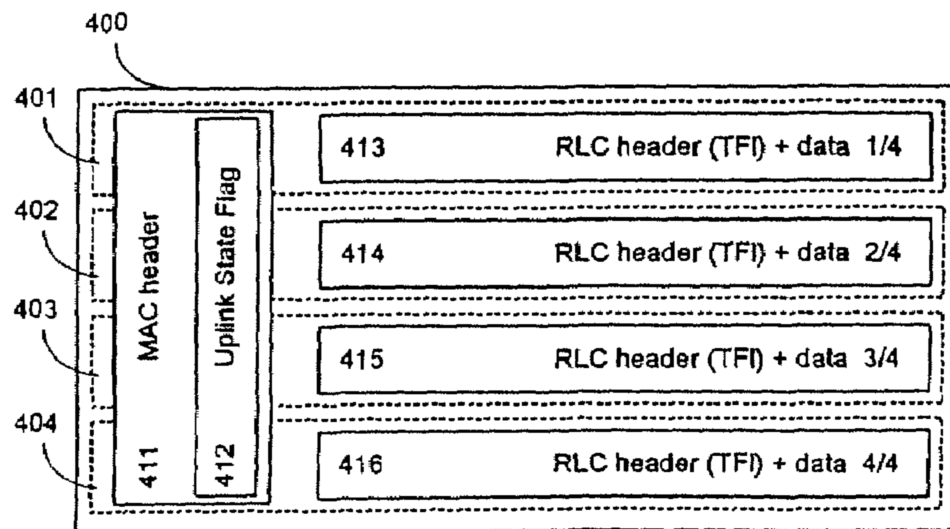
FIG. 4 PRIOR ART
