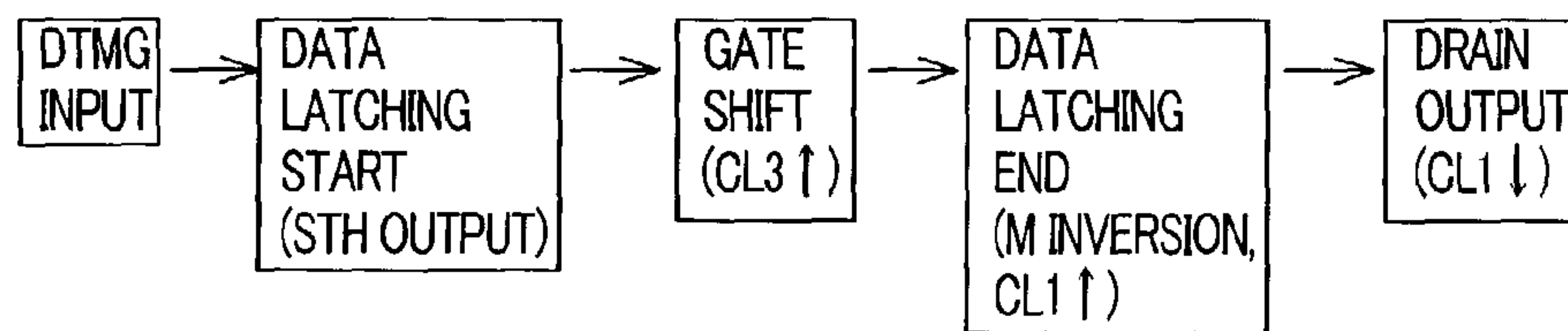
SEQUENCE OF THE LIQUID CRYSTAL DRIVER (EXAMPLE)
