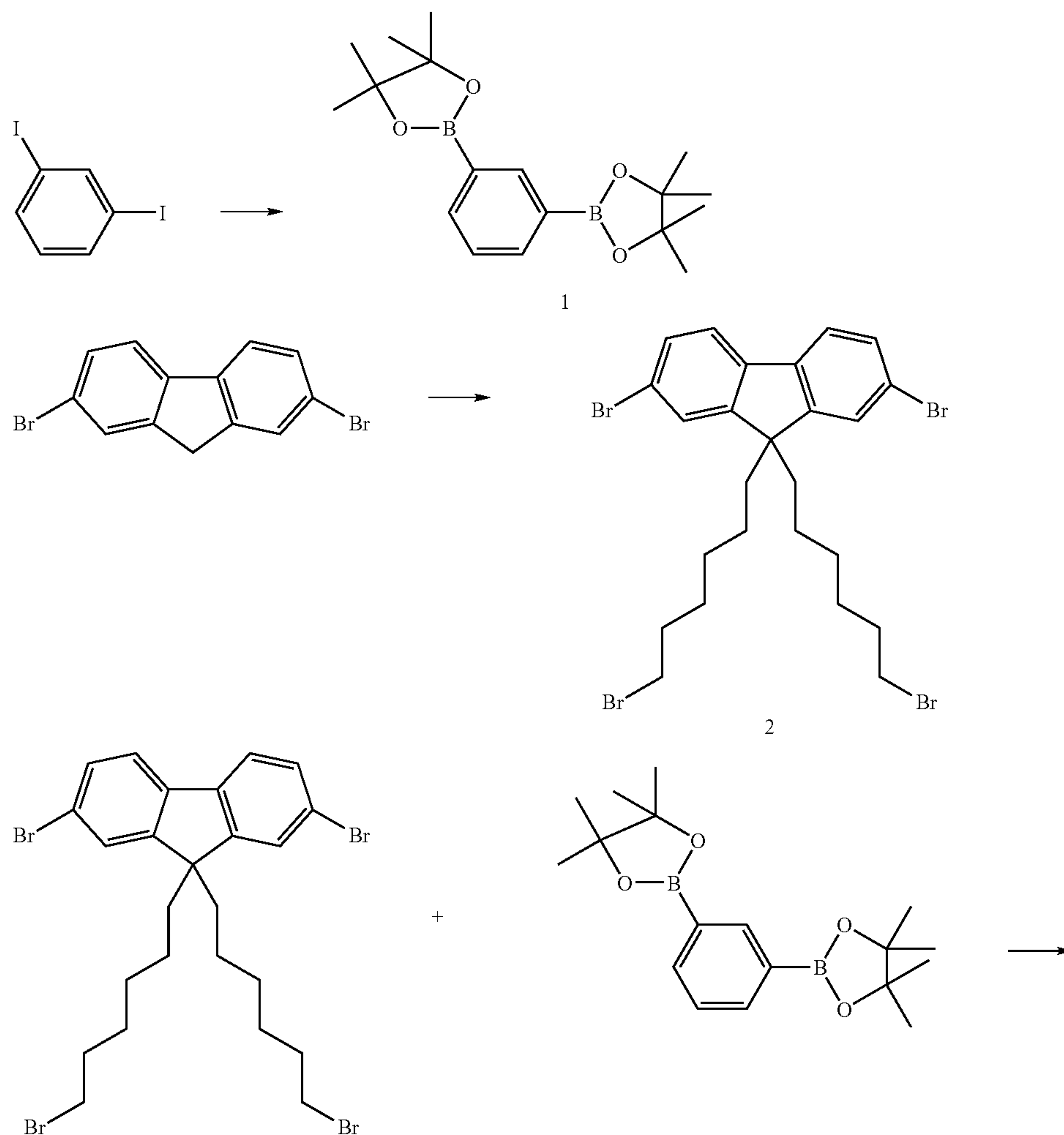
Scheme 1. Synthetic procedure for cationic water-soluble polymers.
