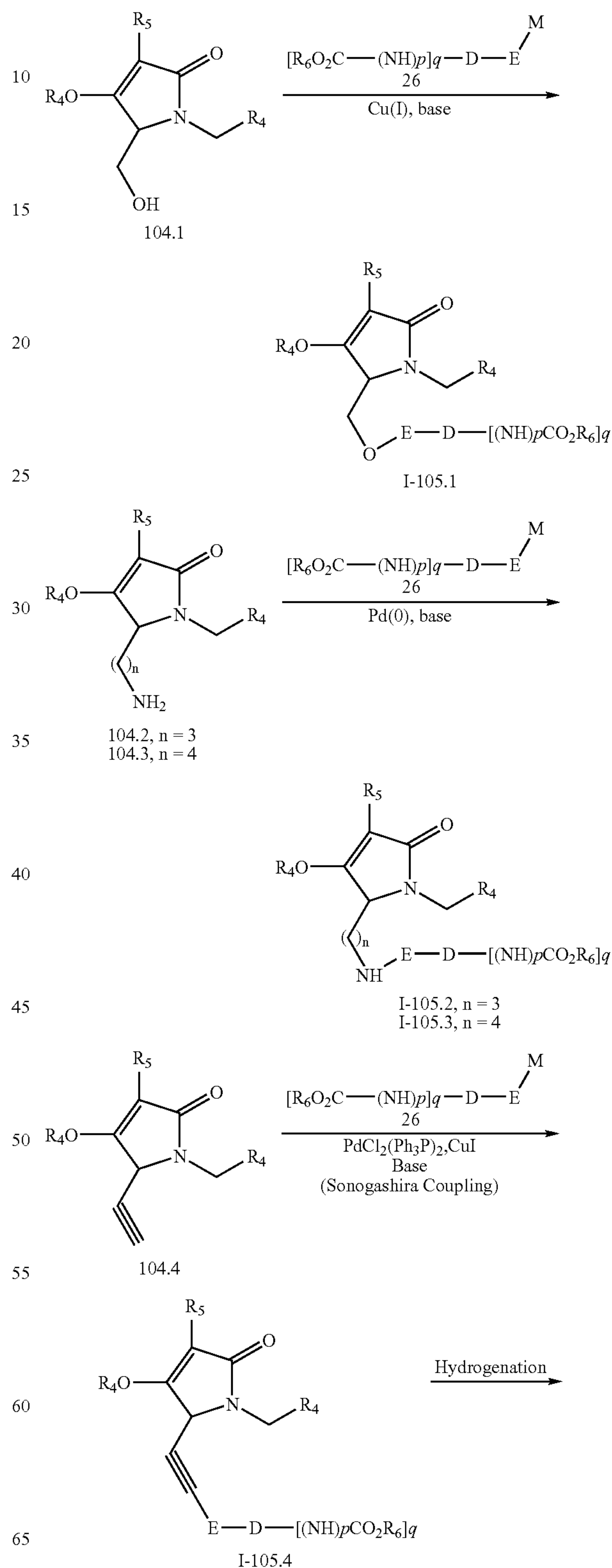
Scheme 17.2
