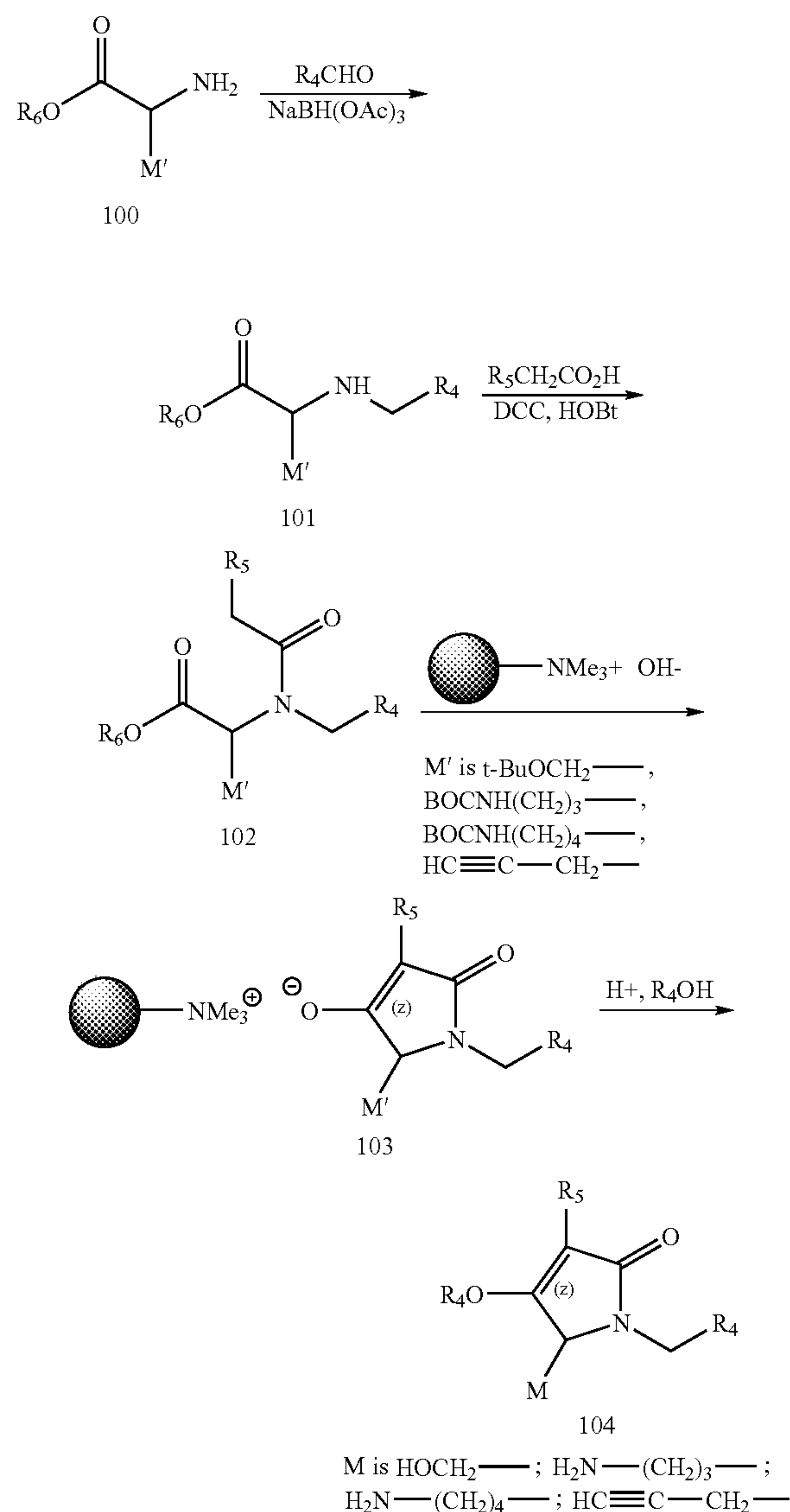
Scheme 17.1
