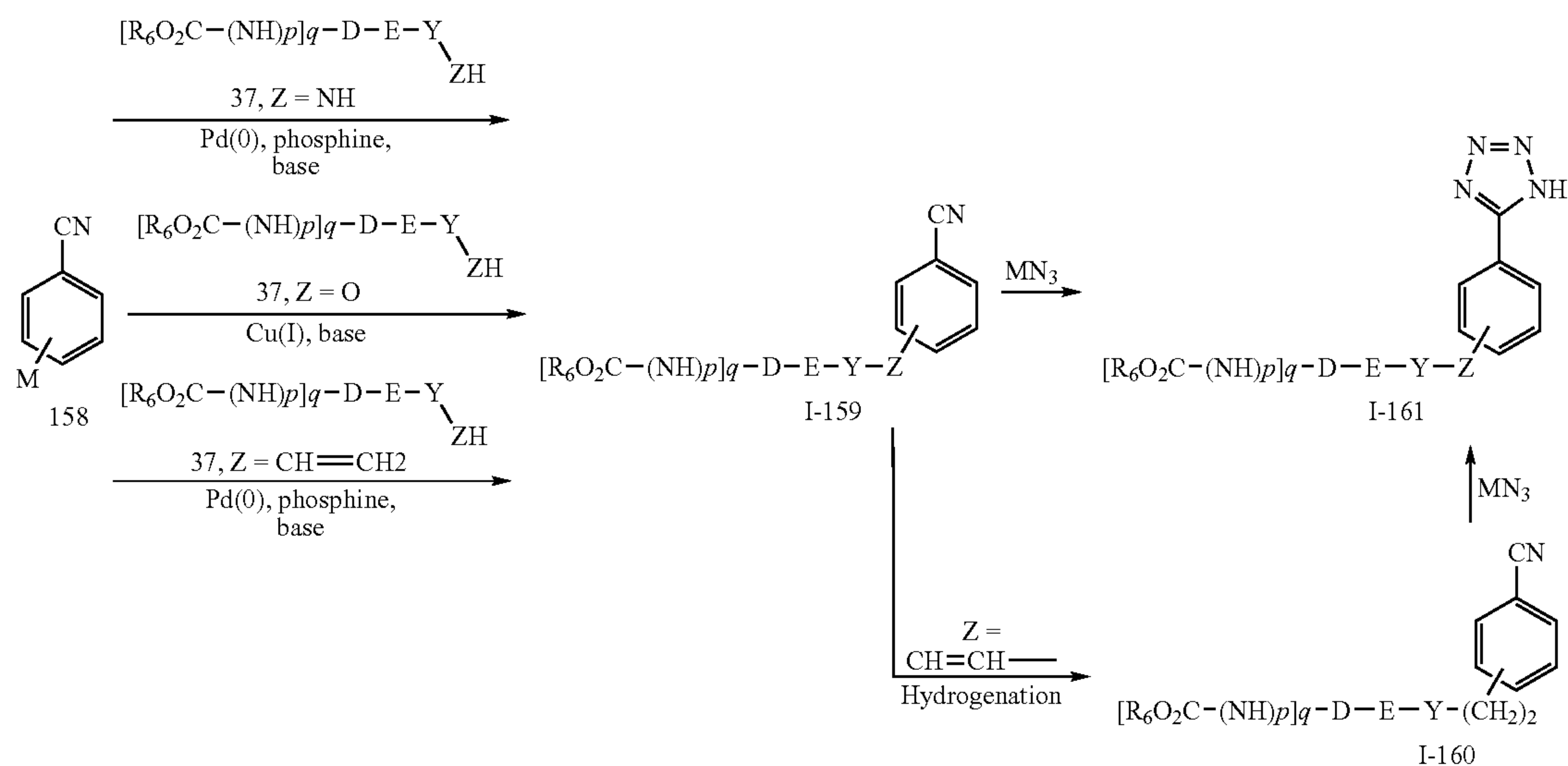
Scheme 25
