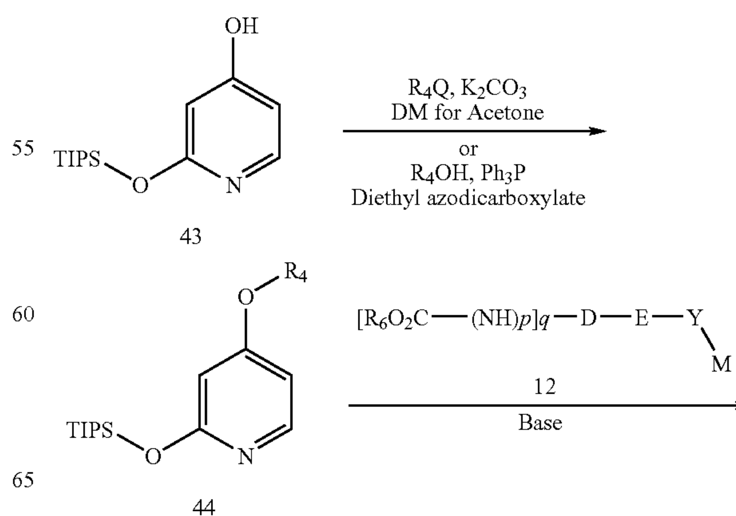
Scheme 8
