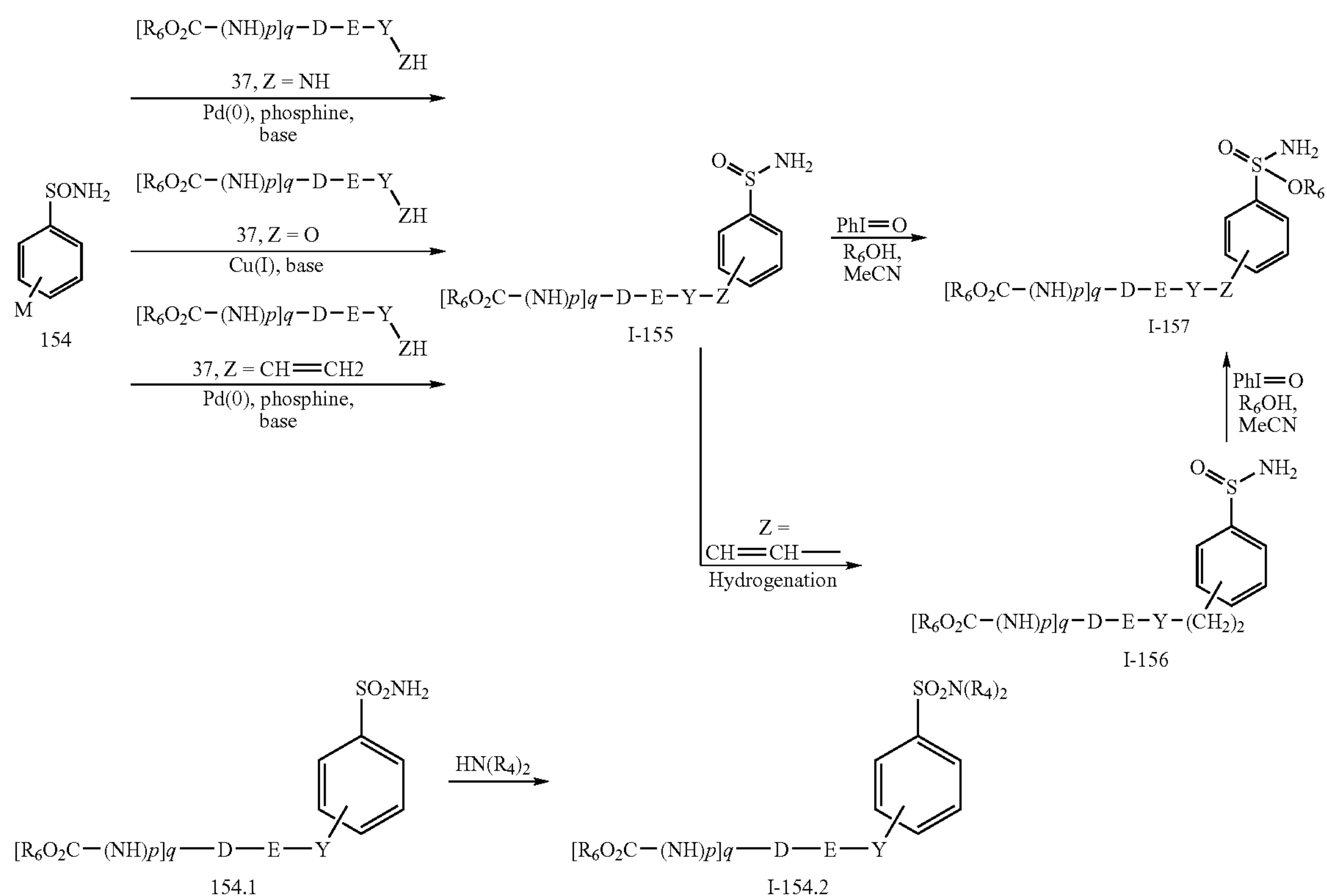
Scheme 24
