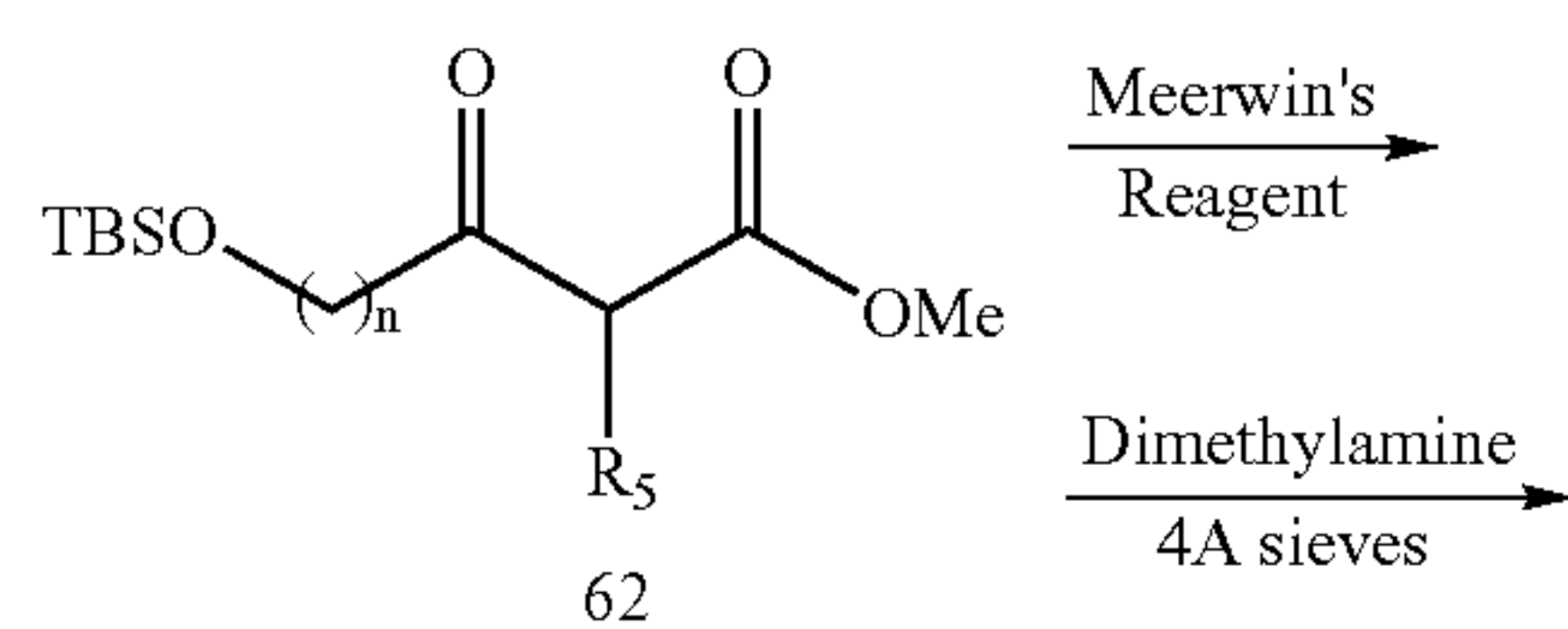
Scheme 11
