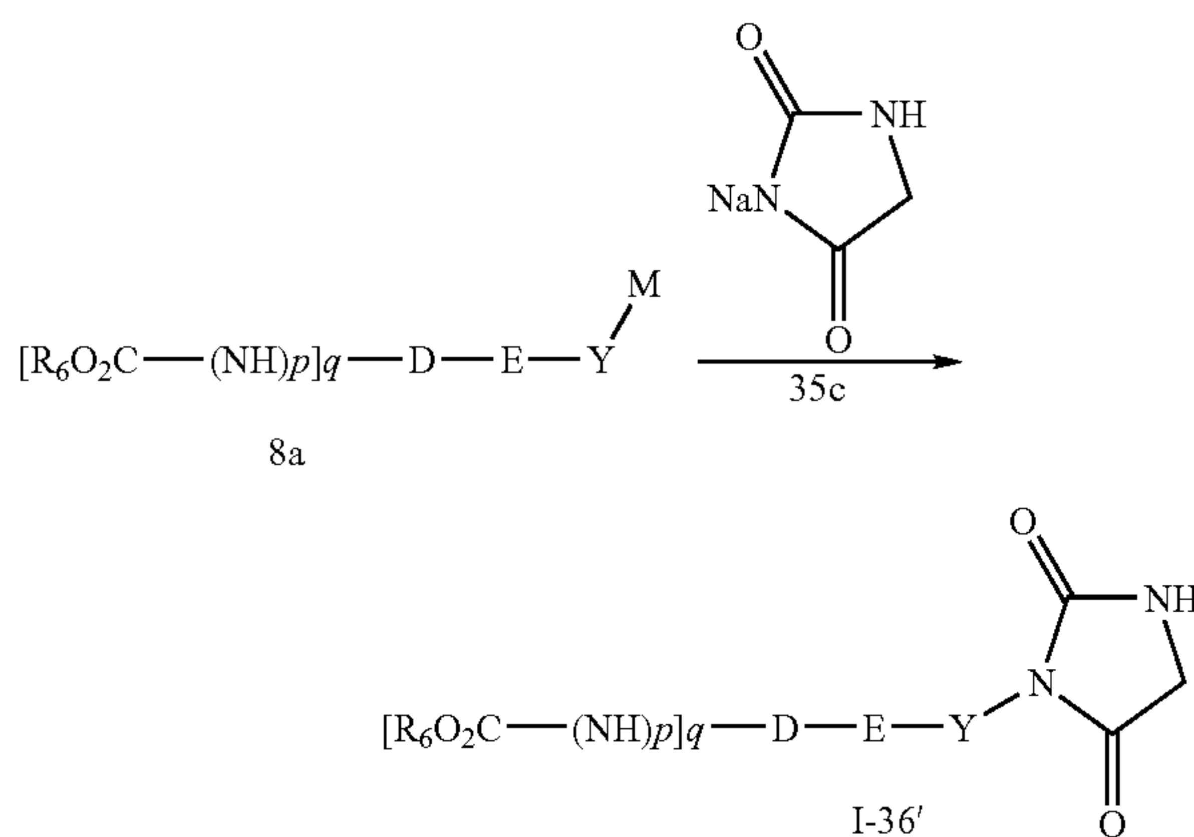
Scheme 6.2
