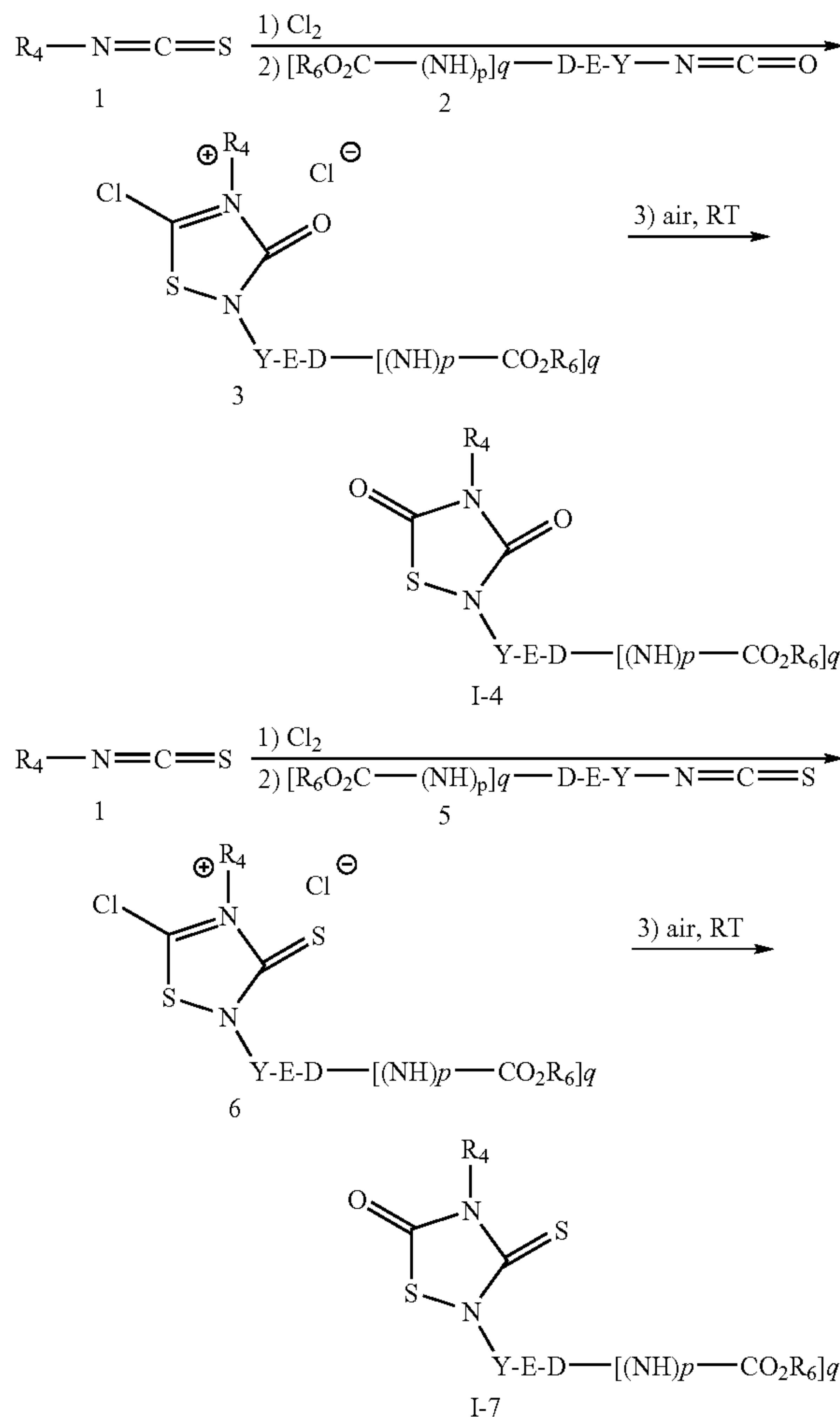
Scheme 1.1
