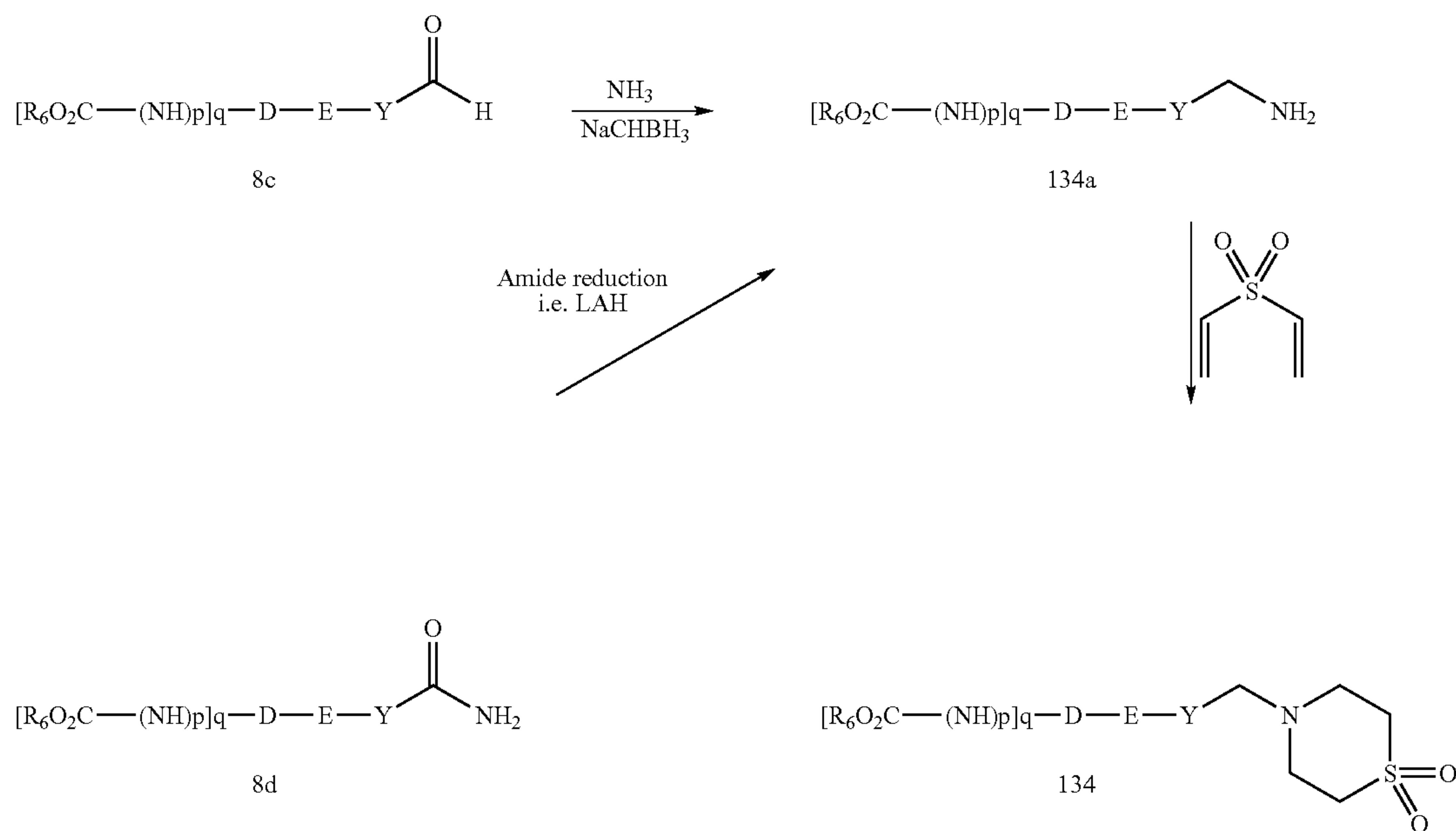
Scheme 21.1
