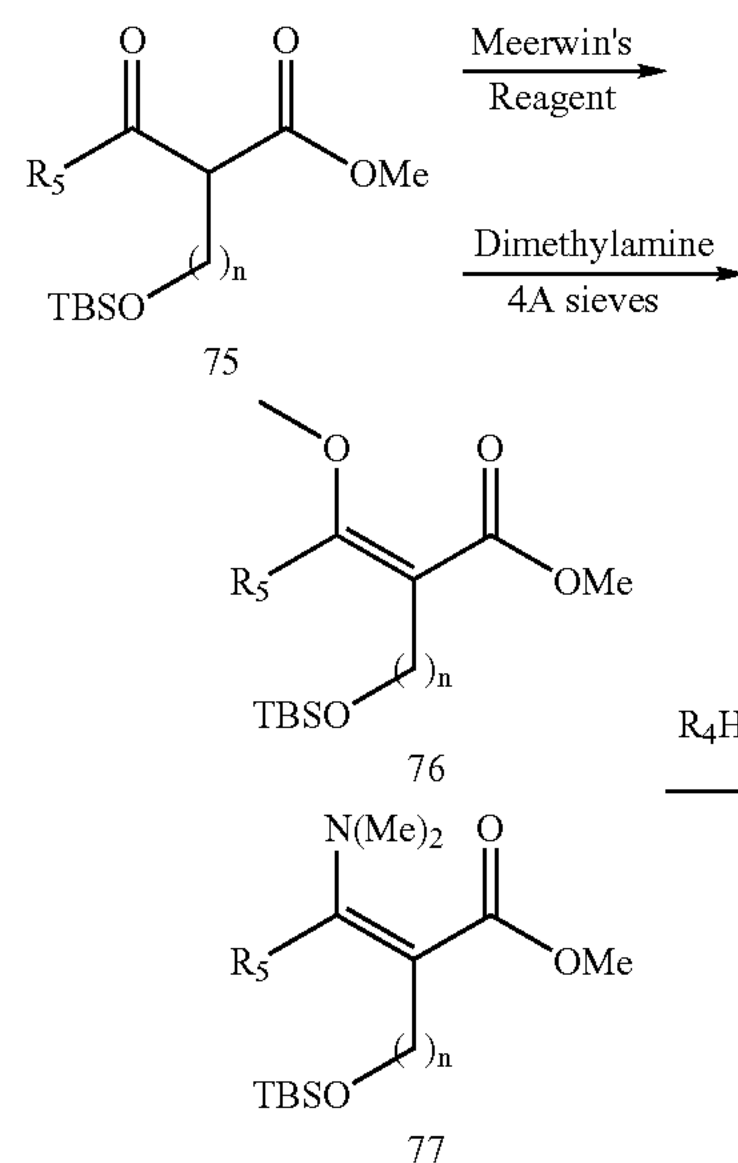
Scheme 13
