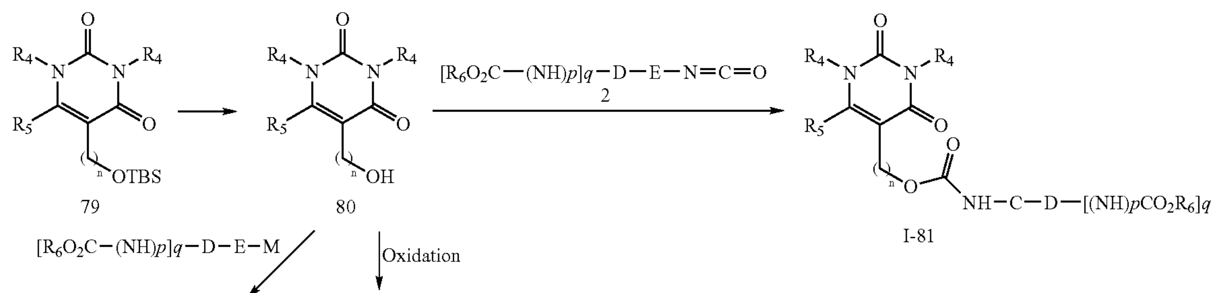
Scheme 14
