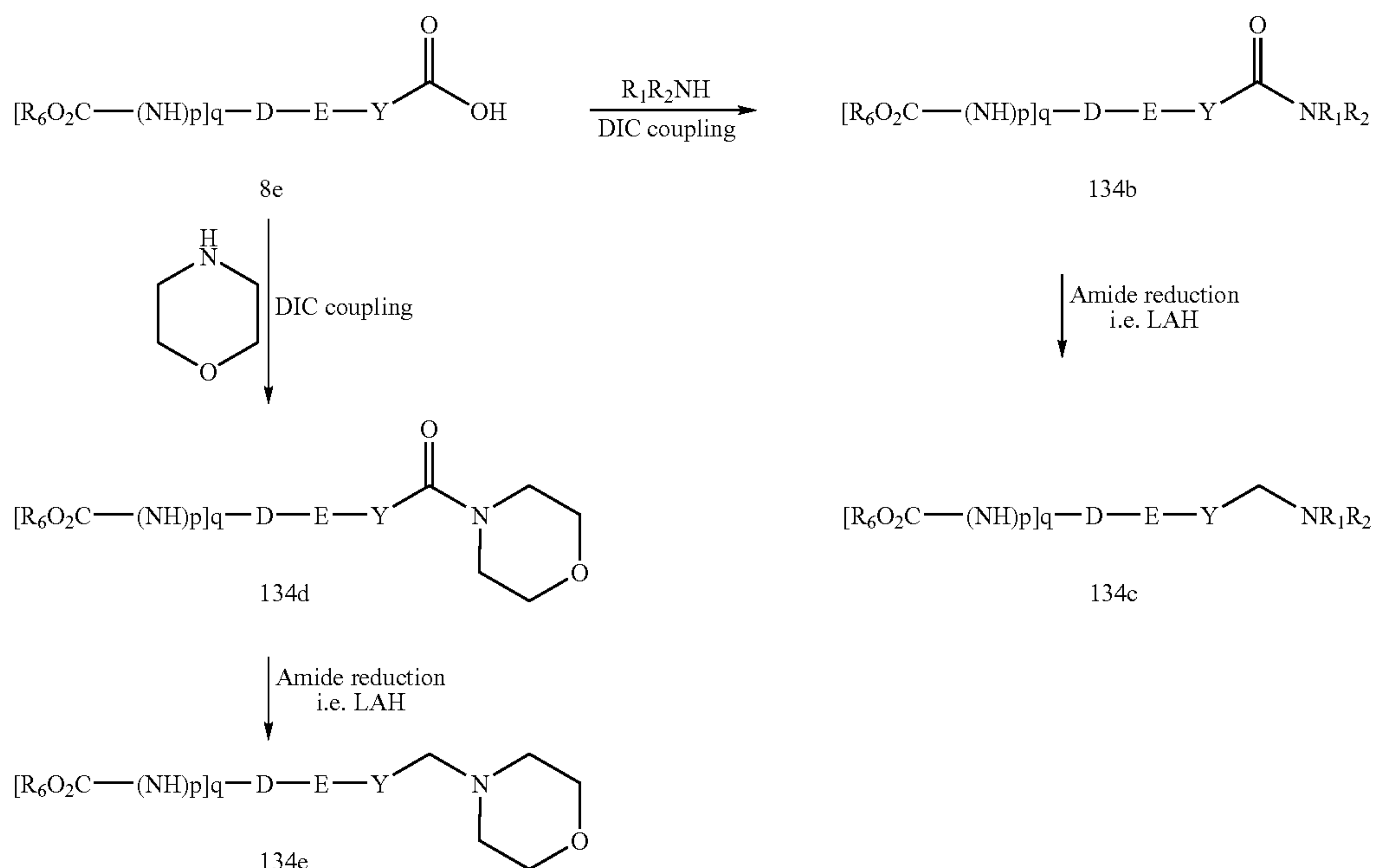
Scheme 21.2
