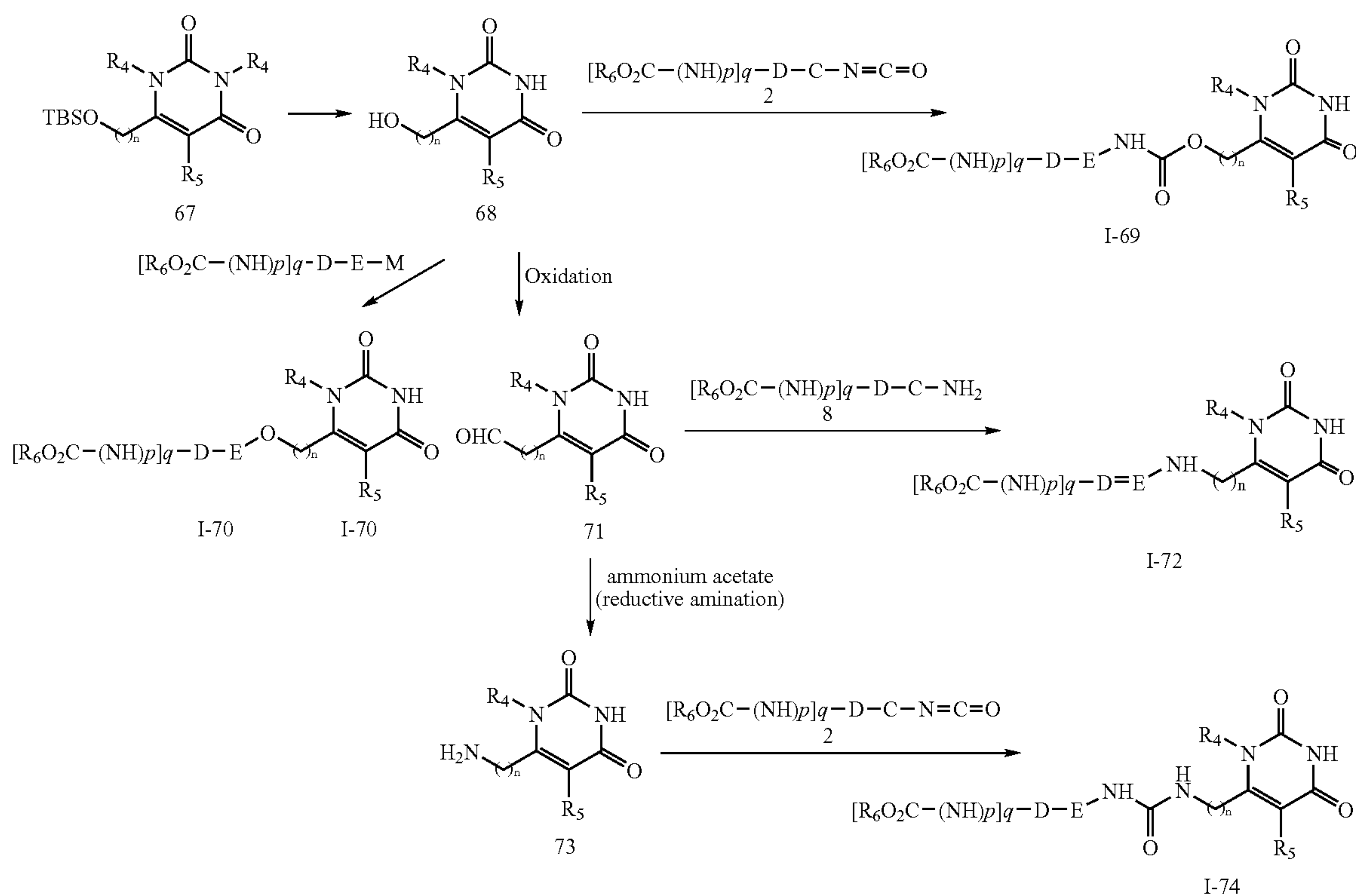
Scheme 12
