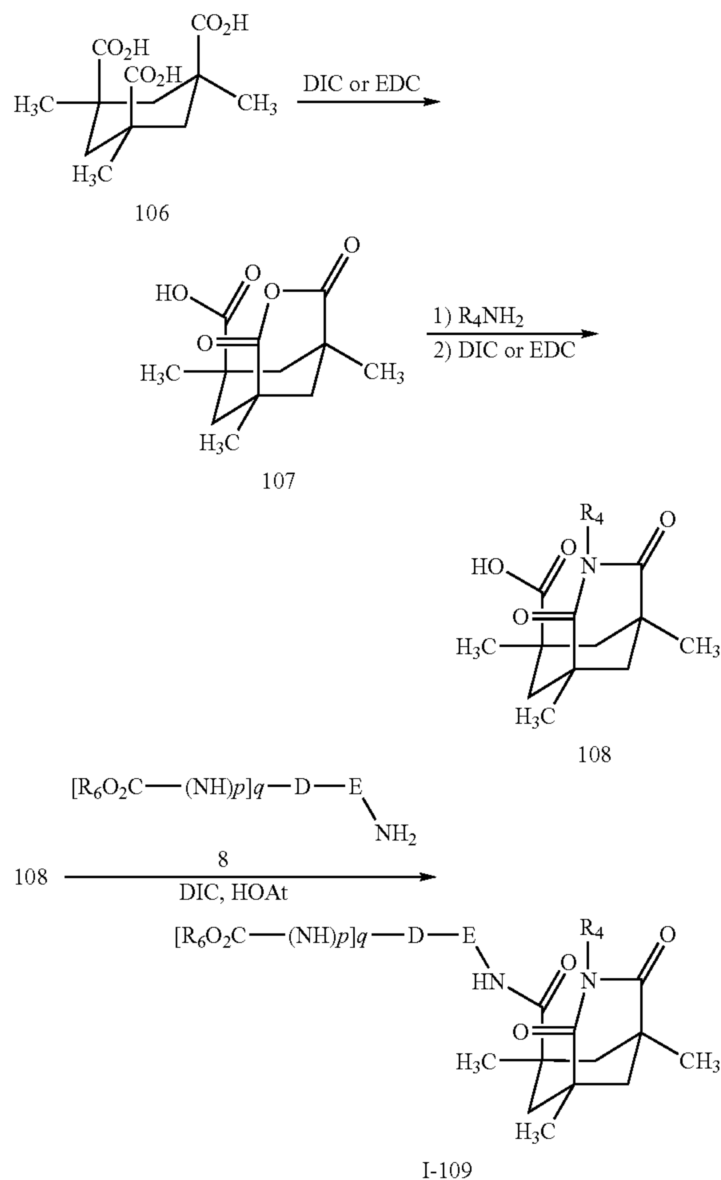
Scheme 18
