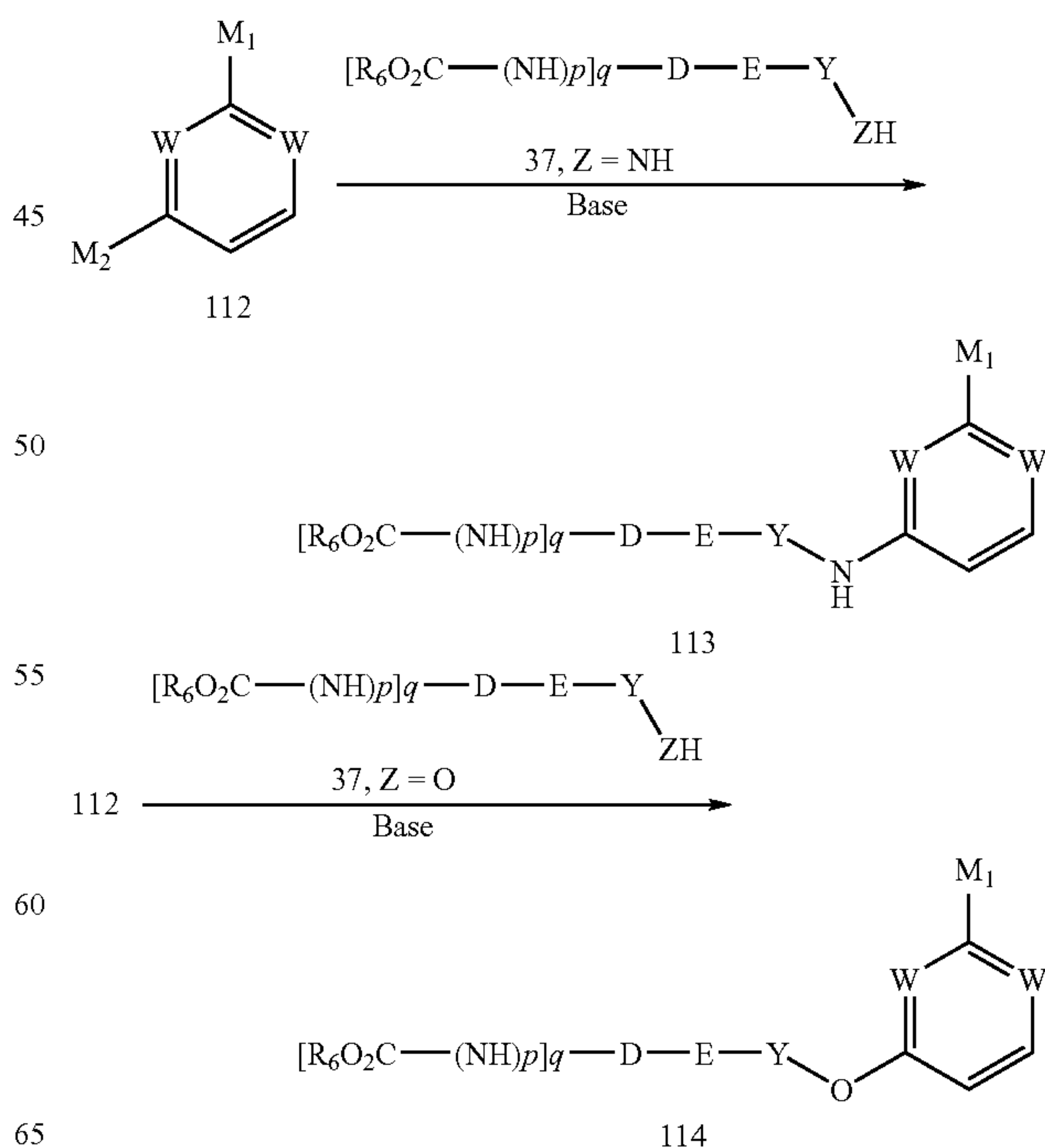
Scheme 19.1
