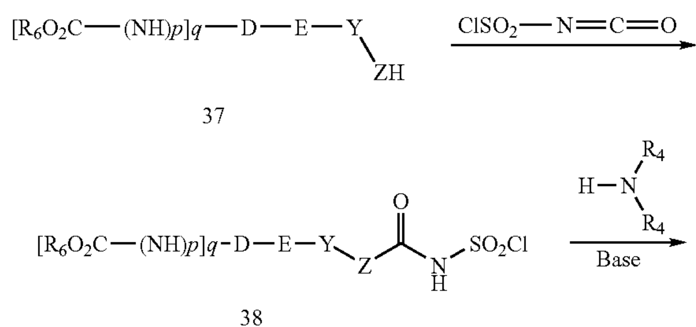
Scheme 7.1
