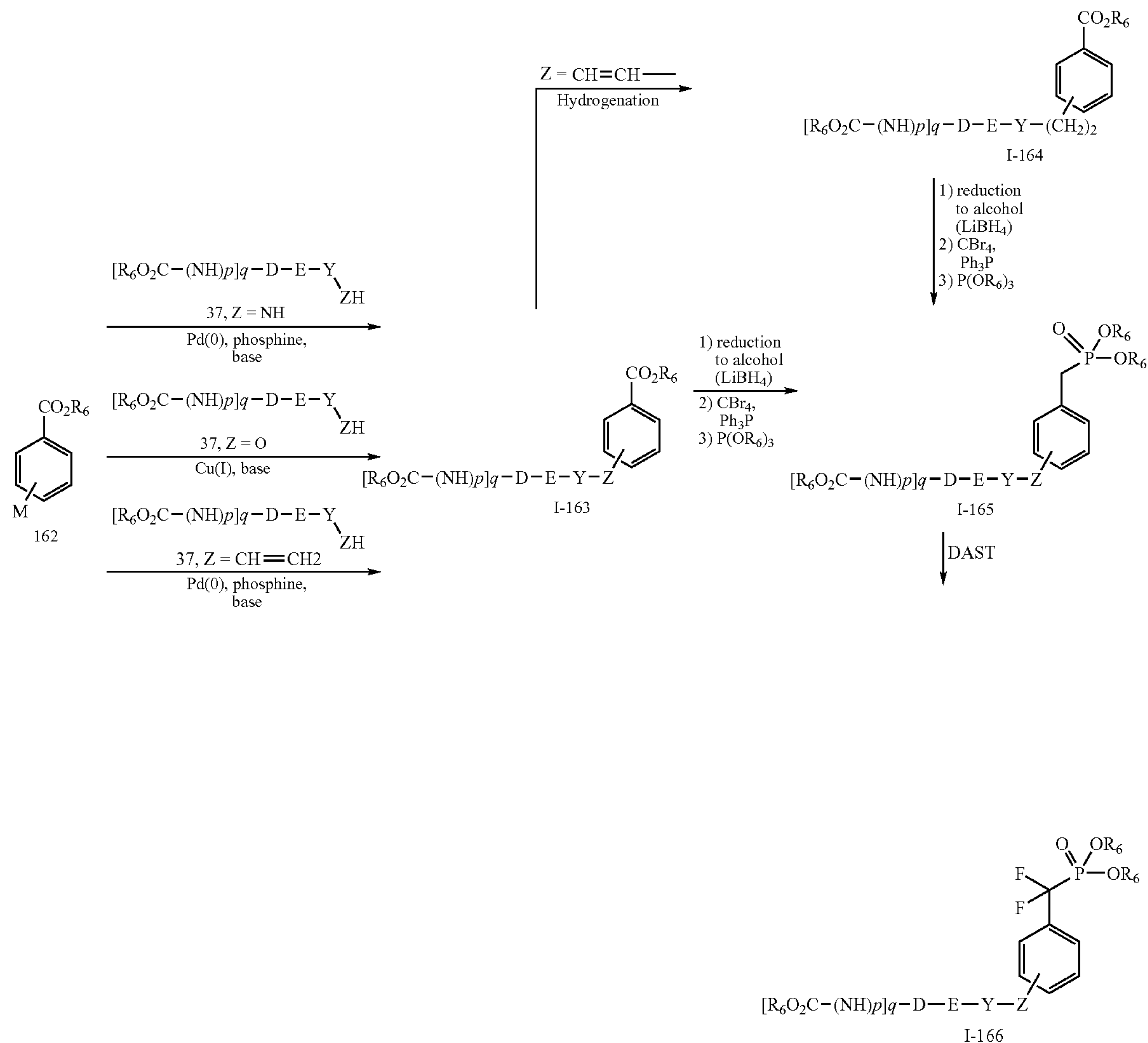
Scheme 26
