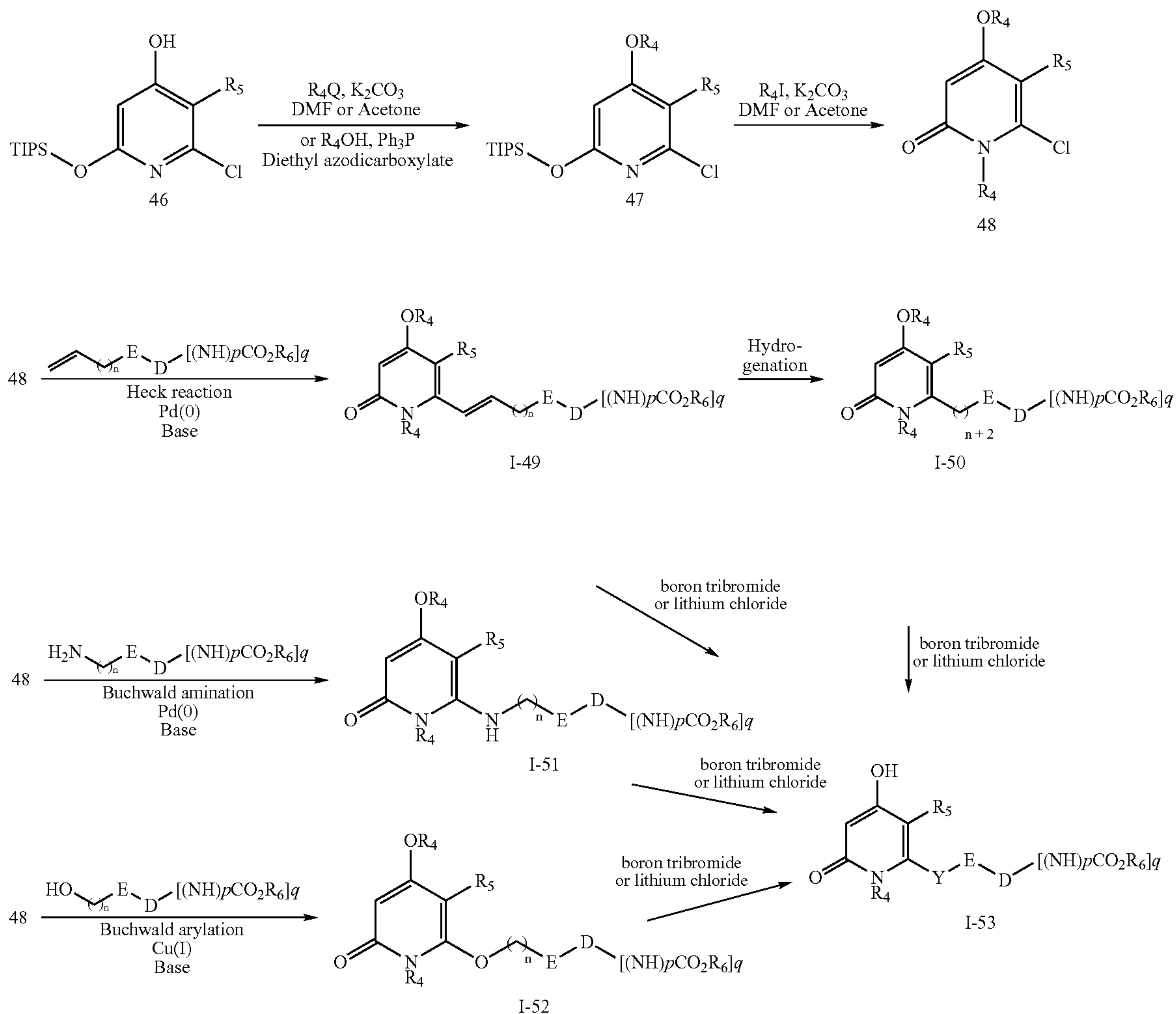
Scheme 9
