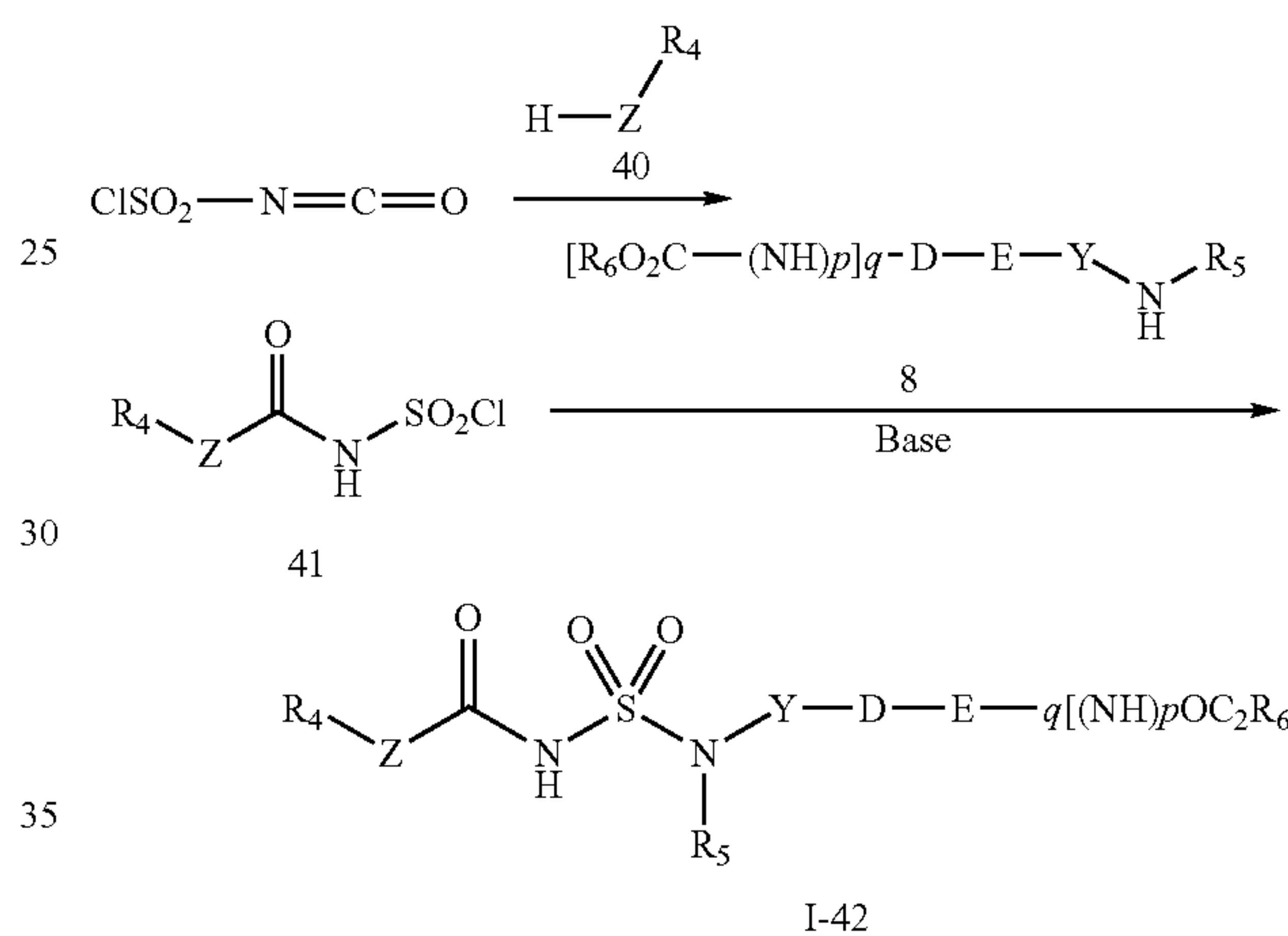
Scheme 7.2
