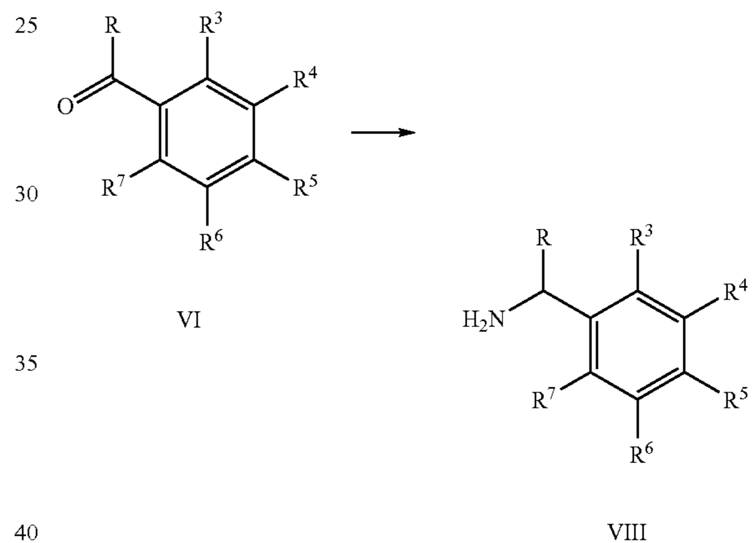
Reaction Scheme 3
