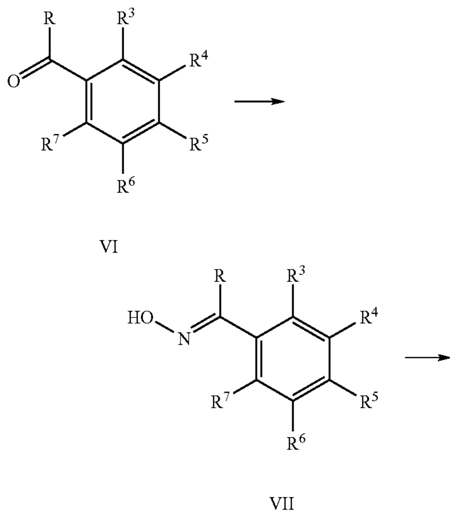
Reaction Scheme 2
