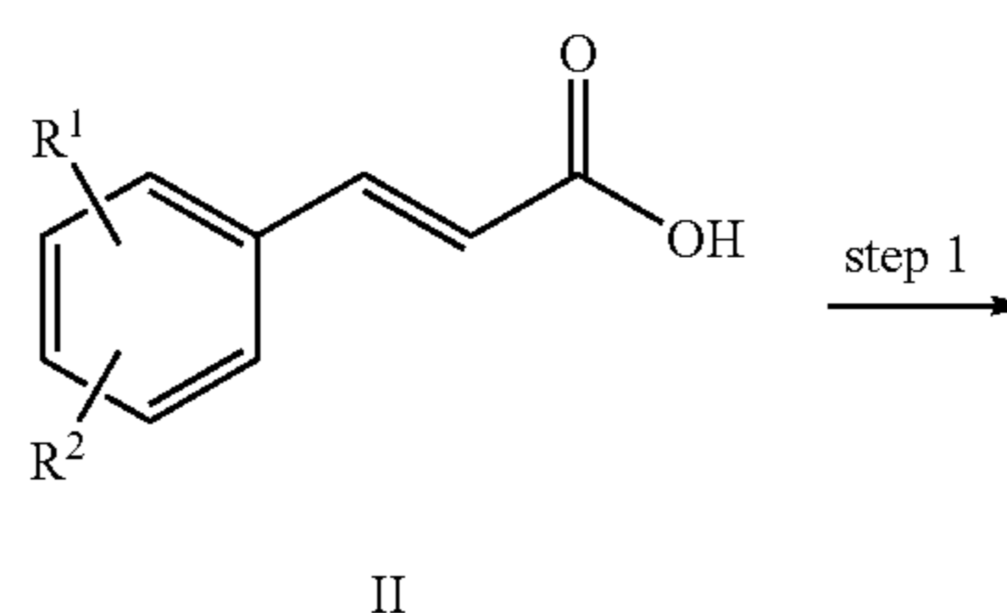
Reaction Scheme 1
