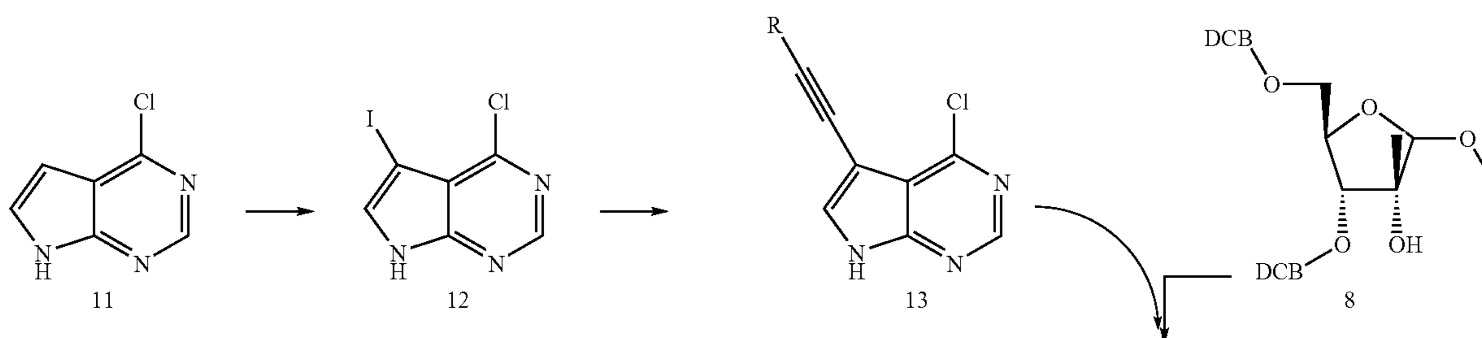
Scheme 3
