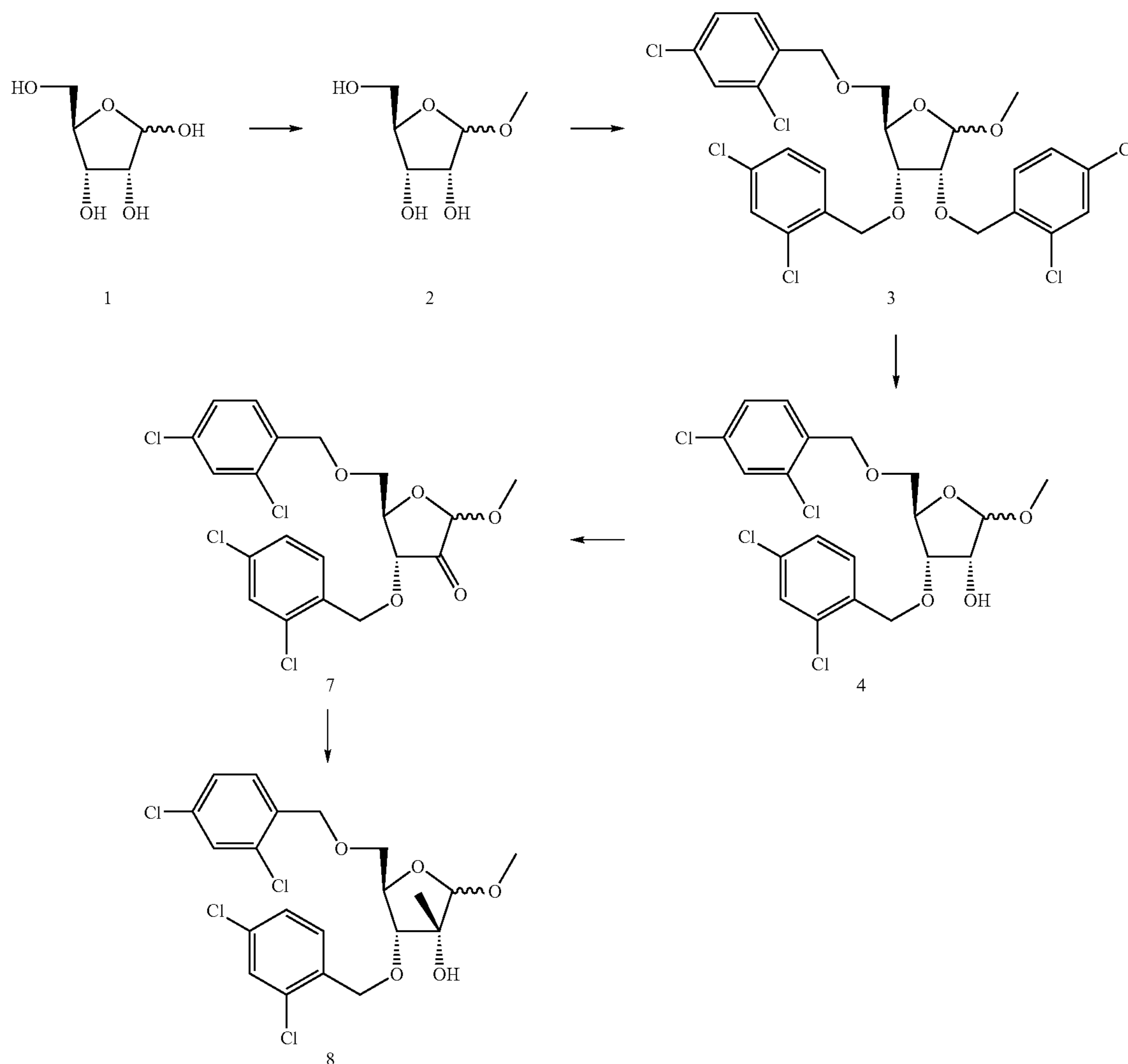
Scheme 2
