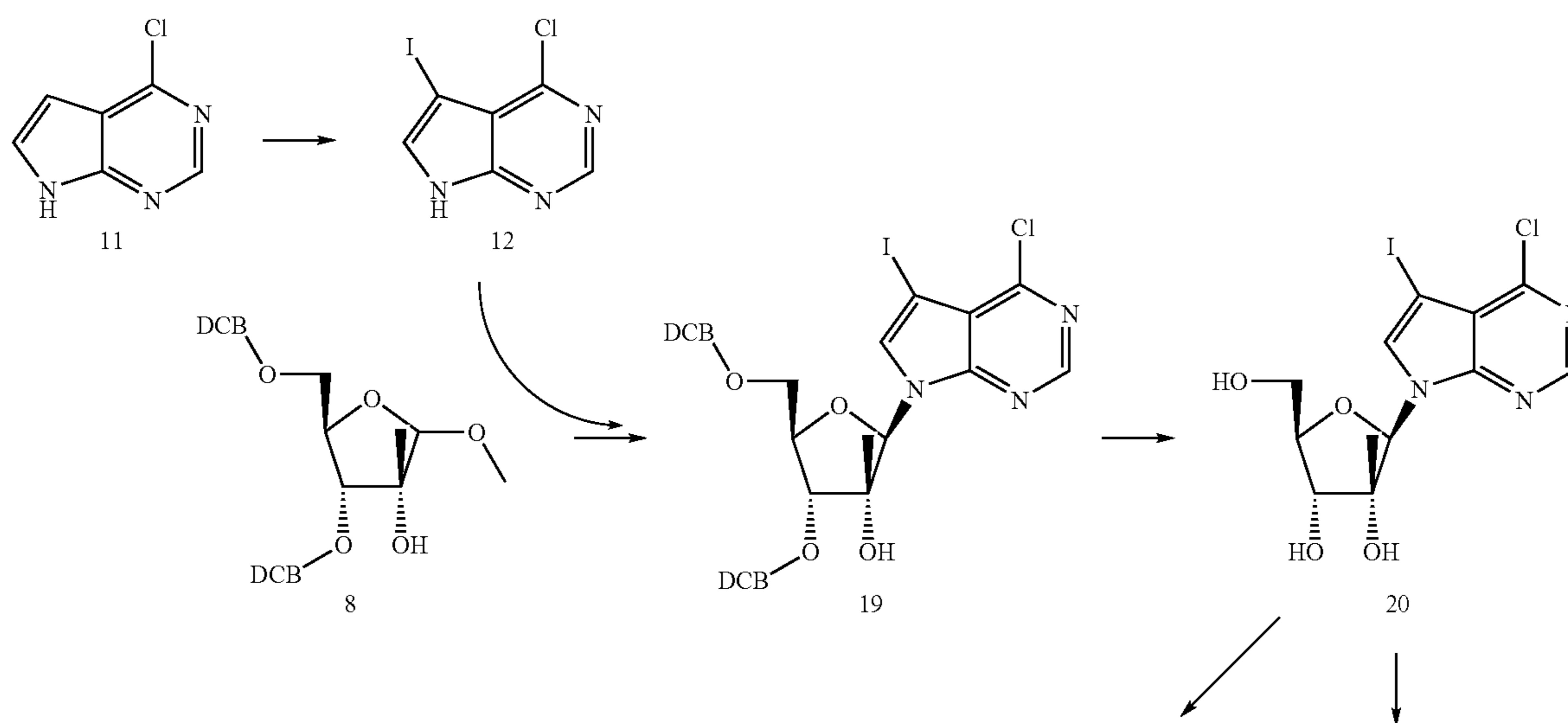
Scheme 4
