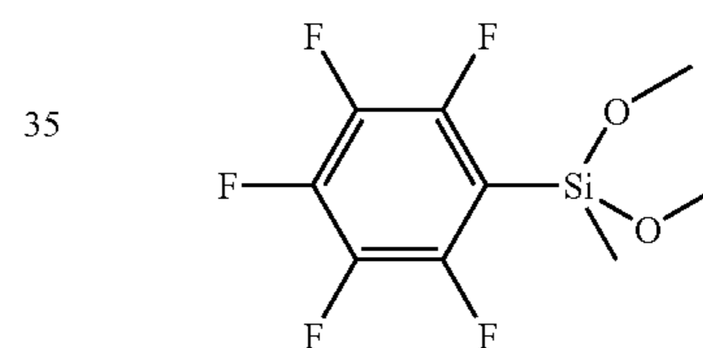
Methylpentafluorophenyl dimethoxy-silane
