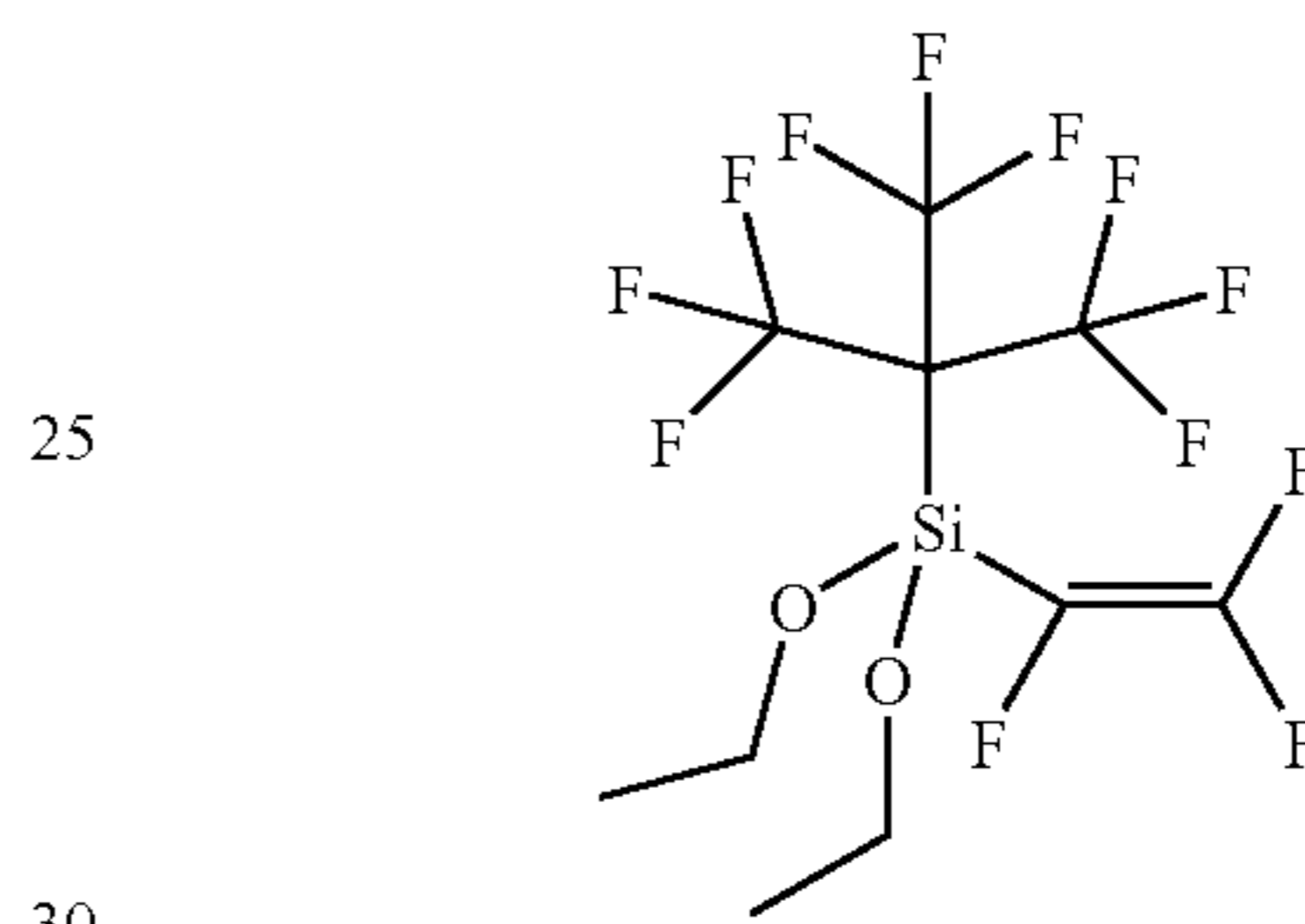
Perfluoro(t-butyl)trifluorovinyl-diethoxysilane
