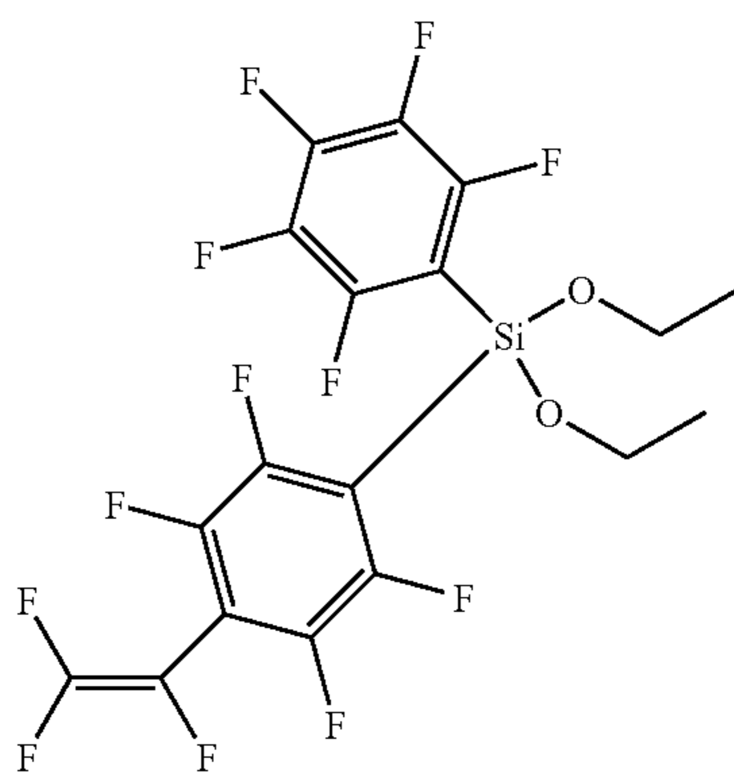
Pentafluorophenylperfluorostyryl-diethoxysilane
