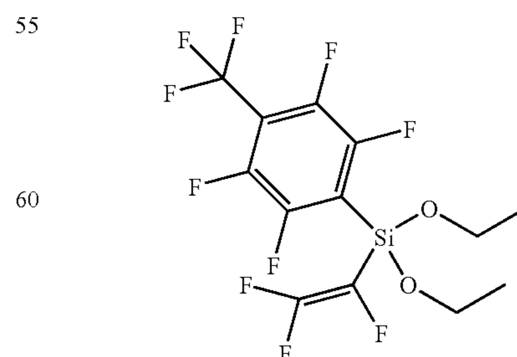
Perfluorotoluenetrifluorovinyl diethoxy-silane
