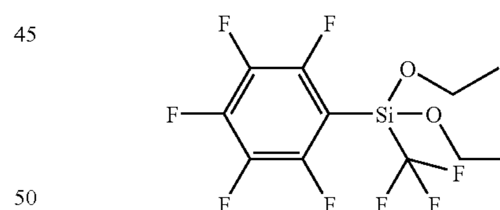
Pentafluorophenyltrifluoromethyl diethoxysilane
