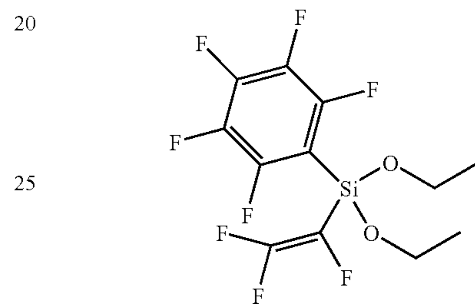
Pentafluorophenyltrifluorovinyl diethoxy-silane
