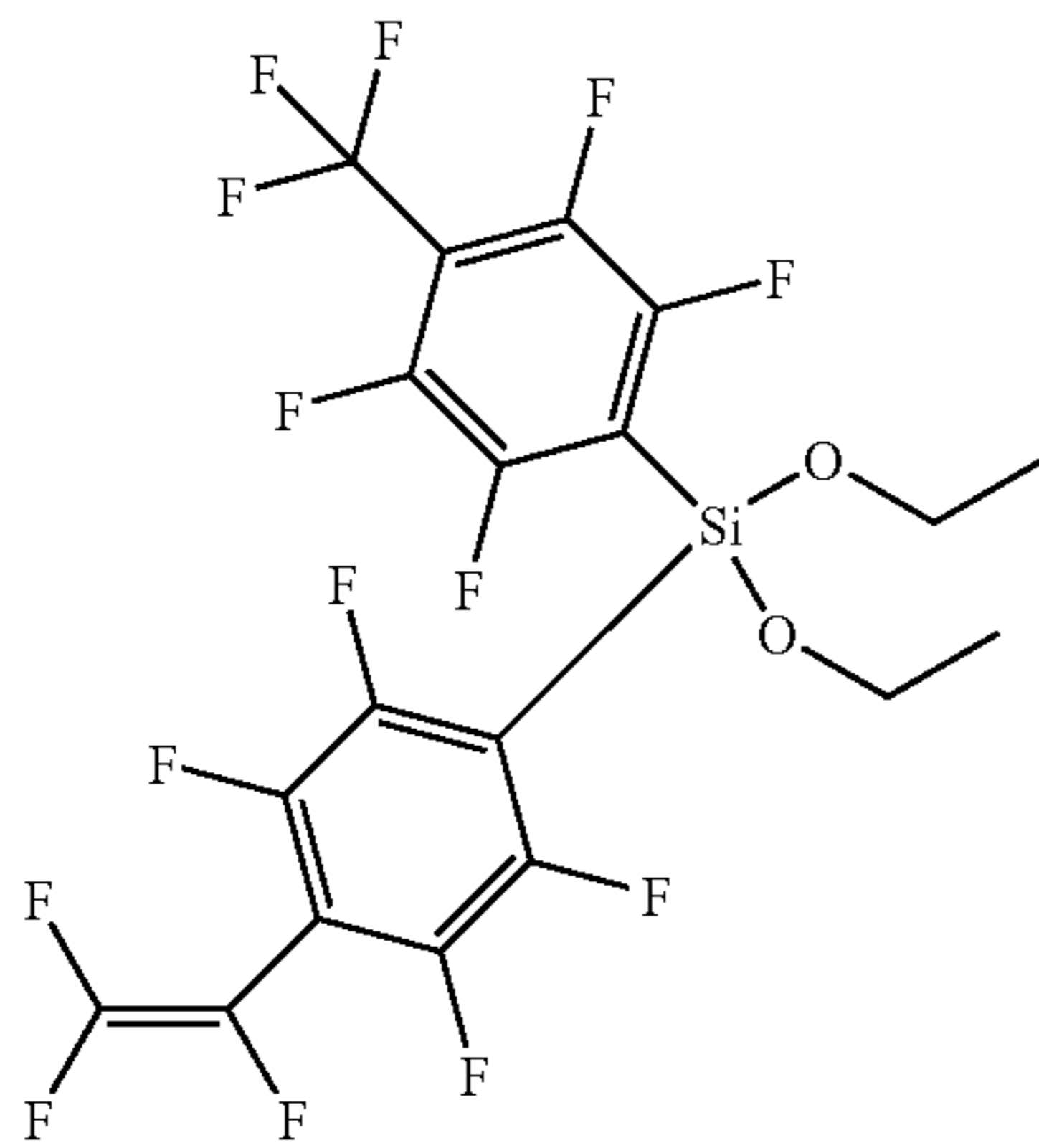
Perfluorostyreneperfluorotoluenediethoxysilane
