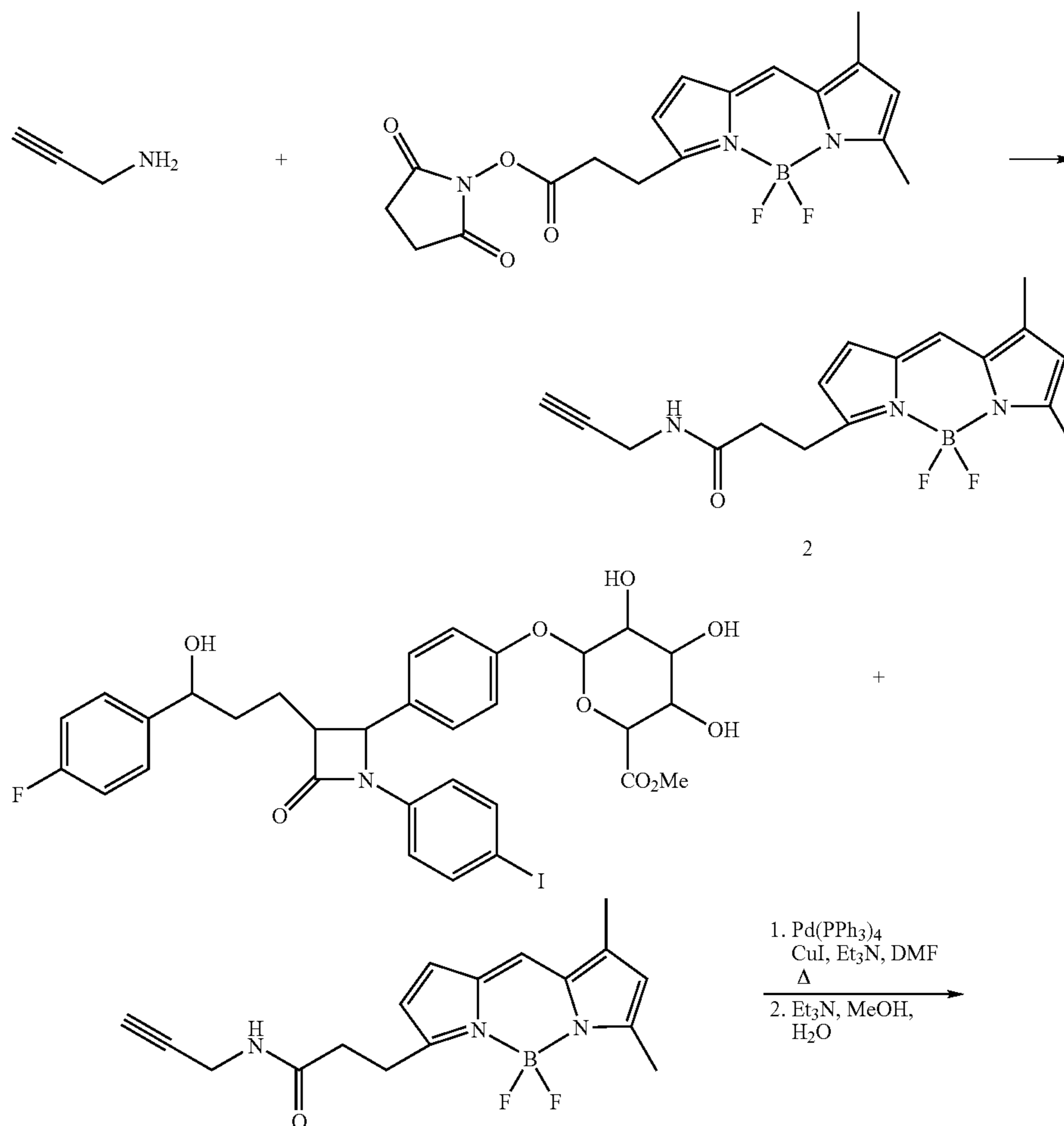
Scheme 1.
