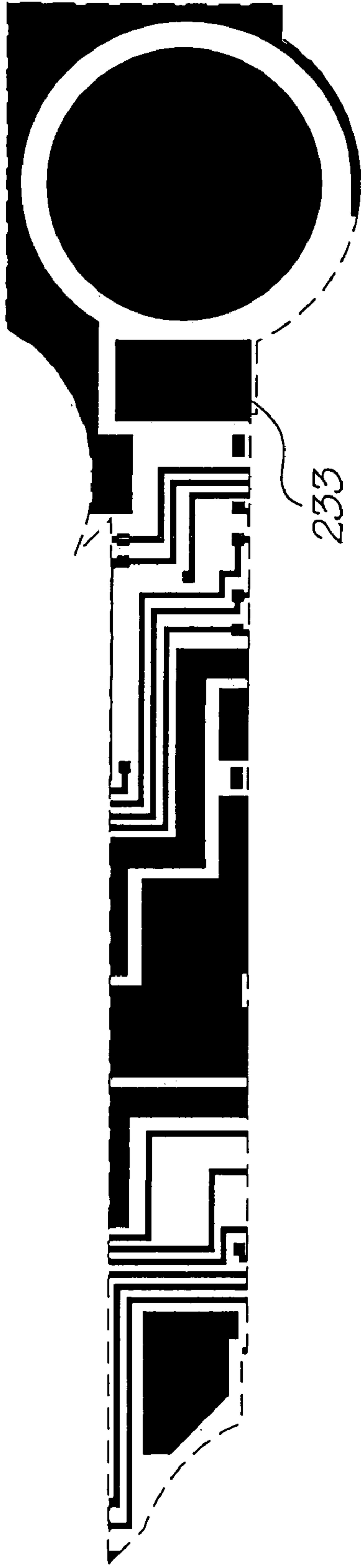
Metal 2 mask
