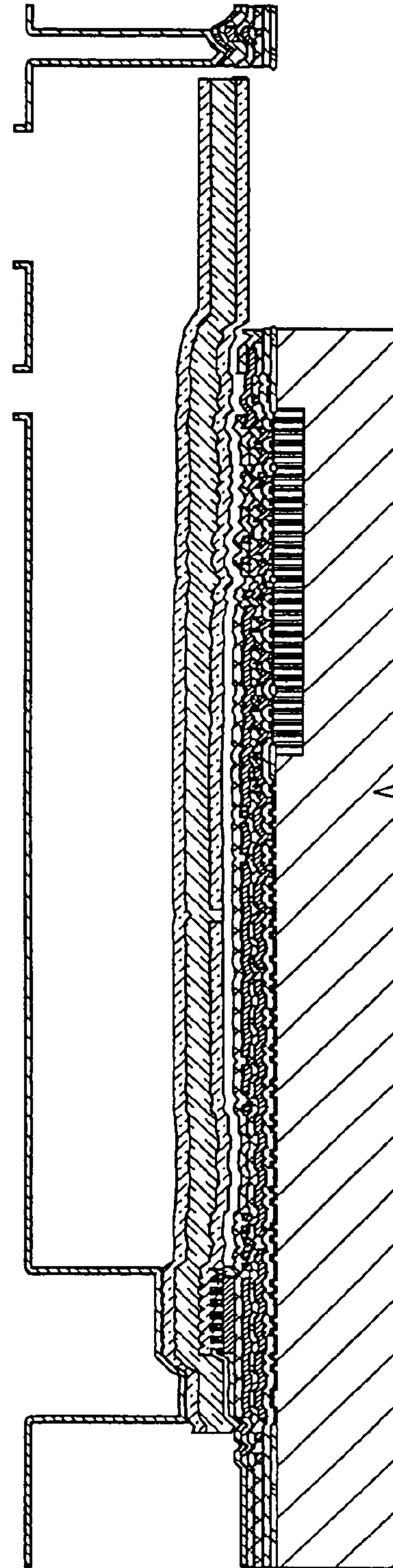
Detach from wafer blank, etch sacrificial material
