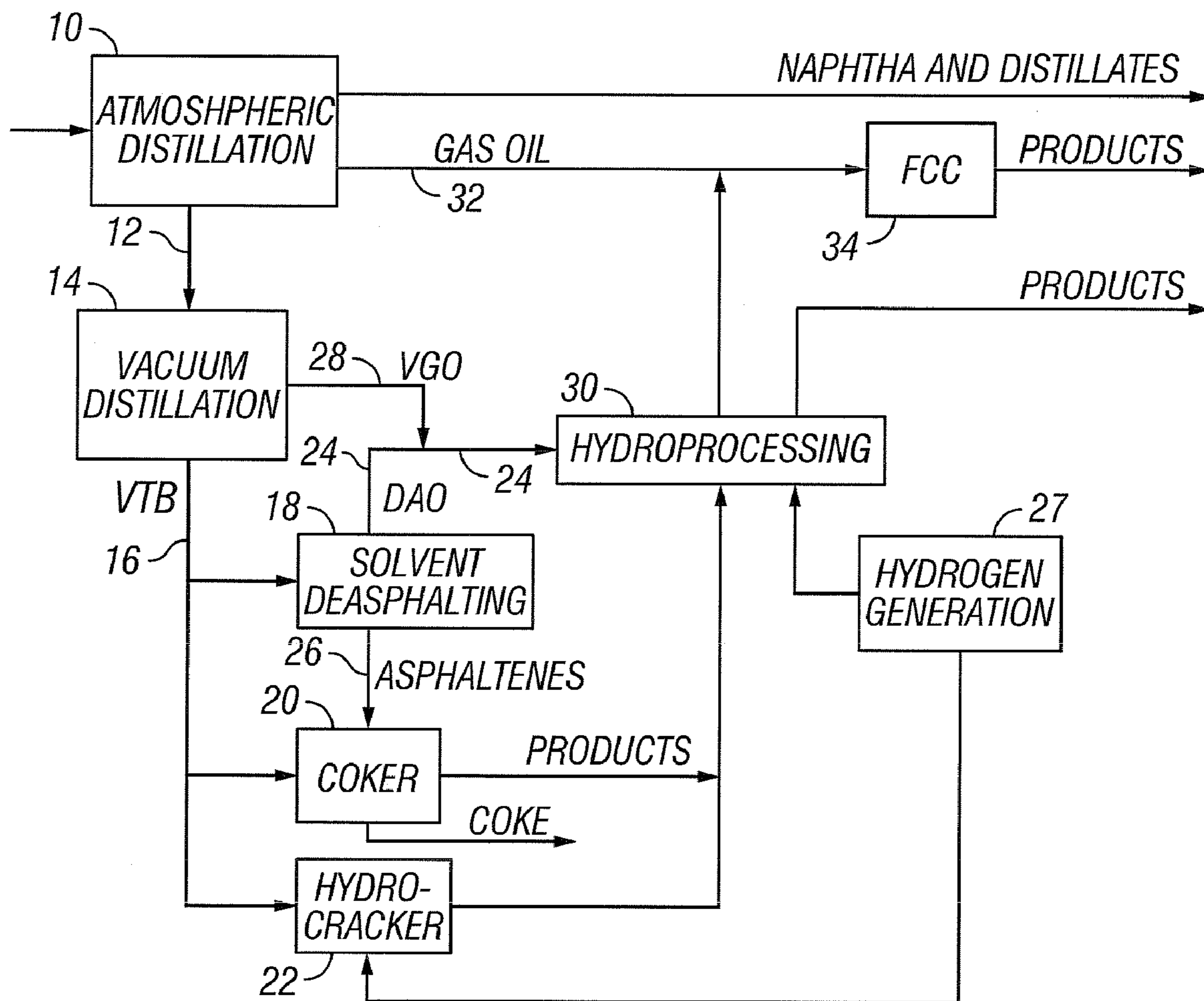
FIG. 1 (Prior Art)
