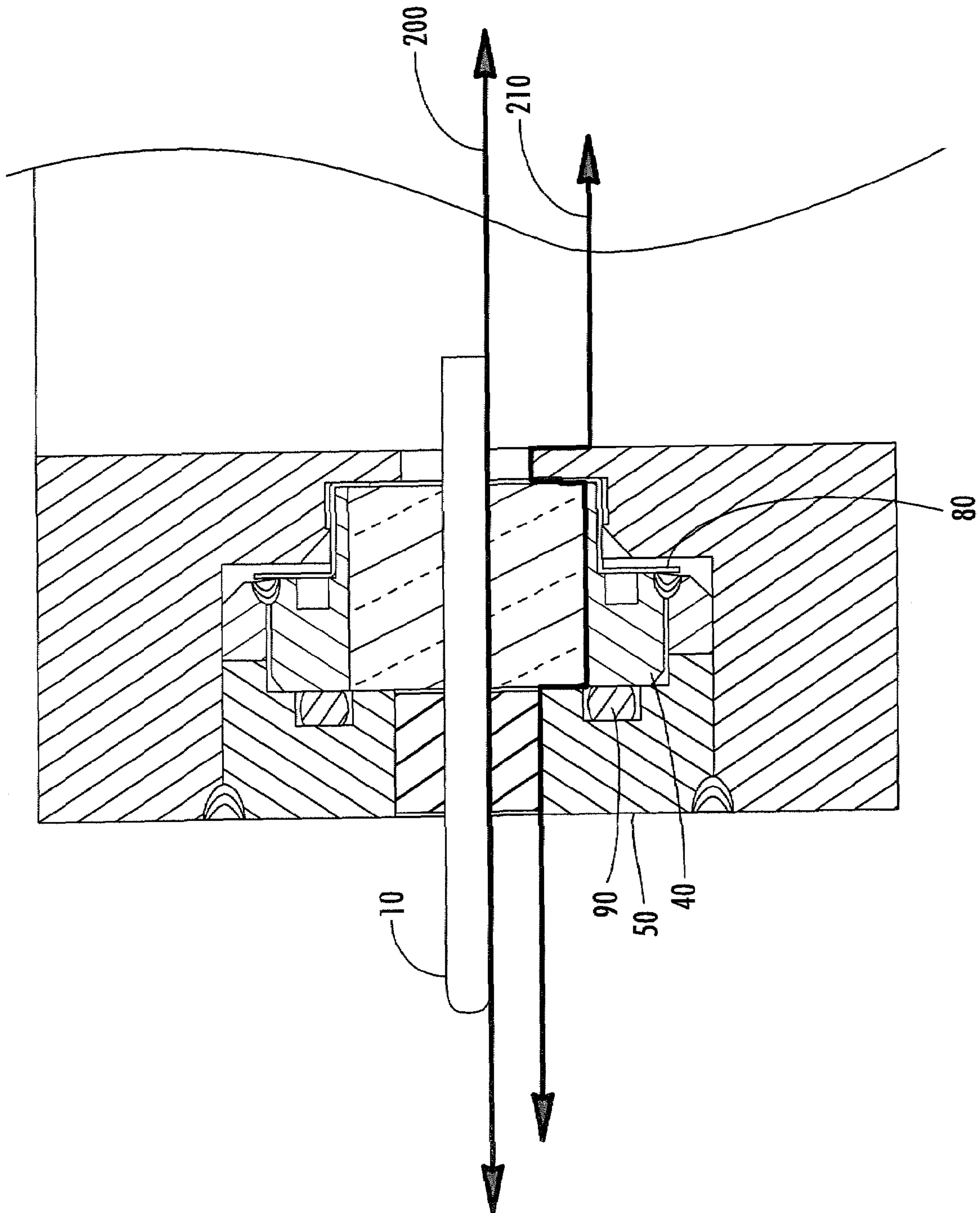
FIG. 2 (PRIOR ART)
