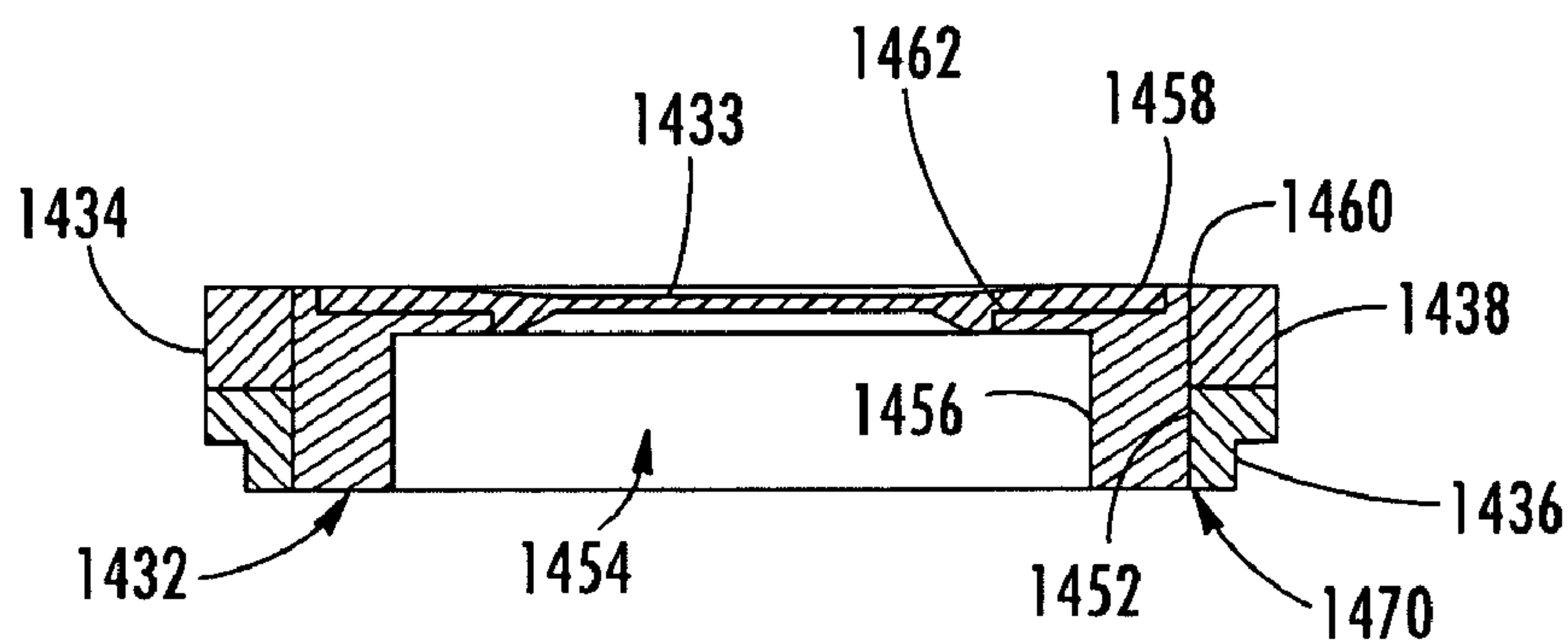
FIG. 14 (PRIOR ART)
