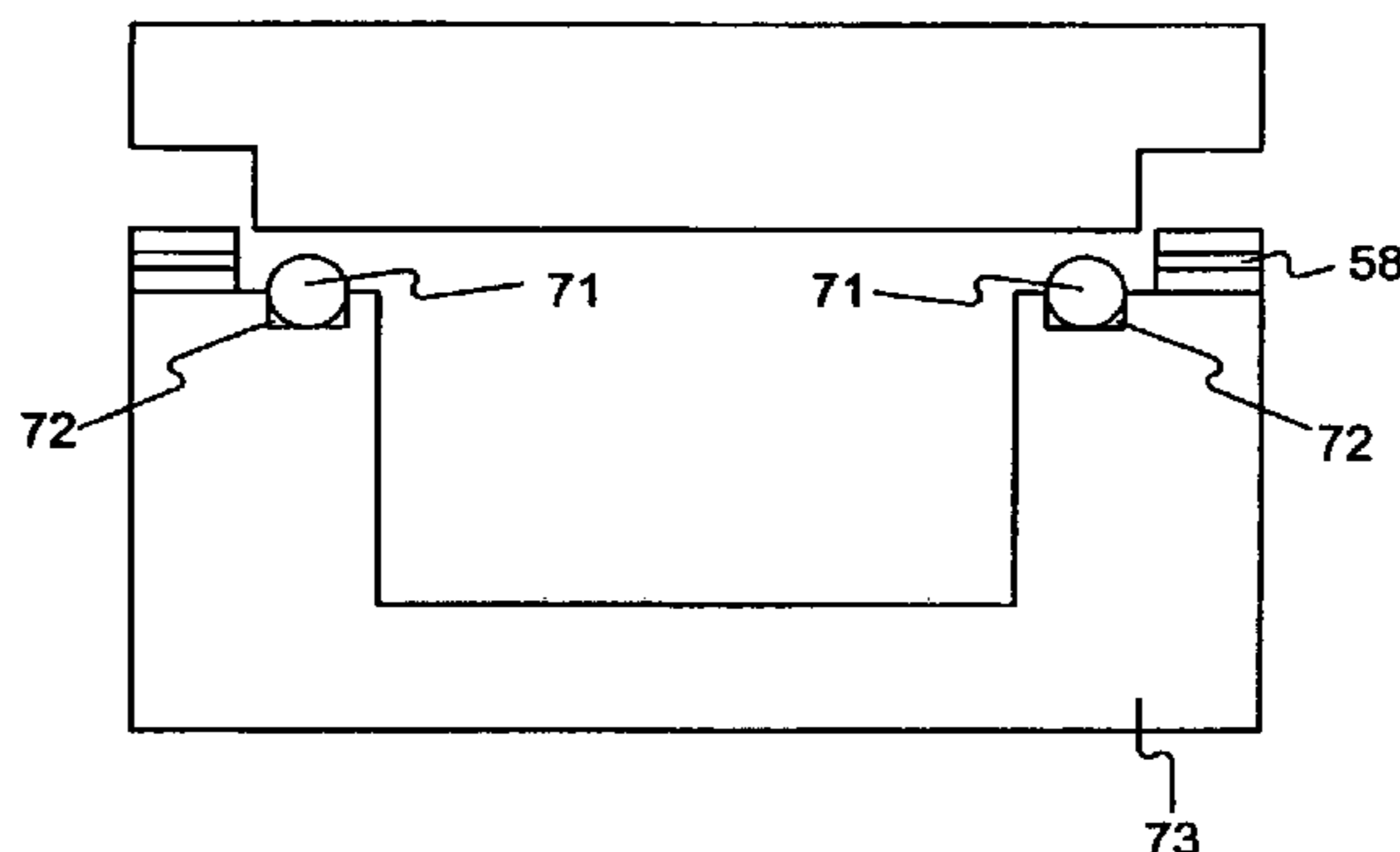
BEFORE JOINING
