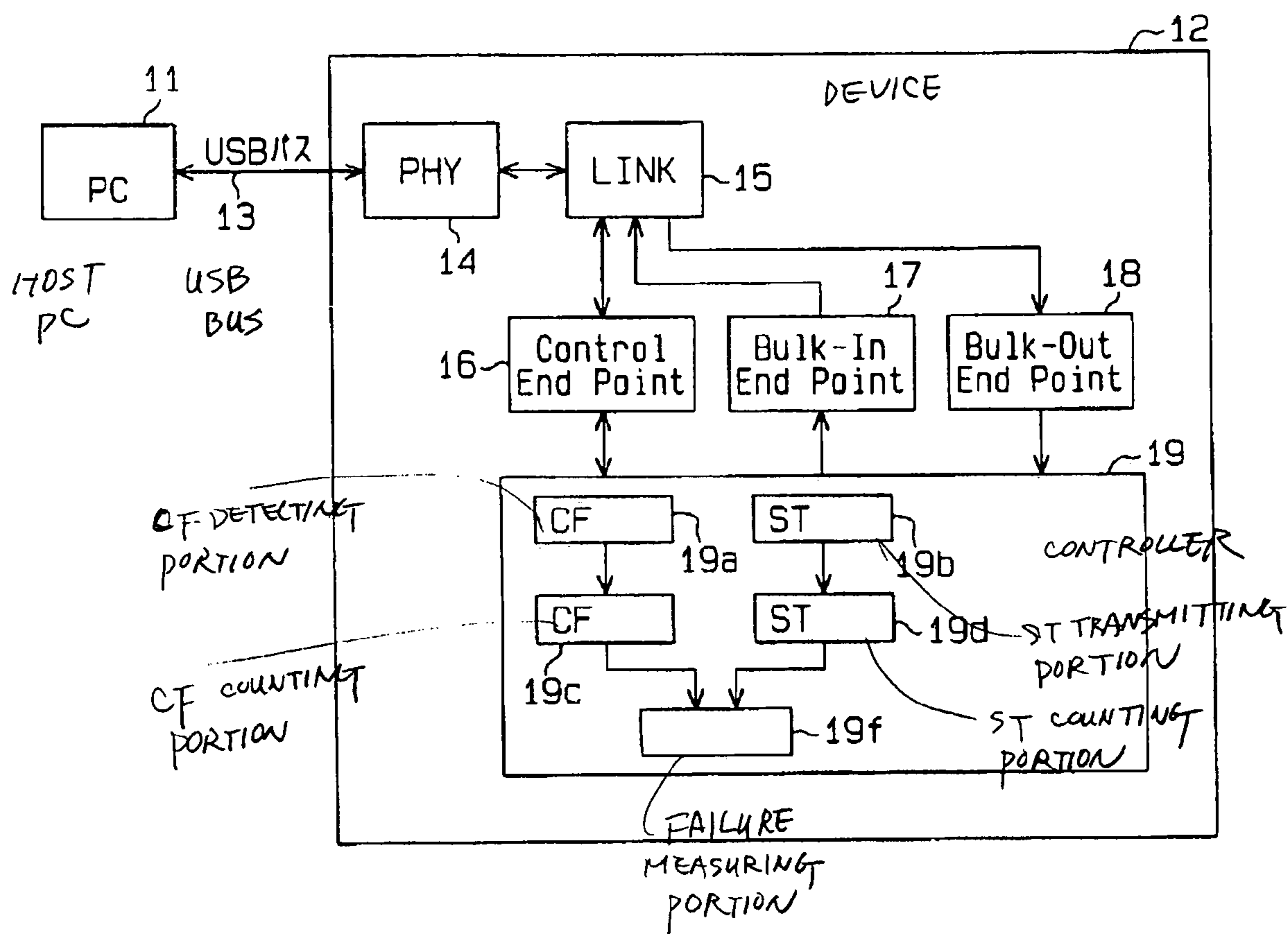
BLOCK DIAGRAM ILLUSTRATING THE THIRD EMBODIMENT
