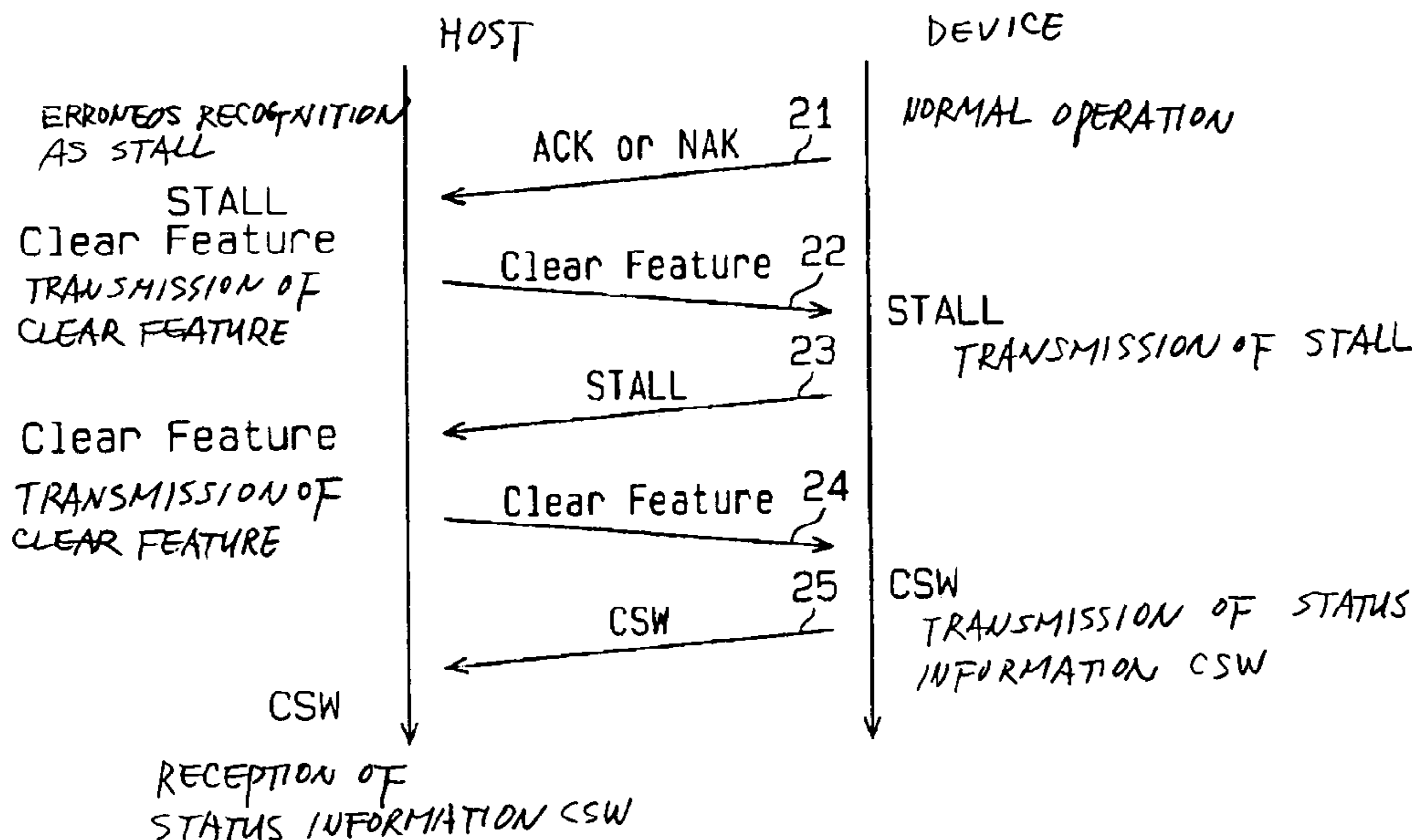
DIAGRAM FOR DESCRIBING OPERATIONS IN OCCURRENCE OF ERRONEOUS RECOGNITION
