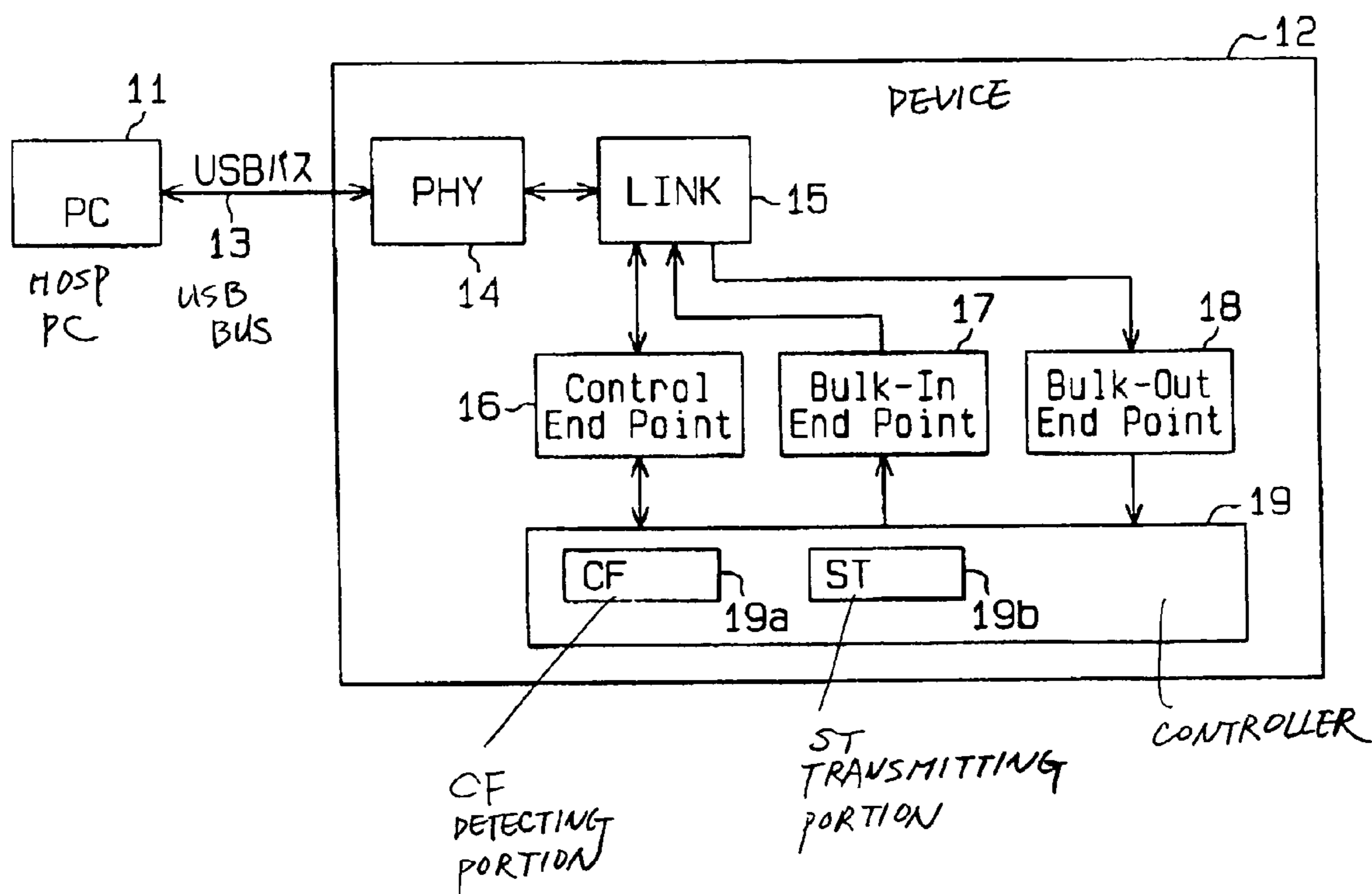
BLOCK DIAGRAM ILLUSTRATING THE FIRST EMBODIMENT
