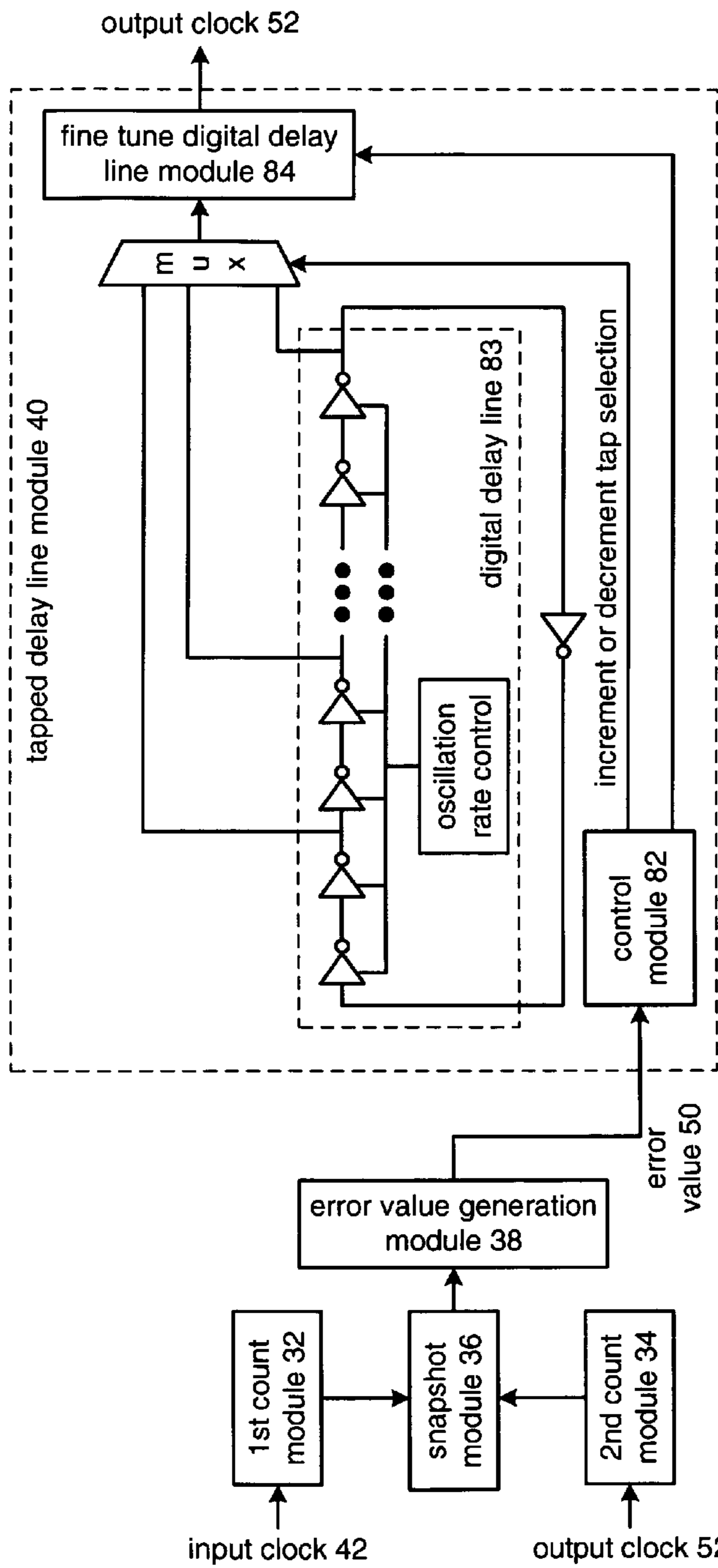
FIG. 6 CLK_{OUT} = (M/D) * CLK_{IN}
