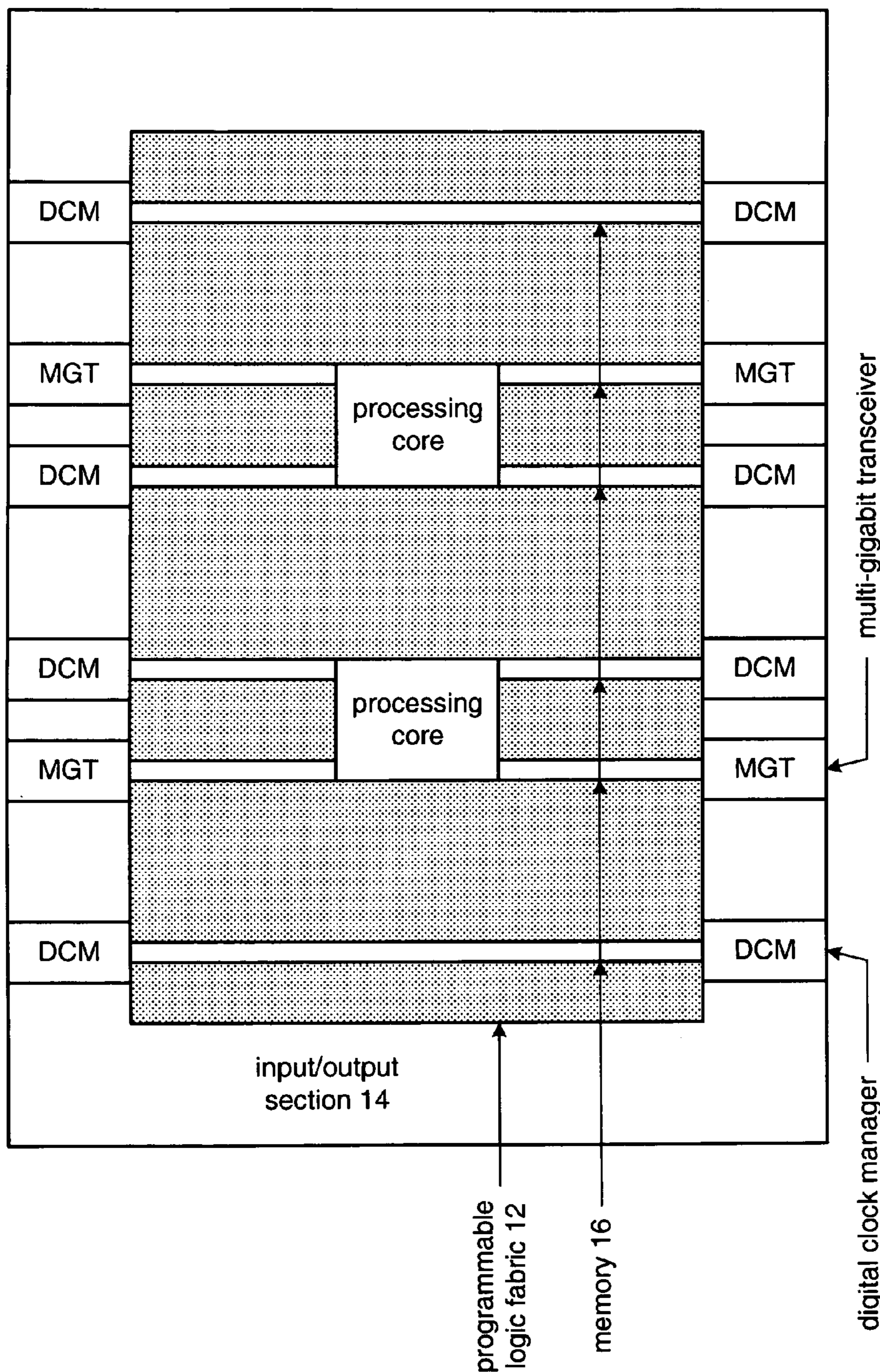
FIG. 3 programmable logic device 10
