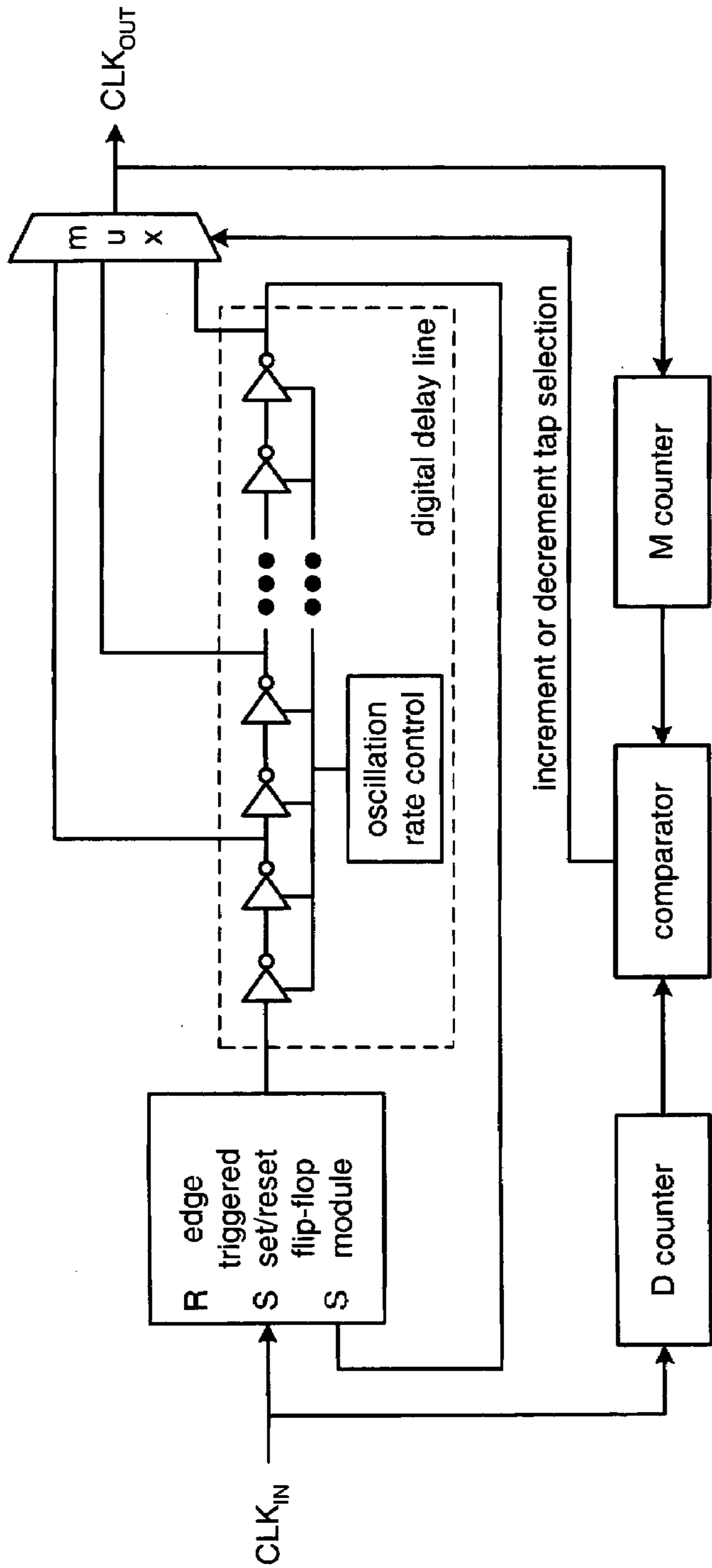
FIG. 1 - Prior Art
