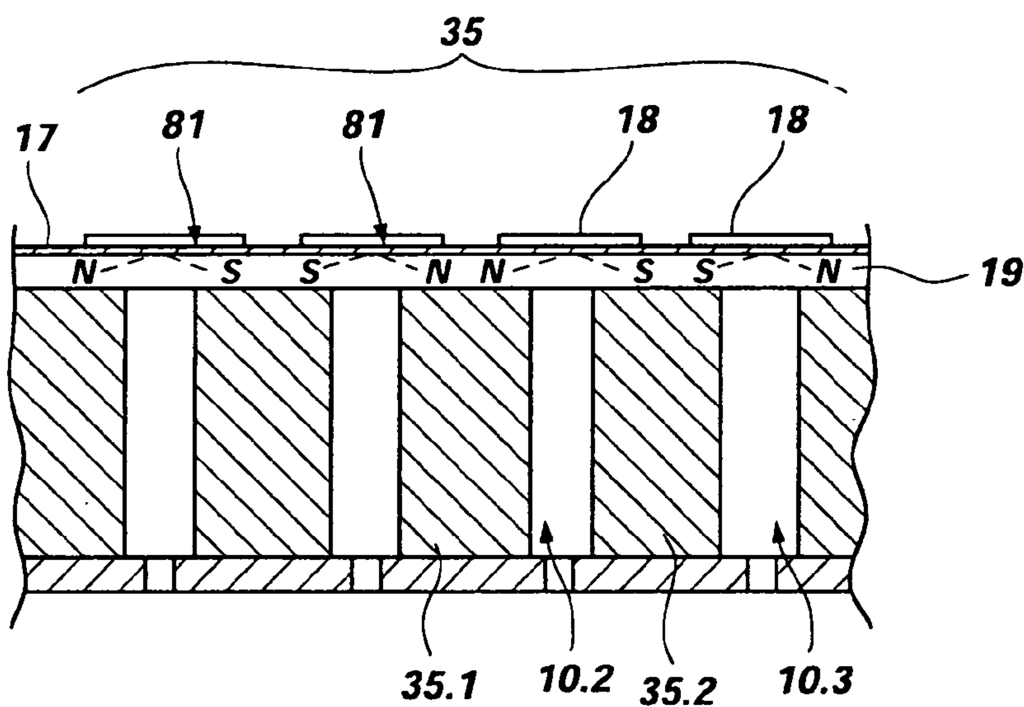
Fig. 2 (PRIOR ART)
