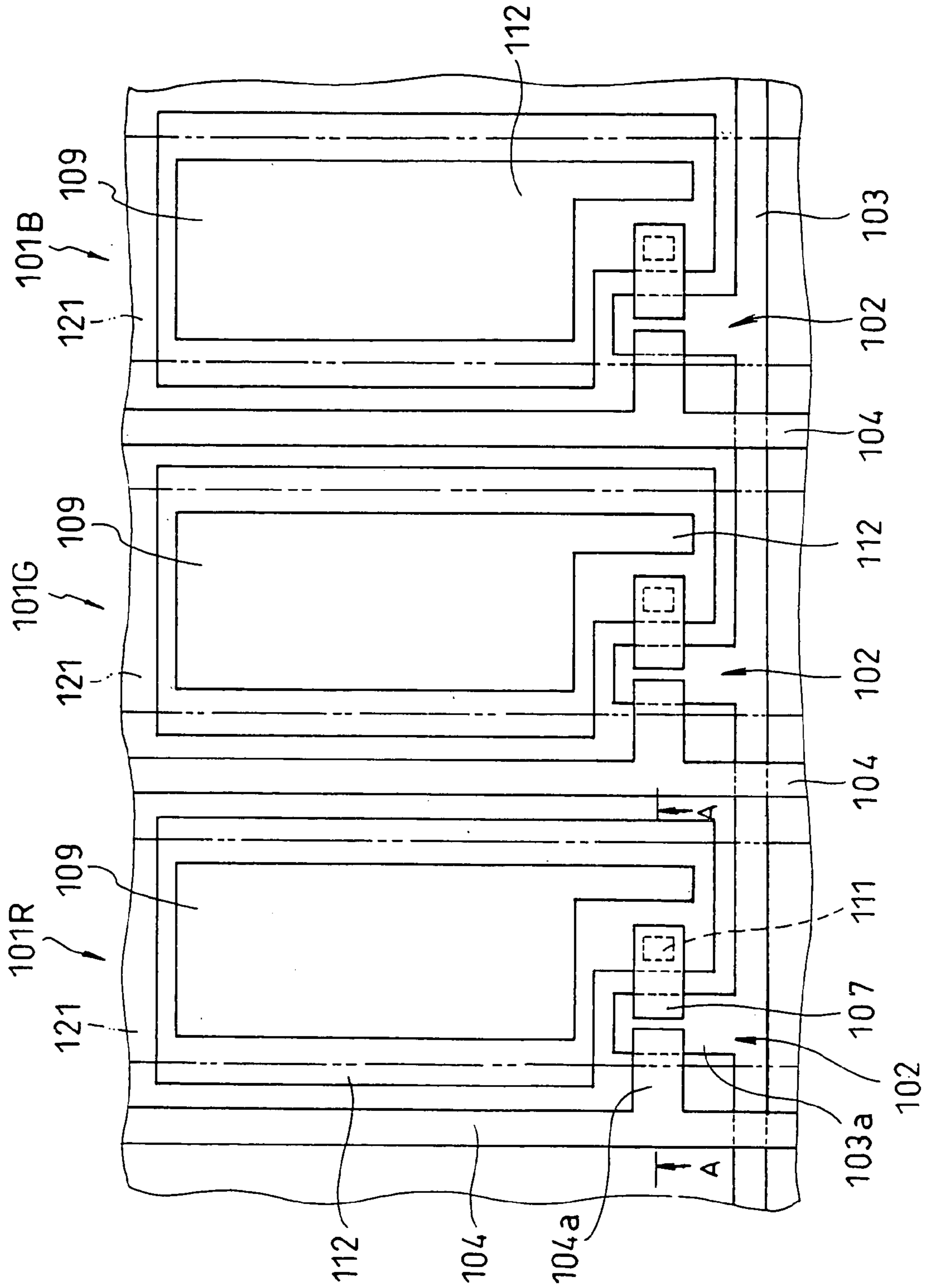
FIG. 1 (PRIOR ART)
