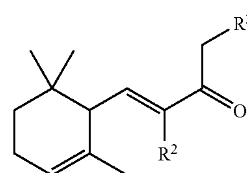
\alpha -Isomer
