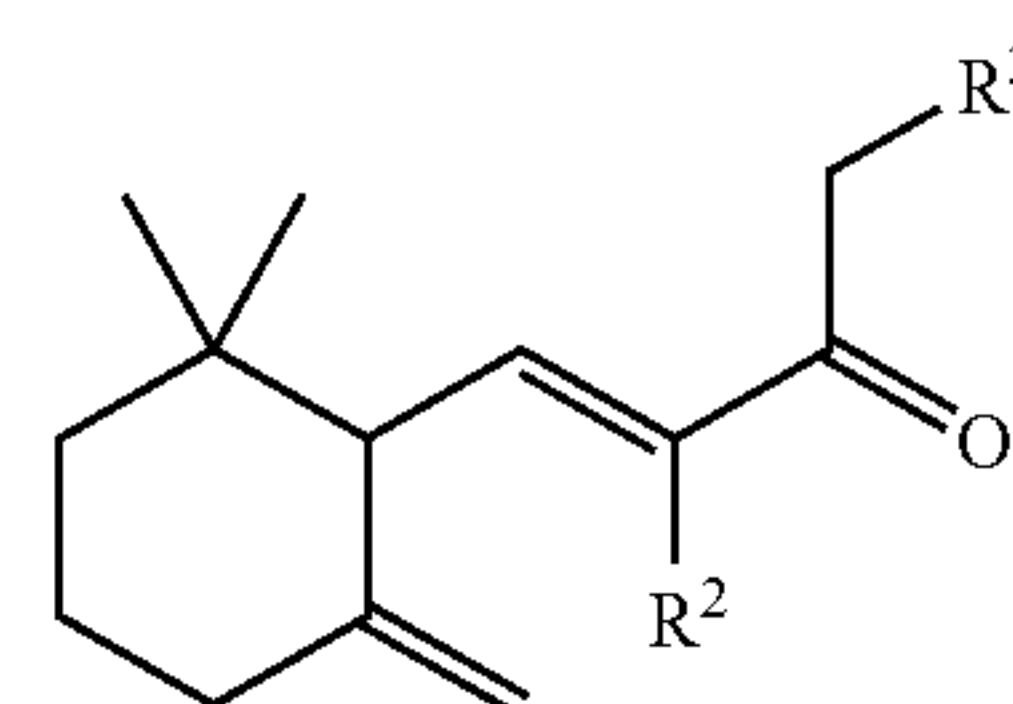
\gamma -Isomer
