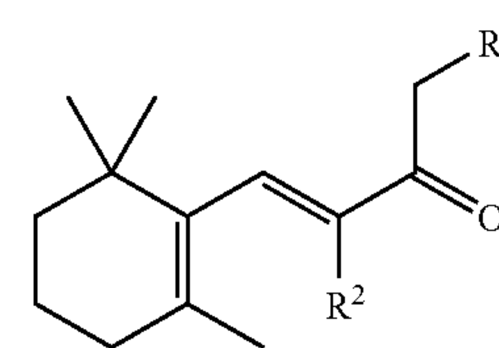
\beta -Isomer
