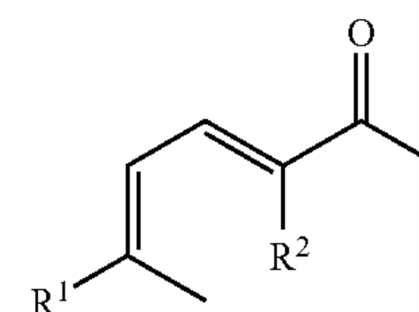
iso-alkylpseudoionone
