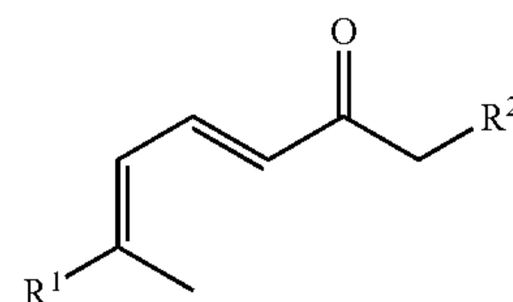
n-alkylpseudoionone
