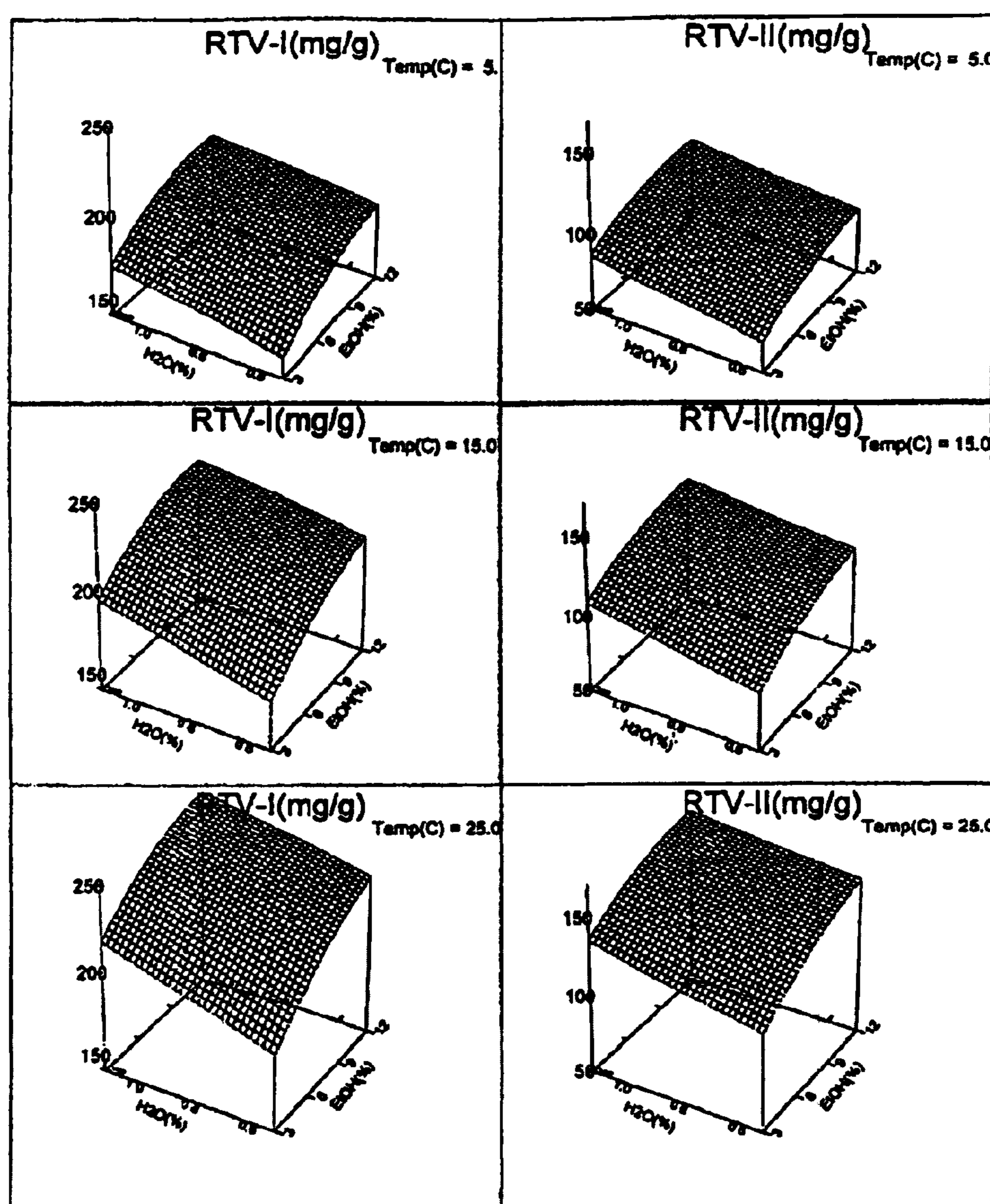
Figure 7. 3D Plots for the Solubility of Ritonavir Form I and II As a Function of Temperature, Water and Ethanol.
