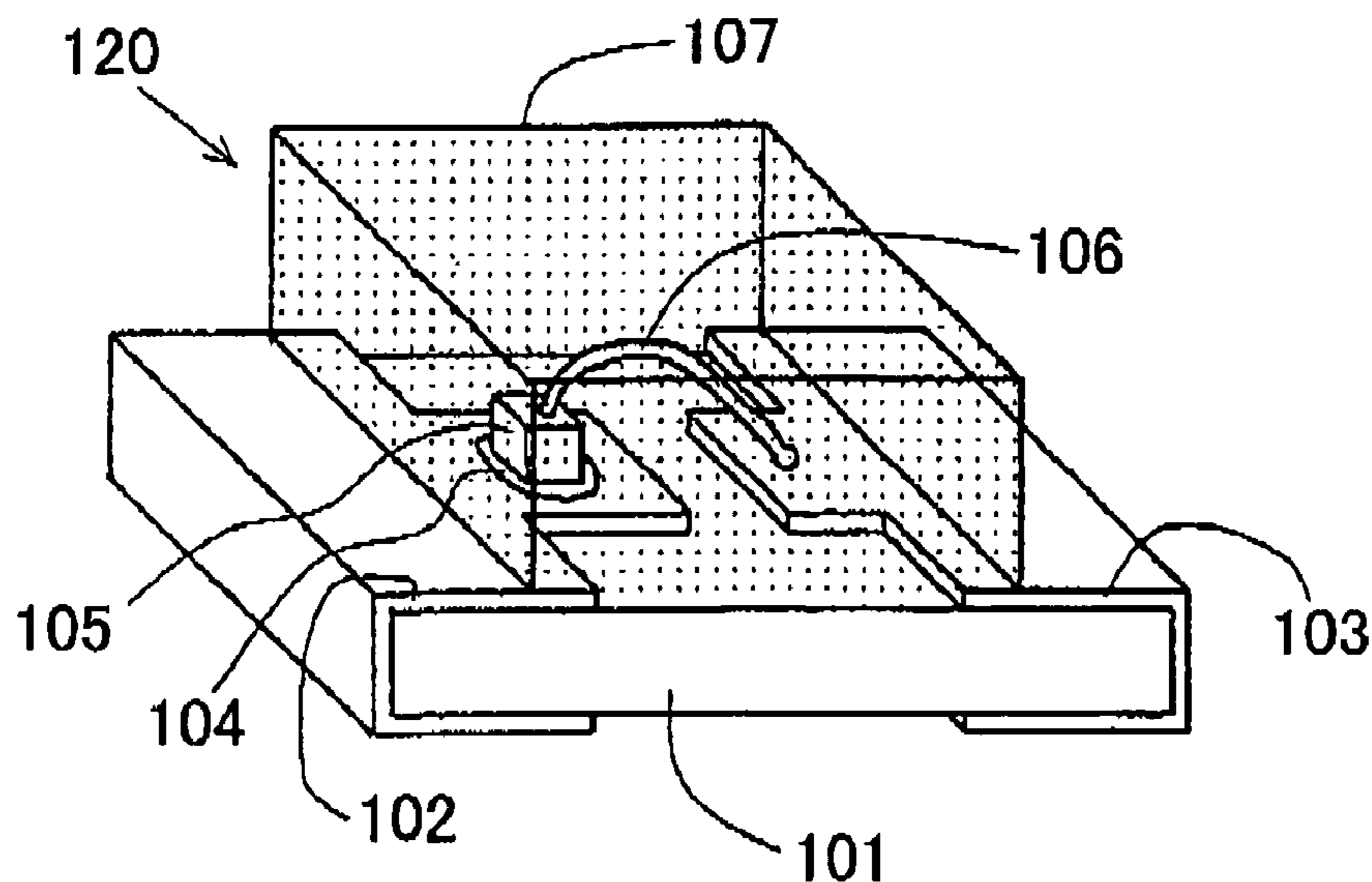
FIG. 18 PRIOR ART
