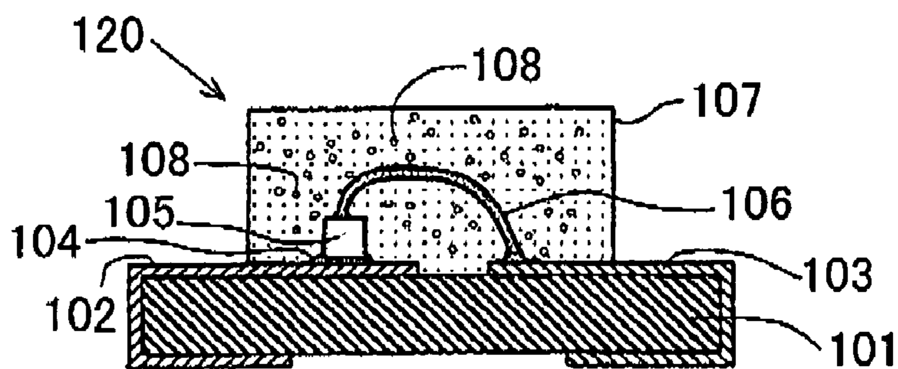
FIG. 19 PRIOR ART
