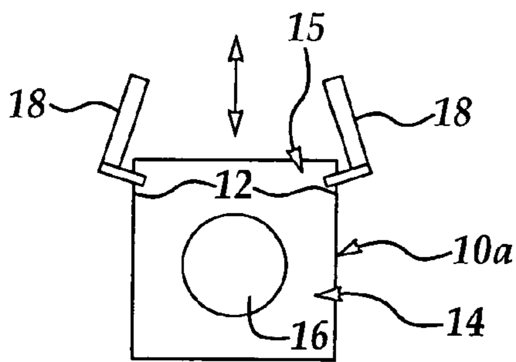
Figure 2 Prior Art
