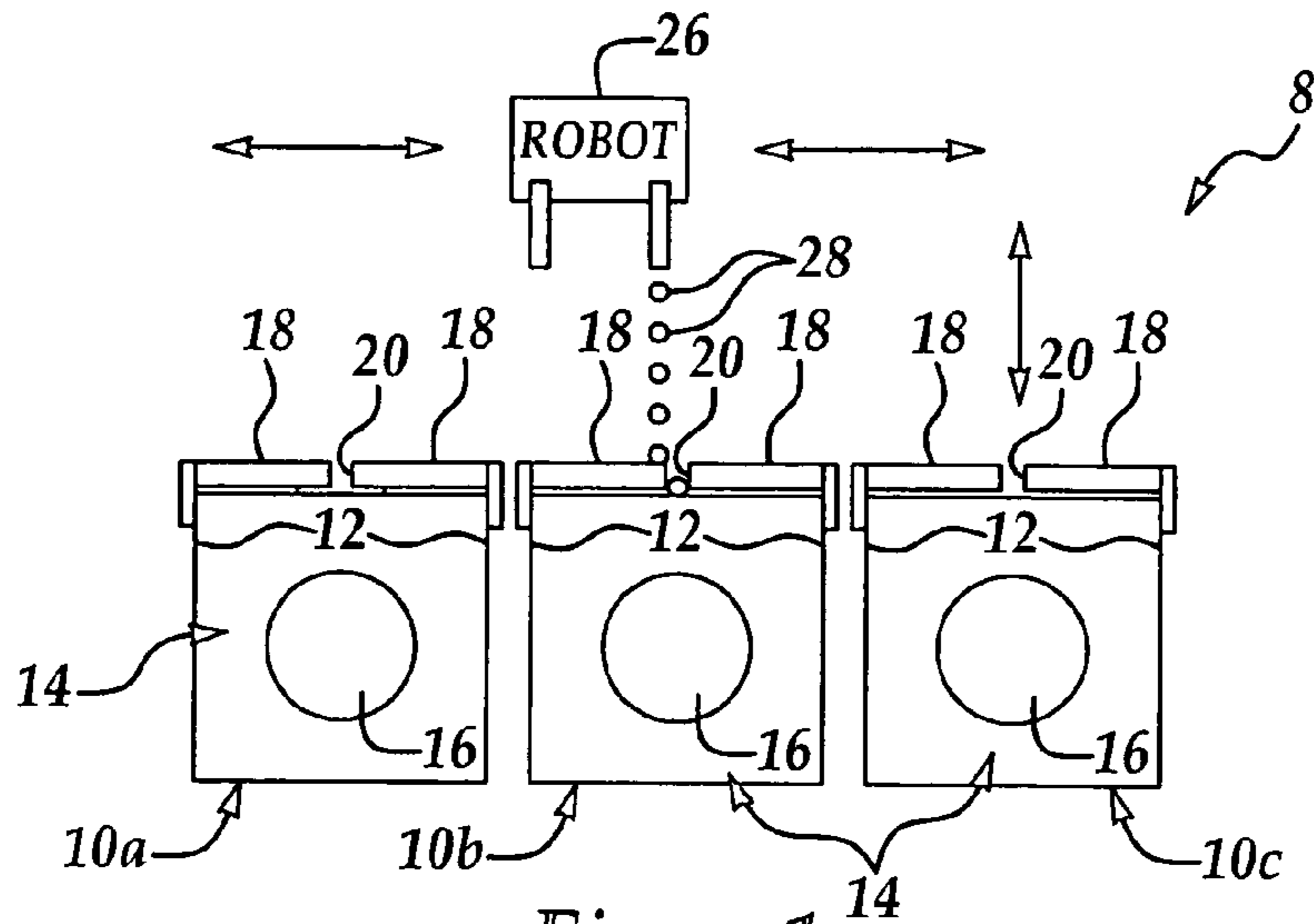
Figure 1 Prior Art
