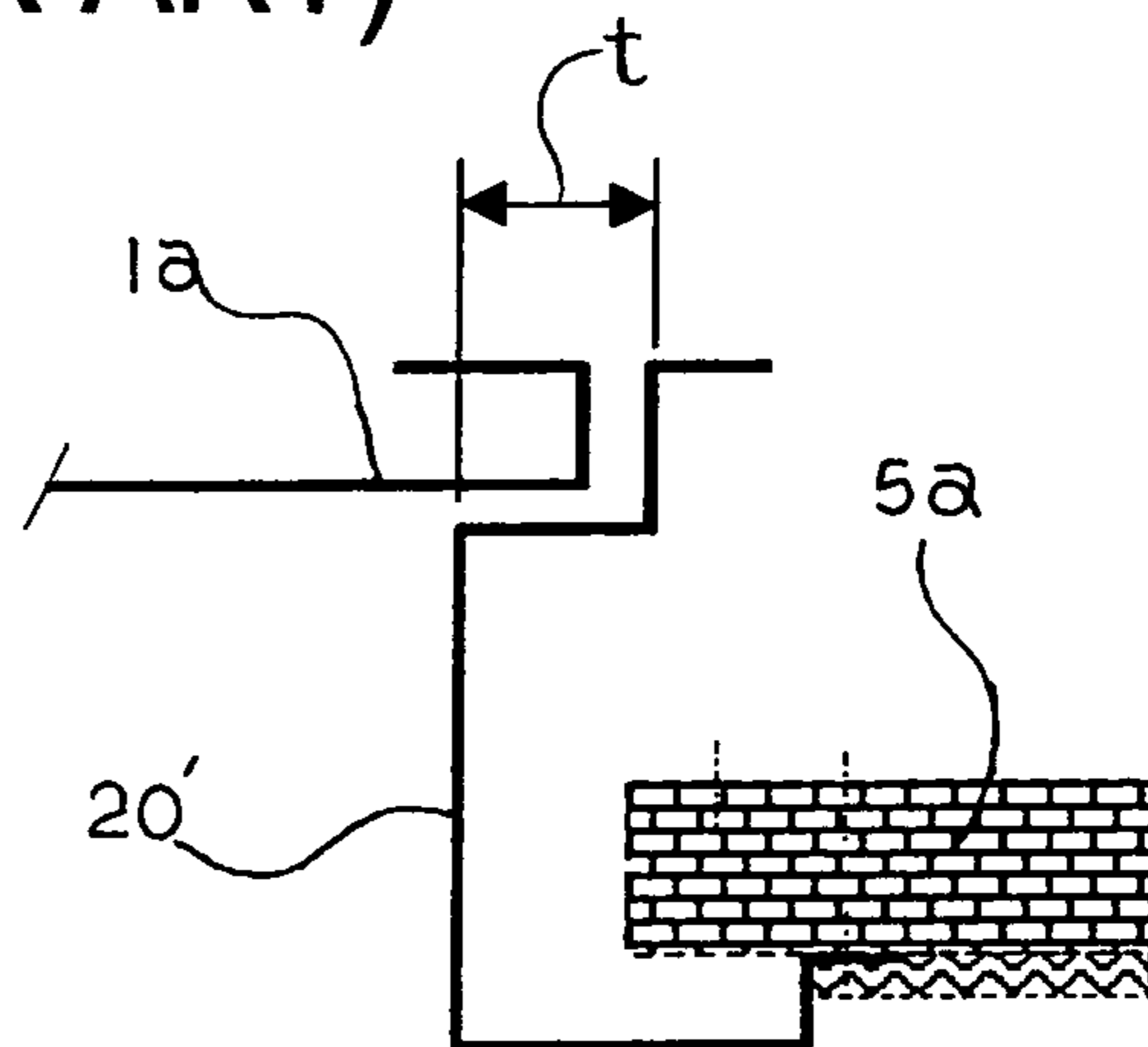
FIG. 4 (PRIOR ART)
