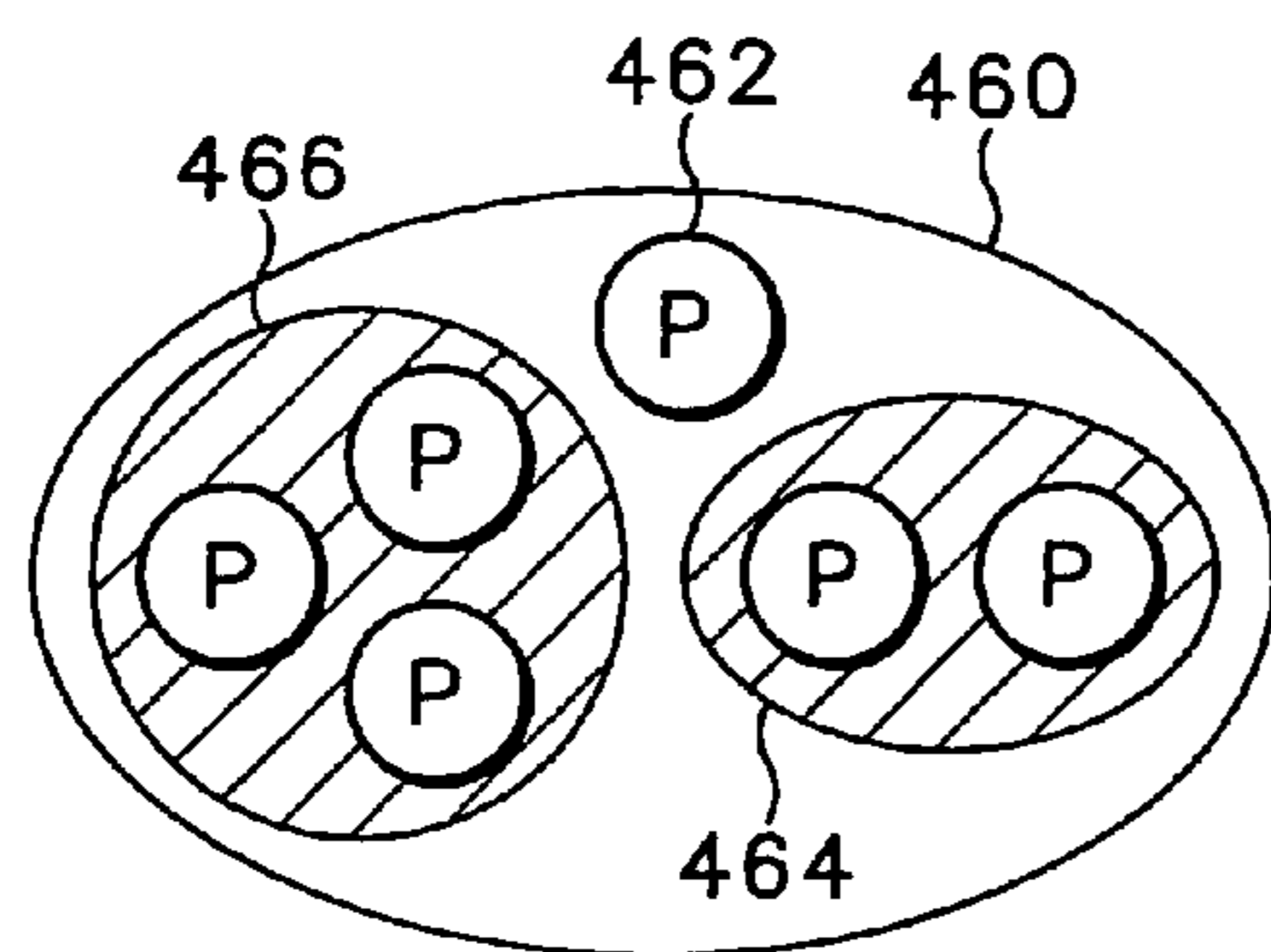
OBJECT HEIRARCHY
