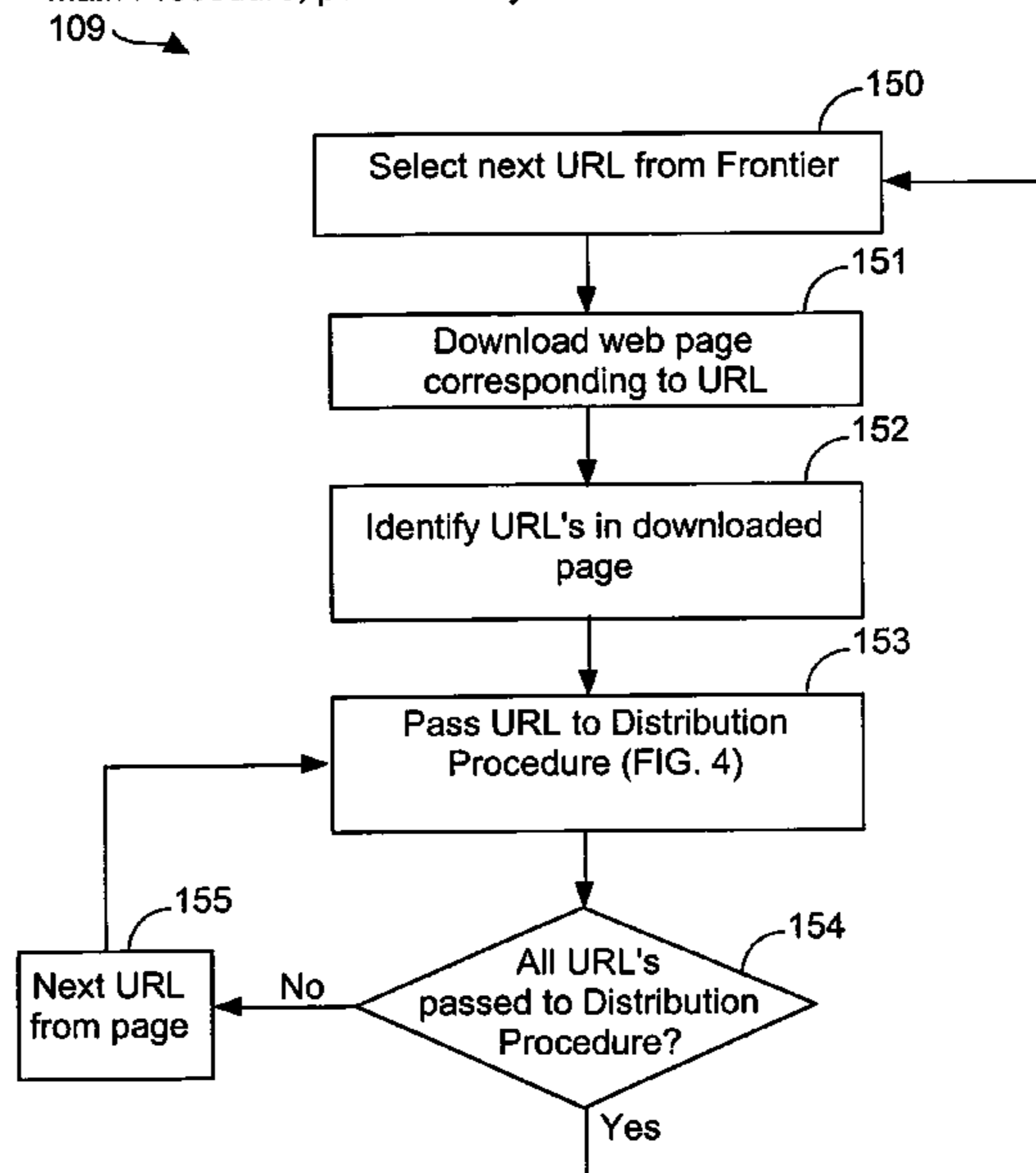
Main Procedure, performed by each thread
