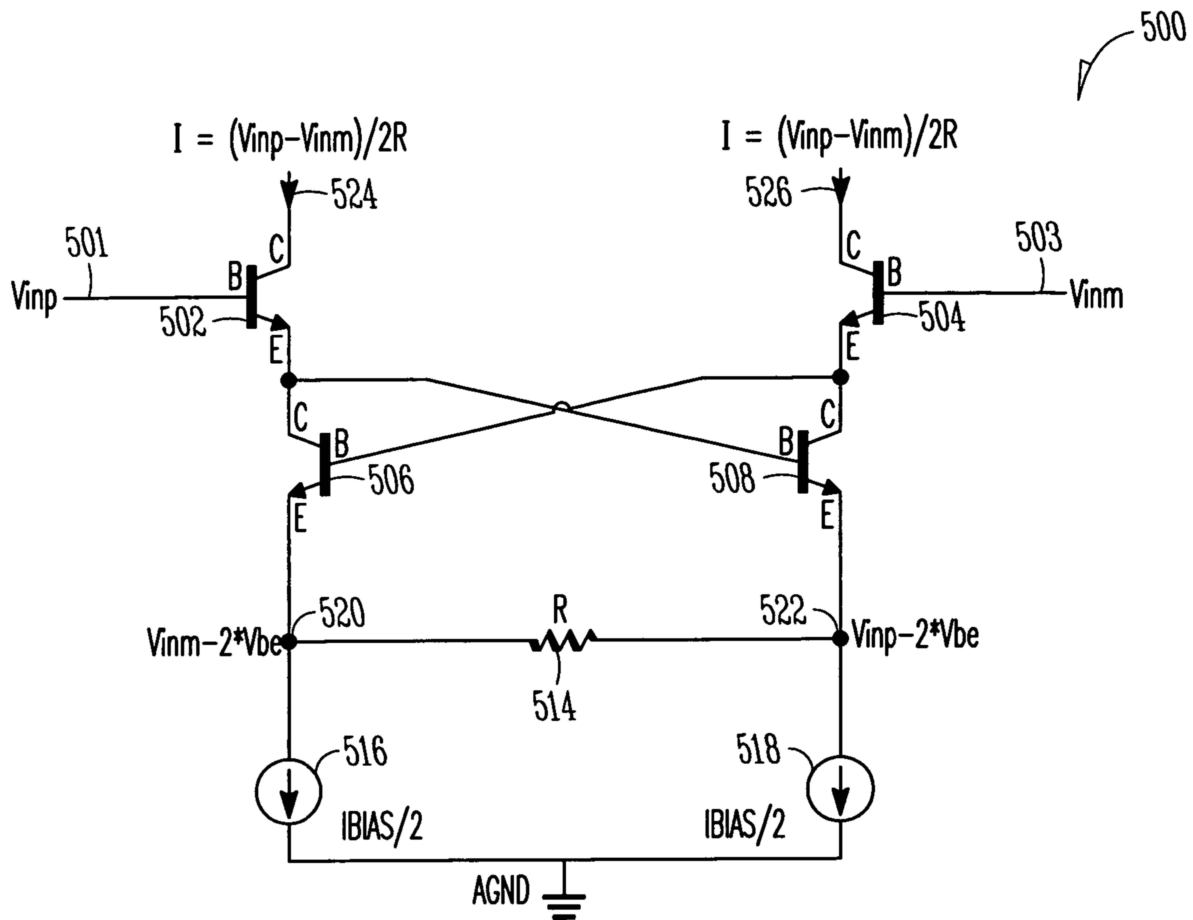
TRANSCONDUCTANCE - AMPLIFIER CIRCUIT
