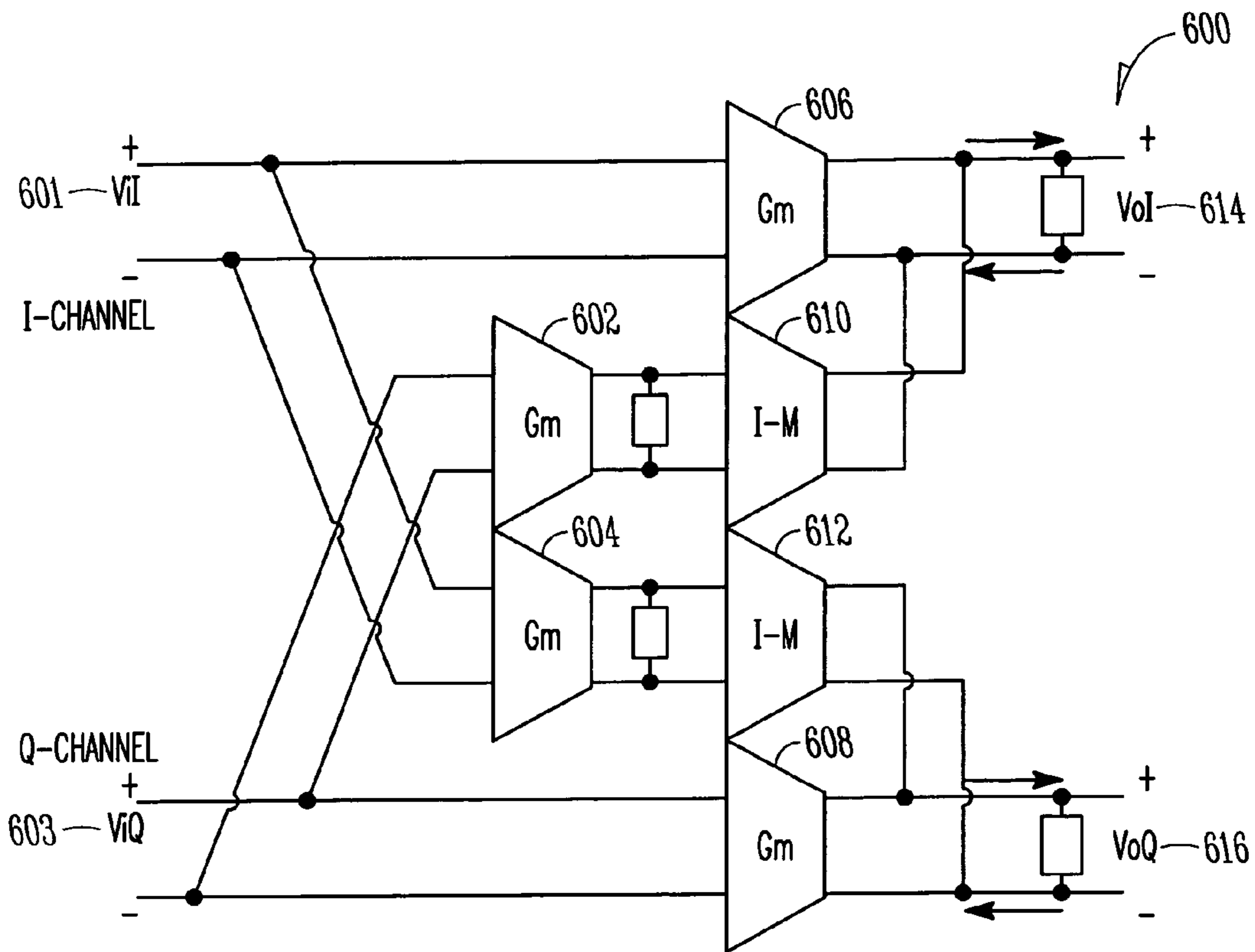
GmC POLYPHASE FILTER
