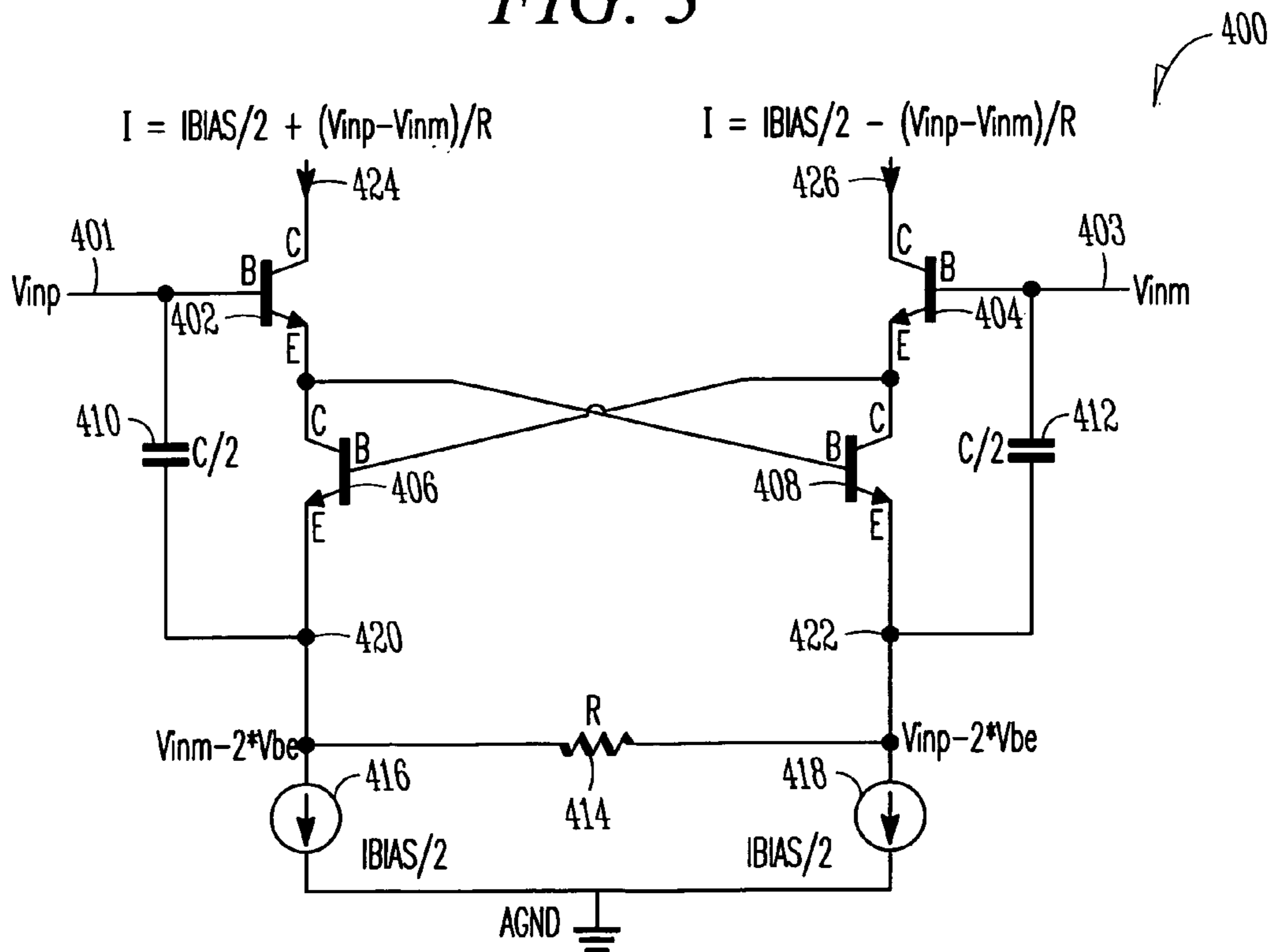
TRANSCONDUCTANCE - CAPACITOR CIRCUIT
