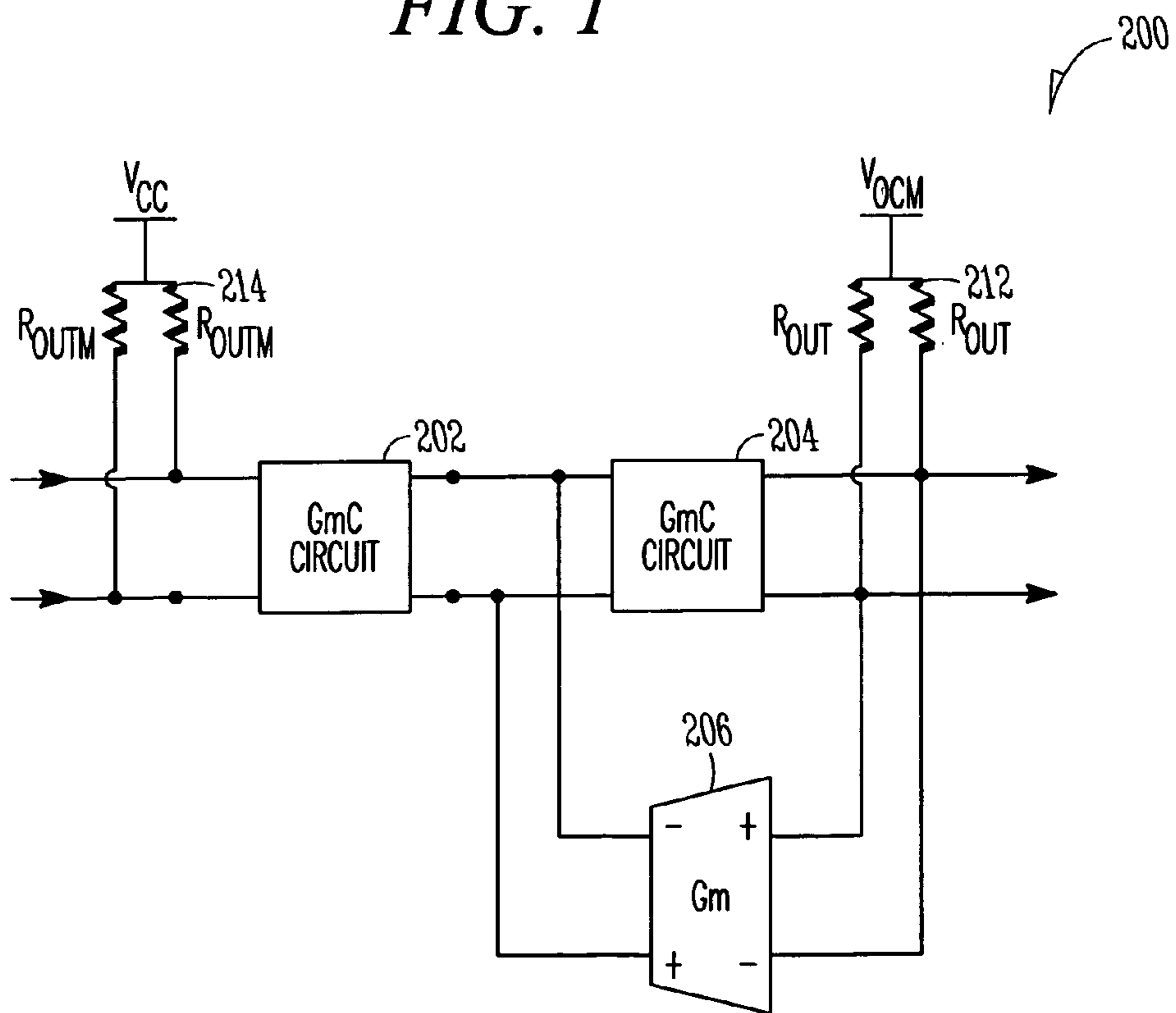
GmC FILTER
