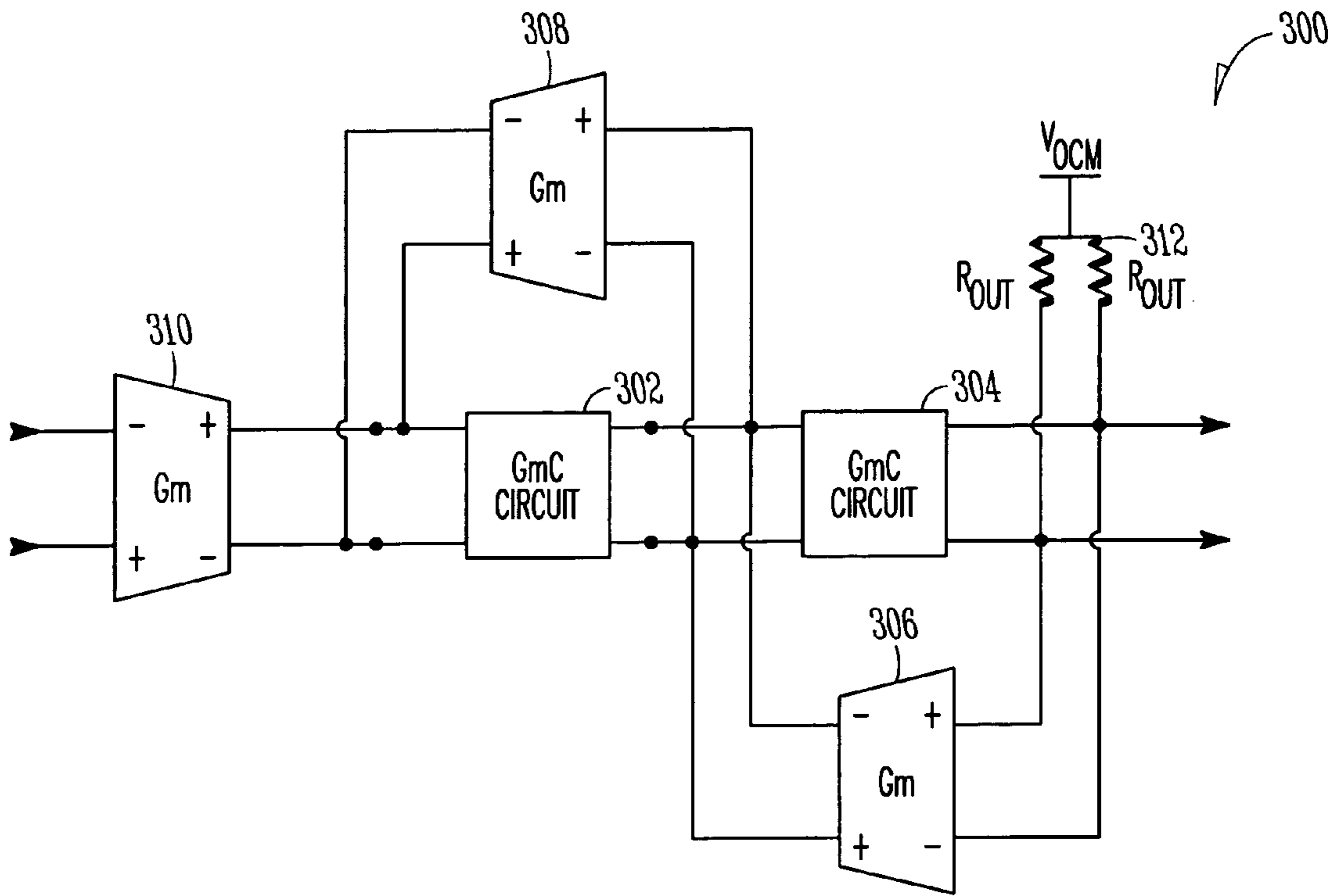
GmC FILTER FIG. 3
