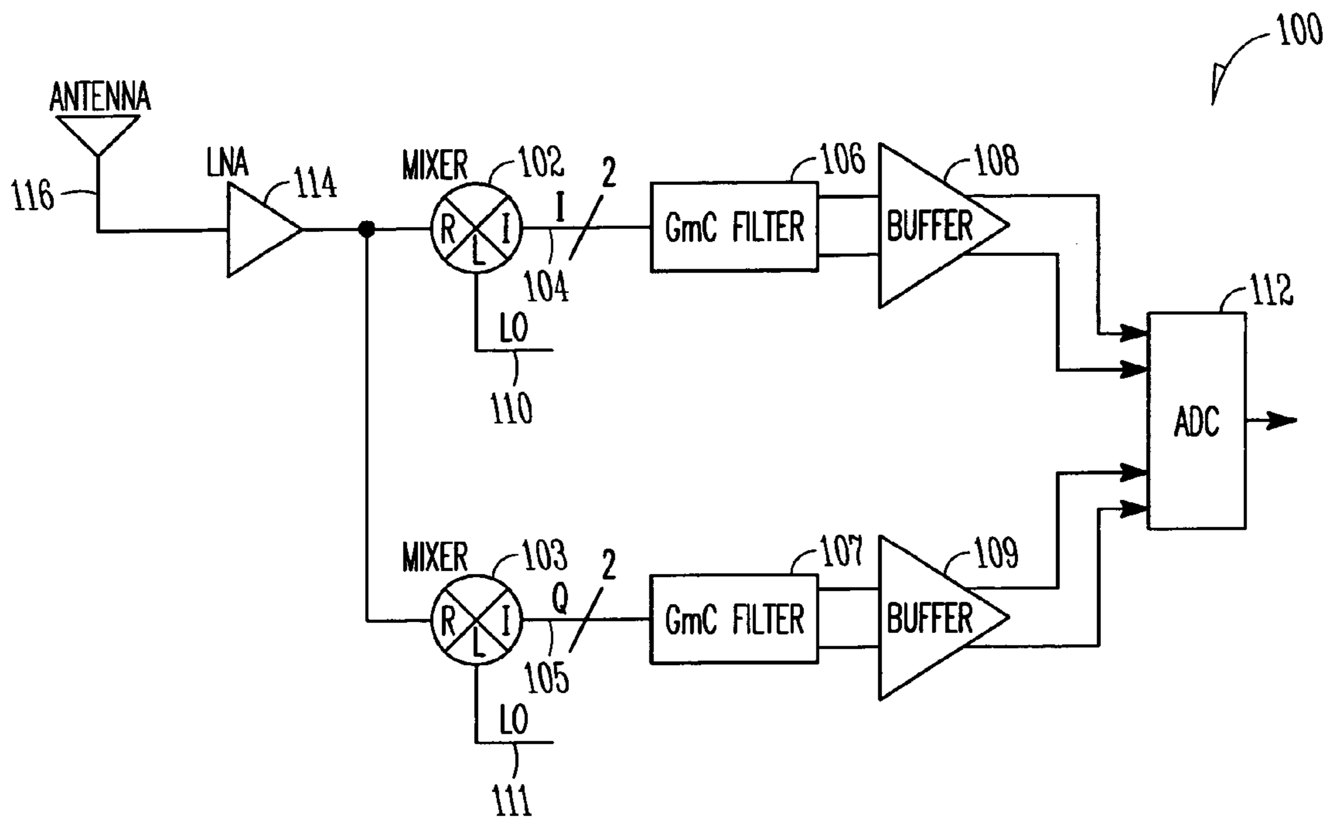
RECEIVER
