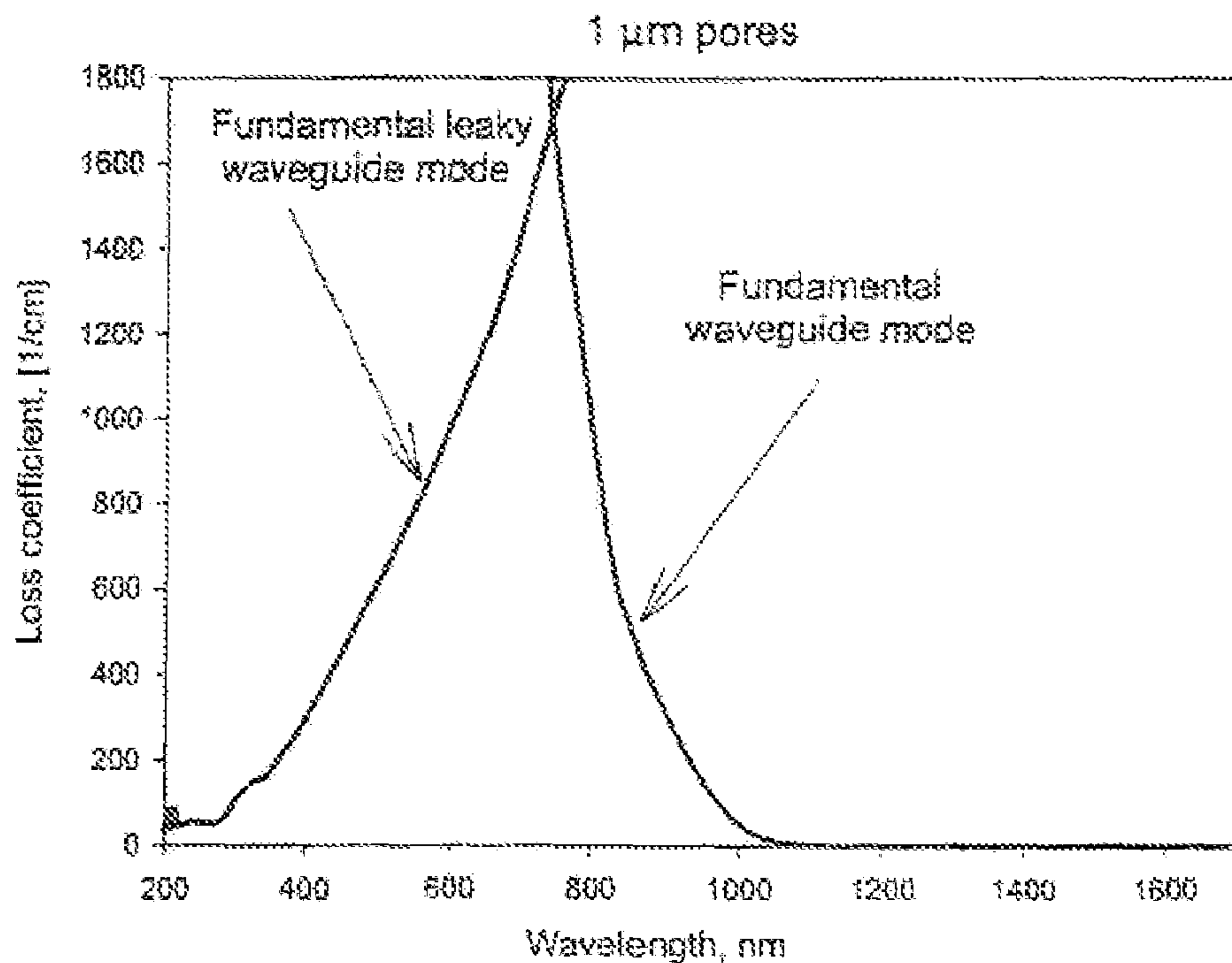
Fig. 3 (PRIOR ART)
