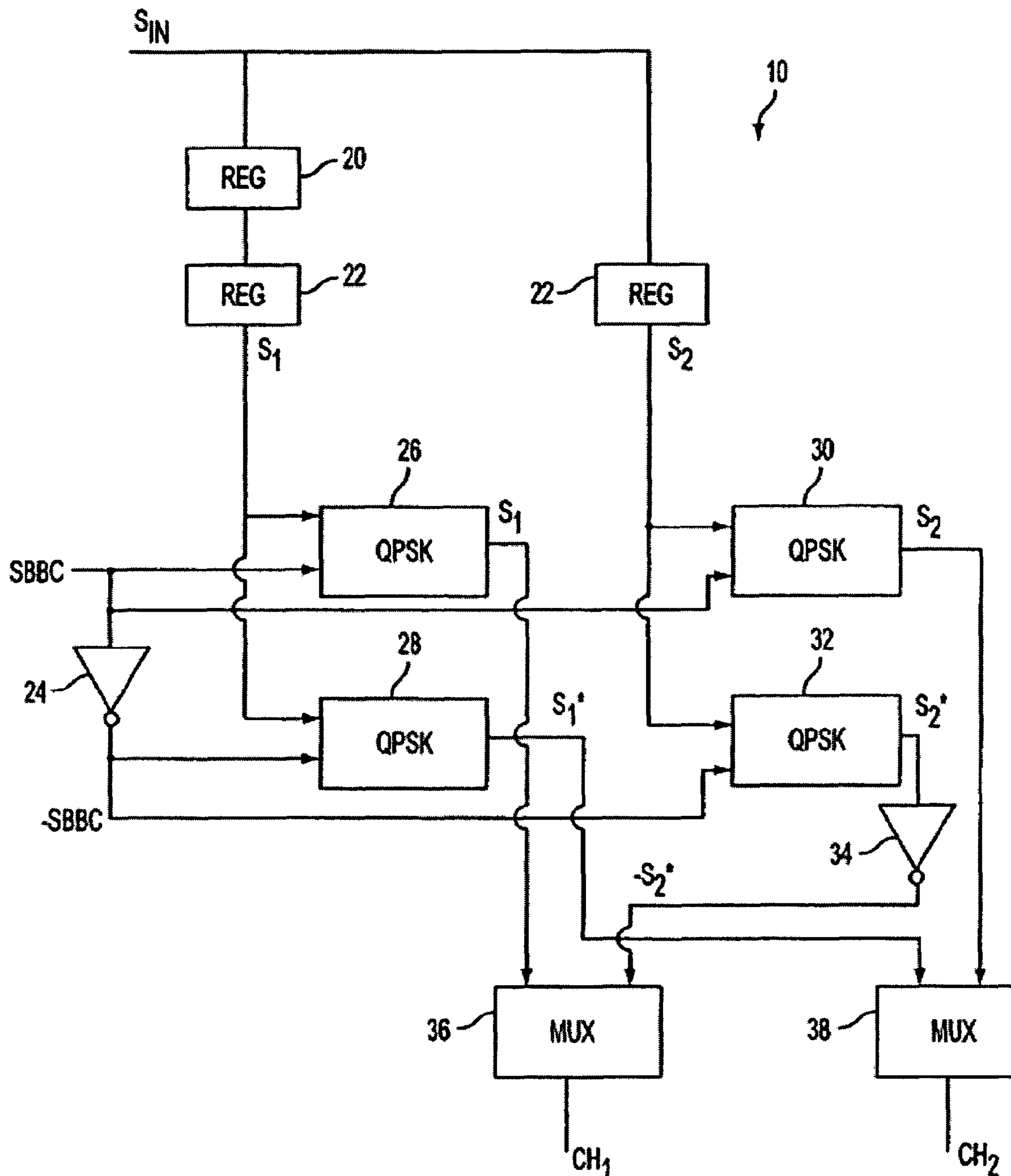
FIG. 3 (PRIOR ART)
