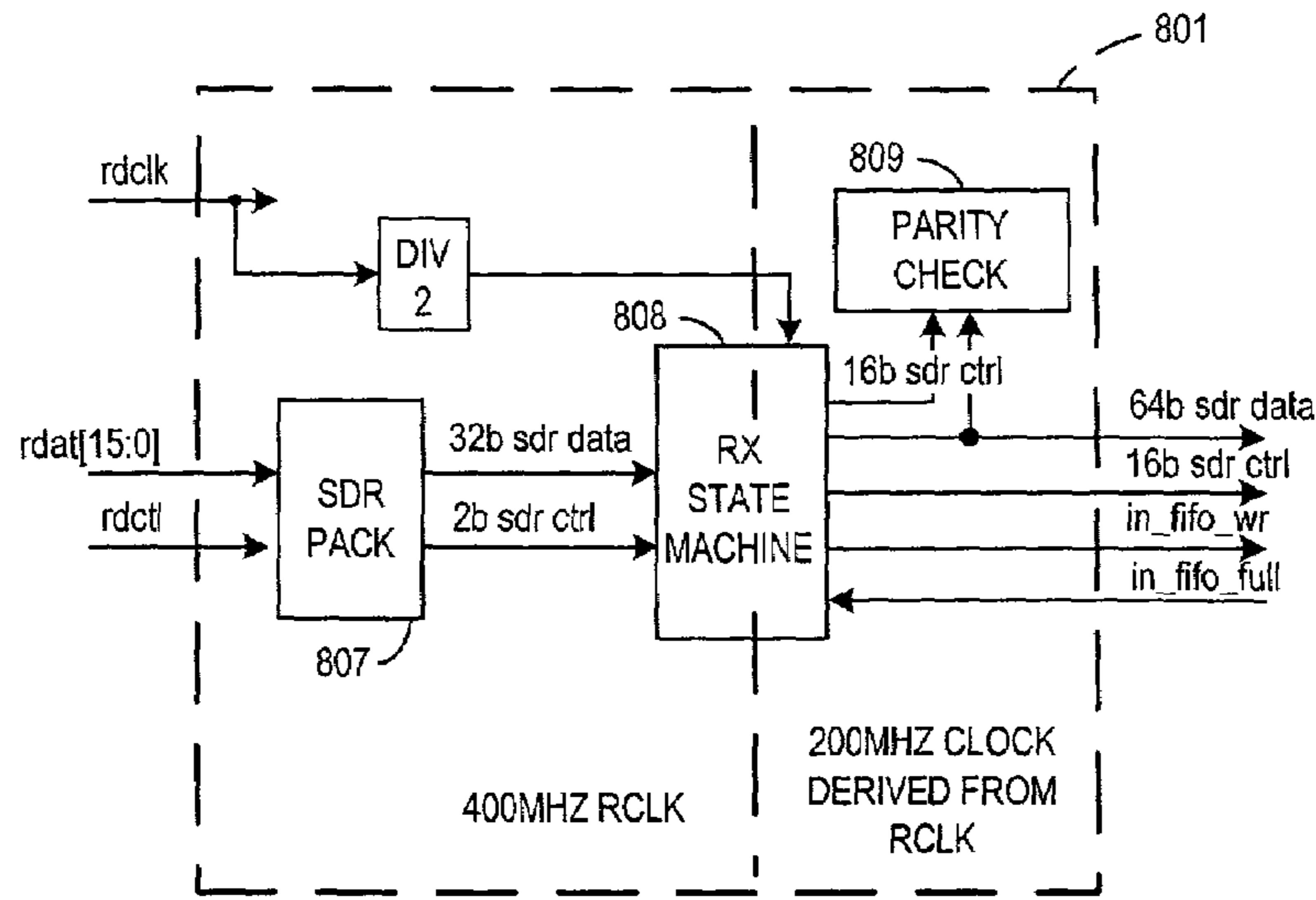
INPUT CONTROL BLOCK
