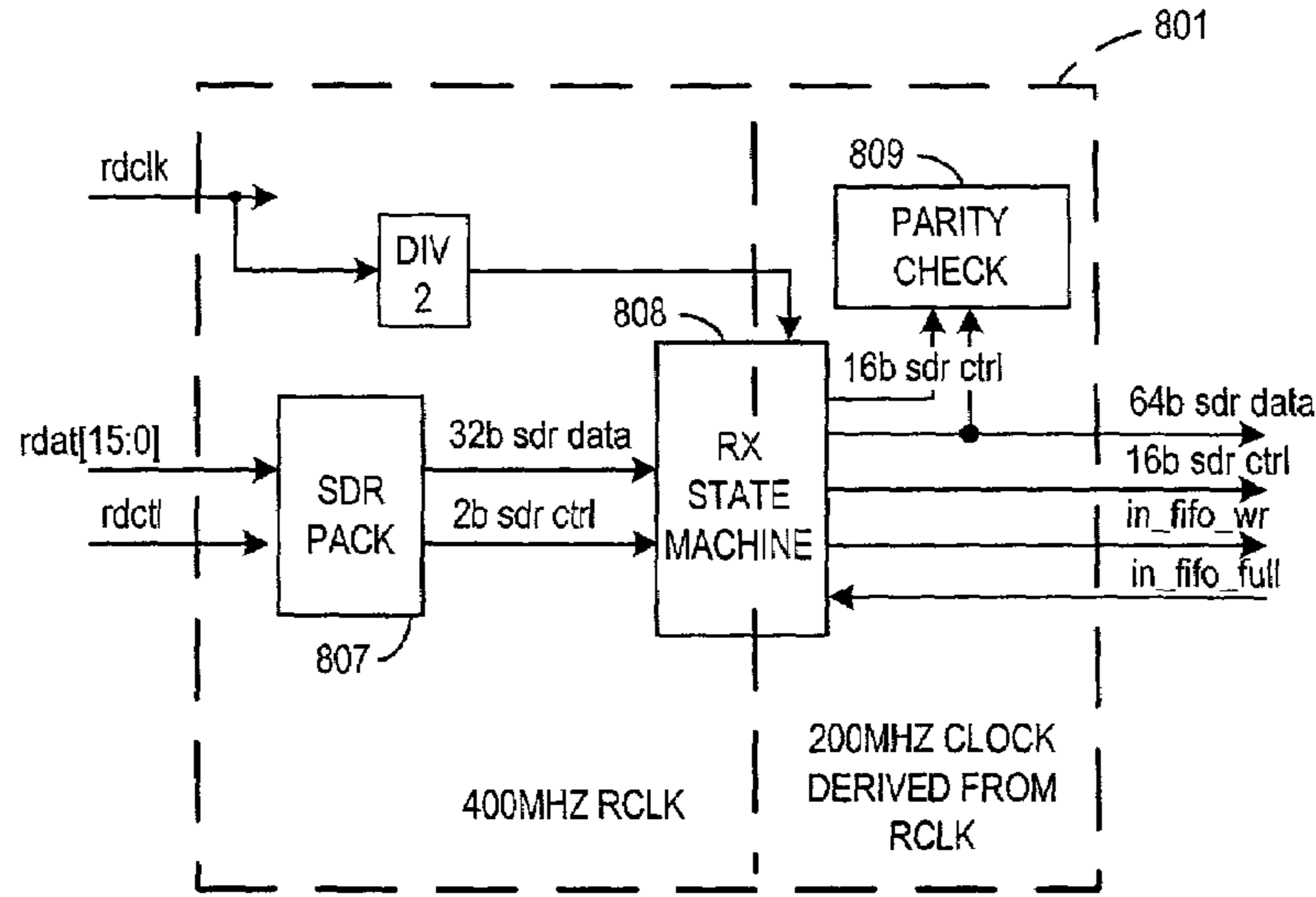
INPUT CONTROL BLOCK
