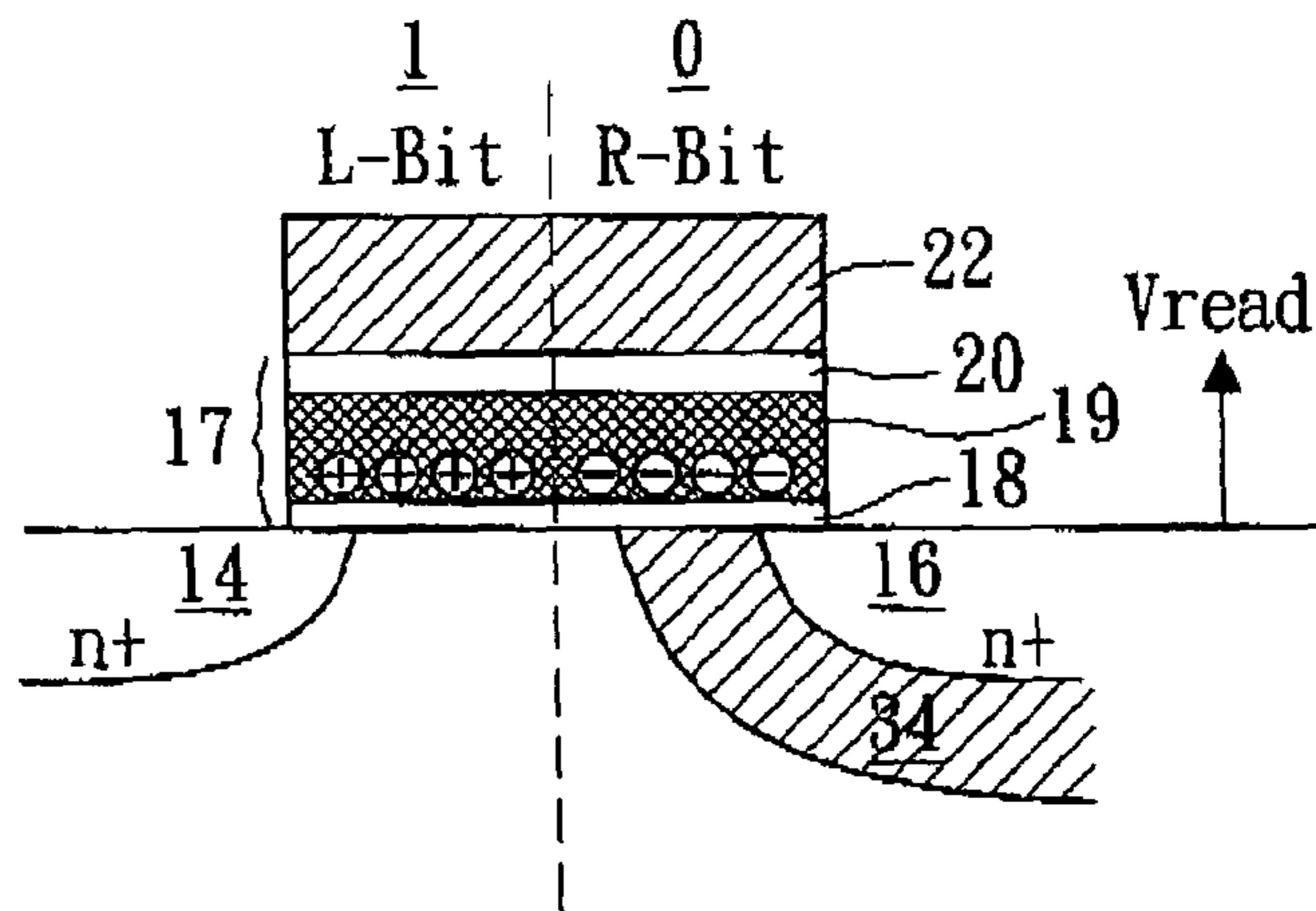
FIG. 3F(PRIOR ART)
