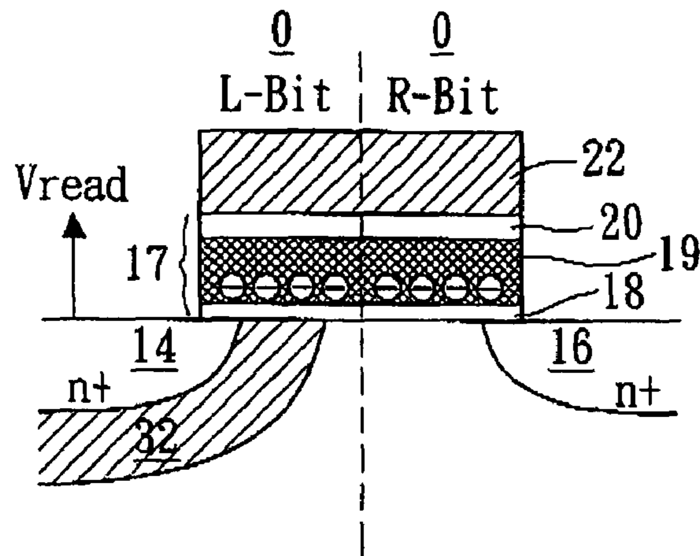
FIG. 3A(PRIOR ART)
