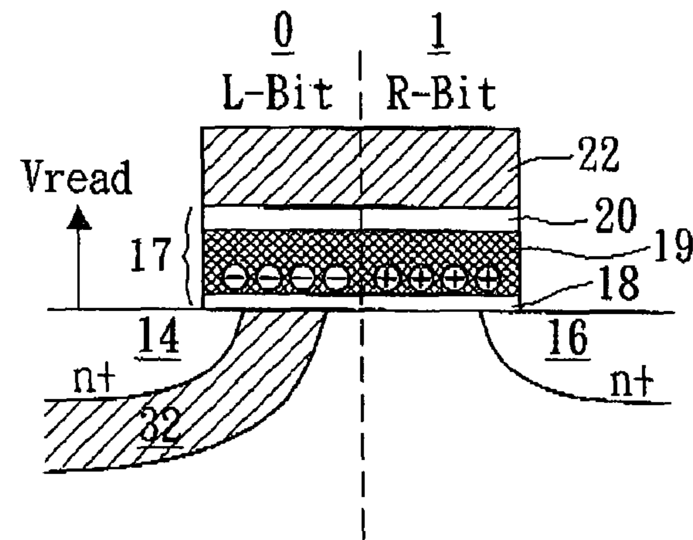
FIG. 3C(PRIOR ART)
