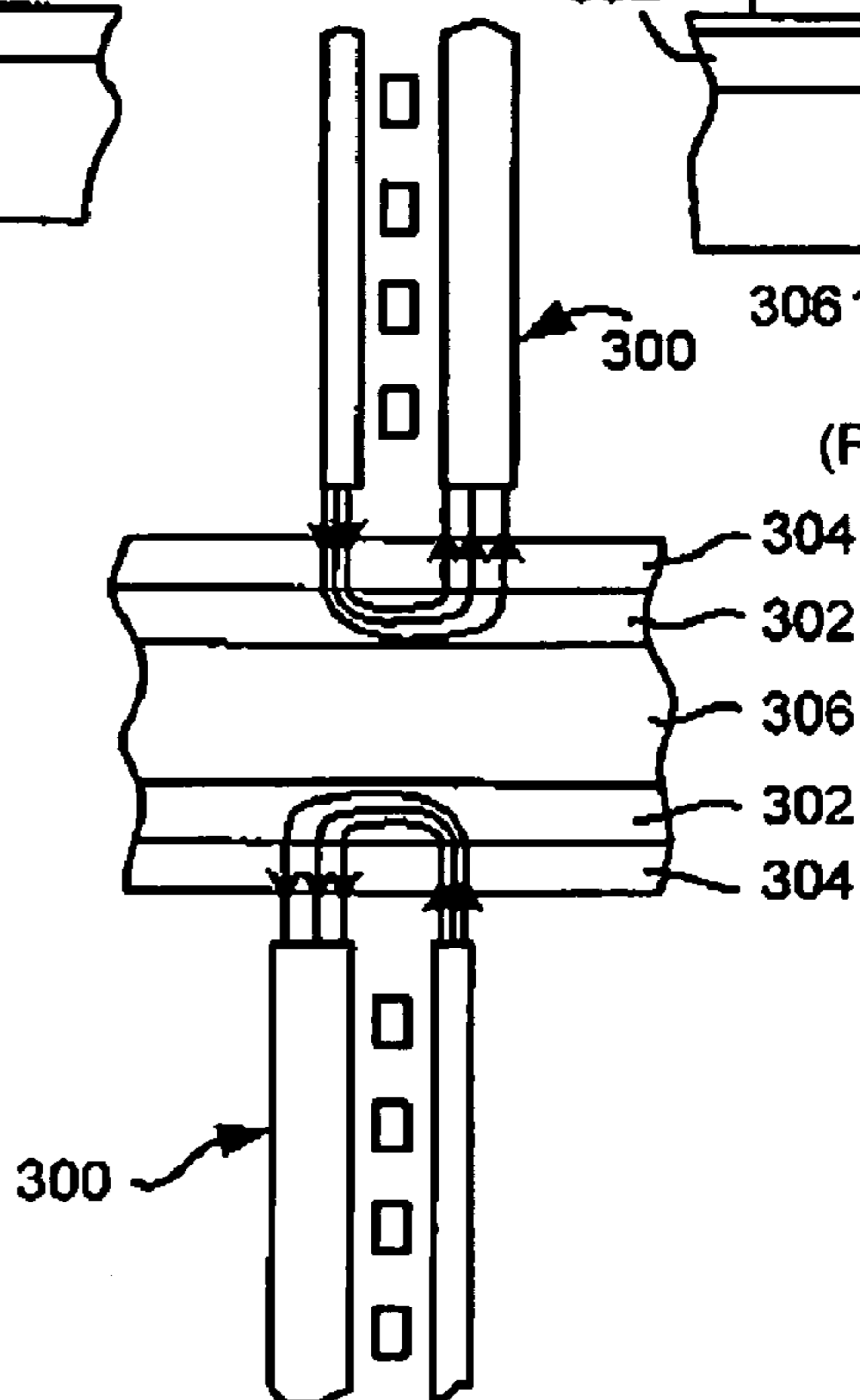
FIG. 5 (PRIOR ART)
