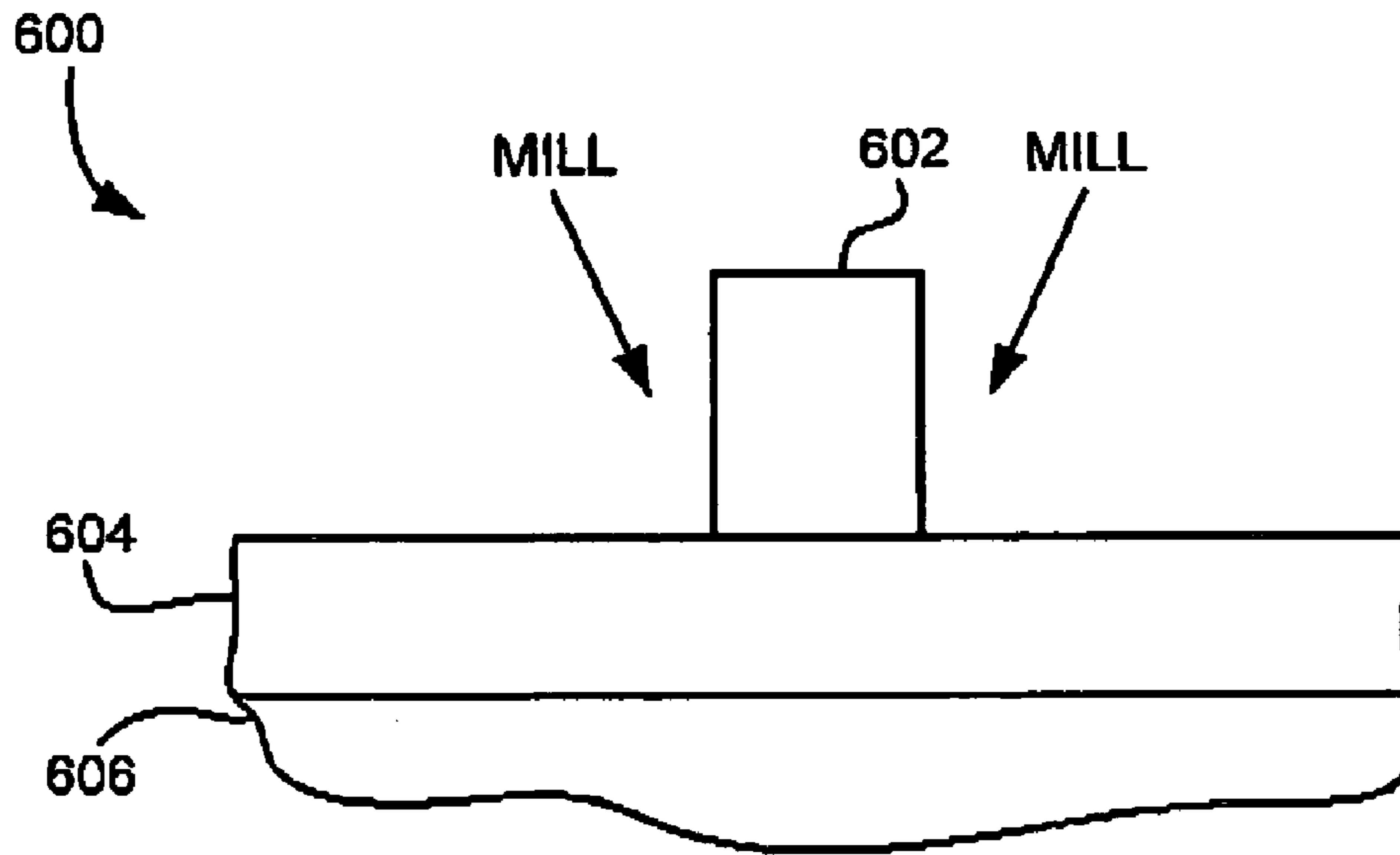
FIG. 6 (PRIOR ART)
