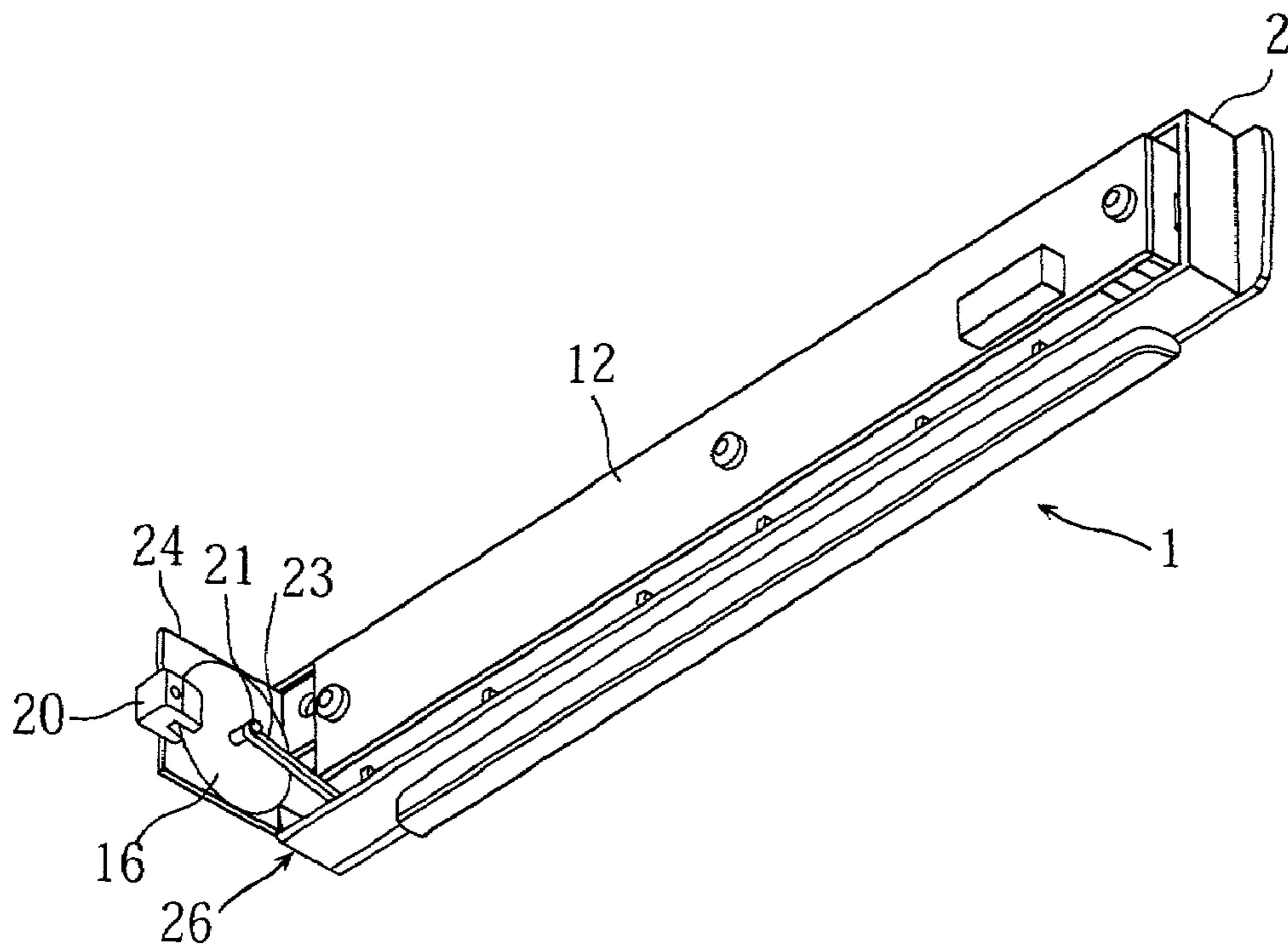
FIG. 10 PRIOR ART
