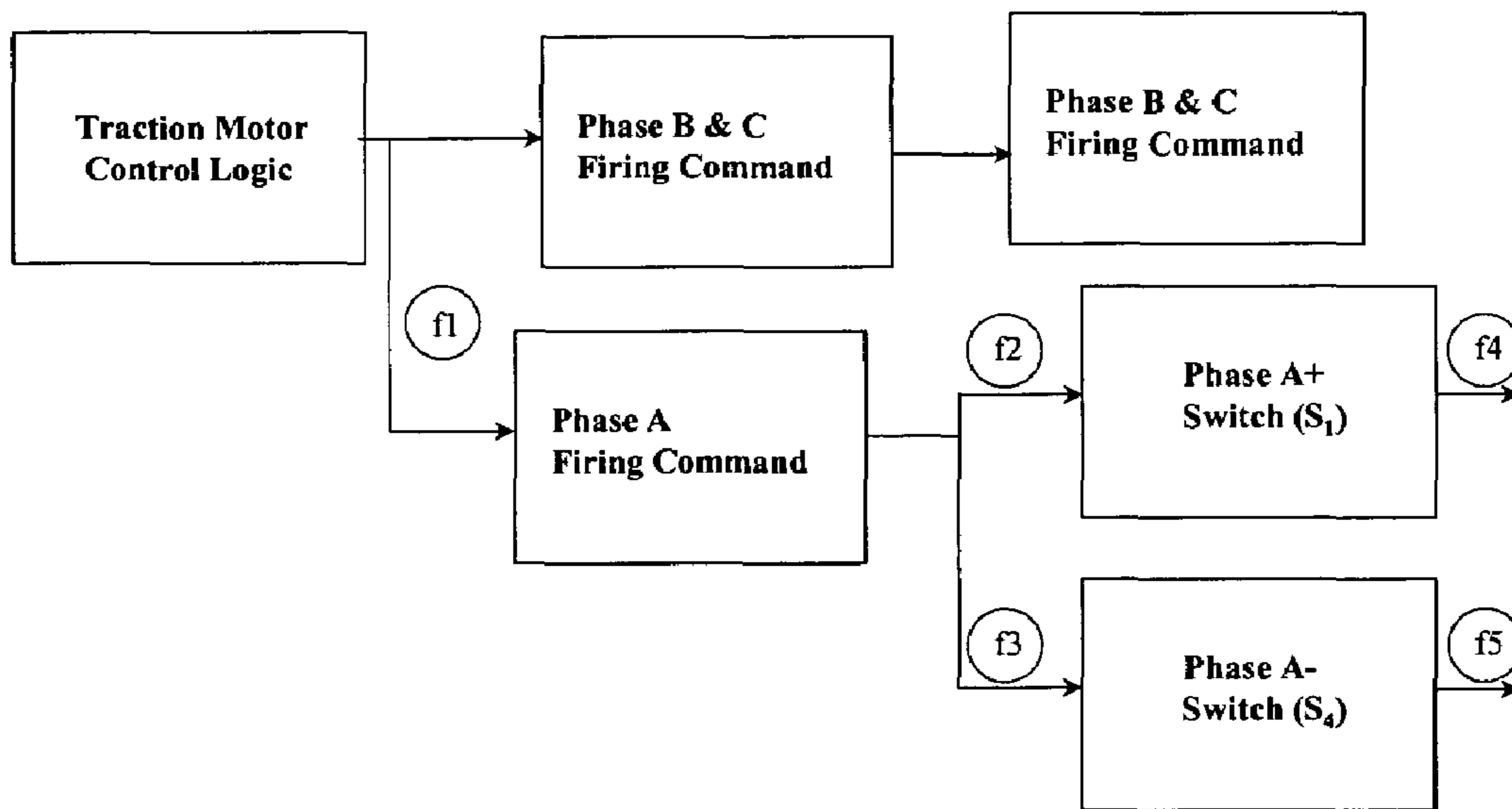
FIG. 2 Prior Art
