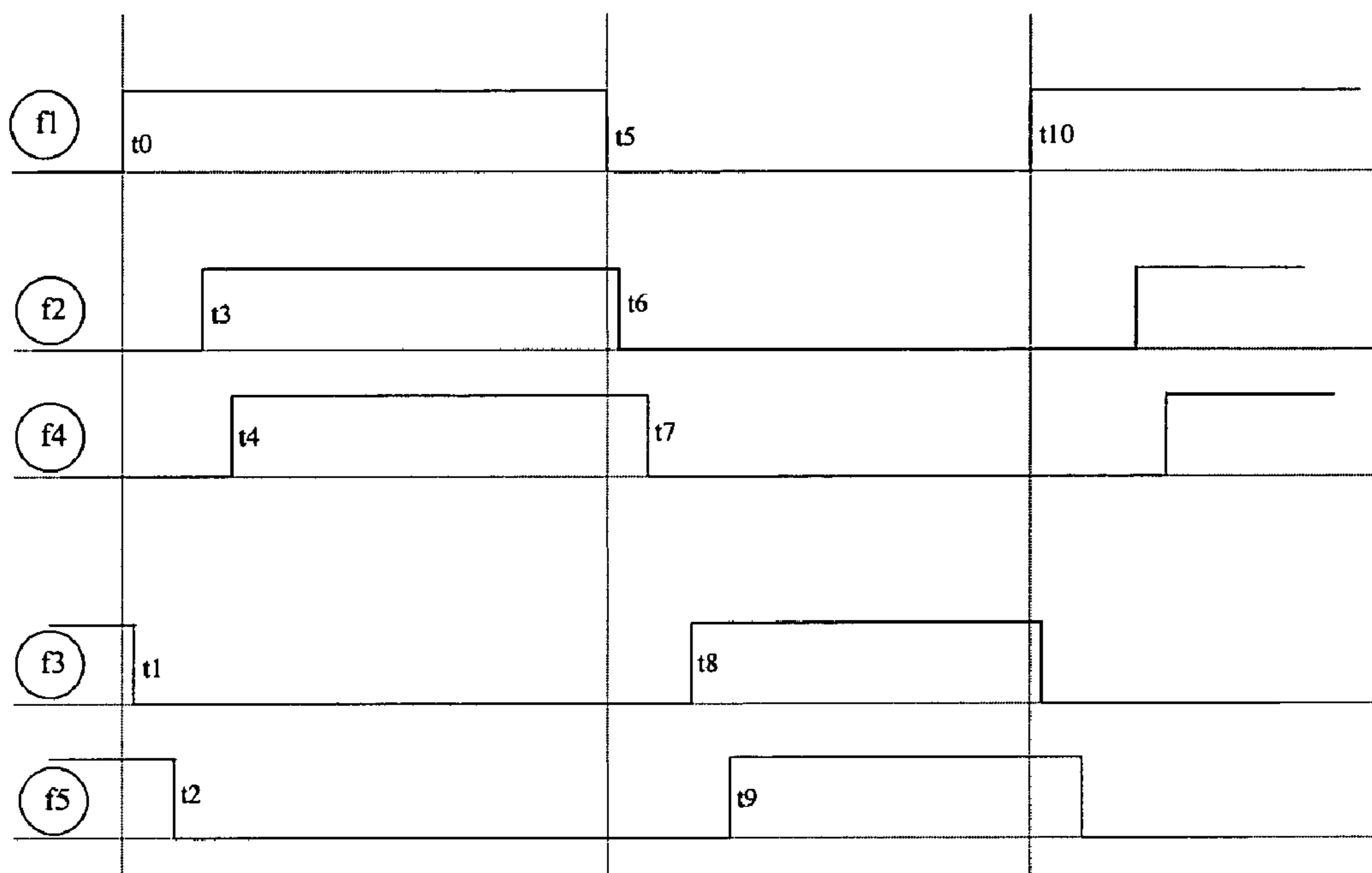
FIG. 3 Prior Art
