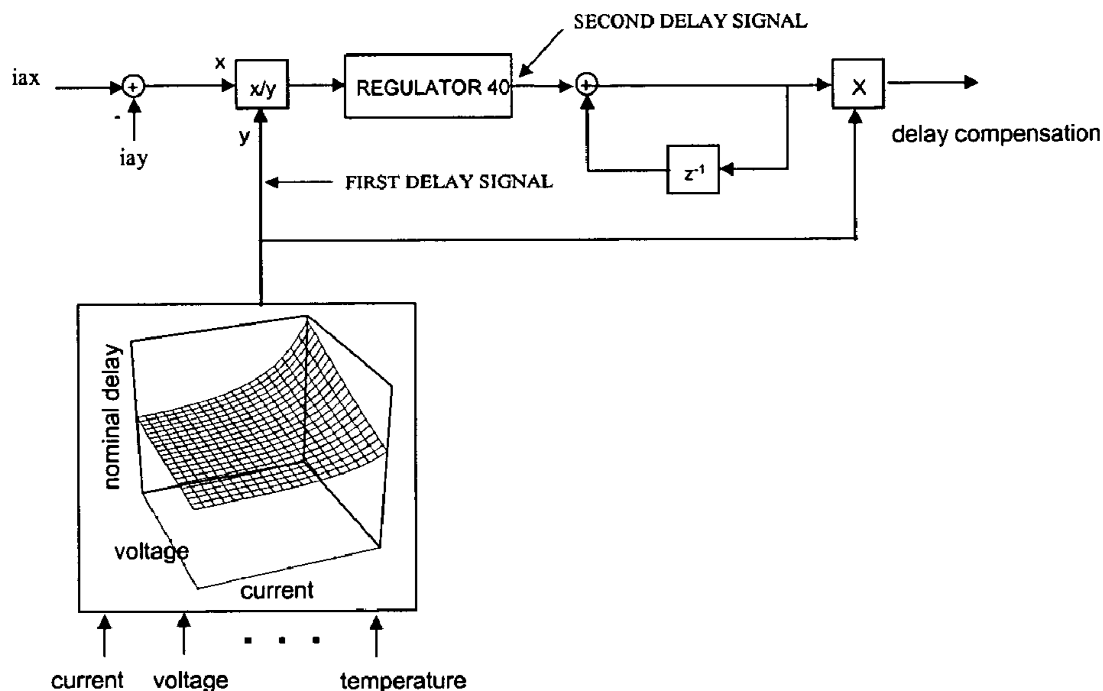
Current equalizing regulator option 2
