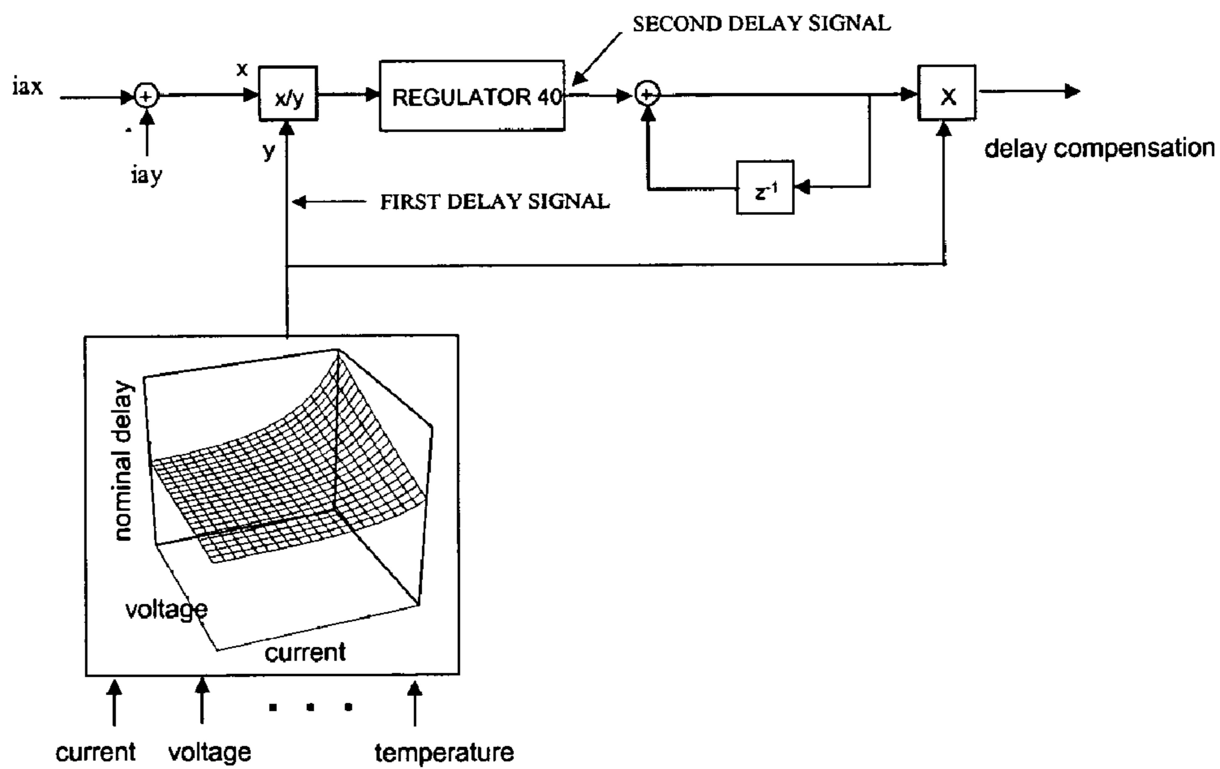
FIG. 14 Current equalizing regulator option 2
