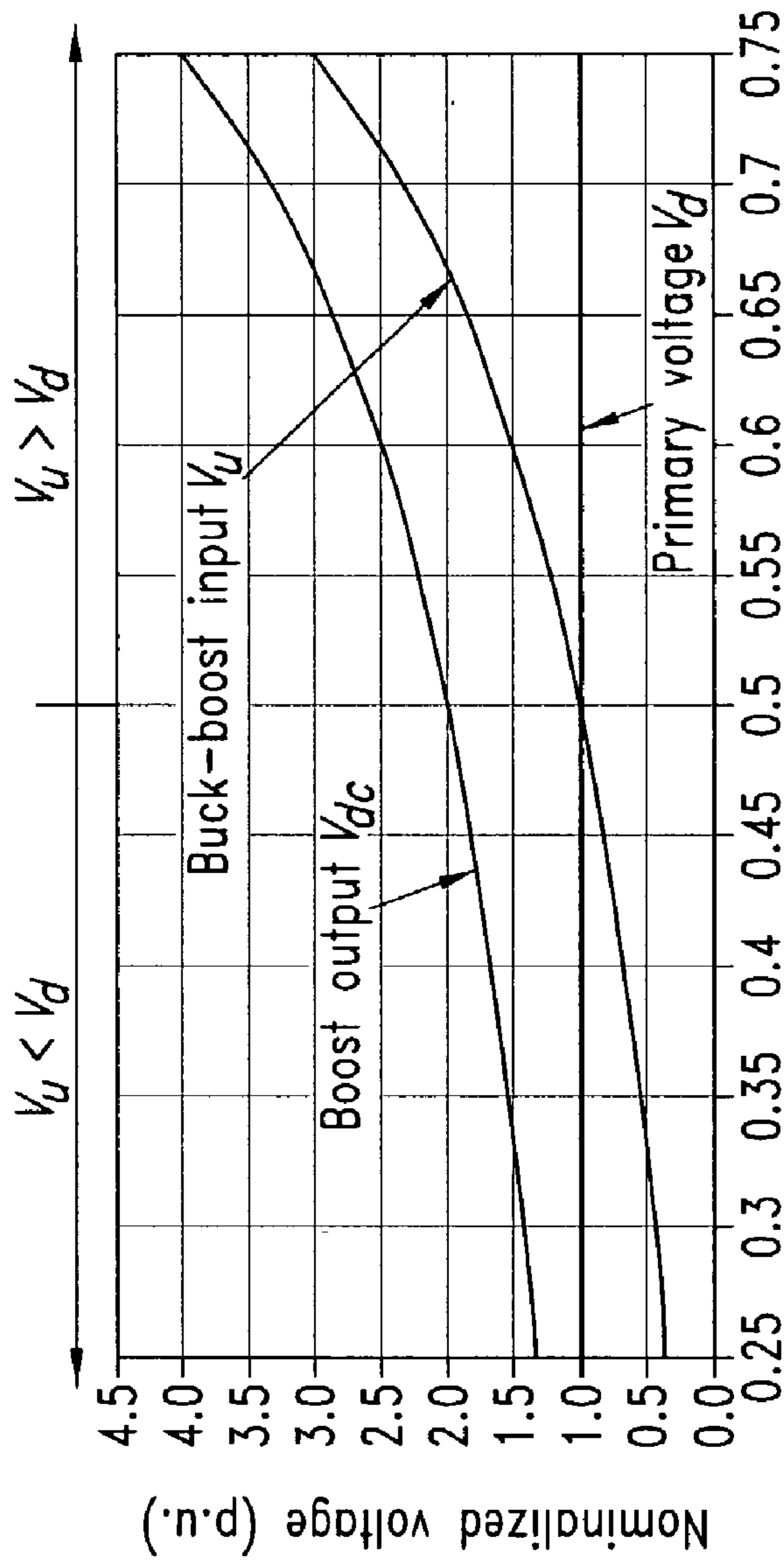
Duty cycle of primary (boost) converter ( D )
