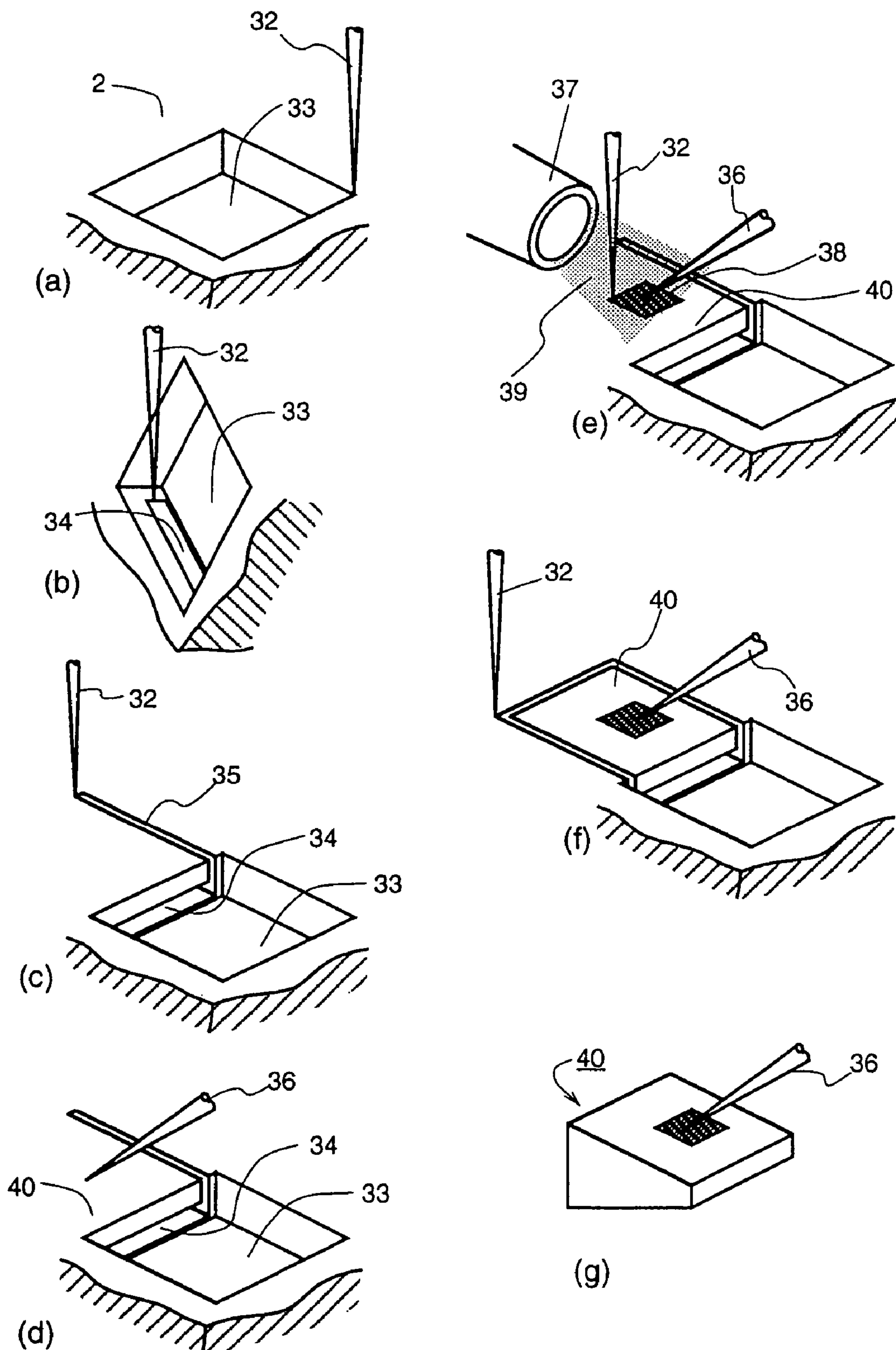
FIG.4 (PRIOR ART)
