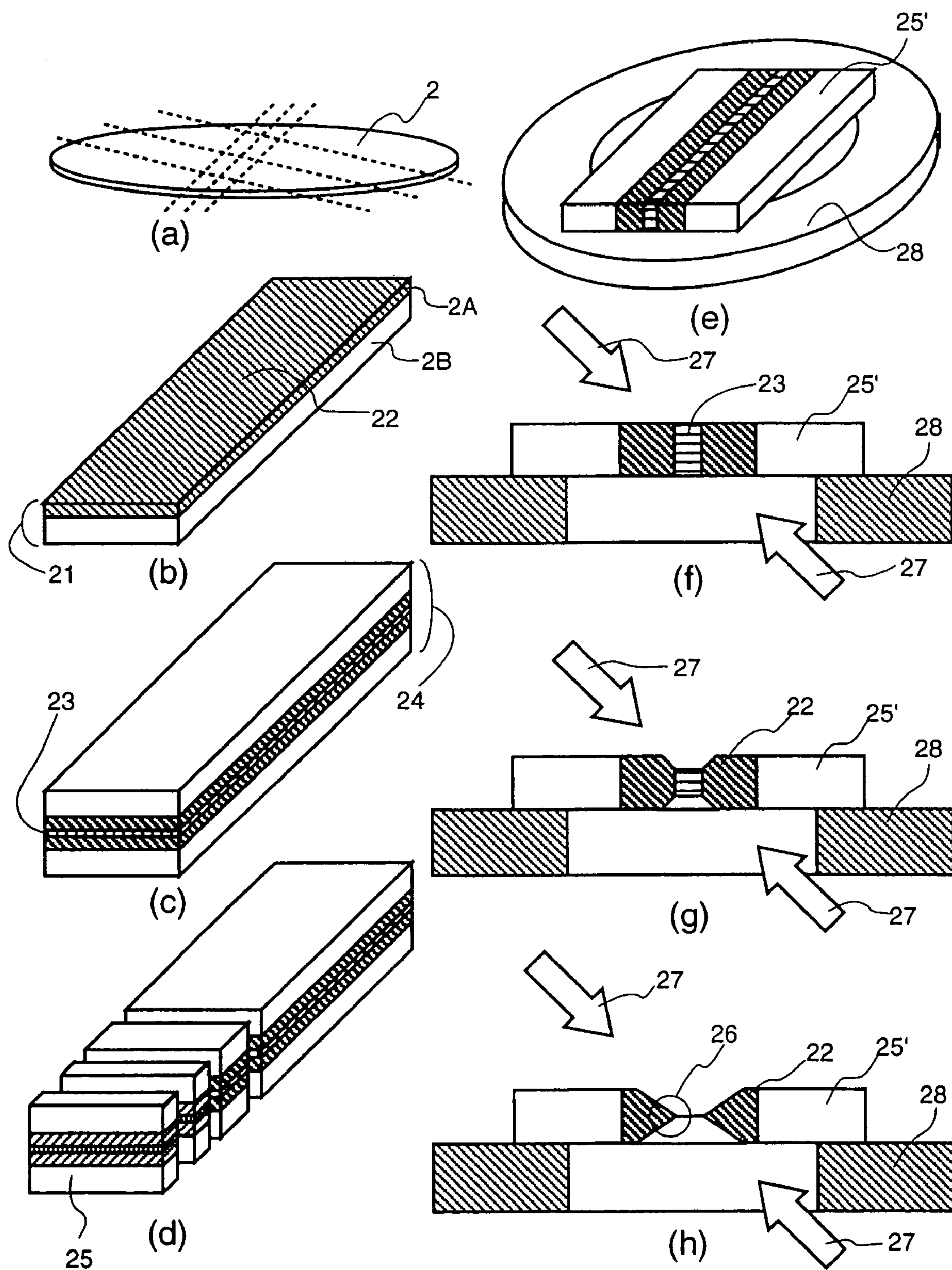
FIG.2 (PRIOR ART)
