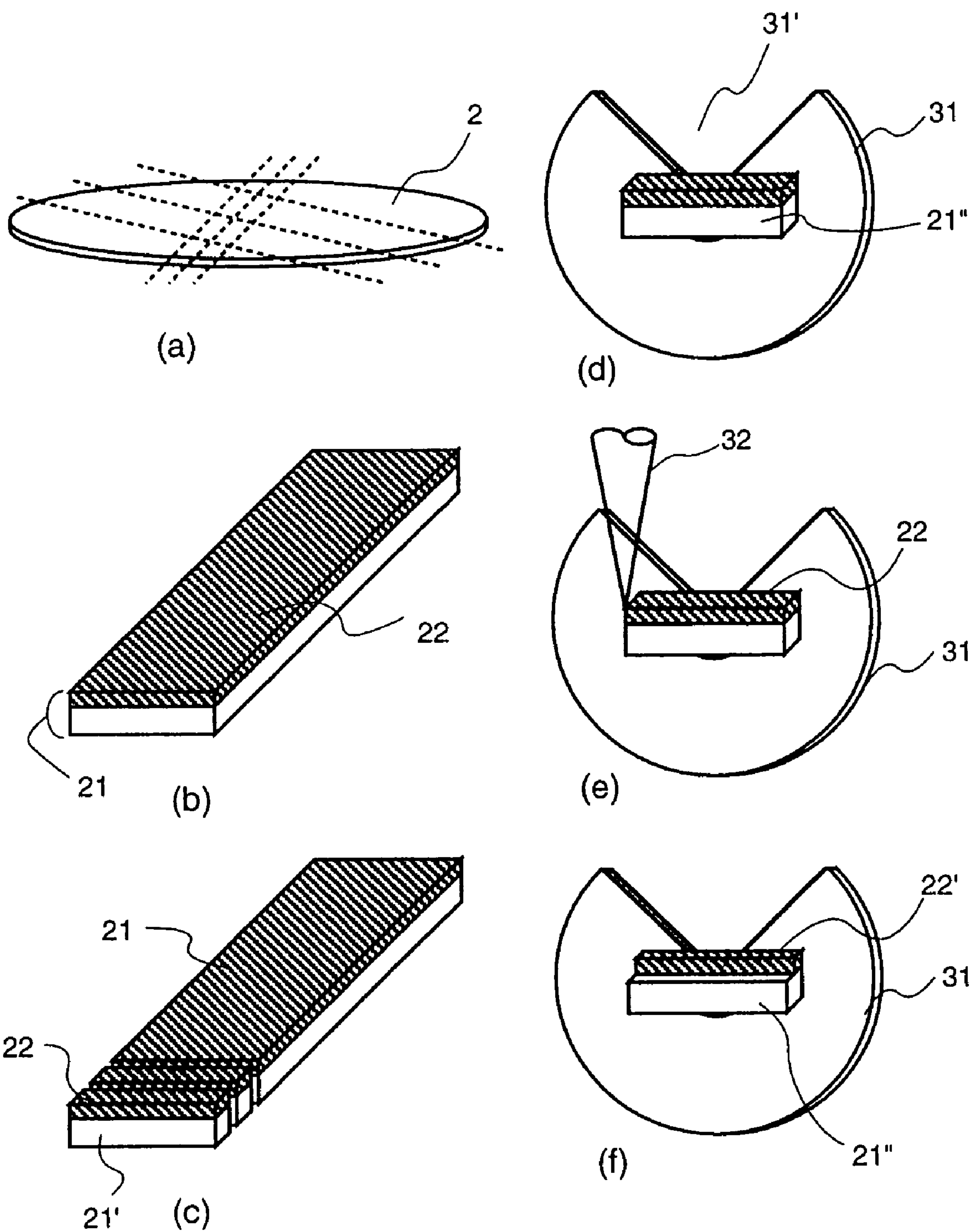
FIG.3 (PRIOR ART)
