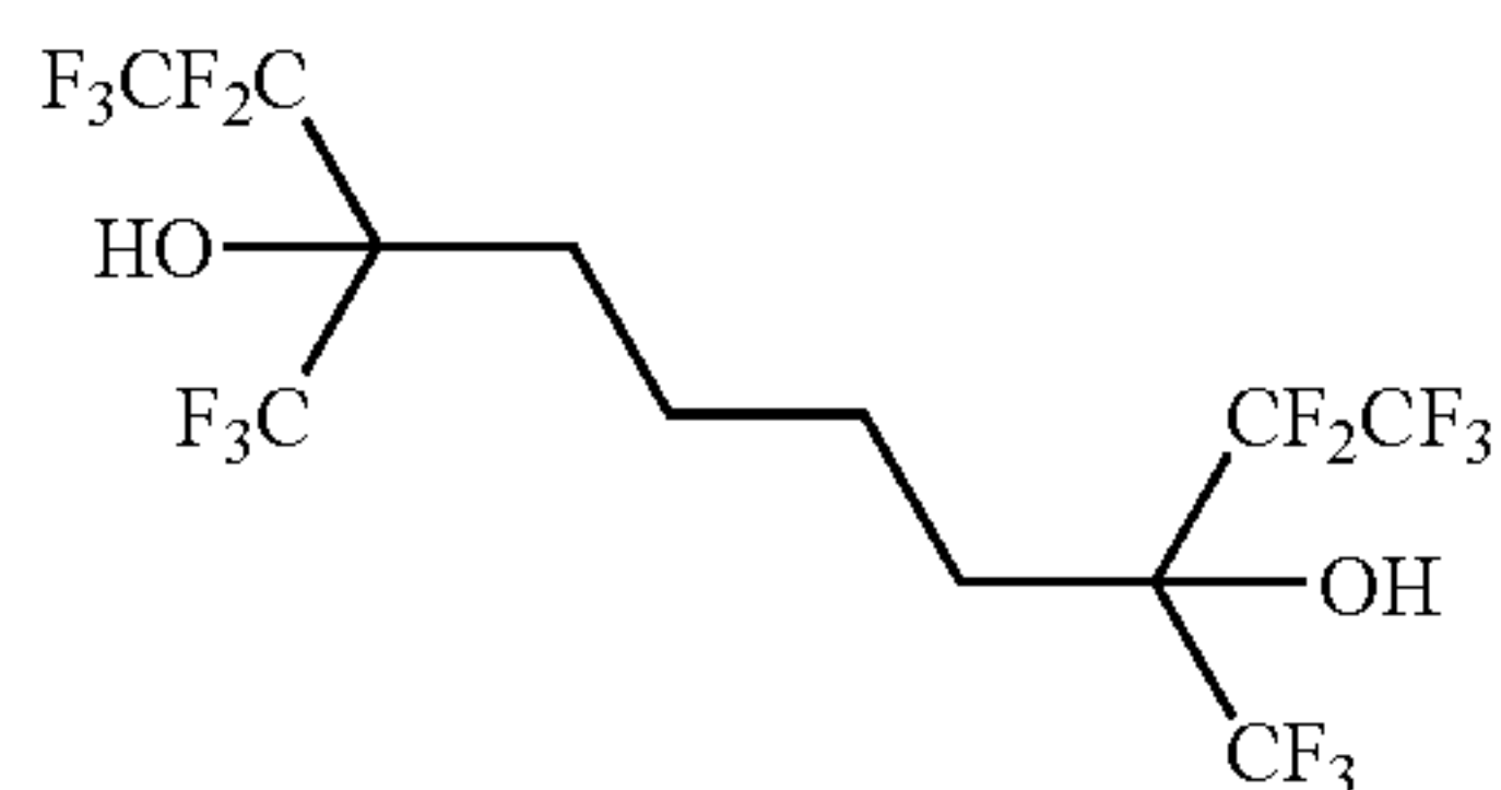
3,8-bis(trifluoromethyl)-1,1,1,2,2,9,9,10,10,10-decafluorodecane-3,8-diol
