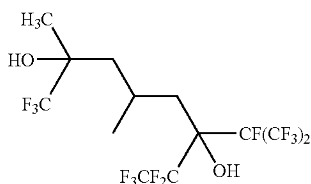
1,1,1,7,7,8,8,8-octafluoro-2,4-dimethyl-6-[1,2,2,2-tetrafluoro-1-(trifluoromethyl)ethyl]octane-2,6-diol
