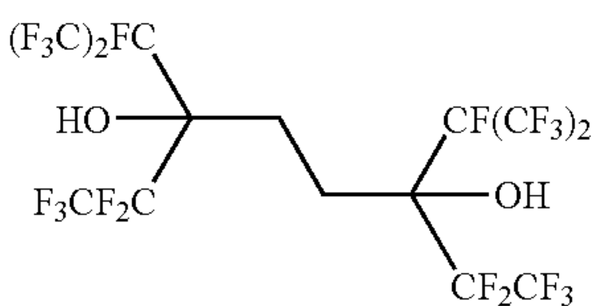
3,6-bis[1,2,2,2-tetrafluoro-1-(trifluoromethyl)ethyl]-1,1,1,2,2,7,7,8,8,8-decafluorooctane-3,6-diol
