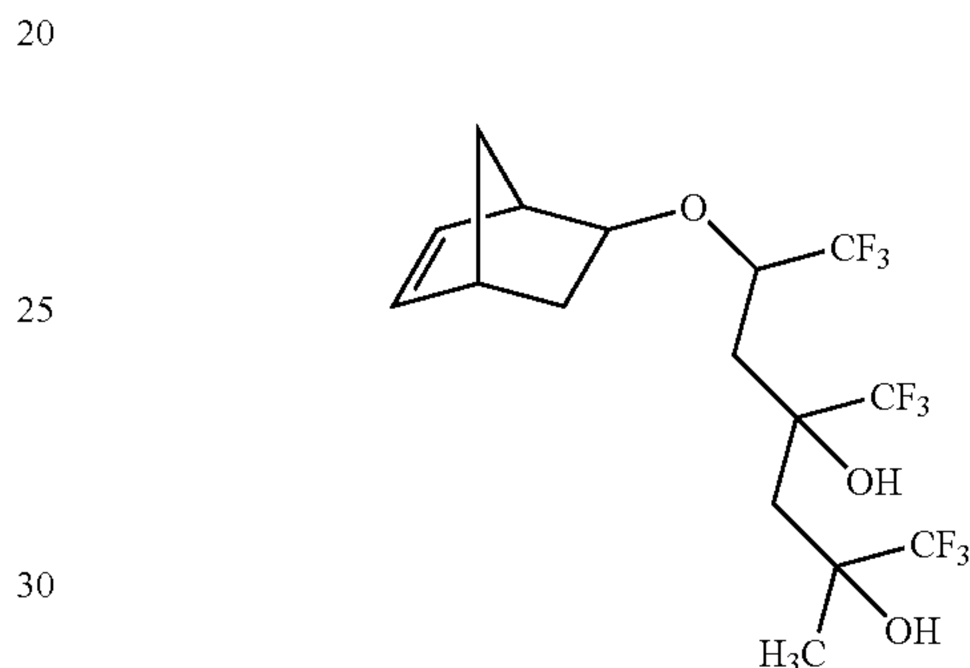
6-bicyclo[2.2.1]hept-5-en-2-yloxy-1,1,1,7,7,7-hexafluoro-2-methyl-4-(trifluoromethyl)heptane-2,4-diol
