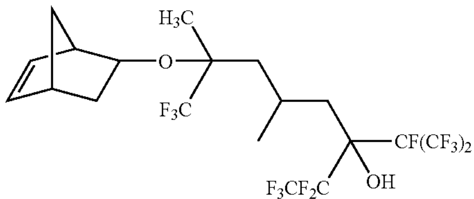
7-bicyclo[2.2.1]hept-5-en-2-yloxy-1,1,1,2,2,8,8,8-octafluoro-5,7-dimethyl-3-[1,2,2,2-tetrafluoro-1-(trifluoromethyl)ethyl]octan-3-ol
