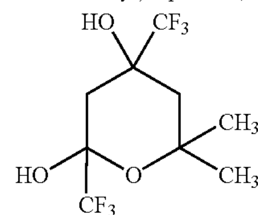
6-methyl-2,4,6-tris(trifluoromethyl)-2H-3,4,5,6-tetrahydropyran-2,4-diol
