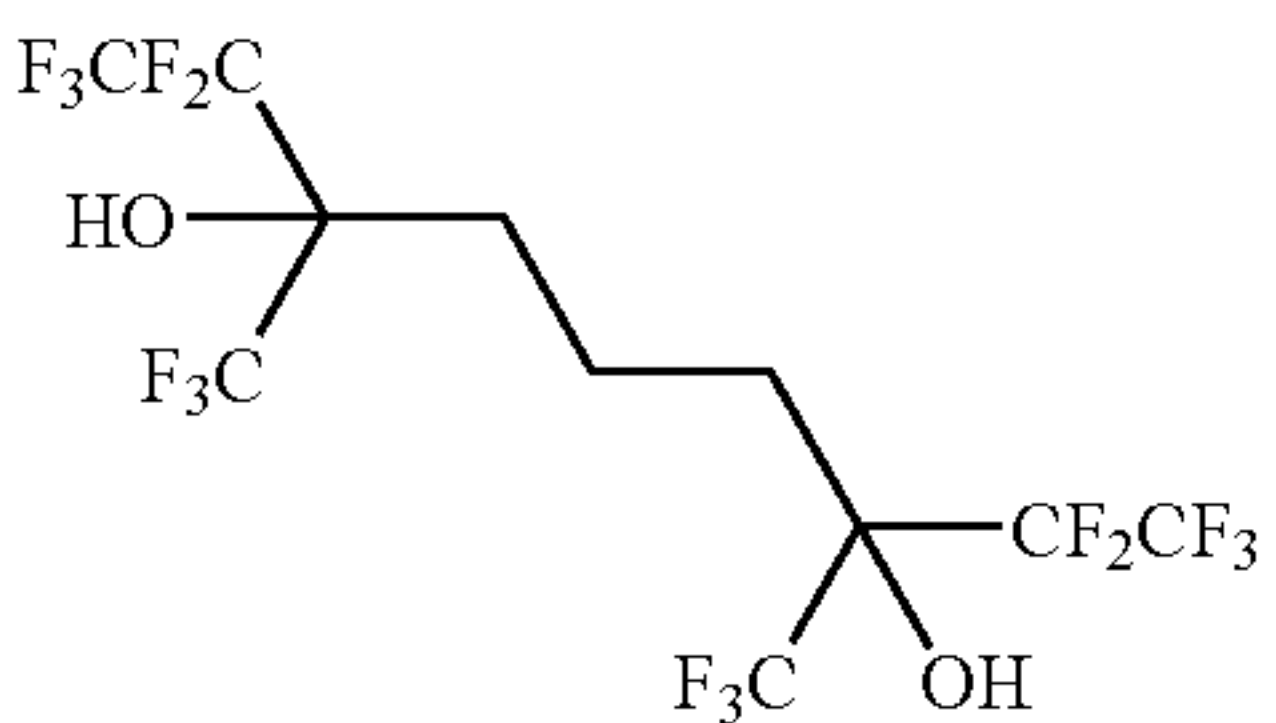
3,7-bis(trifluoromethyl)-1,1,1,2,2,8,8,9,9,9-decafluorononane-3,7-diol
