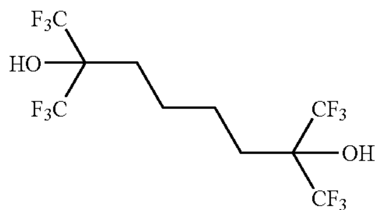
2,7-bis(trifluoromethyl)-1,1,1,8,8,8-hexafluorooctane-2,7-diol
