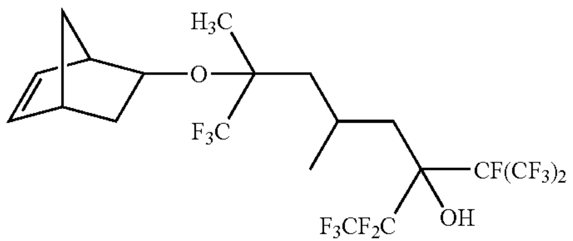
7-bicyclo[2.2.1]hept-5-en-2-yloxy-1,1,1,2,2,8,8,8-octafluoro-5,7-dimethyl-3-[1,2,2,2-tetrafluoro-1-(trifluoromethyl)ethyl]octan-3-ol
