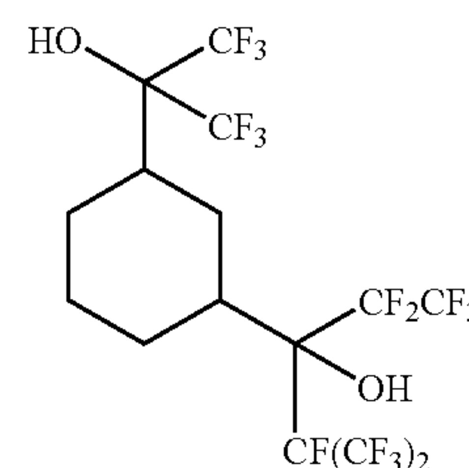
1,1,1,2,2,4,5,5,5-nonafluoro-3-{3-[2,2,2-trifluoro-1-hydroxy-1-(trifluoromethyl)ethyl]cyclohexyl}-4-(trifluoromethyl)pentan-3-ol
