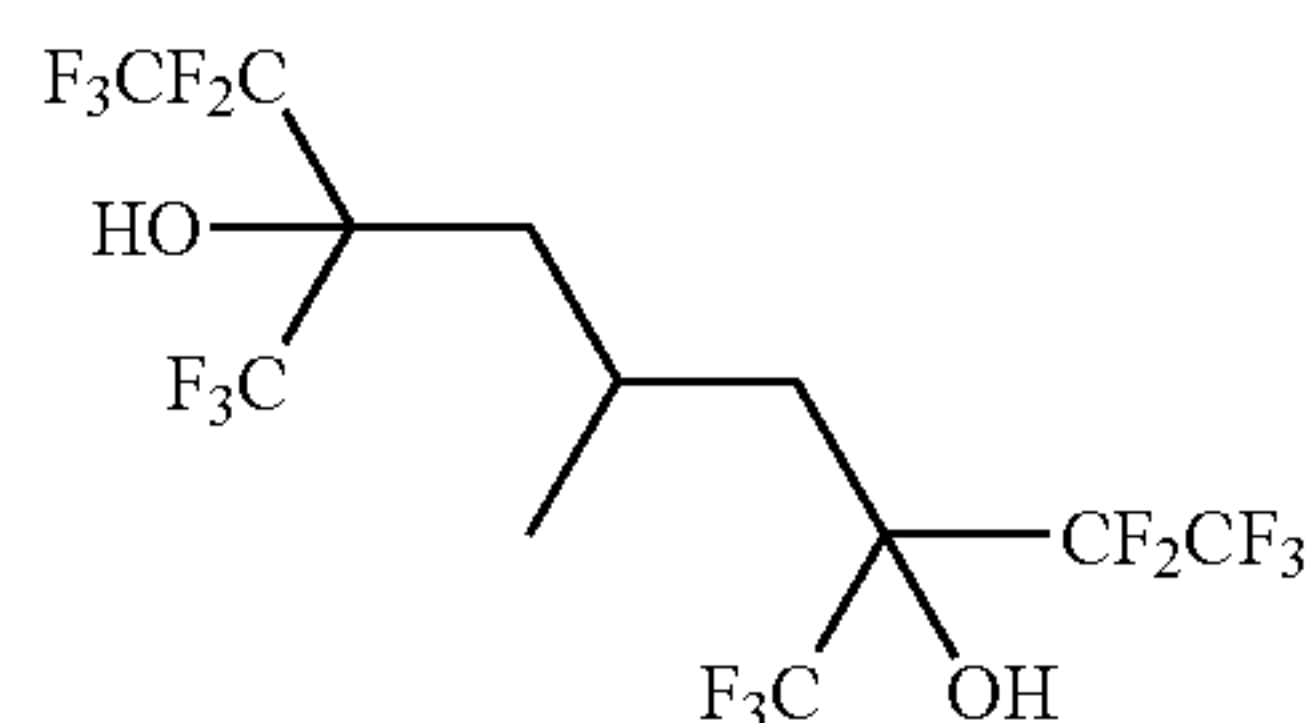
3,7-bis(trifluoromethyl)-1,1,1,2,2,8,8,9,9,9-decafluoro-5-methylnonane-3,7-diol
