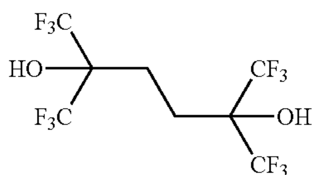
2,5-bis(trifluoromethyl)-1,1,1,6,6,6-hexafluorohexane-2,5-diol
