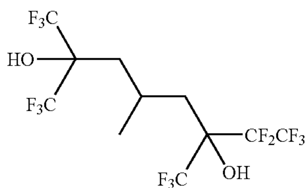
2,6-bis(trifluoromethyl)-1,1,1,7,7,8,8,8-octafluoro-4-methyloctane-2,6-diol
