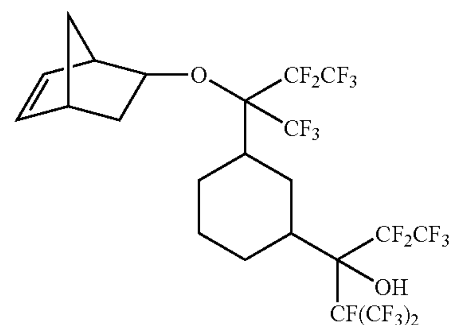
3-{3-[1-Bicyclo[2.2.1]hept-5-en-2-yloxy-2,2,3,3,3-pentafluoro-1-trifluoromethyl-propyl]cyclohexyl}-1,1,1,2,2,4,4,5,5,5-nonafluoro-4-trifluoromethyl-pentan-3-ol
