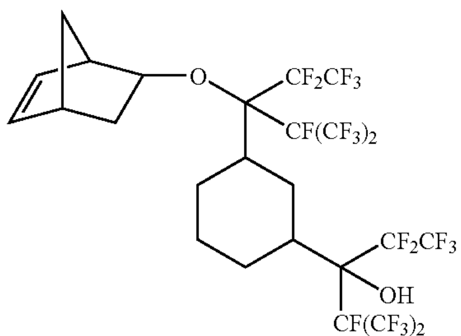
3-{3-[1-bicyclo[2.2.1]hept-5-en-2-yloxy-2,2,3,3,3-pentafluoro-1-[1,2,2,2-tetrafluoro-1-(trifluoromethyl)ethyl]propyl]cyclohexyl}-1,1,1,2,4,4,5,5,5-nonafluoro-2-(trifluoromethyl)pentan-3-ol
