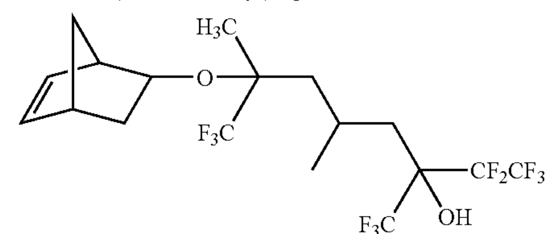
7-bicyclo[2.2.1]hept-5-en-2-yloxy-1,1,1,2,2,8,8,8-octafluoro-5,7-dimethyl-3-(trifluoromethyl)octan-3-ol
