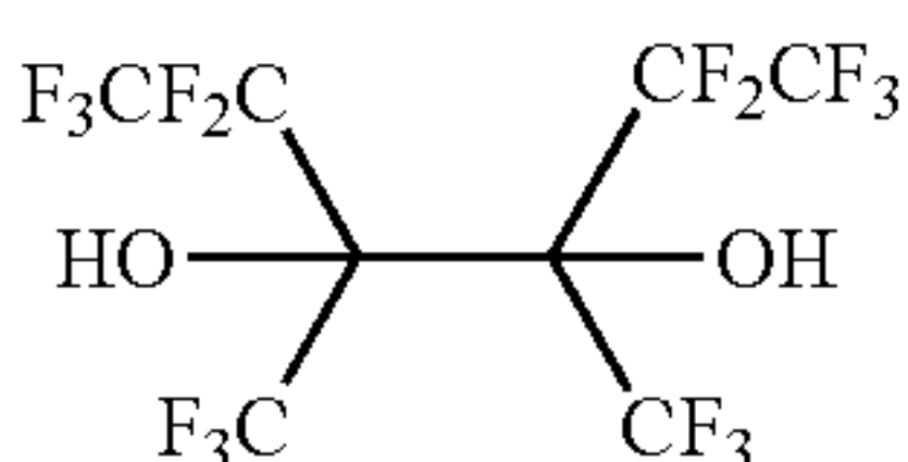
3,4-bis(trifluoromethyl)-1,1,1,2,2,5,5,6,6,6-decafluorohexane-3,4-diol
