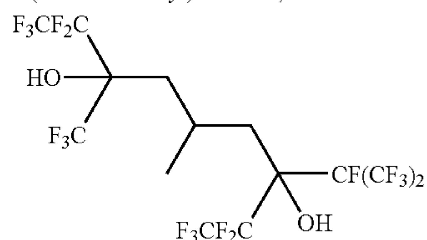
1,1,1,2,2,8,8,9,9,9-decafluoro-5-methyl-3-[1,2,2,2-tetrafluoro-1-(trifluoromethyl)ethyl]-7-(trifluoromethyl)nonane-3,7-diol
