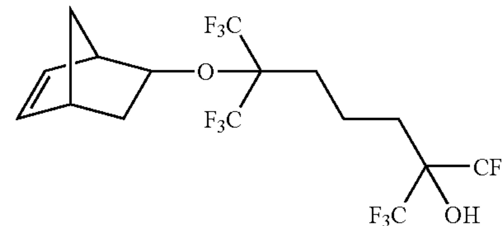
6-bicyclo[2.2.1]hept-5-en-2-yloxy-2,6-bis(trifluoromethyl)-1,1,1,7,7,7-hexafluoroheptan-2-ol
