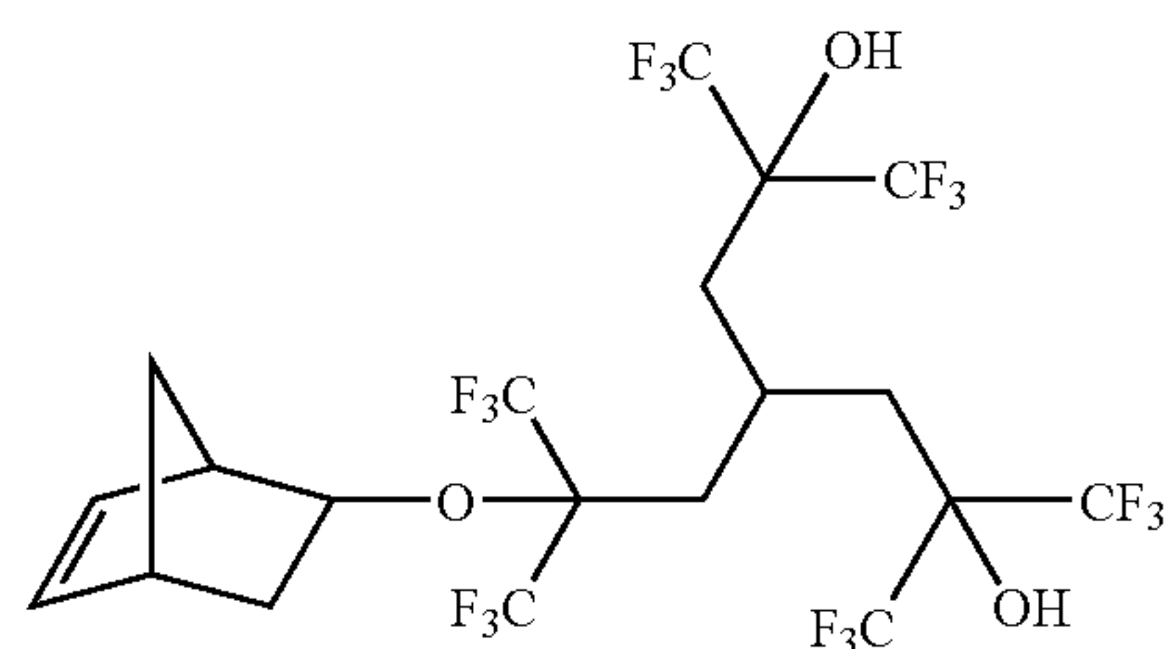
4-[bicyclo[2.2.1]hept-5-en-2-yloxy-3,3,3-trifluoro-2-(trifluoromethyl)propyl]-2,6-bis(trifluoromethyl)-1,1,1,7,7,7-hexafluoroheptane-2,6-diol
