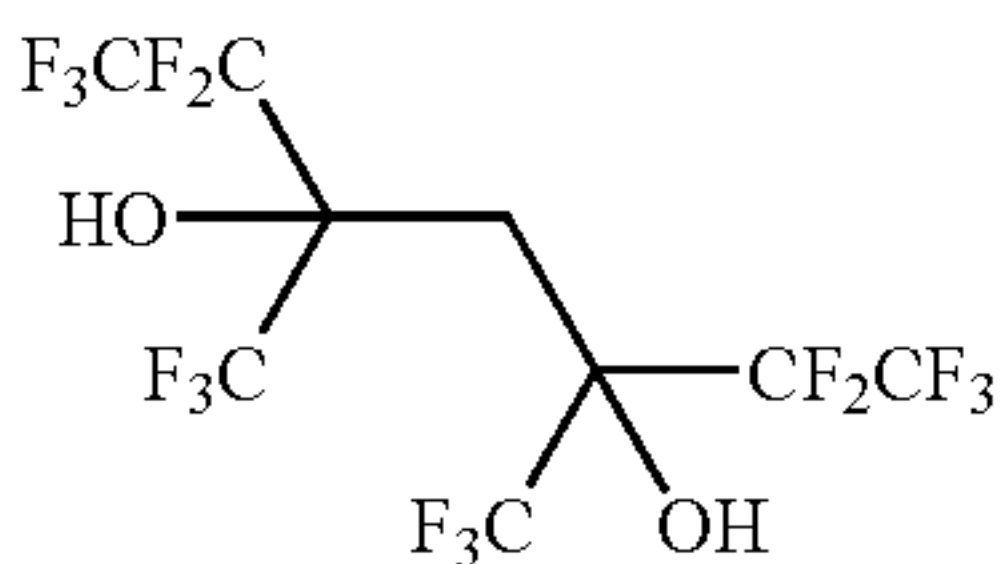
3,5-bis(trifluoromethyl)-1,1,1,2,2,6,6,7,7,7-decafluoroheptane-3,5-diol
