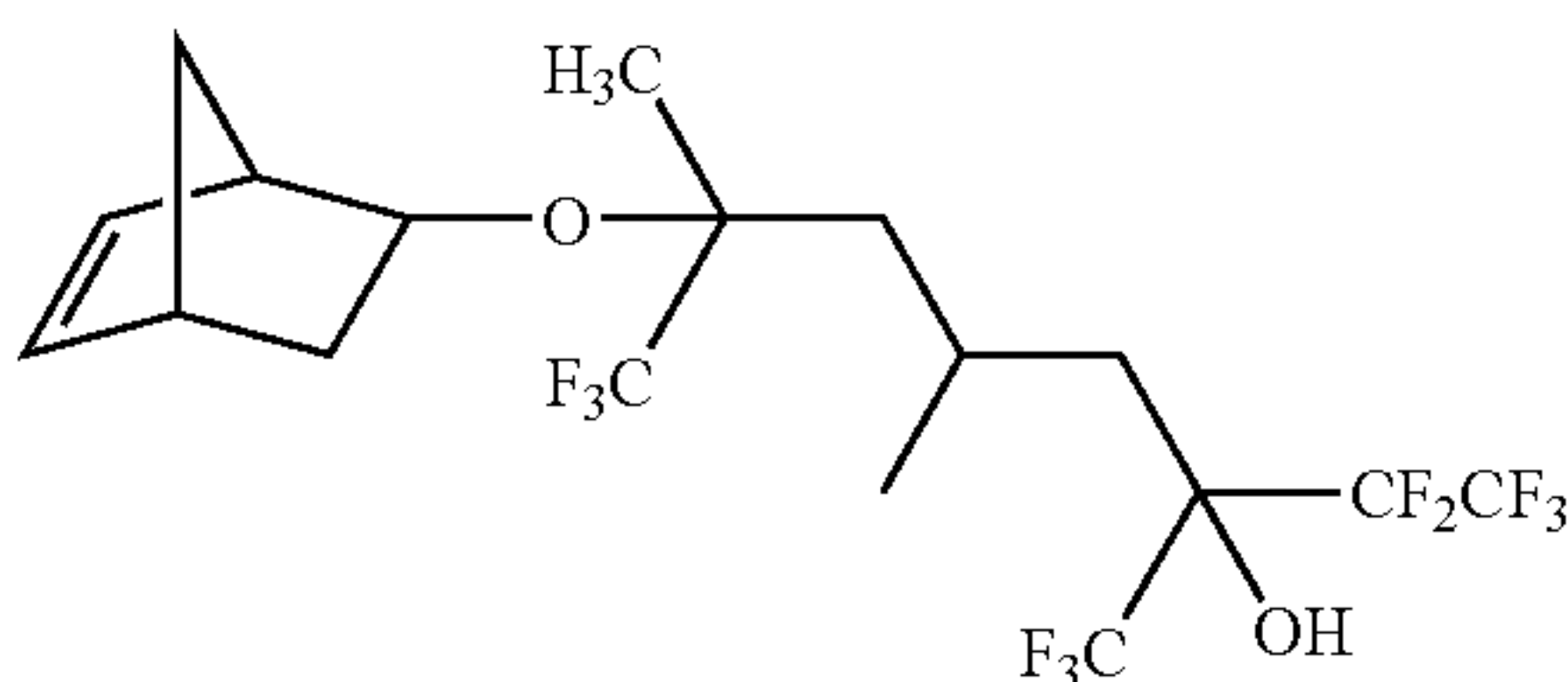
7-bicyclo[2.2.1]hept-5-en-2-yloxy-1,1,1,2,2,8,8,8-octafluoro-5,7-dimethyl-3-(trifluoromethyl)octan-3-ol
