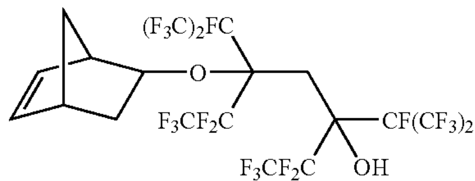
5-bicyclo[2.2.1]hept-5-en-2-yloxy-3,5-bis[1,2,2,2-tetrafluoro-1-(trifluoromethyl)ethyl]-1,1,1,2,2,6,6,7,7,7-decafluoroheptan-3-ol
