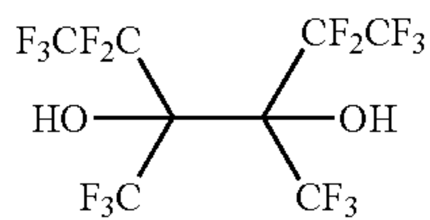
3,4-bis(trifluoromethyl)-1,1,1,2,2,5,5,6,6,6-decafluorohexane-3,4-diol
