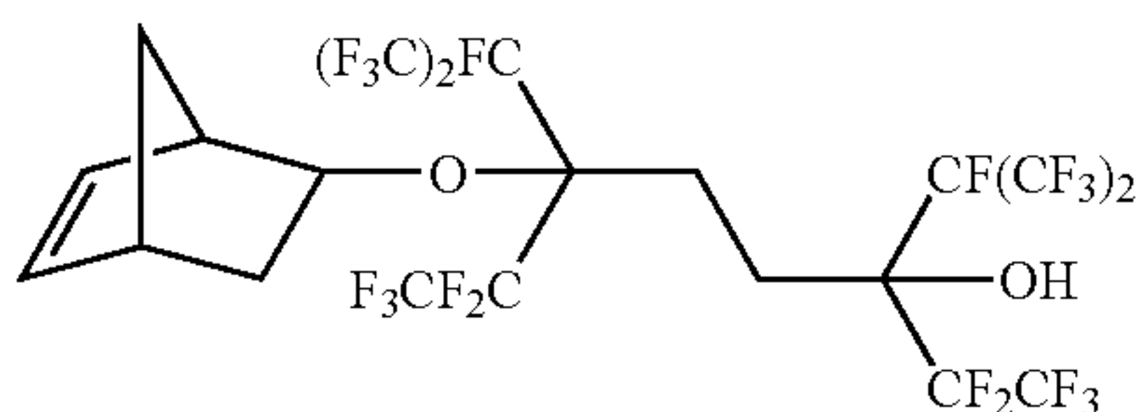
6-bicyclo[2.2.1]hept-5-en-2-yloxy-3,6-bis[1,2,2,2-tetrafluoro-1-(trifluoromethyl)ethyl]-1,1,1,2,2,7,7,8,8,8-decafluorooctan-3-ol
