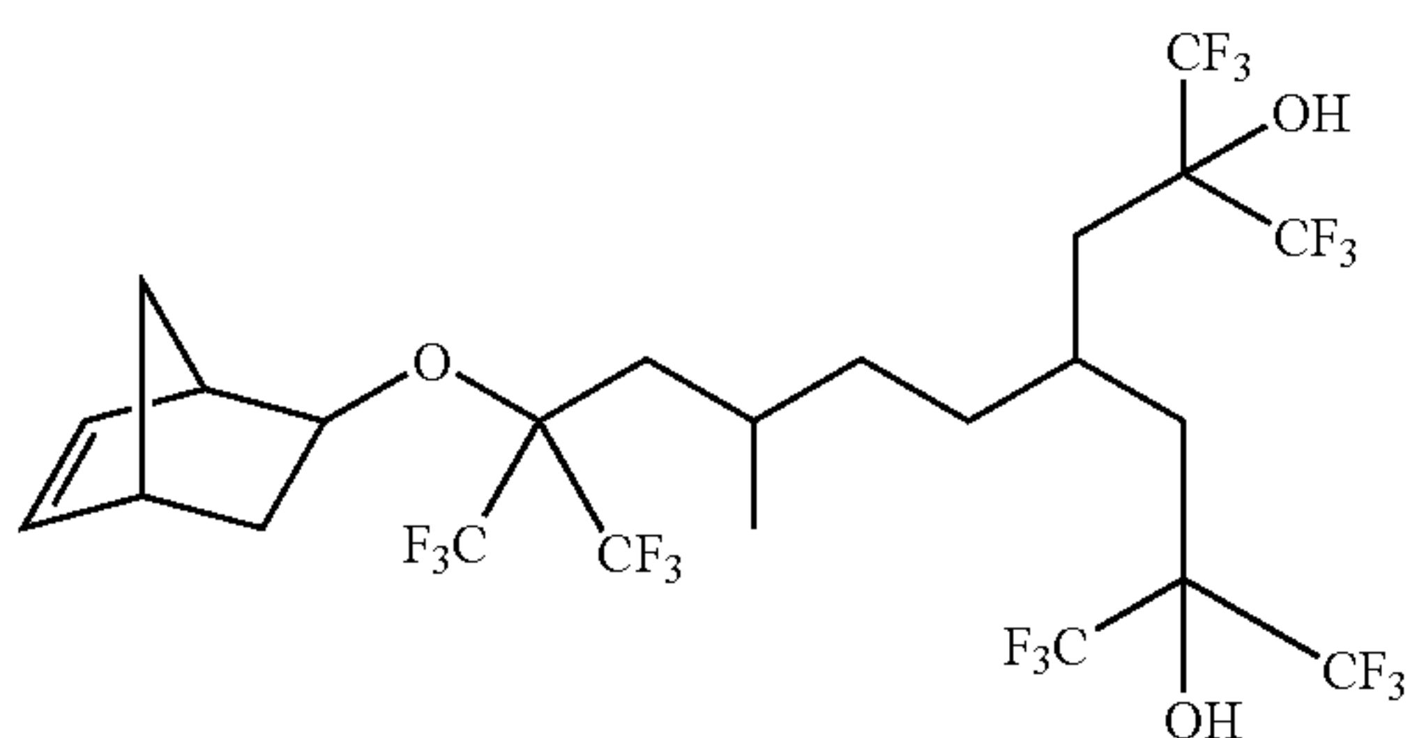
4-[bicyclo[2.2.1]hept-5-en-2-yloxy-6,6,6-trifluoro-3-methyl-5-(trifluoromethyl)hexyl]-2,6-bis(trifluoromethyl)-1,1,1,7,7,7-hexafluoroheptane-2,6-diol
