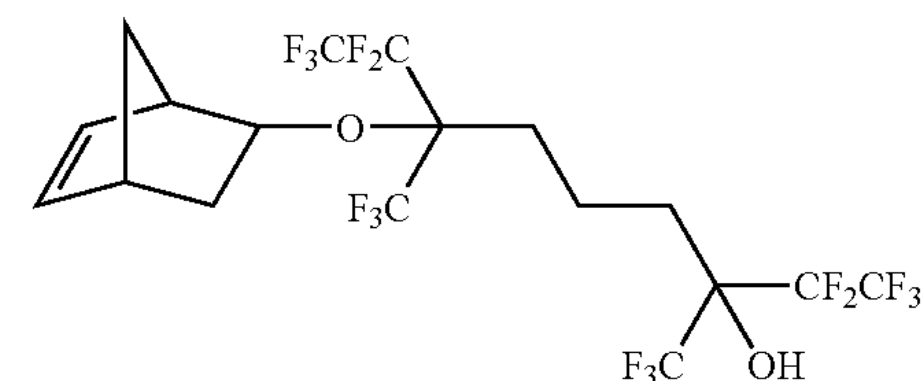
7-bicyclo[2.2.1]hept-5-en-2-yloxy-3,7-bis(trifluoromethyl)-1,1,1,2,2,8,8,9,9,9,9-decafluorononan-3-ol
