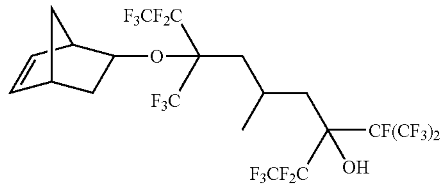
7-bicyclo[2.2.1]hept-5-en-2-yloxy-1,1,1,2,2,8,8,9,9,9-decafluoro-5-methyl-3-[1,2,2,2-tetrafluoro-1-(trifluoromethyl)ethyl]-7-(trifluoromethyl)nonan-3-ol
