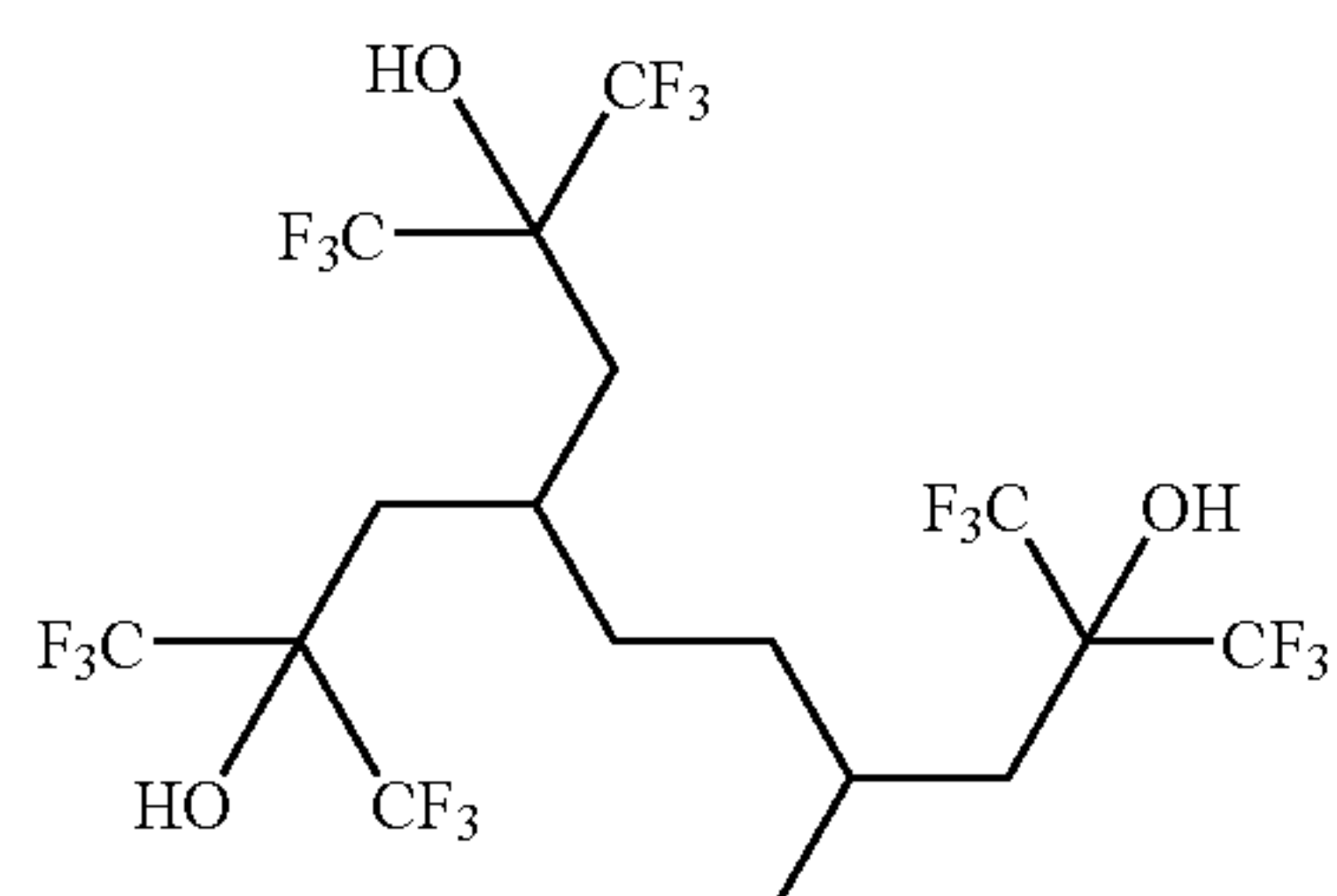
2,9-bis(trifluoromethyl)-1,1,1,10,10,10-hexafluoro-4-methyl-7-[3,3,3-trifluoro-2-hydroxy-2-(trifluoromethyl)propyl]decane-2,9-diol
