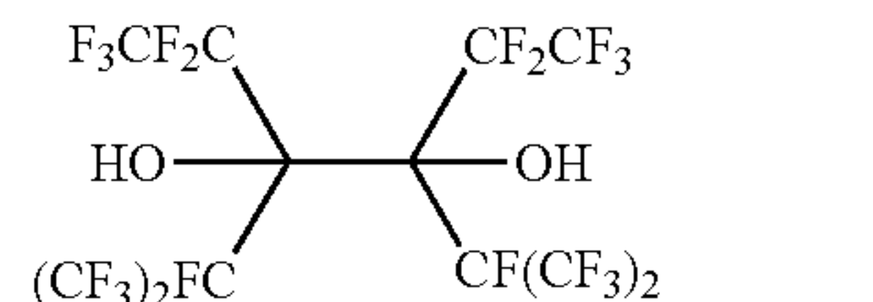
3,4-bis[1,2,2,2-tetrafluoro-1-(trifluoromethyl)ethyl]-1,1,1,2,2,5,5,6,6,6-decafluorohexane-3,4-diol
