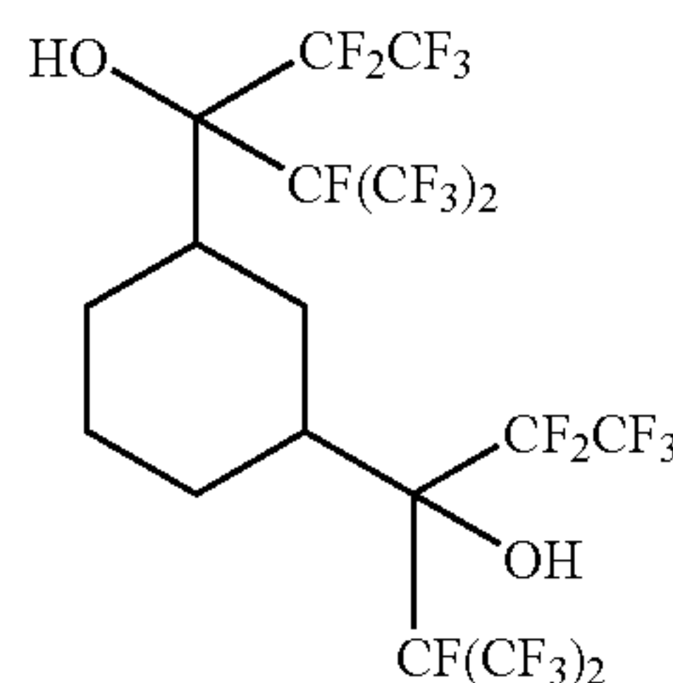
1,1,1,2,4,4,5,5,5-nonafluoro-3-{3-[2,2,3,3,3-pentafluoro-1-hydroxy-1-[1,2,2,2-tetrafluoro-(trifluoromethyl)ethyl]propyl]cyclohexyl}-2-(trifluoromethyl)pentan-3-ol
