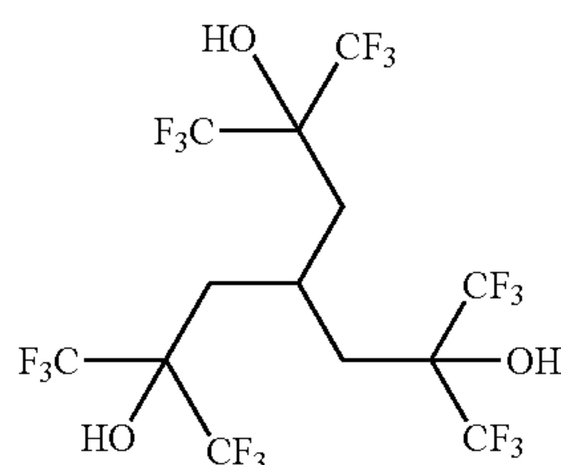
2,6-bis(trifluoromethyl)-1,1,1,7,7,7-hexafluoro-4-[3,3,3-trifluoro-2-hydroxy-2-(trifluoromethyl)propyl]heptane-2,6-diol
