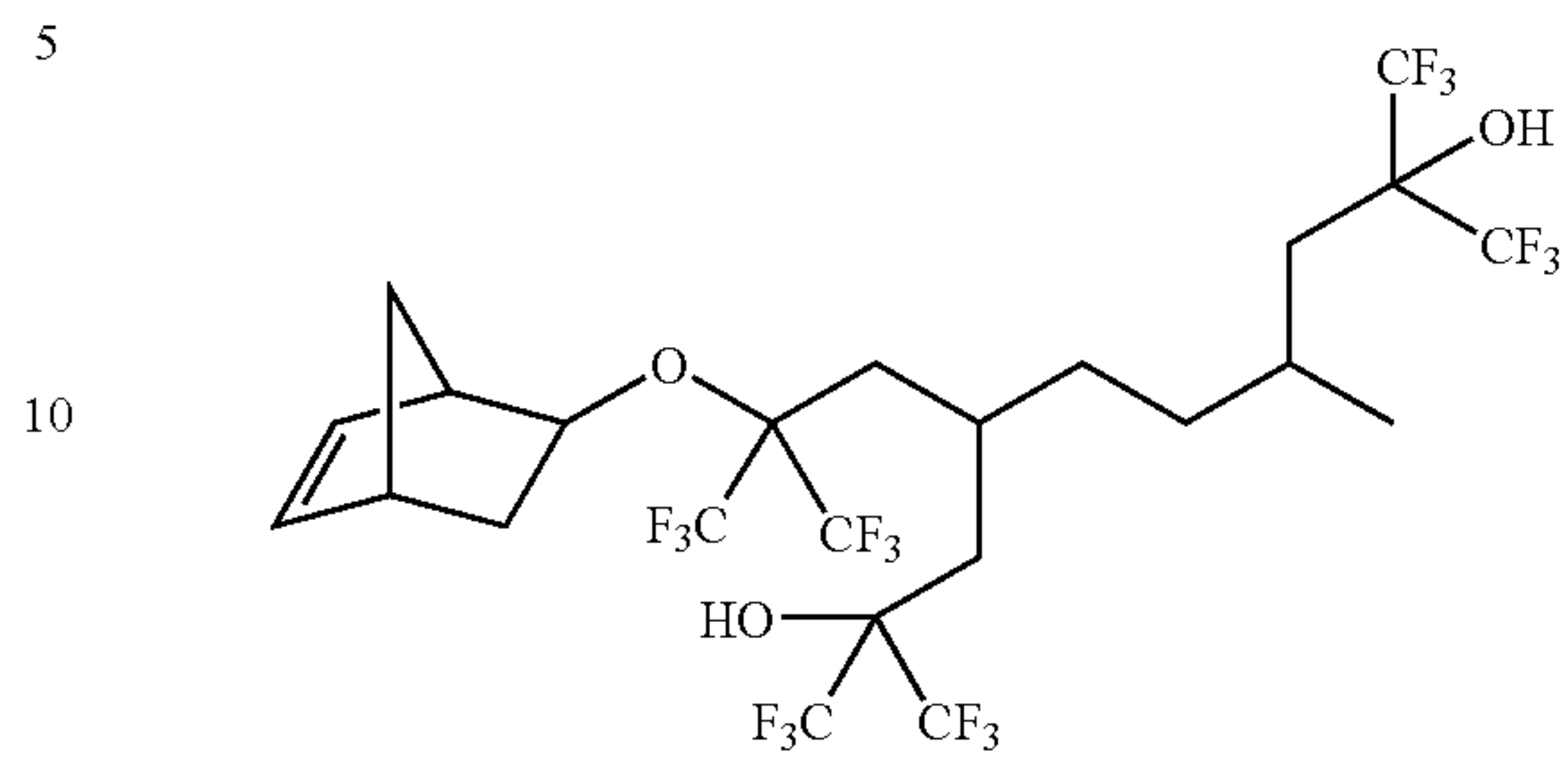
4-[bicyclo[2.2.1]hept-5-en-2-yloxy-3,3,3-trifluoro-2-(trifluoromethyl)propyl]-2,9-bis(trifluoromethyl)-1,1,1,10,10,10-hexafluoro-7-methyldecane-2,9-diol
