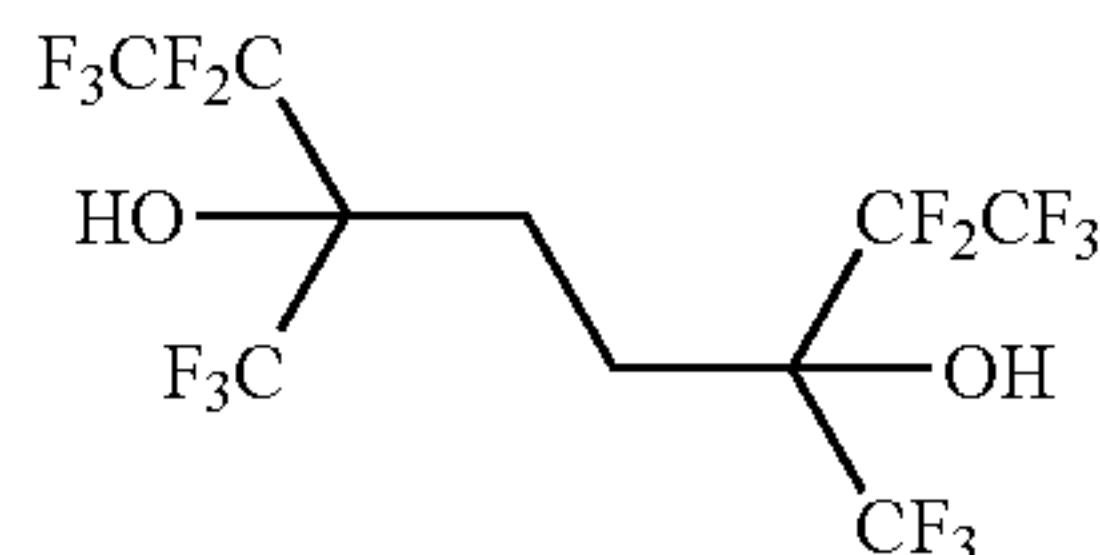
3,6-bis(trifluoromethyl)-1,1,1,2,2,7,7,8,8,8-nonafluorooctane-3,6-diol
