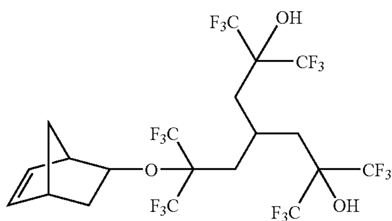
4-[bicyclo[2.2.1]hept-5-en-2-yloxy-3,3,3-trifluoro-2-(trifluoromethyl)-propyl]-2,6-bis(trifluoromethyl)-1,1,1,7,7,7-hexafluoroheptane-2,6-diol
