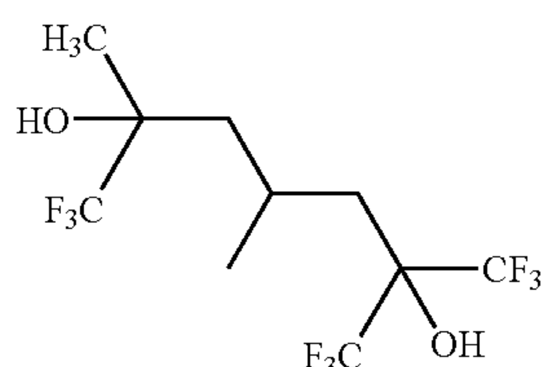
1,1,1,7,7,7-hexafluoro-2,4-dimethyl-6-(trifluoromethyl)heptane-2,6-diol
