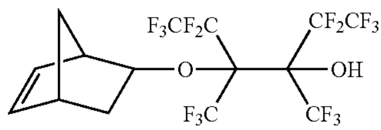
4-bicyclo[2.2.1]hept-5-en-2-yloxy-3,4-bis(trifluoromethyl)-1,1,1,2,2,5,5,6,6,6-decafluorohexan-3-ol
