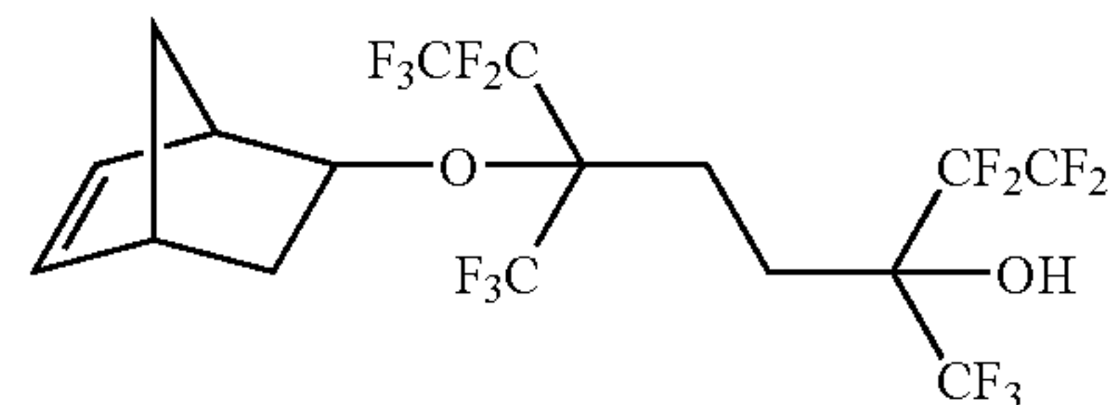
6-bicyclo[2.2.1]hept-5-en-2-yloxy-3,6-bis(trifluoromethyl)-1,1,1,2,2,7,7,8,8,8-nonafluorooctan-3-ol
