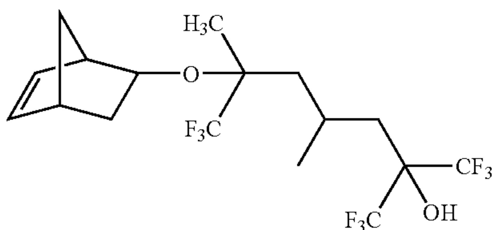
6-bicyclo[2.2.1]hept-5-en-2-yloxy-1,1,1,7,7,7-hexafluoro-4,6-dimethyl-2-(trifluoromethyl)heptan-2-ol
