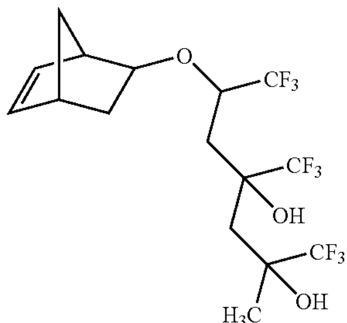
6-bicyclo[2.2.1]hept-5-en-2-yloxy-1,1,1,7,7,7-hexafluoro-2-methyl-4-(trifluoromethyl)heptane-2,4-diol
