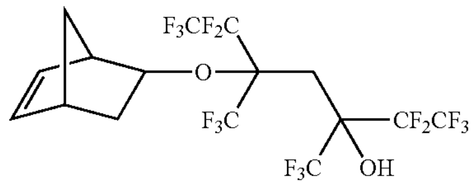
5-bicyclo[2.2.1]hept-5-en-2-yloxy-3,5-bis(trifluoromethyl)-1,1,1,2,2,6,6,7,7,7-decafluoroheptan-3-ol
