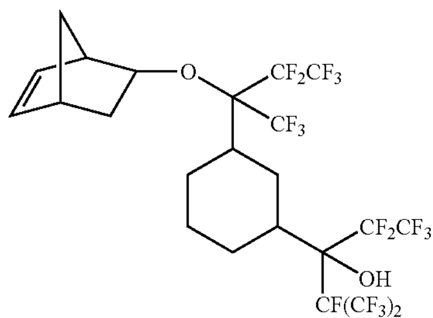
3-{3-[1-Bicyclo[2.2.1]hept-5-en-2-yloxy-2,2,3,3,3-pentafluoro-1-trifluoromethyl-propyl]-cyclohexyl}-1,1,1,2,2,4,5,5,5-nonafluoro-4-trifluoromethyl-pentan-3-ol
