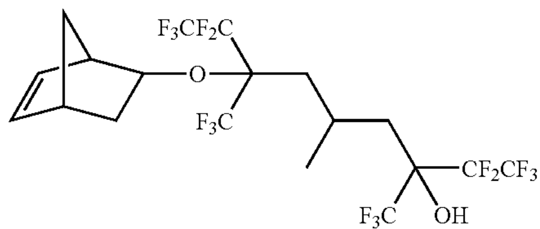
7-bicyclo[2.2.1]hept-5-en-2-yloxy-3,7-bis(trifluoromethyl)-1,1,1,2,2,8,8,9,9,9-decafluoro-5-methylnonan-3-ol
