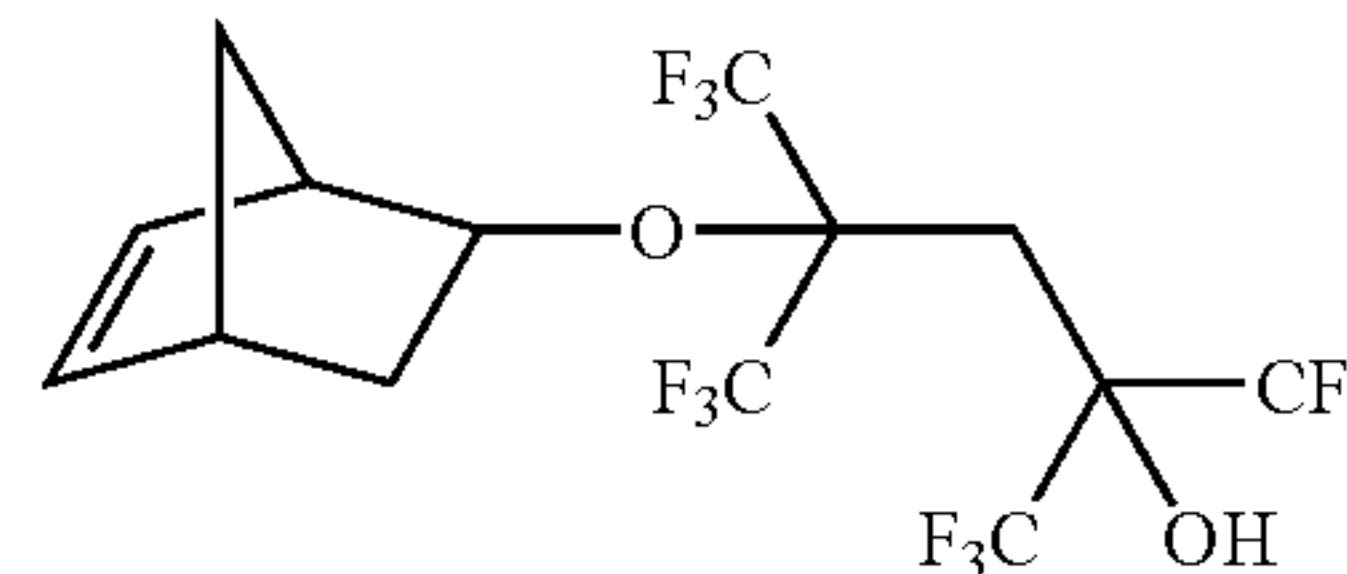
4-bicyclo[2.2.1]hept-5-en-2-yloxy-2,4-bis(trifluoromethyl)-1,1,1,5,5,5-hexafluoropentan-2-ol
