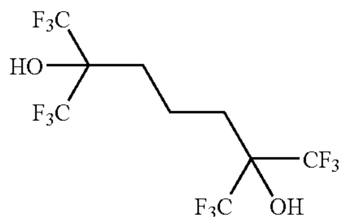
2,6-bis(trifluoromethyl)-1,1,1,7,7,7-hexafluoroheptane-2,6-diol
