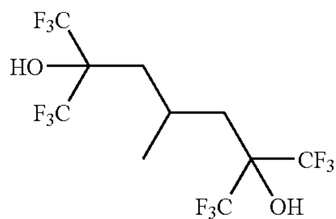
2,6-bis(trifluoromethyl)-1,1,1,7,7,7-hexafluoro-4-methylheptane-2,6-diol
