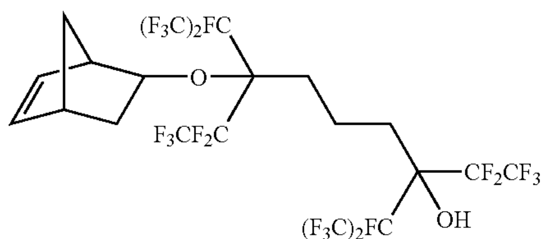
7-bicyclo[2.2.1]hept-5-en-2-yloxy-3,7-bis[1,2,2,2-tetrafluoro-1-(trifluoromethyl)ethyl]-1,1,1,2,2,8,8,9,9,9-decafluorononan-3-ol
