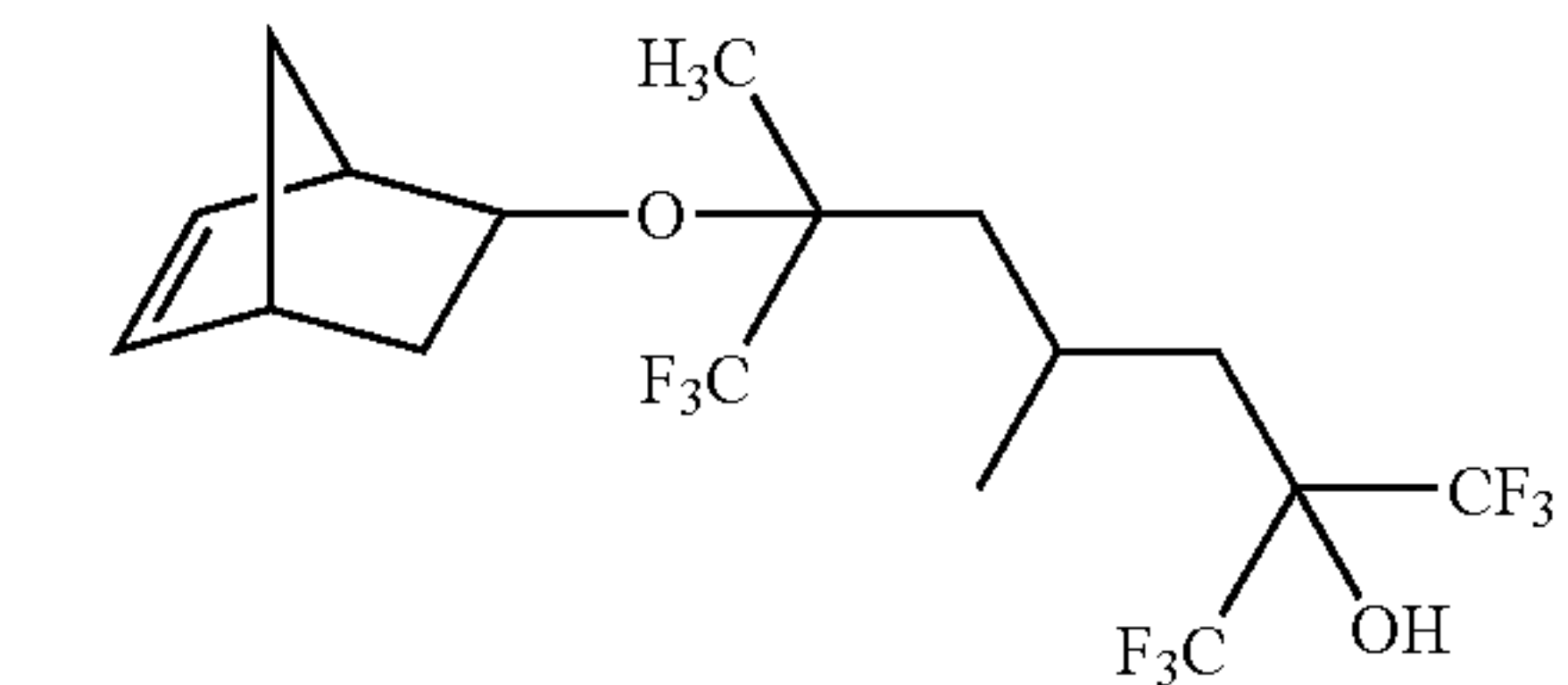
6-bicyclo[2.2.1]hept-5-en-2-yloxy-1,1,1,7,7,7-hexafluoro-4,6-dimethyl-2-(trifluoromethyl)heptan-2-ol
