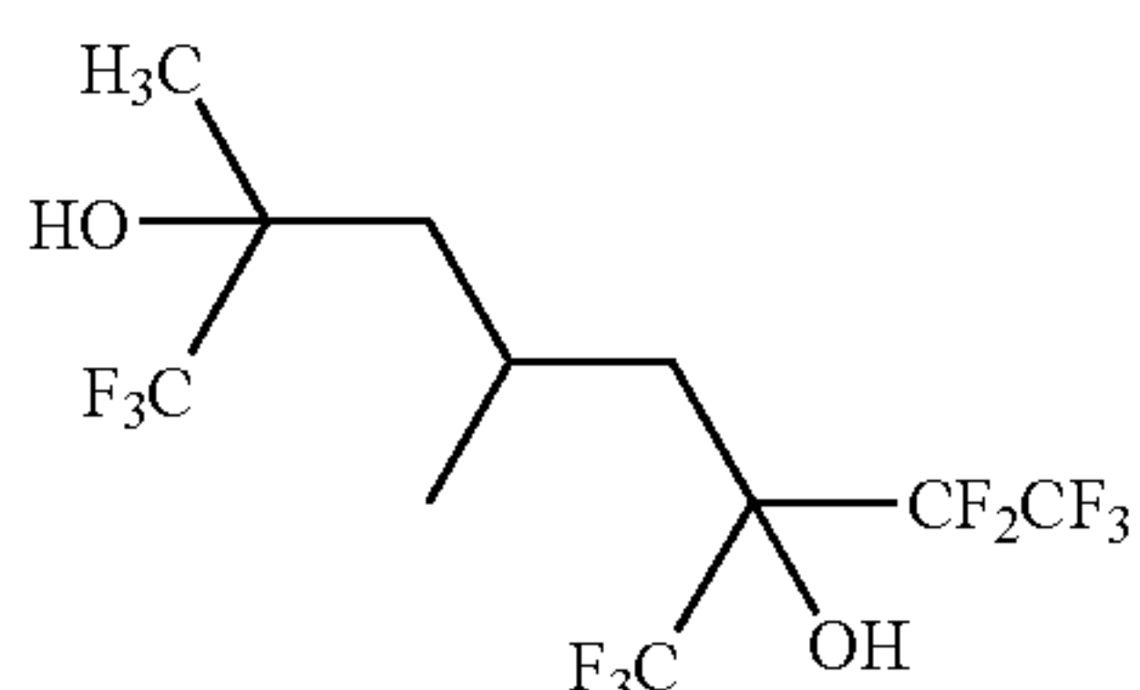
1,1,1,7,7,8,8,8-octafluoro-2,4-dimethyl-6-(trifluoromethyl)octane-2,6-diol
