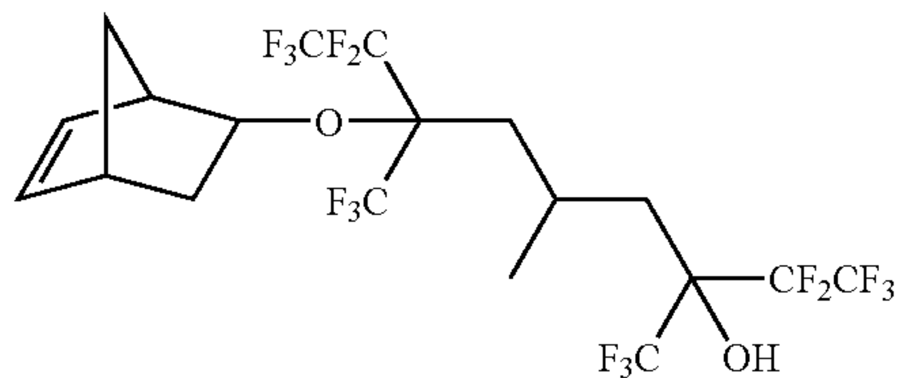
7-bicyclo[2.2.1]hept-5-en-2-yloxy-3,7-bis(trifluoromethyl)-1,1,1,2,2,8,8,9,9,9-decafluoro-5-methylnonan-3-ol
