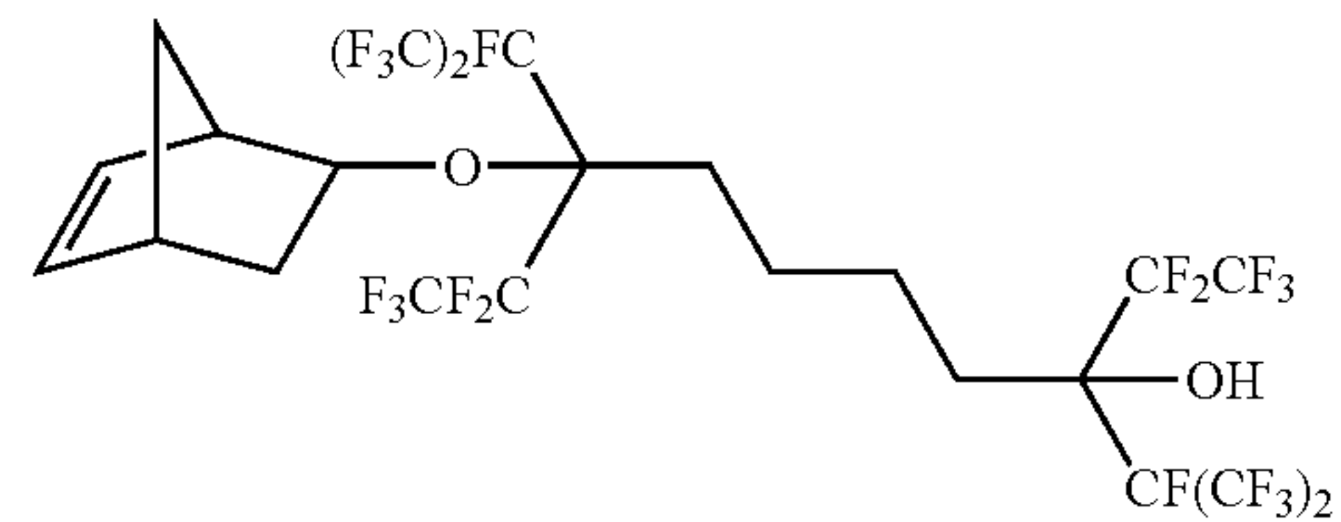
7-bicyclo[2.2.1]hept-5-en-2-yloxy-3,7-bis[1,2,2,2-tetrafluoro-1-(trifluoromethyl)ethyl]-1,1,1,2,2,8,8,9,9,9-decafluorononan-3-ol
