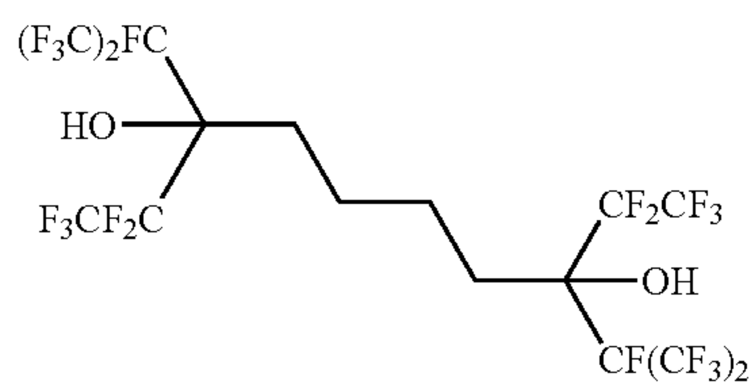
3,8-bis[1,2,2,2-tetrafluoro-1-(trifluoromethyl)ethyl]-1,1,1,2,2,9,9,10,10,10-decafluorodecane-3,8-diol
