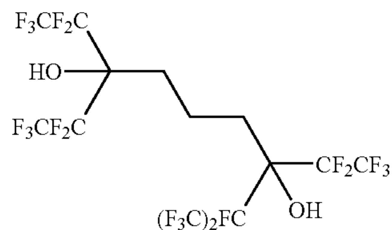
3,7-bis[1,2,2,2-tetrafluoro-1-(trifluoromethyl)ethyl]-1,1,1,2,2,8,8,9,9,9-decafluorononane-3,7-diol
