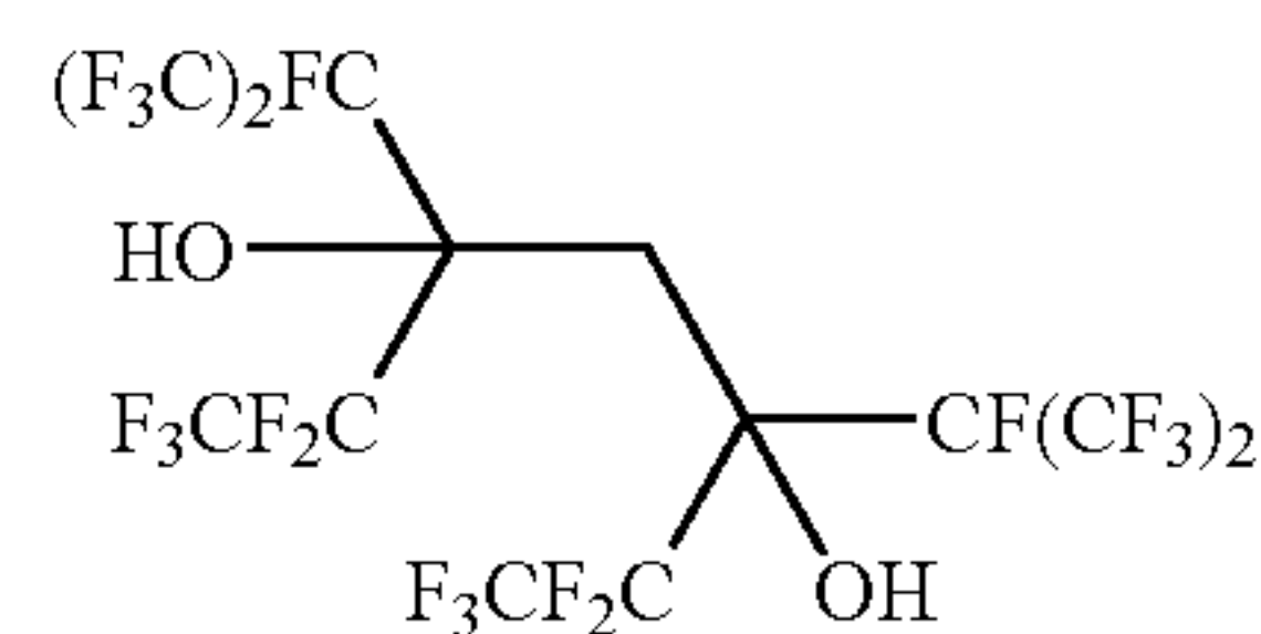
3,5-bis[1,2,2,2-tetrafluoro-1-(trifluoromethyl)ethyl]-1,1,1,2,2,6,6,7,7,7-decafluoroheptane-3,5-diol
