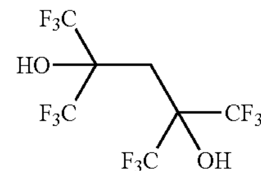
2,4-bis(trifluoromethyl)-1,1,1,5,5,5-hexafluoropentane-2,4-diol
