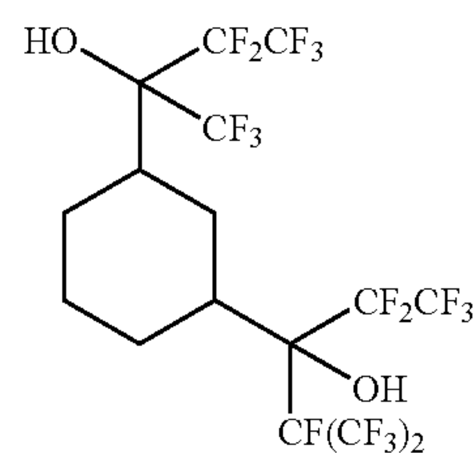
1,1,1,2,2,4,5,5,5-nonafluoro-3-{3-[2,2,3,3,3-pentafluoro-1-hydroxy-1-(trifluoromethyl)propyl]cyclohexyl}-4-(trifluoromethyl)pentan-3-ol
