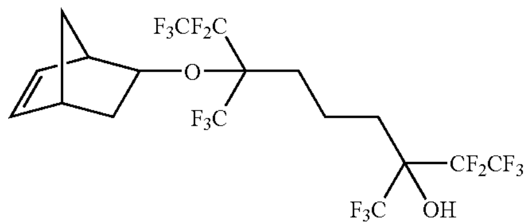
7-bicyclo[2.2.1]hept-5-en-2-yloxy-3,7-bis(trifluoromethyl)-1,1,1,2,2,8,8,9,9,9-decafluorononan-3-ol
