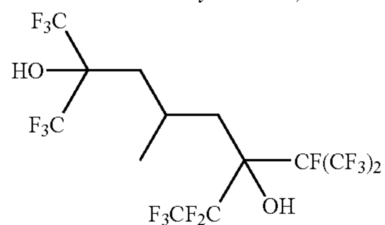
1,1,1,7,7,8,8,8-octafluoro-4-methyl-6-[1,2,2,2-tetrafluoro-1-(trifluoromethyl)ethyl]-2-(trifluoromethyl)octane-2,6-diol
