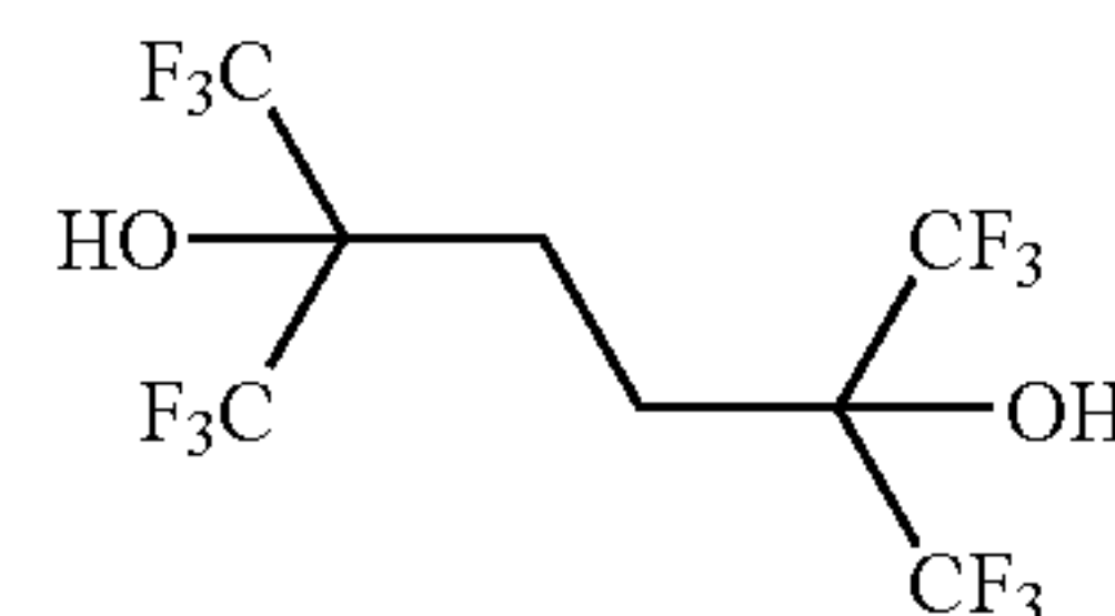
2,5-bis(trifluoromethyl)-1,1,1,6,6,6-hexafluorohexane-2,5-diol
