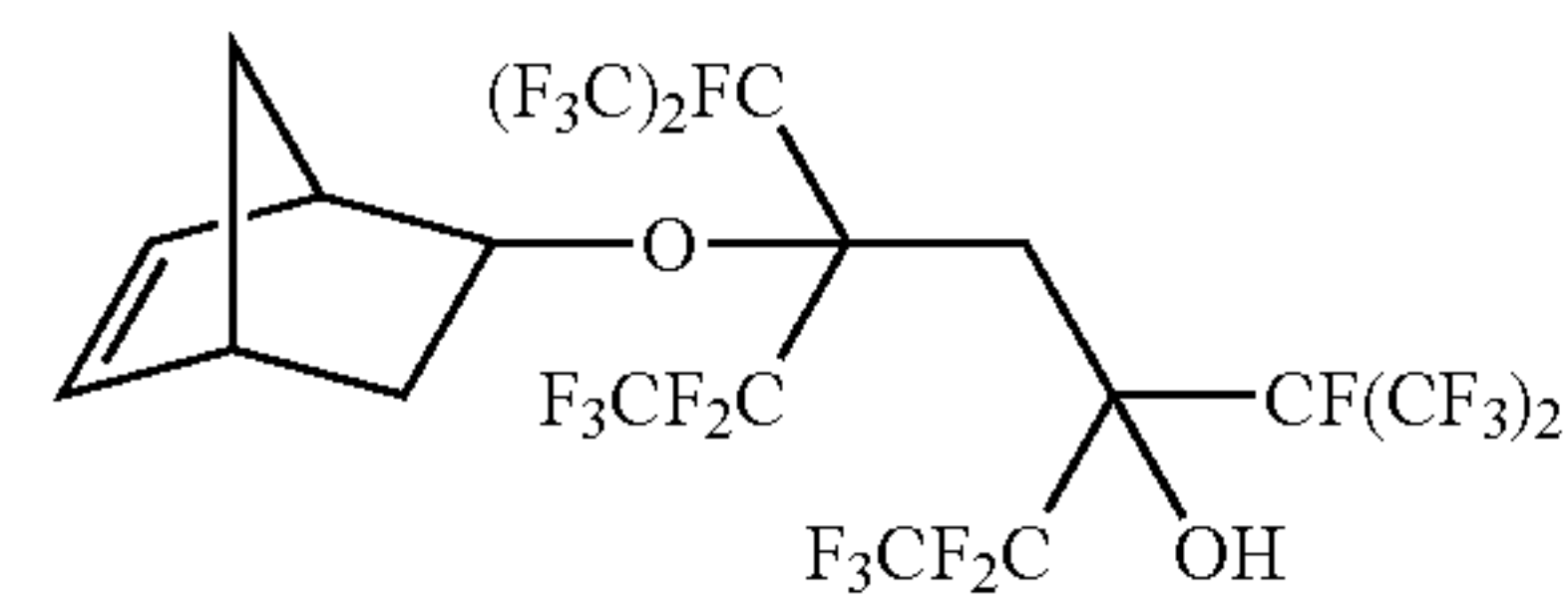
5-bicyclo[2.2.1]hept-5-en-2-yloxy-3,5-bis[1,2,2,2-tetrafluoro-1-(trifluoromethyl)ethyl]-1,1,1,2,2,6,6,7,7,7-decafluoroheptan-3-ol
