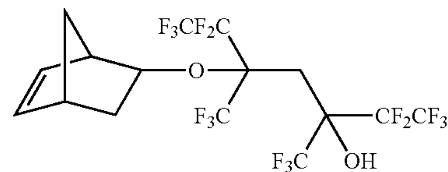
5-bicyclo[2.2.1]hept-5-en-2-yloxy-3,5-bis(trifluoromethyl)-1,1,1,2,2,6,6,7,7,7,7-decafluoroheptan-3-ol
