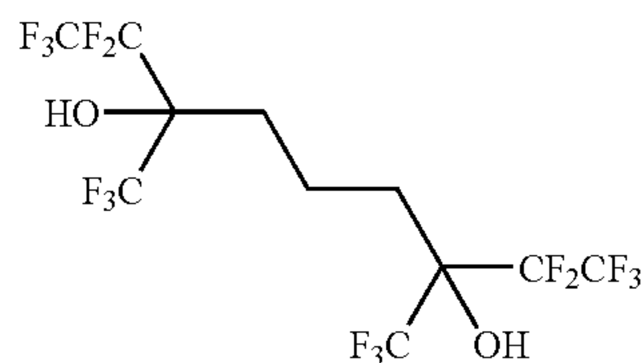
3,7-bis(trifluoromethyl)-1,1,1,2,2,8,8,9,9,9-decafluorononane-3,7-diol
