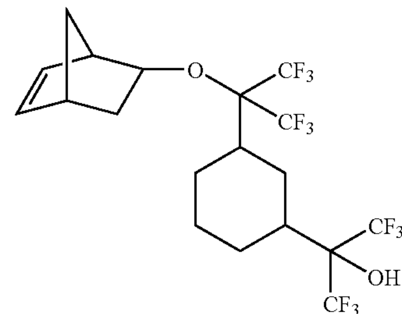
2-{3-[1-bicyclo[2.2.1]hept-5-en-2-yloxy-2,2,2-trifluoro-1-(trifluoromethyl)ethyl]cyclohexyl}-1,1,1,3,3,3-hexafluoropropan-2-ol
