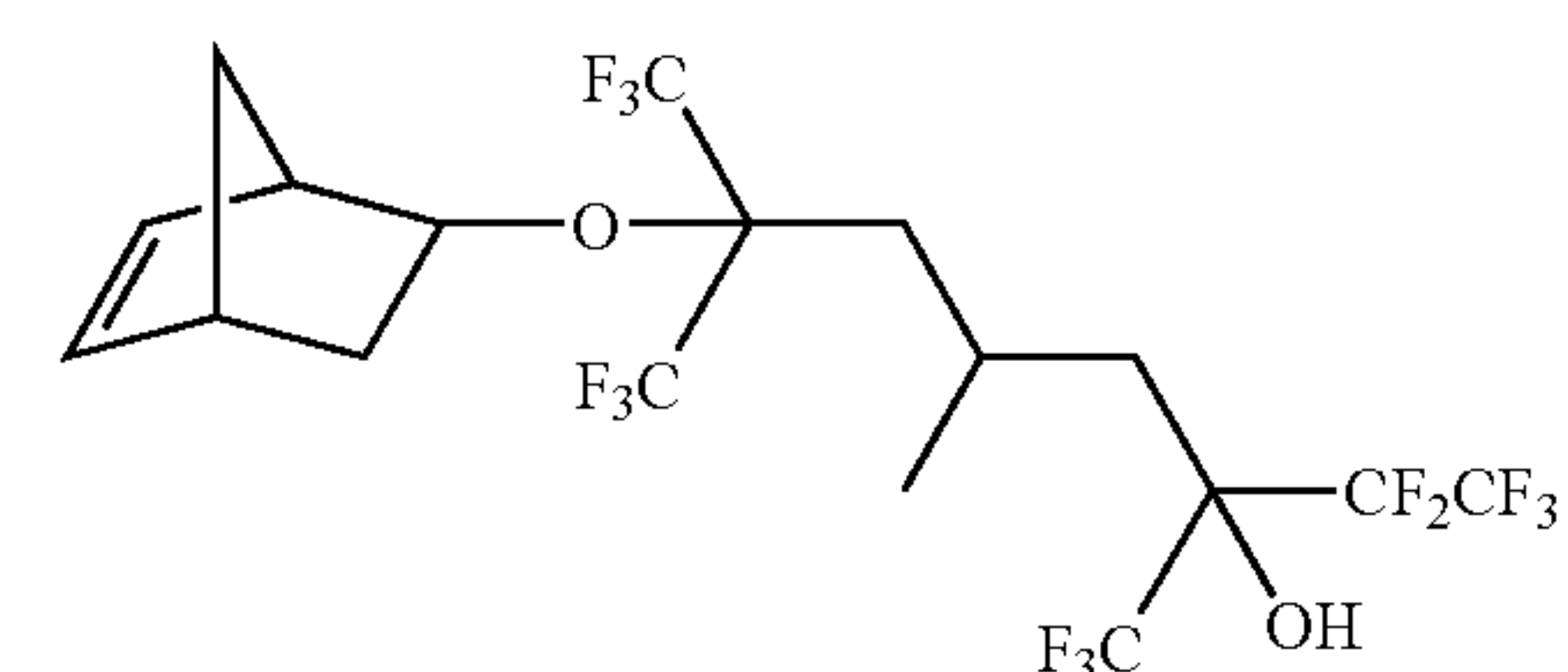
7-bicyclo[2.2.1]hept-5-en-2-yloxy-3,7-bis(trifluoromethyl)-1,1,1,2,2,8,8,8-octafluoro-5-methyloctan-3-ol
