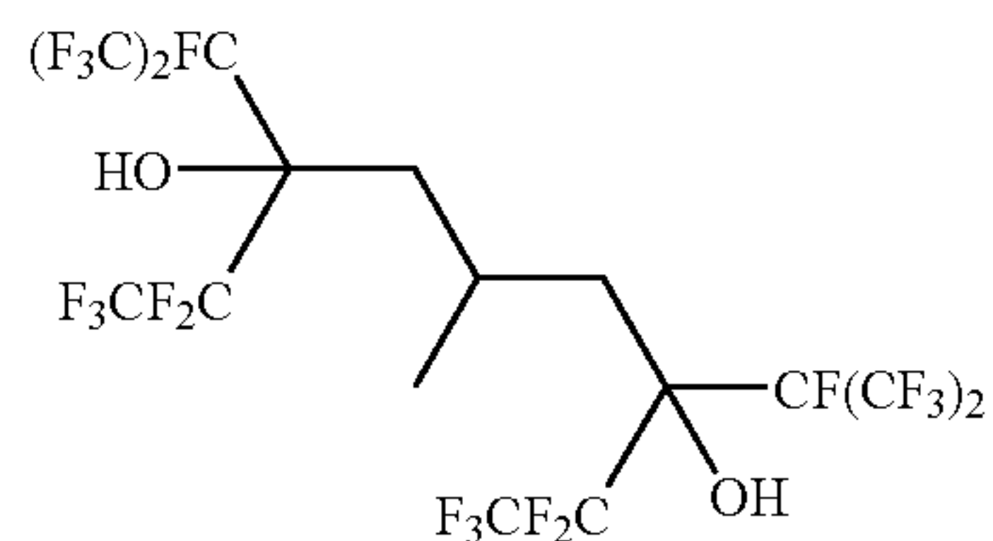
3,7-bis[1,2,2,2-tetrafluoro-1-(trifluoromethyl)ethyl]-1,1,1,2,2,8,8,9,9,9-decafluoro-5-methylnonane-3,7-diol
