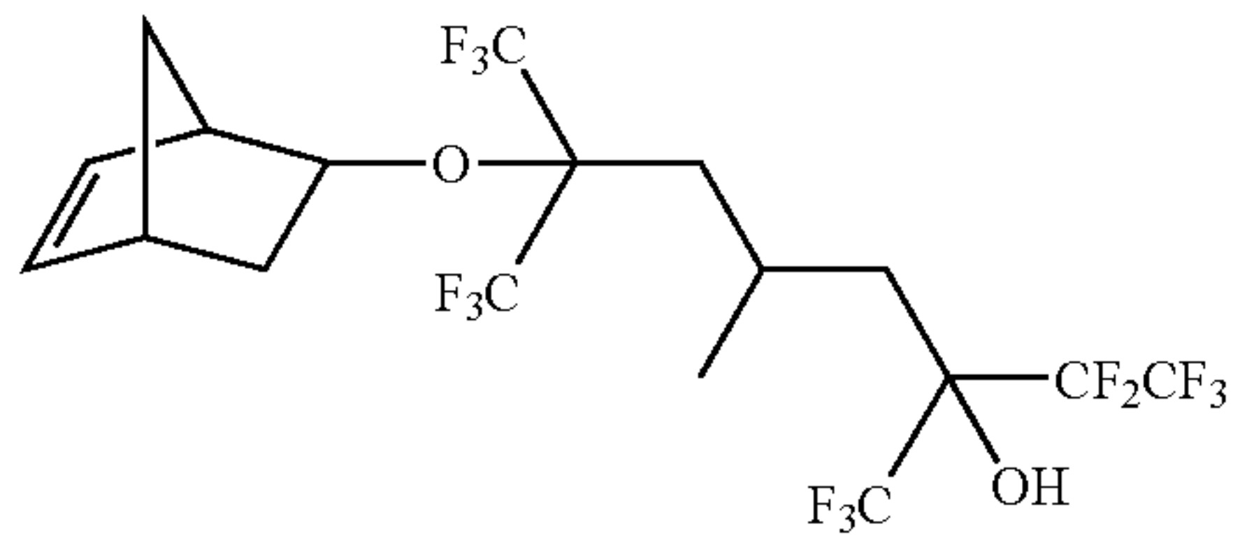
7-bicyclo[2.2.1]hept-5-en-2-yloxy-3,7-bis(trifluoromethyl)-1,1,1,2,2,8,8,8-octafluoro-5-methyloctan-3-ol
