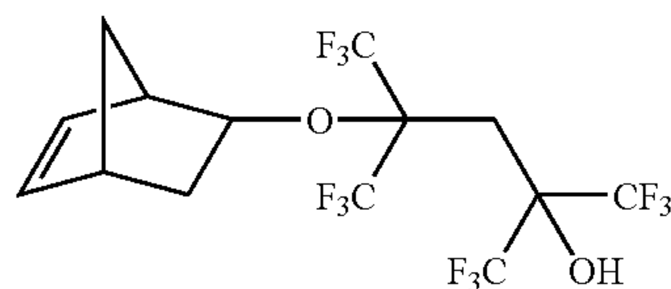
4-bicyclo[2.2.1]hept-5-en-2-yloxy-2,4-bis(trifluoromethyl)-1,1,1,5,5,5-hexafluoropentan-2-ol
