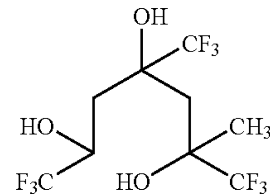
1,1,1,7,7,7-hexafluoro-2-methyl-4-(trifluoromethyl)heptane-2,4,6-triol
