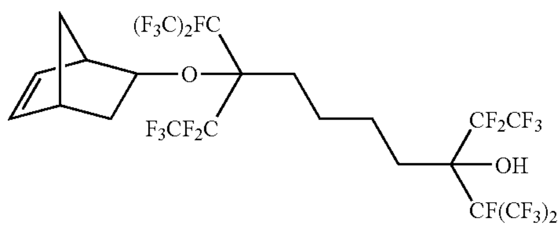
8-bicyclo[2.2.1]hept-5-en-2-yloxy-3,8-bis[1,2,2,2-tetrafluoro-1-(trifluoromethyl)ethyl]-1,1,1,2,2,9,9,10,10,10-decafluorodecan-3-ol
