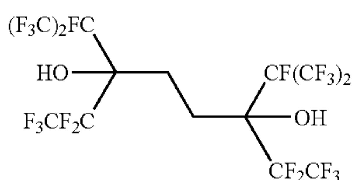
3,6-bis[1,2,2,2-tetrafluoro-1-(trifluoromethyl)ethyl]-1,1,1,2,2,7,7,8,8,8-decafluorooctane-3,6-diol
