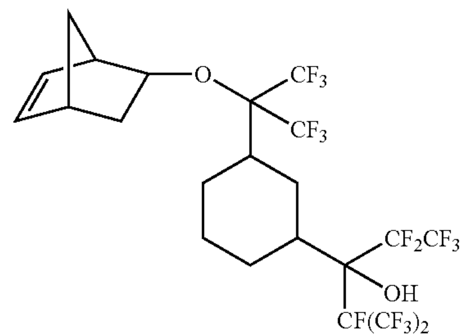
3-{3-[1-Bicyclo[2.2.1]hept-5-en-2-yloxy-2,2,2-trifluoro-1-trifluoromethyl-ethyl]cyclohexyl}-1,1,1,2,2,4,4,5,5,5-nonafluoro-4-trifluoromethyl-pentan-3-ol
