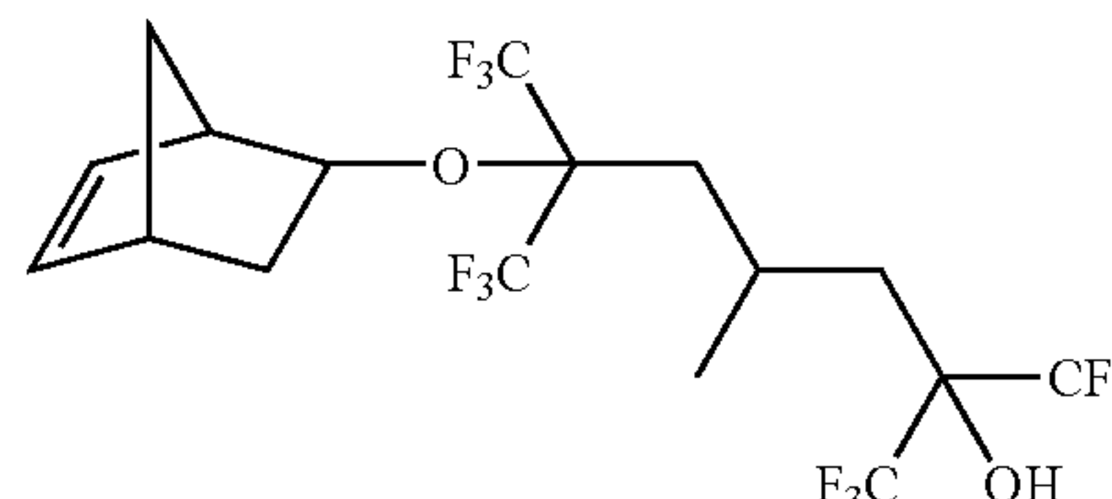
6-bicyclo[2.2.1]hept-5-en-2-yloxy-2,6-bis(trifluoromethyl)-1,1,1,7,7,7-hexafluoro-4-methylheptan-2-ol
