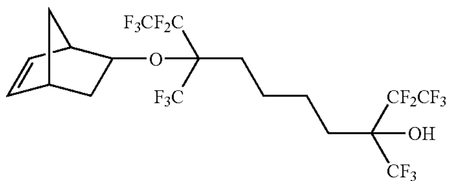
8-bicyclo[2.2.1]hept-5-en-2-yloxy-3,8-bis(trifluoromethyl)-1,1,1,2,2,9,9,10,10,10-decafluorodecan-3-ol
