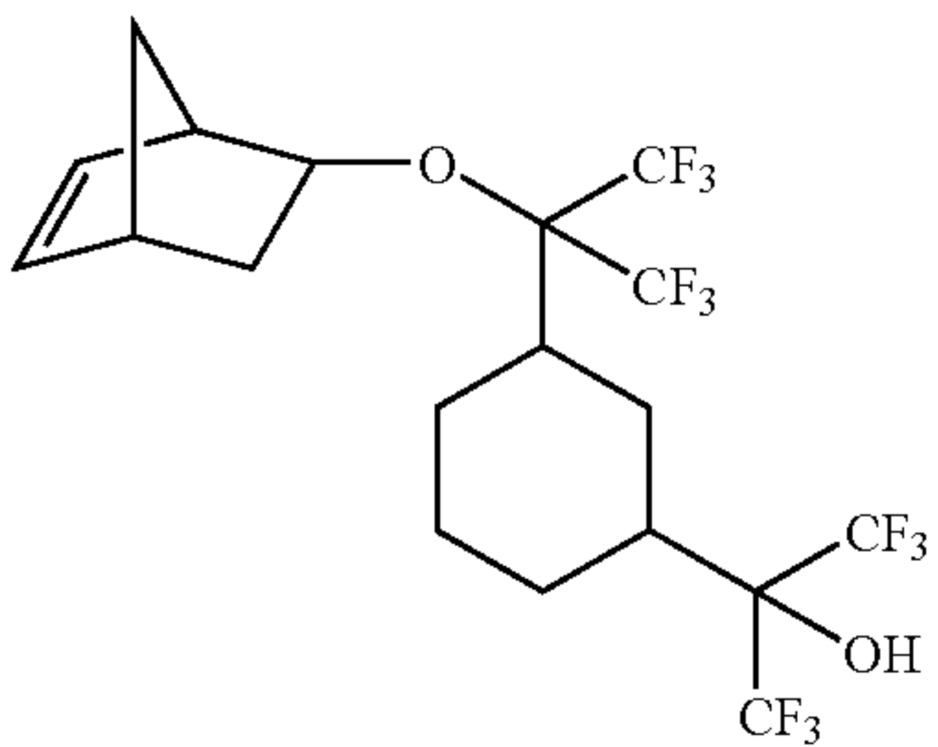
2-{3-[1-bicyclo[2.2.1]hept-5-en-2-yloxy-2,2,2-trifluoro-1-(trifluoromethyl)ethyl]cyclohexyl}-1,1,1,3,3,3-hexafluoropropan-2-ol
