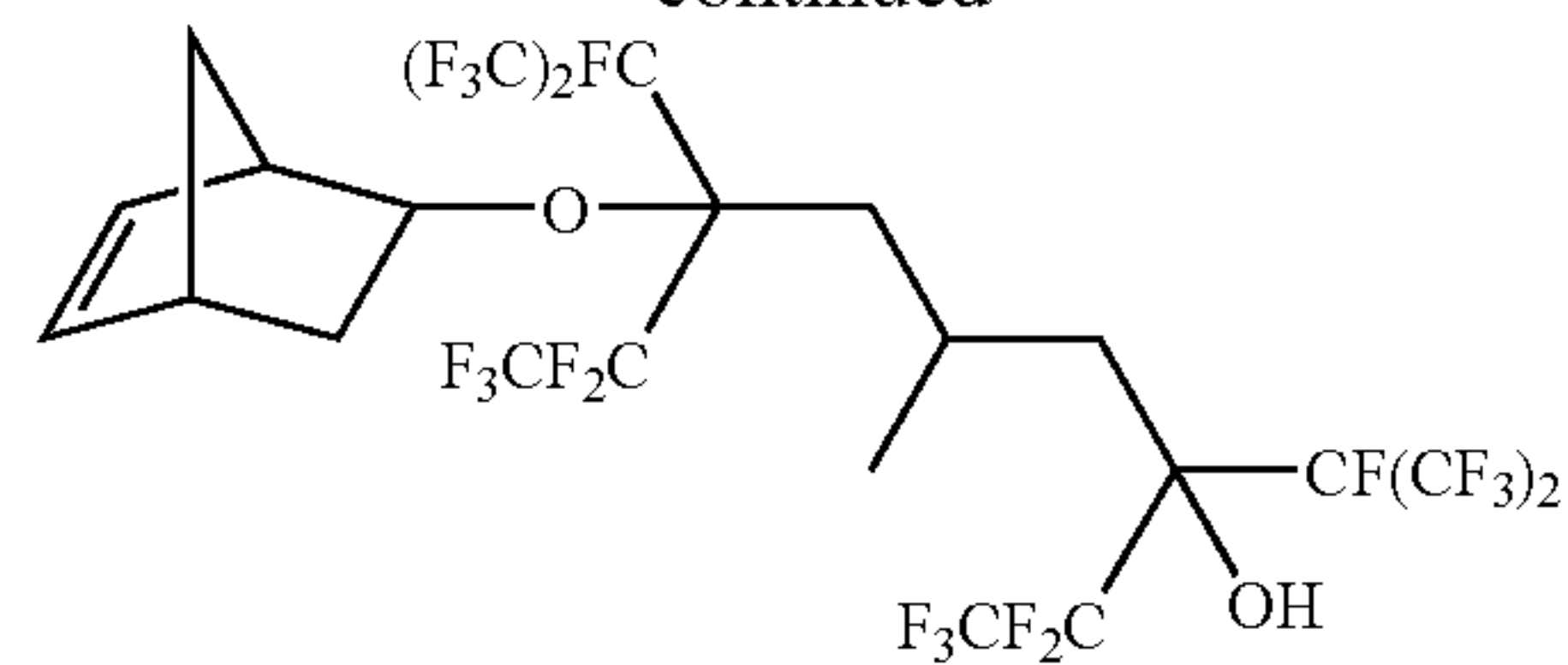
7-bicyclo[2.2.1]hept-5-en-2-yloxy-3,7-bis[1,2,2,2-tetrafluoro-1-(trifluoromethyl)ethyl]-1,1,1,2,2,8,8,9,9,9-decafluoro-5-methylnonan-3-ol
