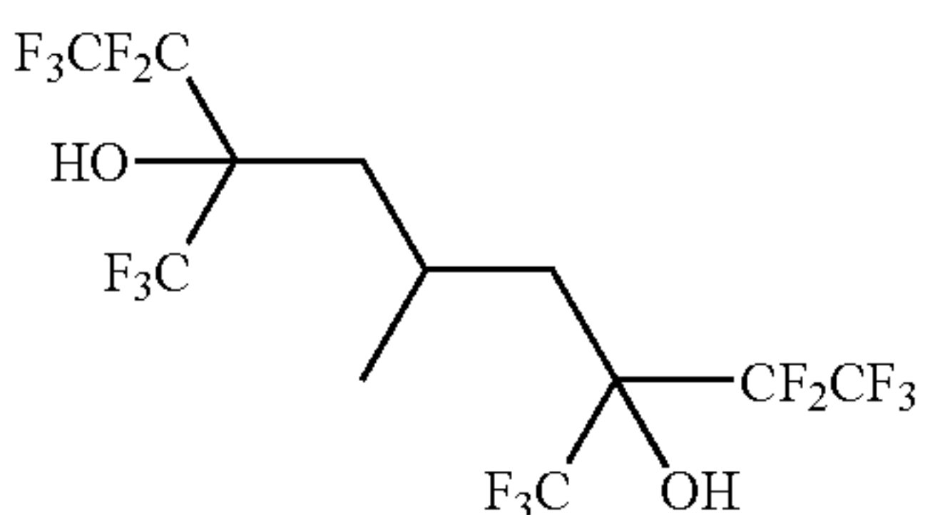
3,7-bis(trifluoromethyl)-1,1,1,2,2,8,8,9,9,9-decafluoro-5-methylnonane-3,7-diol
