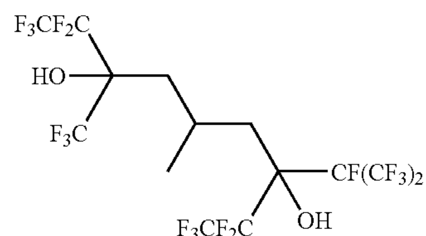
1,1,1,2,2,8,8,9,9-decafluoro-5-methyl-3-[1,2,2,2-tetrafluoro-1-(trifluoromethyl)ethyl]-7-(trifluoromethyl)nonane-3,7-diol
