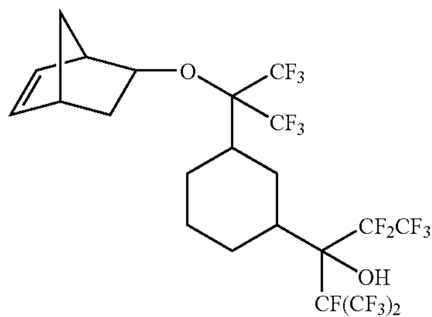
3-{3-[1-Bicyclo[2.2.1]hept-5-en-2-yloxy-2,2,2-trifluoro-1-trifluoromethyl-ethyl]-cyclohexyl}-1,1,1,2,2,4,5,5,5-nonafluoro-4-trifluoromethyl-pentan-3-ol
