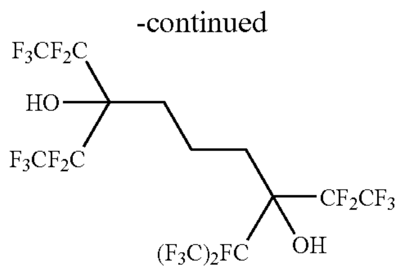
3,7-bis[1,2,2,2-tetrafluoro-1-(trifluoromethyl)ethyl]-1,1,1,2,2,8,8,9,9,9-decafluorononane-3,7-diol
