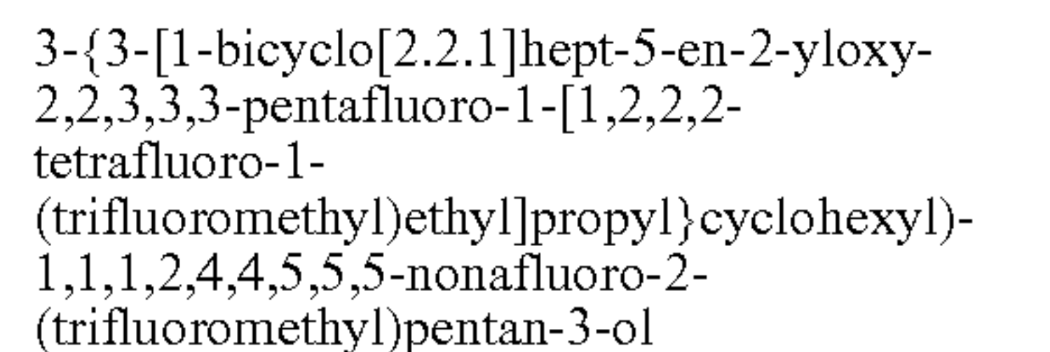
3-{3-[1-bicyclo[2.2.1]hept-5-en-2-yloxy-2,2,3,3,3-pentafluoro-1-[1,2,2,2-tetrafluoro-1-(trifluoromethyl)ethyl]propyl]cyclohexyl}-1,1,1,2,4,4,5,5,5-nonafluoro-2-(trifluoromethyl)pentan-3-ol
