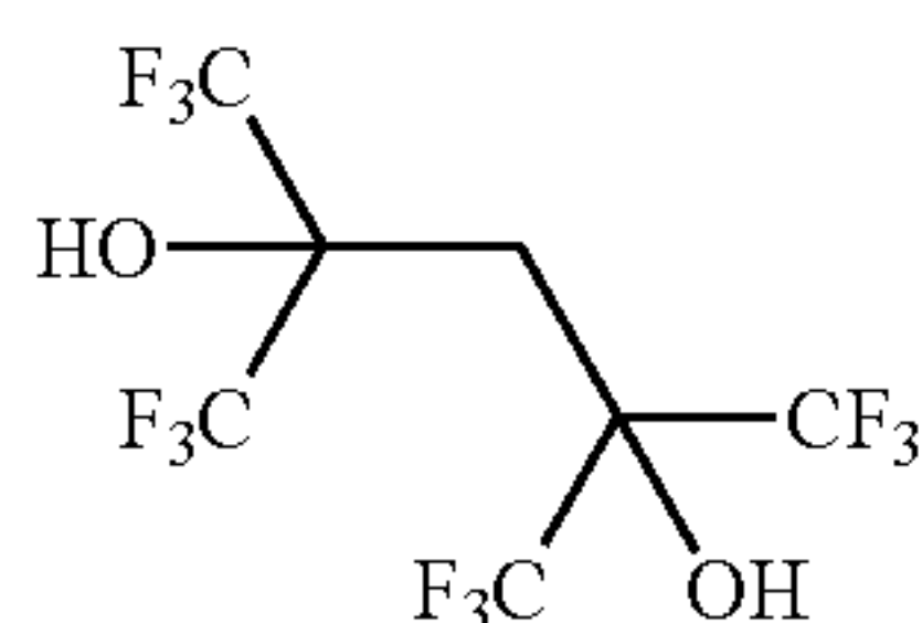
2,4-bis(trifluoromethyl)-1,1,1,5,5,5-hexafluoropentane-2,4-diol
