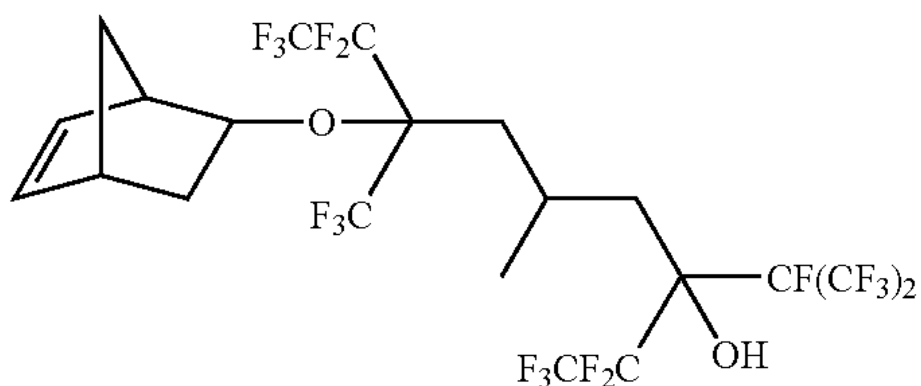
7-bicyclo[2.2.1]hept-5-en-2-yloxy-1,1,1,2,2,8,8,9,9,9-decafluoro-5-methyl-3-[1,2,2,2-tetrafluoro-1-(trifluoromethyl)ethyl]-7-(trifluoromethyl)nonan-3-ol
