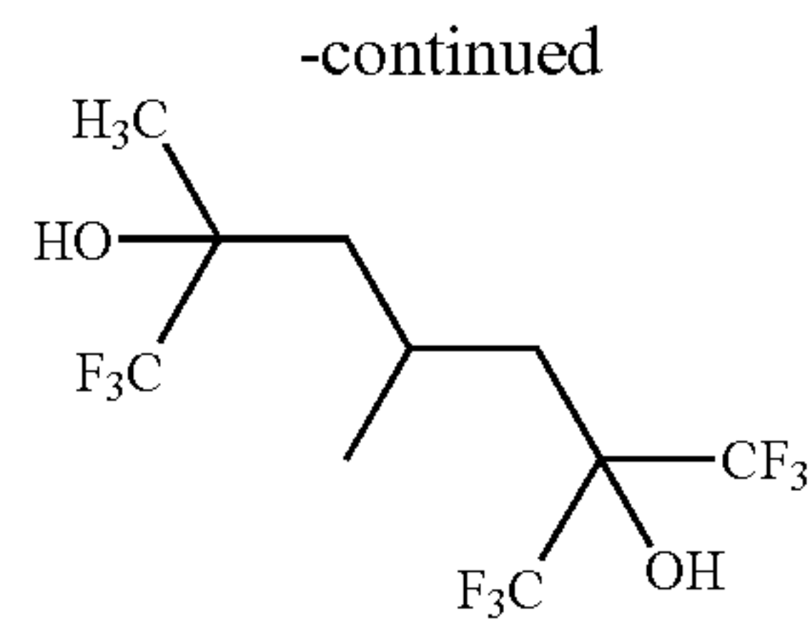
1,1,1,7,7,7-hexafluoro-2,4-dimethyl-6-(trifluoromethyl)heptane-2,6-diol
