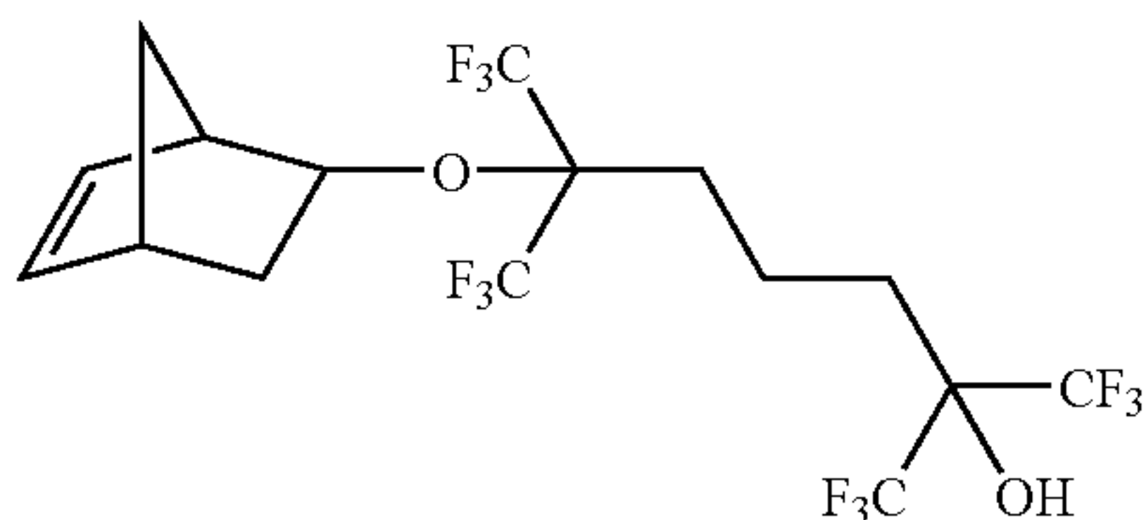
6-bicyclo[2.2.1]hept-5-en-2-yloxy-2,6-bis(trifluoromethyl)-1,1,1,7,7,7-hexafluoroheptan-2-ol
