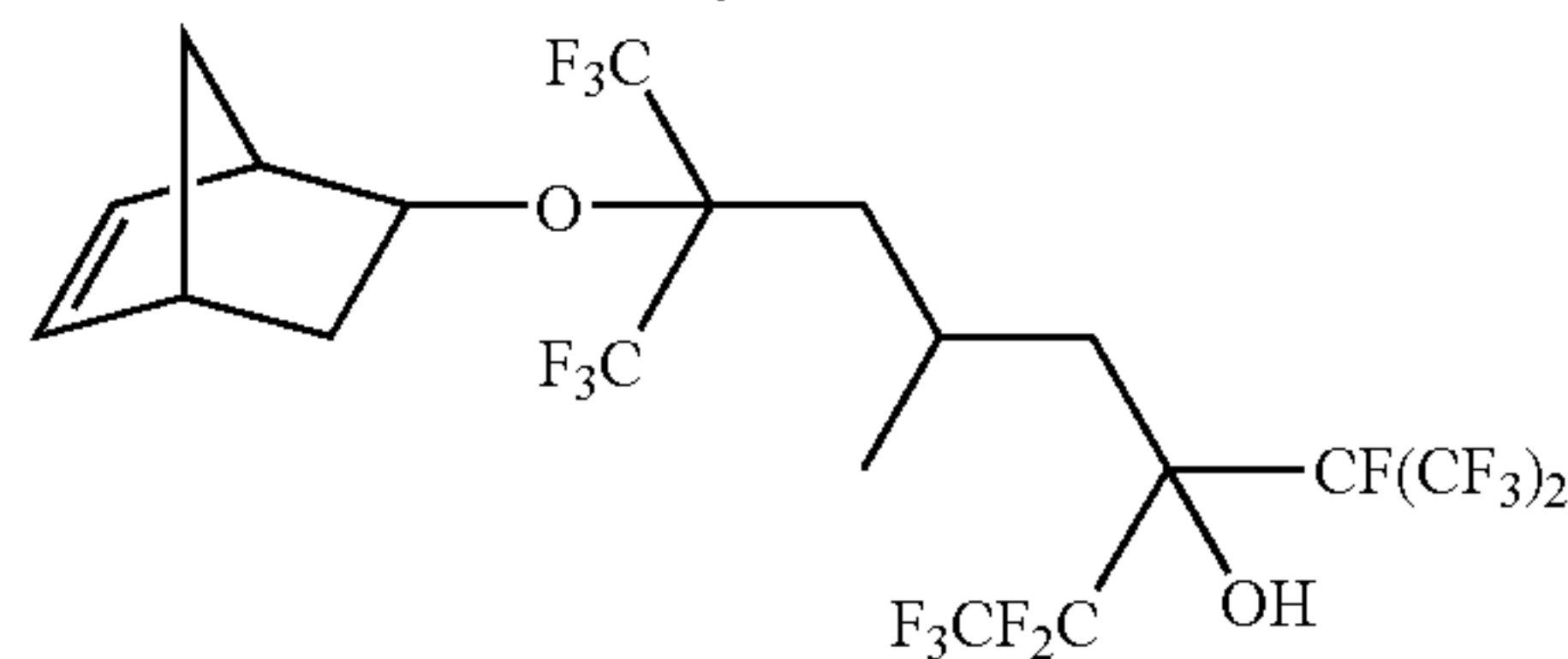
7-bicyclo[2.2.1]hept-5-en-2-yloxy-1,1,1,2,2,8,8,8-octafluoro-5-methyl-3-[1,2,2,2-tetrafluoro-1-(trifluoromethyl)ethyl]-7-(trifluoromethyl)octan-3-ol
