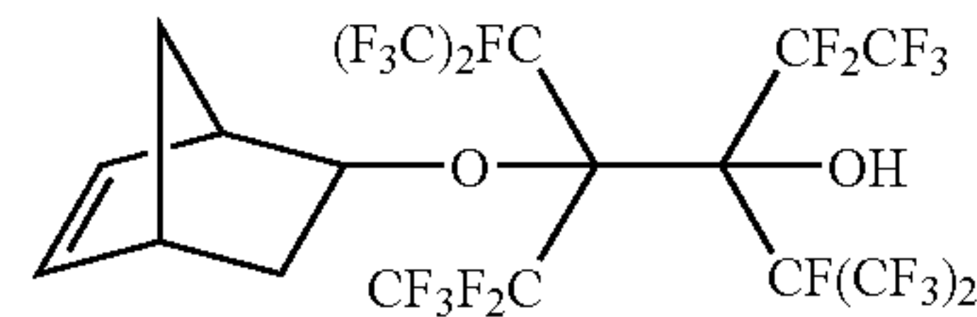
4-bicyclo[2.2.1]hept-5-en-2-yloxy-3,4-bis[1,2,2,2-tetrafluoro-1-(trifluoromethyl)ethyl]-1,1,1,2,2,5,5,6,6,6-decafluorohexan-3-ol
