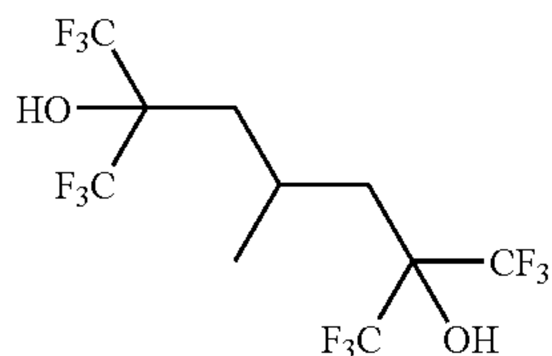
2,6-bis(trifluoromethyl)-1,1,1,7,7,7-hexafluoro-4-methylheptane-2,6-diol
