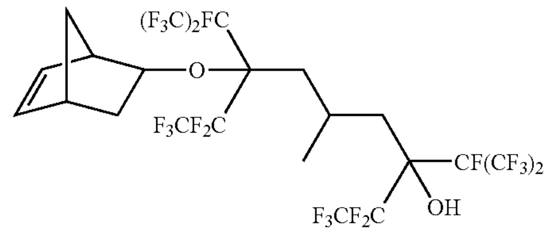
8-bicyclo[2.2.1]hept-5-en-2-yloxy-3,8-bis[1,2,2,2-tetrafluoro-1-(trifluoromethyl)ethyl]-1,1,1,2,2,9,9,10,10,10-decafluorodecan-3-ol
