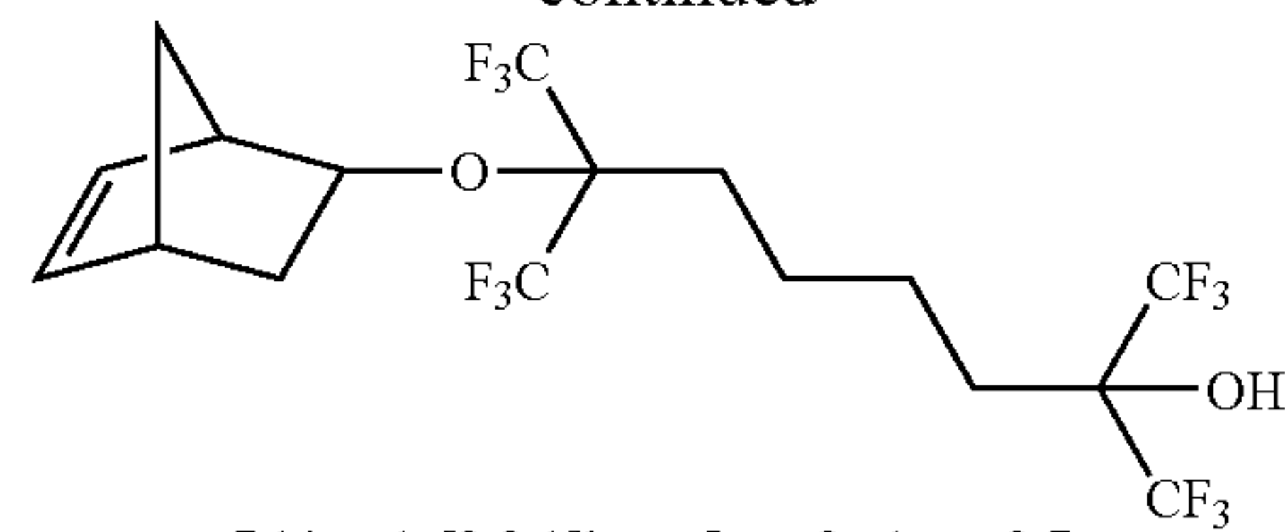
7-bicyclo[2.2.1]hept-5-en-2-yloxy-2,7-bis(trifluoromethyl)-1,1,1,8,8,8-hexafluorooctan-2-ol
