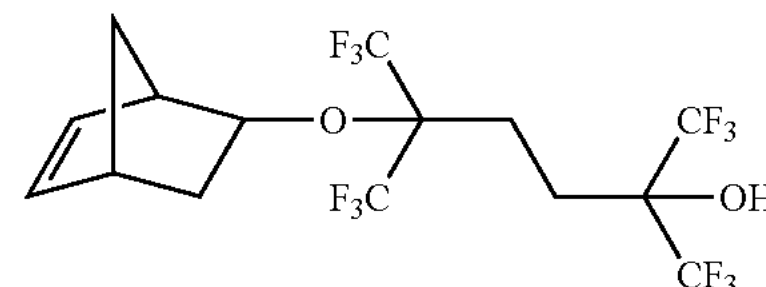
5-bicyclo[2.2.1]hept-5-en-2-yloxy-2,5-bis(trifluoromethyl)-1,1,1,6,6,6-hexafluorohexan-2-ol
