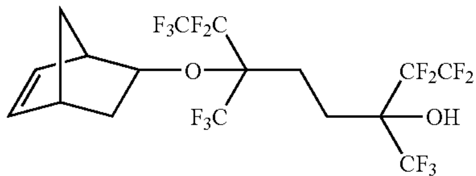
6-bicyclo[2.2.1]hept-5-en-2-yloxy-3,6-bis(trifluoromethyl)-1,1,1,2,2,7,7,8,8,8-nonafluorooctan-3-ol
