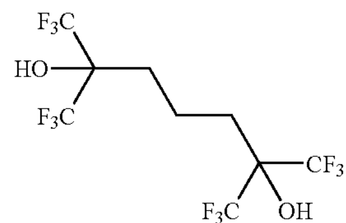
2,6-bis(trifluoromethyl)-1,1,1,7,7,7-hexafluoroheptane-2,6-diol
