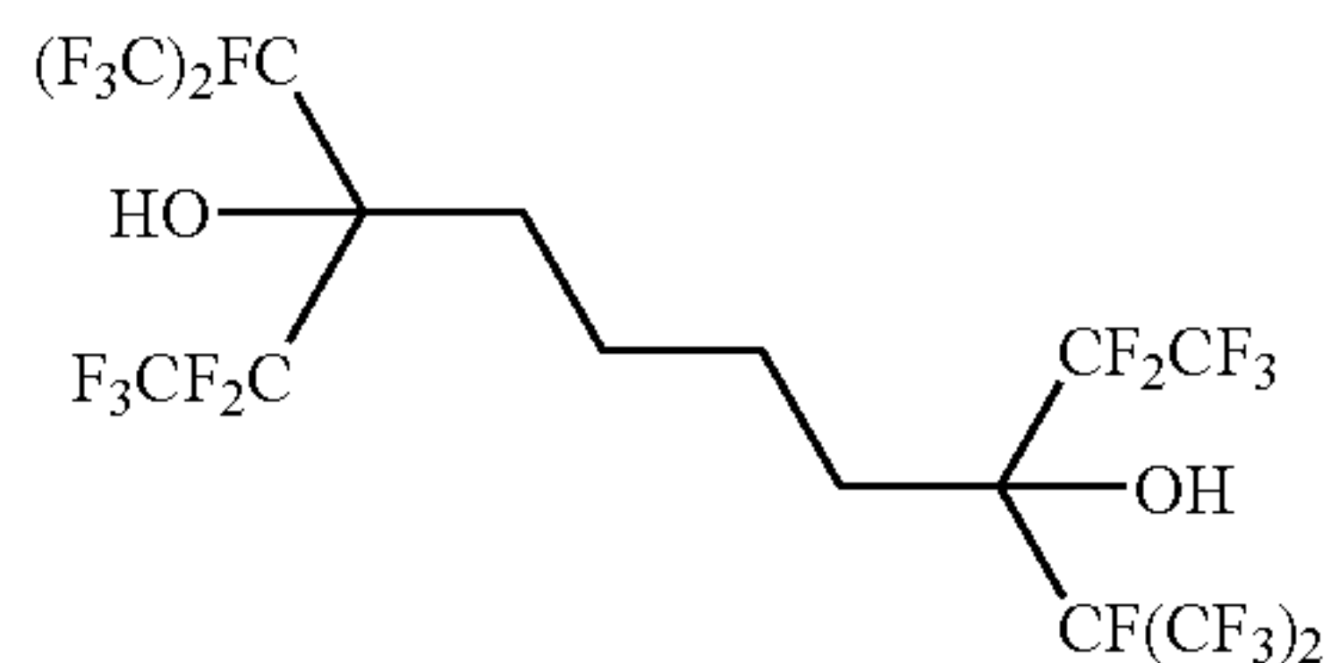
3,8-bis[1,2,2,2-tetrafluoro-1-(trifluoromethyl)ethyl]-1,1,1,2,2,9,9,10,10,10-decafluorodecane-3,8-diol
