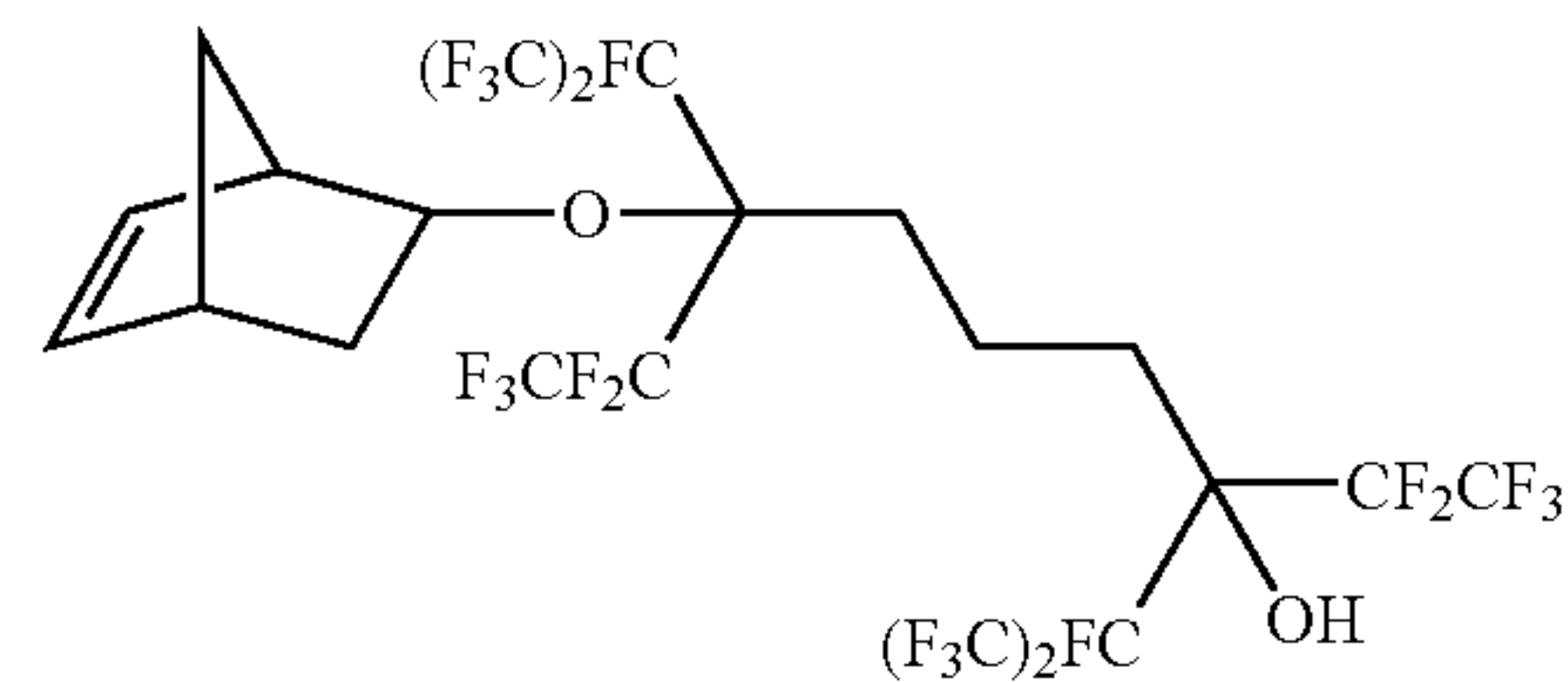
6-bicyclo[2.2.1]hept-5-en-2-yloxy-3,6-bis[1,2,2,2-tetrafluoro-1-(trifluoromethyl)ethyl]-1,1,1,2,2,7,7,8,8,8-decafluorooctan-3-ol
