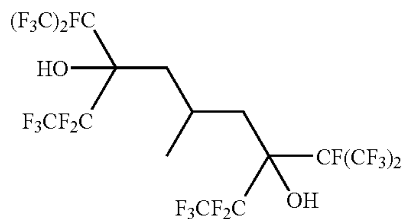
3,7-bis[1,2,2,2-tetrafluoro-1-(trifluoromethyl)ethyl]-1,1,1,2,2,8,8,9,9,9-decafluoro-5-methylnonane-3,7-diol
