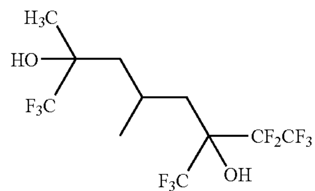
1,1,1,7,7,8,8,8-octafluoro-2,4-dimethyl-6-(trifluoromethyl)octane-2,6-diol
