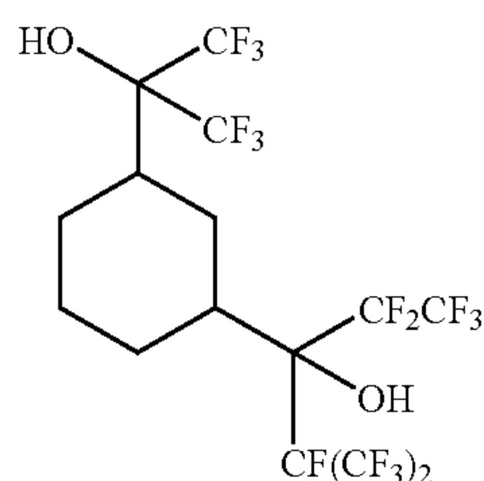
1,1,1,2,2,4,5,5,5-nonafluoro-3-(3-[2,2,2-trifluoro-1-hydroxy-1-(trifluoromethyl)ethyl]cyclohexyl)-4-(trifluoromethyl)pentan-3-ol
