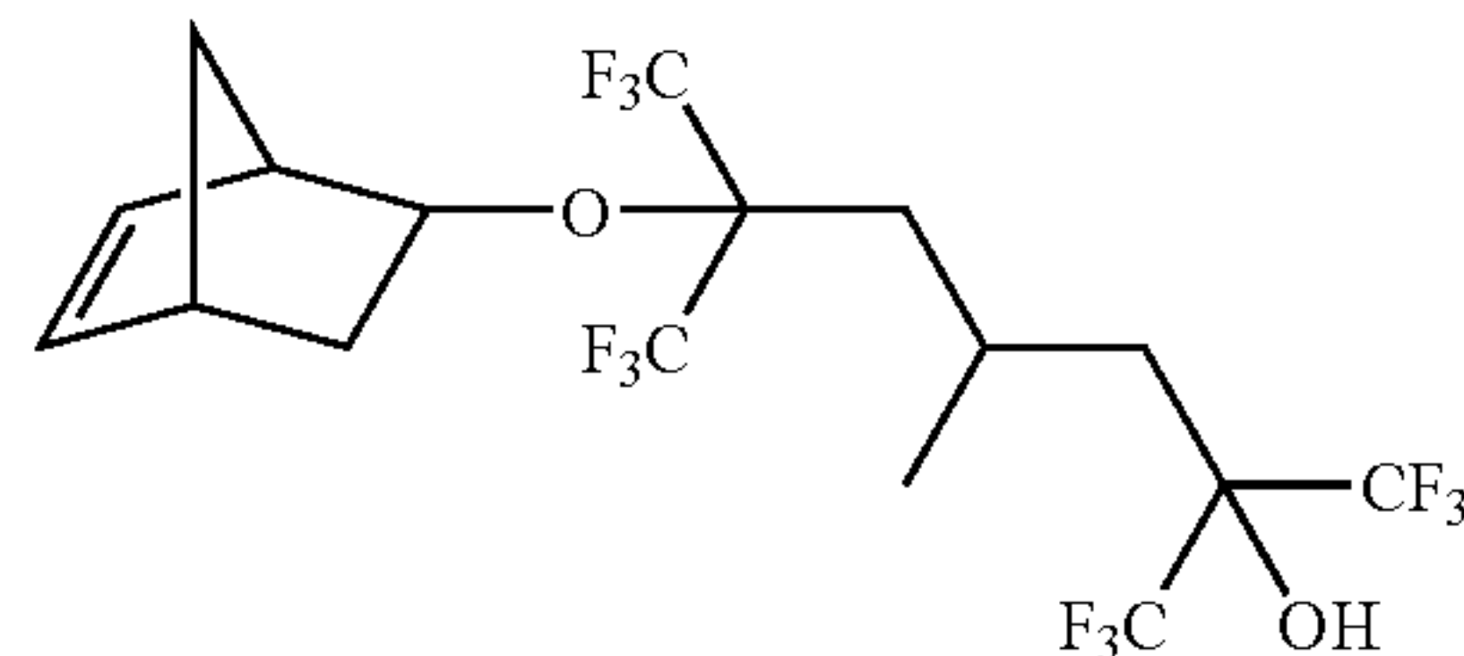
6-bicyclo[2.2.1]hept-5-en-2-yloxy-2,6-bis(trifluoromethyl)-1,1,1,7,7,7-hexafluoro-4-methylheptan-2-ol
