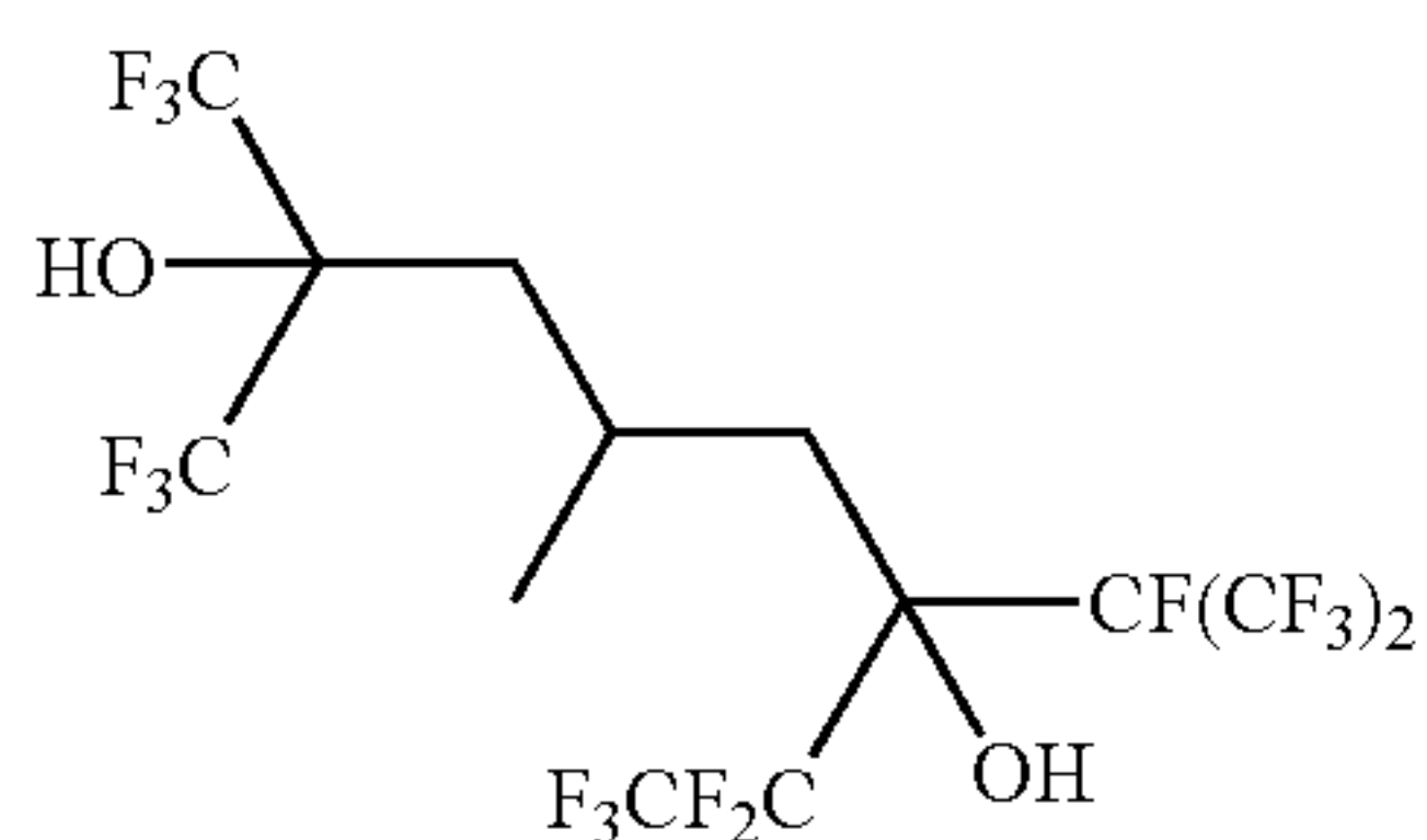
1,1,1,7,7,8,8,8-octafluoro-4-methyl-6-[1,2,2,2-tetrafluoro-1-(trifluoromethyl)ethyl]-2-(trifluoromethyl)octane-2,6-diol
