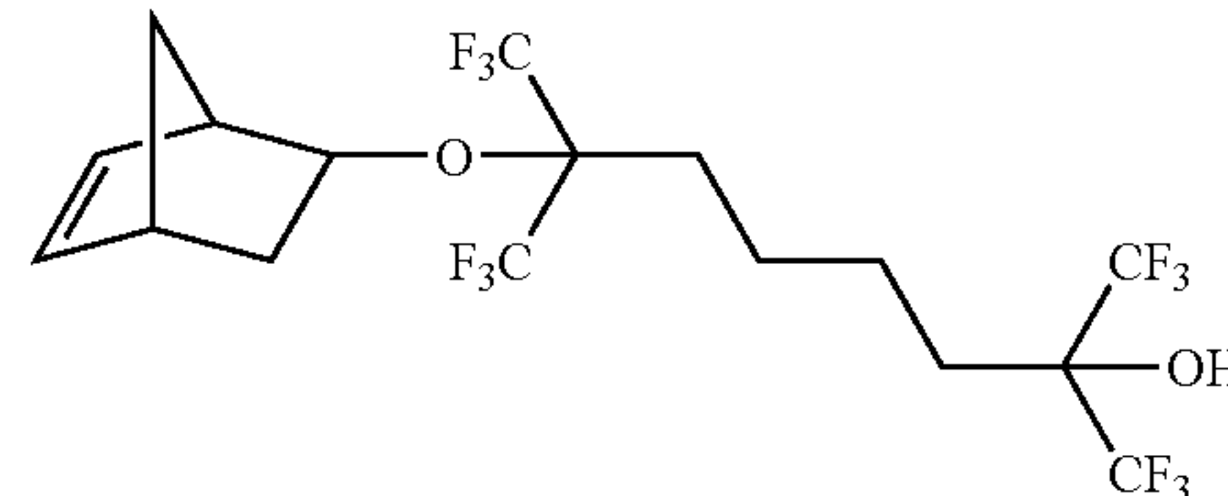
7-bicyclo[2.2.1]hept-5-en-2-yloxy-2,7-bis(trifluoromethyl)-1,1,1,8,8,8-hexafluoro-octan-2-ol
