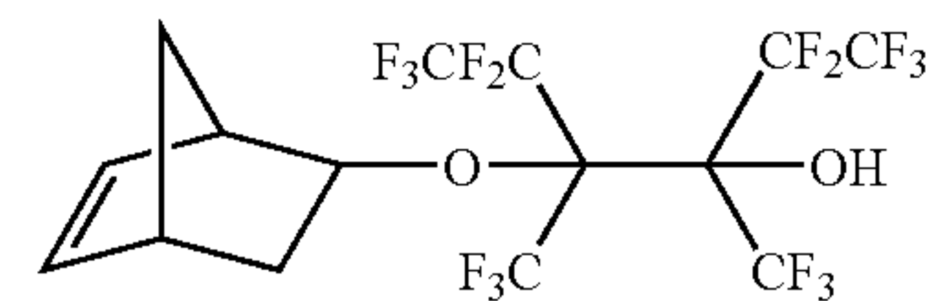
4-bicyclo[2.2.1]hept-5-en-2-yloxy-3,4-bis(trifluoromethyl)-1,1,1,2,2,5,5,6,6,6-decafluorohexan-3-ol
