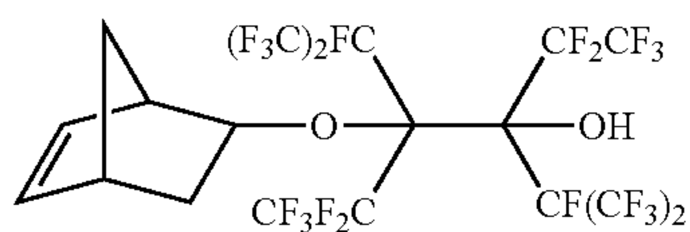
4-bicyclo[2.2.1]hept-5-en-2-yloxy-3,4-bis[1,2,2,2-tetrafluoro-1-(trifluoromethyl)ethyl]-1,1,1,2,2,5,5,6,6,6-decafluorohexan-3-ol
