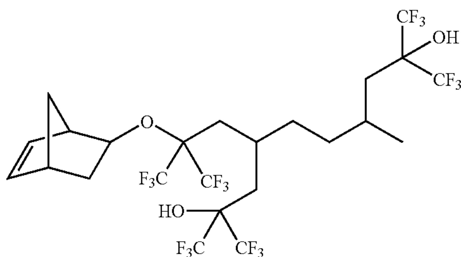
4-[bicyclo[2.2.1]hept-5-en-2-yloxy-3,3,3-trifluoro-2-trifluoromethylpropyl]-2,9-bis(trifluoromethyl)-1,1,1,10,10,10-hexafluoro-7-methyldecane-2,9-diol
