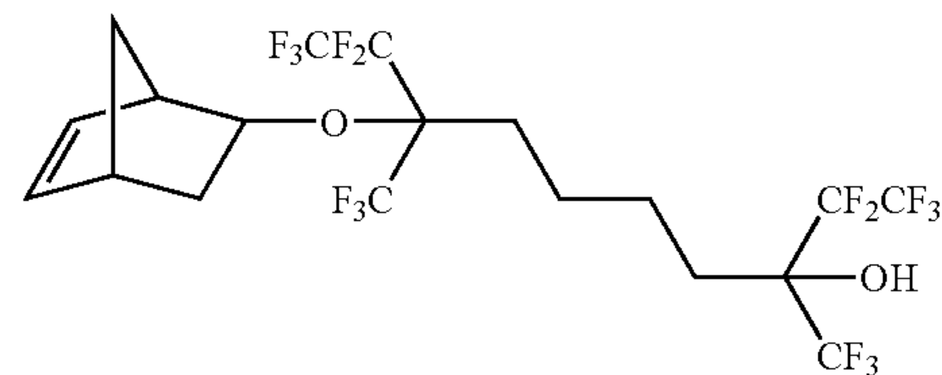
8-bicyclo[2.2.1]hept-5-en-2-yloxy-3,8-bis(trifluoromethyl)-1,1,1,2,2,9,9,10,10,10-decafluorodecan-3-ol
