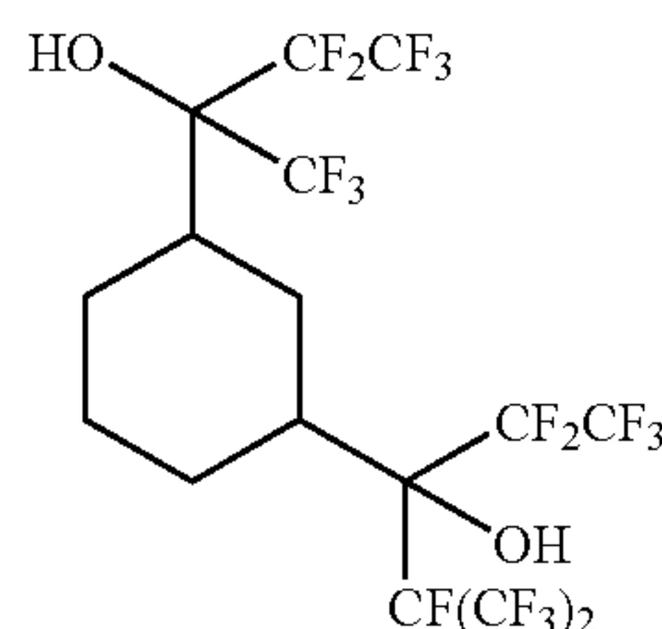
1,1,1,2,2,4,5,5,5-nonafluoro-3-(3-[2,2,3,3-pentafluoro-1-hydroxy-1-(trifluoromethyl)propyl]cyclohexyl)-4-(trifluoromethyl)pentan-3-ol
