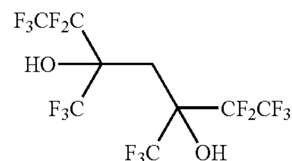
3,5-bis(trifluoromethyl)-1,1,1,2,2,6,6,7,7,7-decafluoroheptane-3,5-diol
