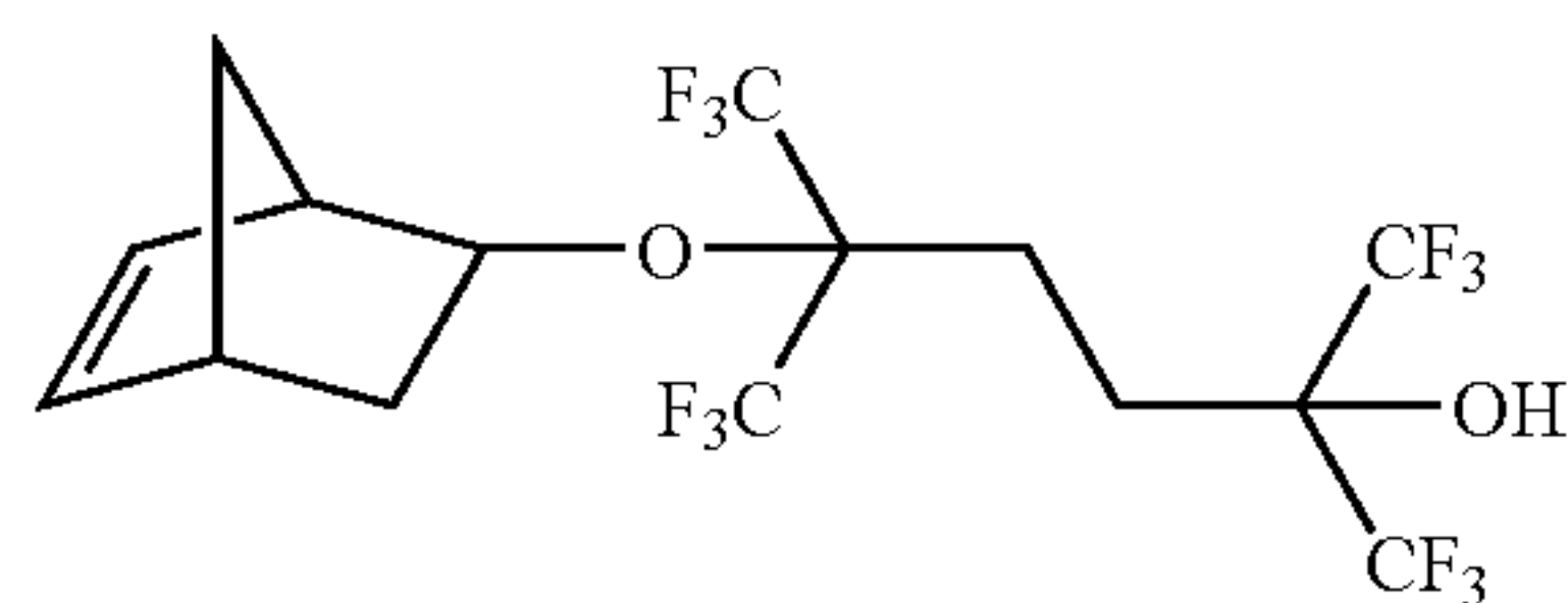
5-bicyclo[2.2.1]hept-5-en-2-yloxy-2,5-bis(trifluoromethyl)-1,1,1,6,6,6-hexafluorohexan-2-ol
