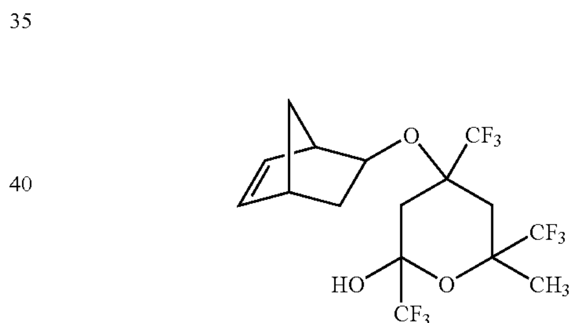
4-bicyclo[2.2.1]hept-5-en-2-yloxy-6-methyl-2,4,6-tris(trifluoromethyl)-2H-3,4,5,6-tetrahydropyran-2-ol
