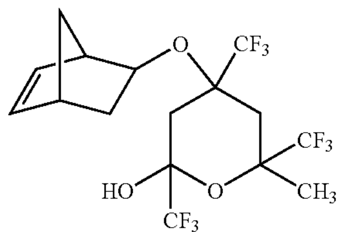
4-bicyclo[2.2.1]hept-5-en-2-yloxy-6-methyl-2,4,6-tris(trifluoromethyl)-2H-3,4,5,6-tetrahydropyran-2-ol.
