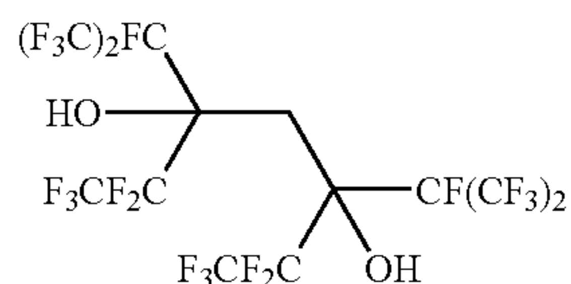
3,5-bis[1,2,2,2-tetrafluoro-1-(trifluoromethyl)ethyl]-1,1,1,2,2,6,6,7,7,7-decafluoroheptane-3,5-diol
