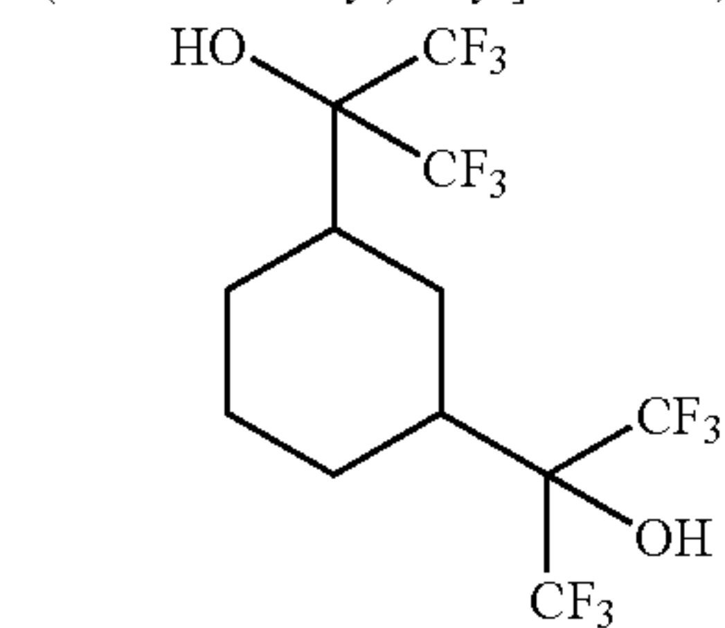
1,1,1,3,3,3-hexafluoro-2-(3-[2,2,2-trifluoro-1-hydroxy-1-(trifluoromethyl)ethyl]cyclohexyl)propan-2-ol
