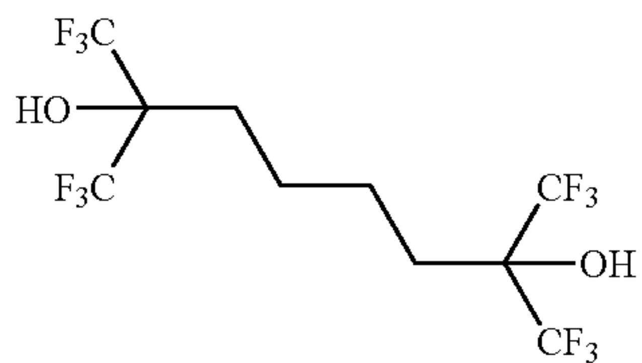
2,7-bis(trifluoromethyl)-1,1,1,8,8,8-hexafluorooctane-2,7-diol
