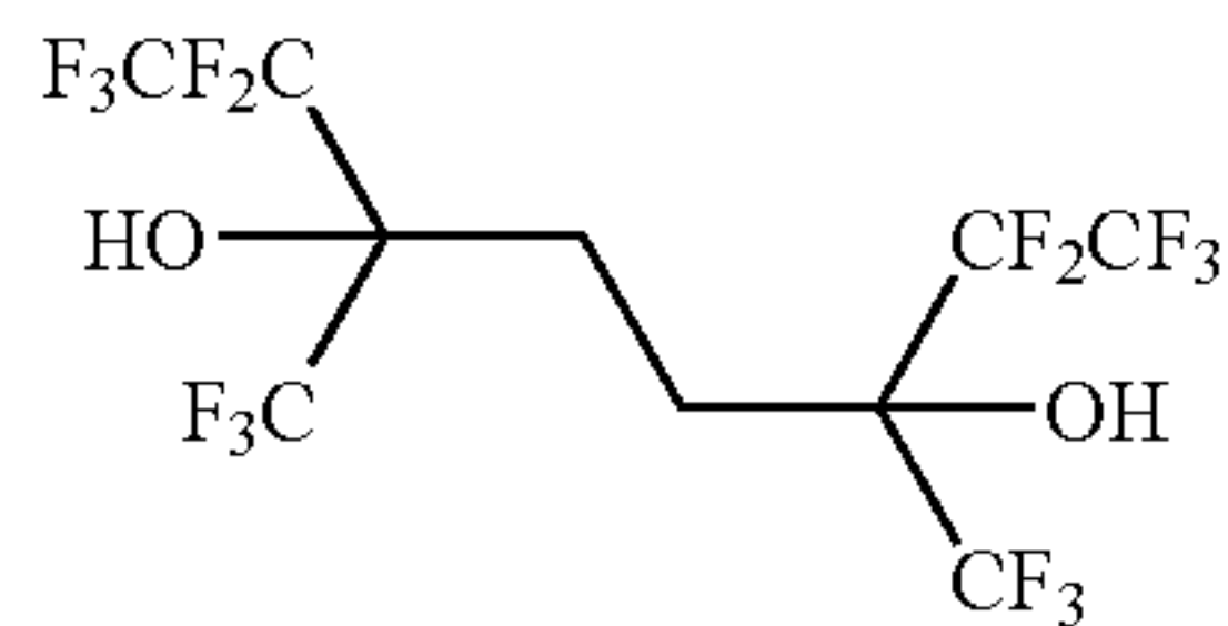
3,6-bis(trifluoromethyl)-1,1,1,2,2,7,7,8,8,8-nonafluorooctane-3,6-diol
