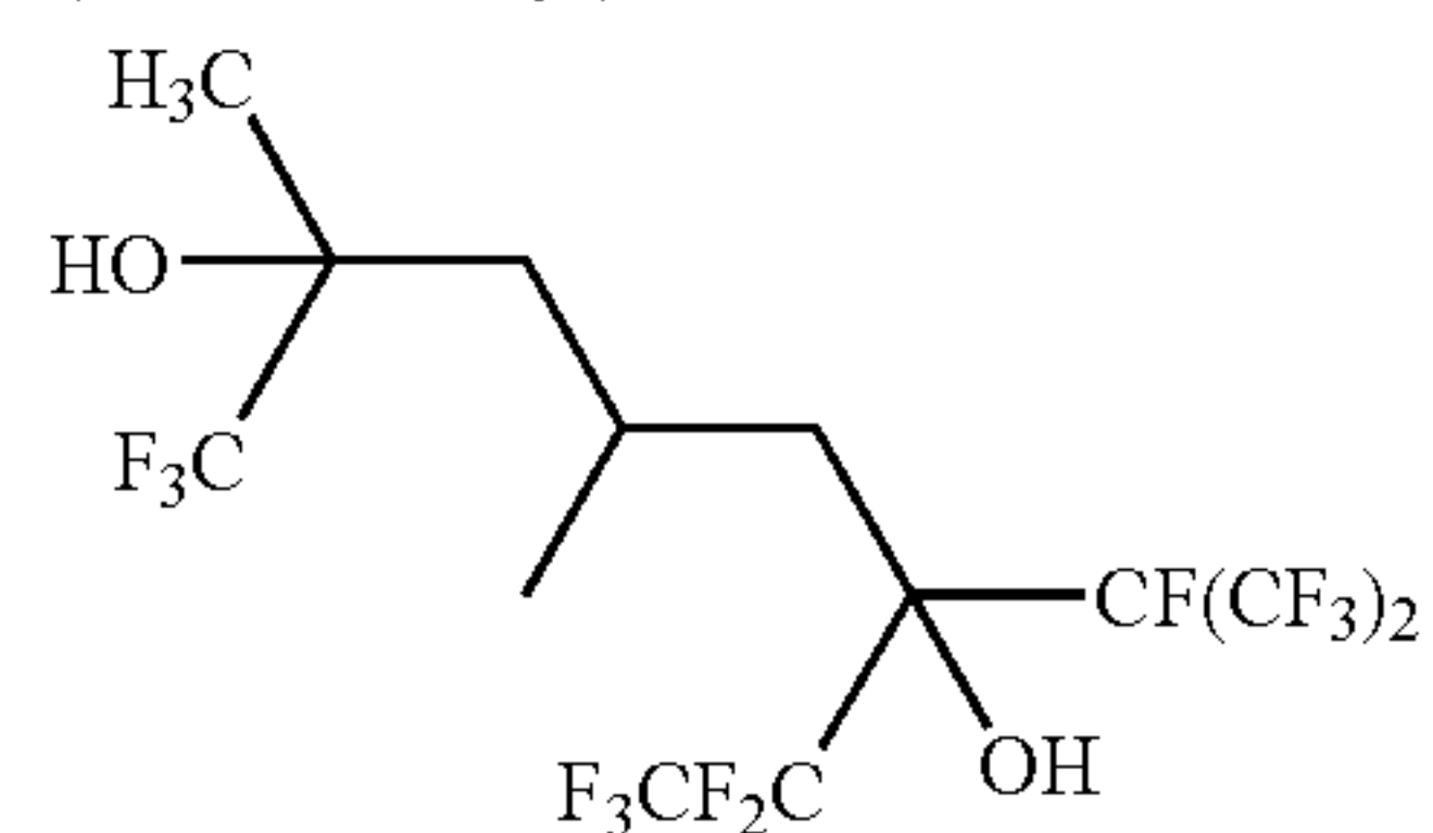
1,1,1,7,7,8,8,8-octafluoro-2,4-dimethyl-6-[1,2,2,2-tetrafluoro-1-(trifluoromethyl)ethyl]octane-2,6-diol
