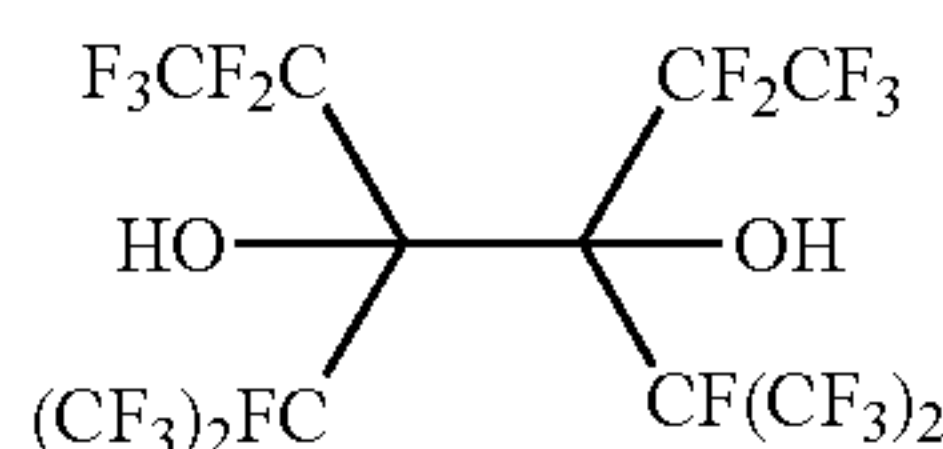
3,4-bis[1,2,2,2-tetrafluoro-1-(trifluoromethyl)ethyl]-1,1,1,2,2,5,5,6,6,6-decafluorohexane-3,4-diol
