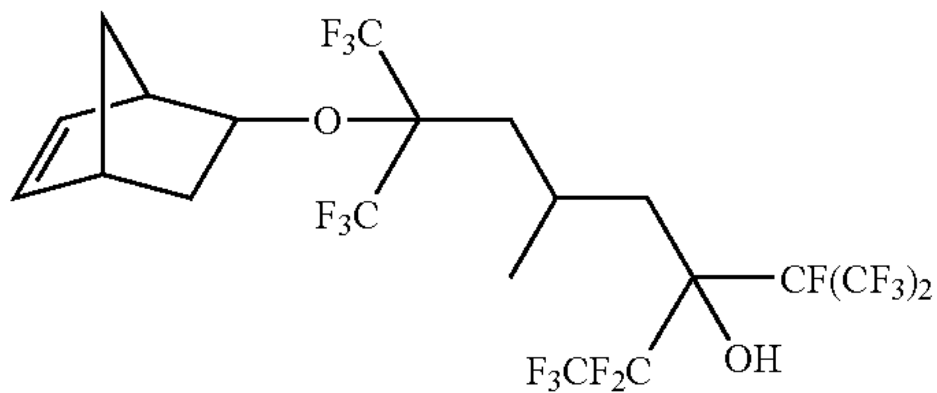
7-bicyclo[2.2.1]hept-5-en-2-yloxy-1,1,1,2,2,8,8,8-octafluoro-5-methyl-3-[1,2,2,2-tetrafluoro-1-(trifluoromethyl)ethyl]-7-(trifluoromethyl)octan-3-ol
