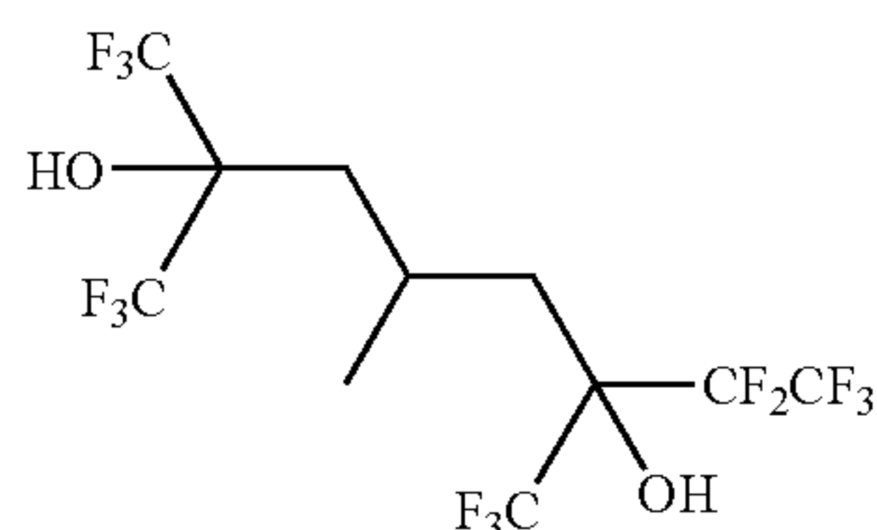
2,6-bis(trifluoromethyl)-1,1,1,7,7,8,8,8-octafluoro-4-methyloctane-2,6-diol
