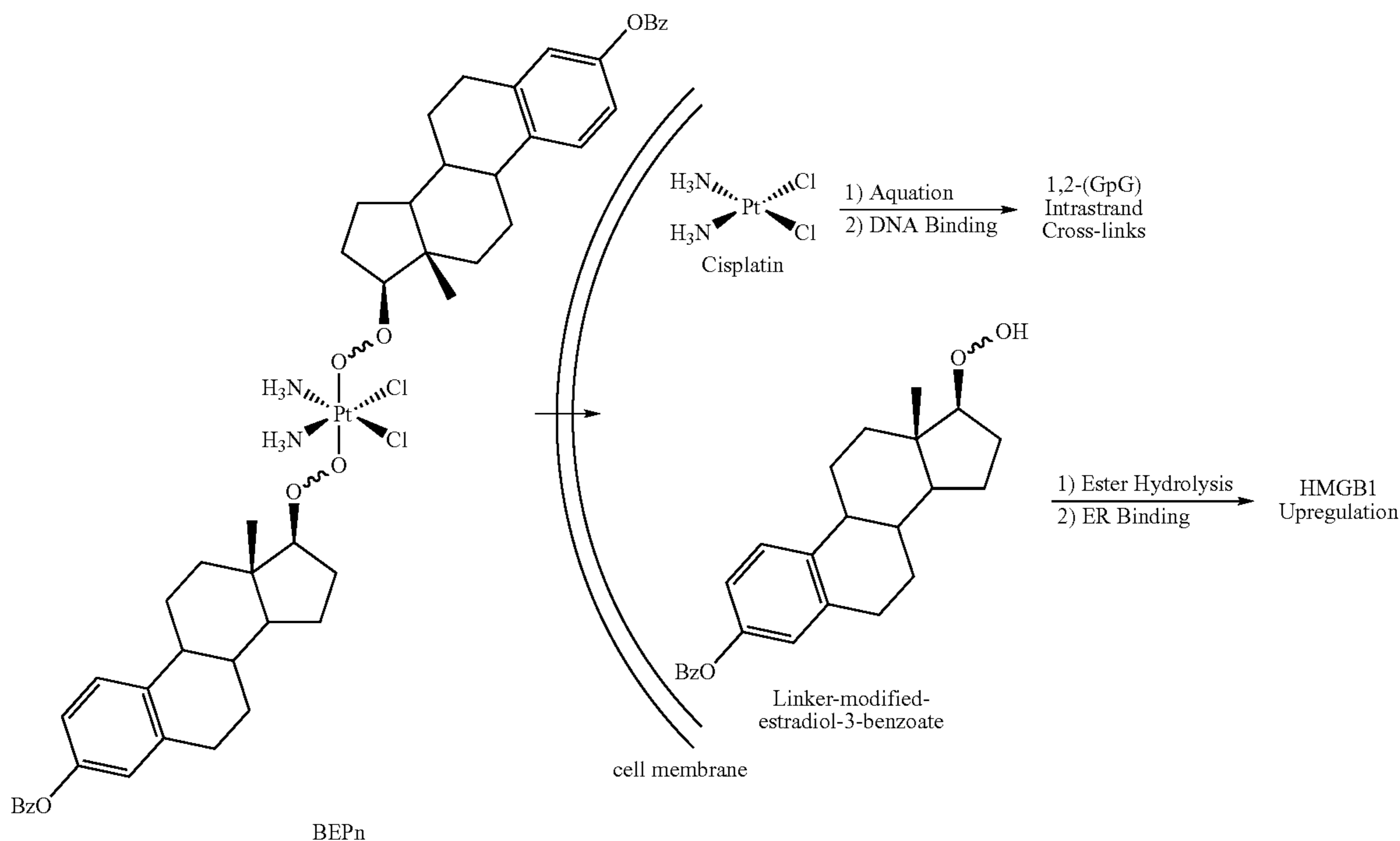
Scheme 1. Reduction of proposed platinum (IV) complexes to platinum (II) upon entering the reducing environment of the cell.
