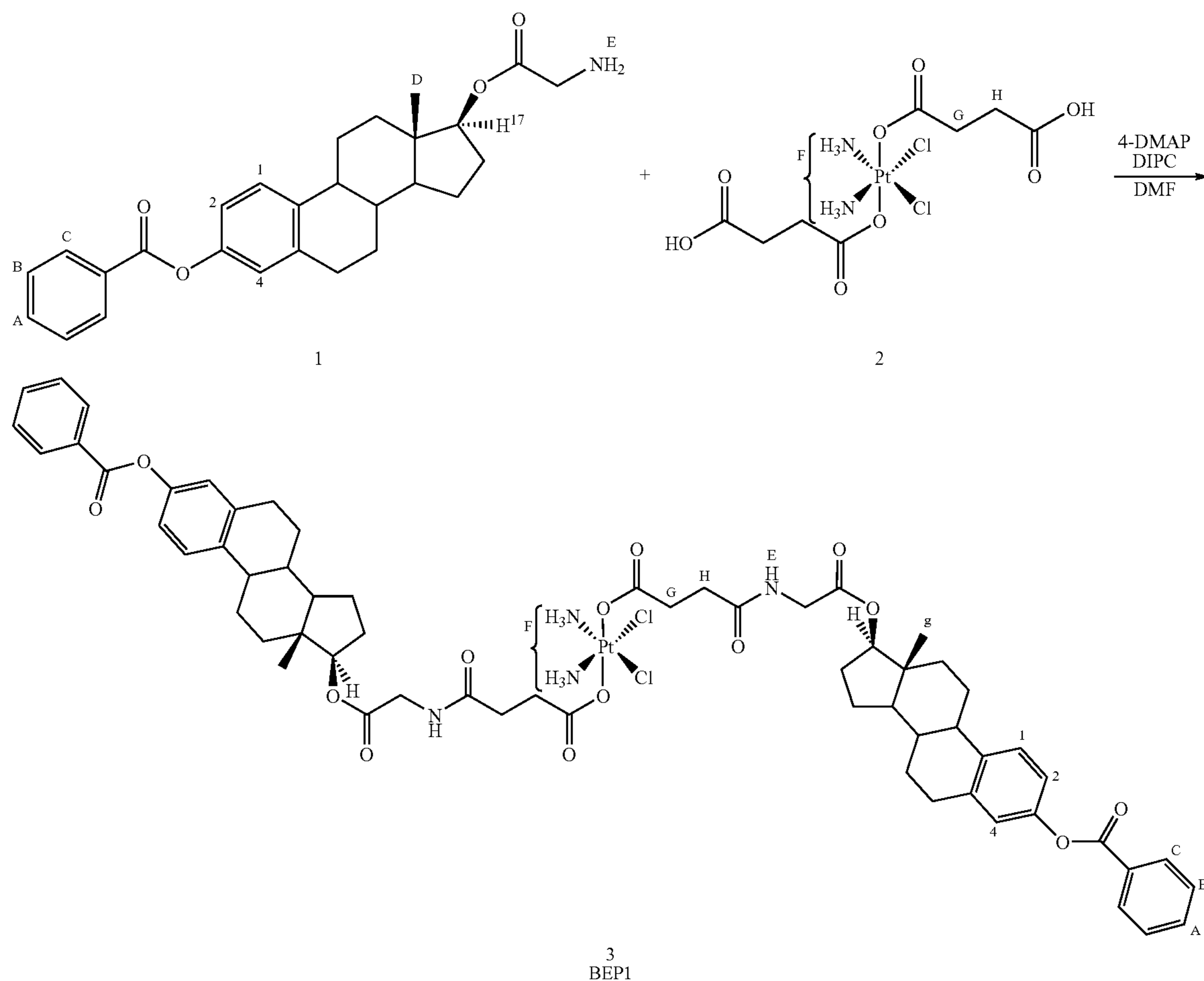
Scheme 4. Synthesis and ^1\text{H} NMR proton designations for BEP1.
