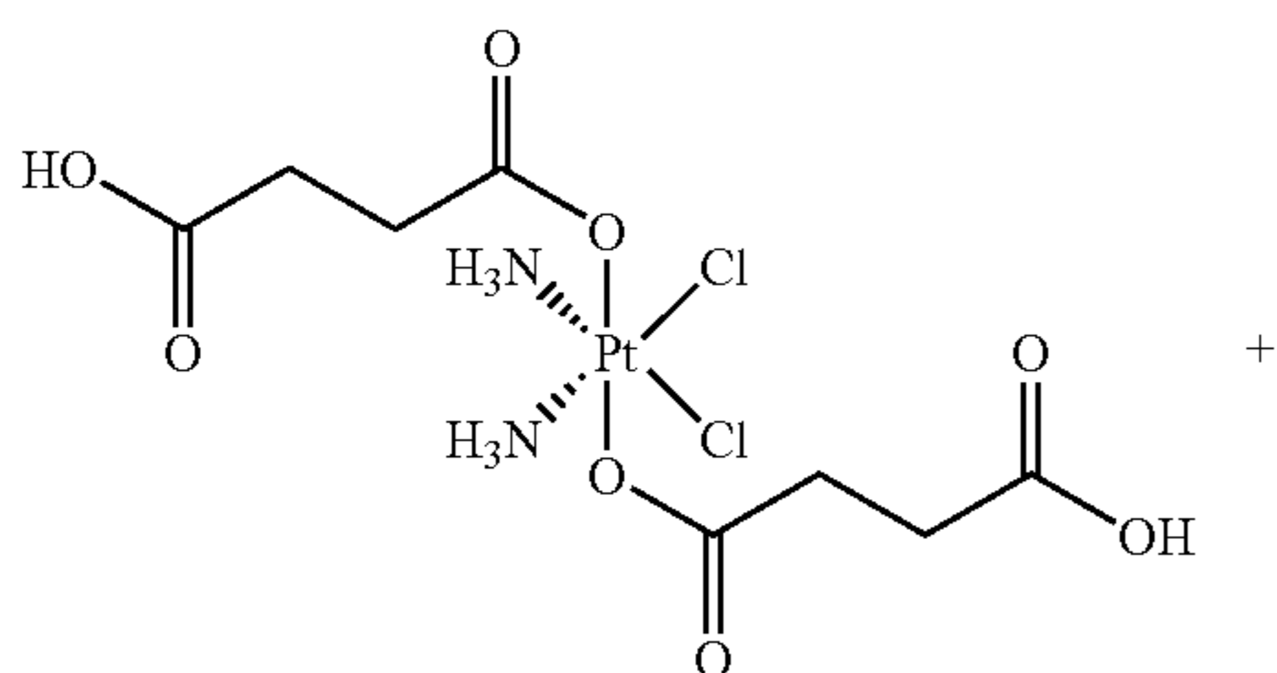
Scheme 5. Synthesis of peptide containing cisplatin complex.
