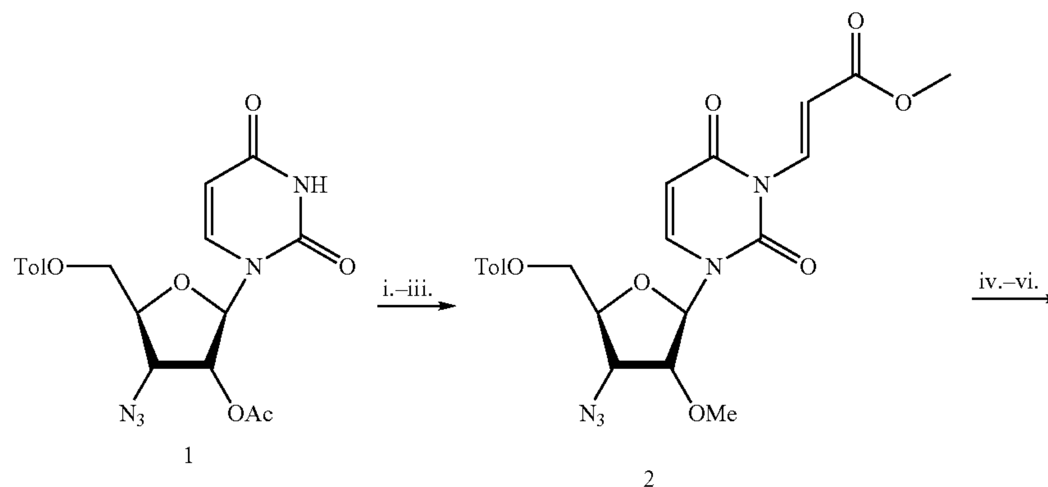
Scheme 1
