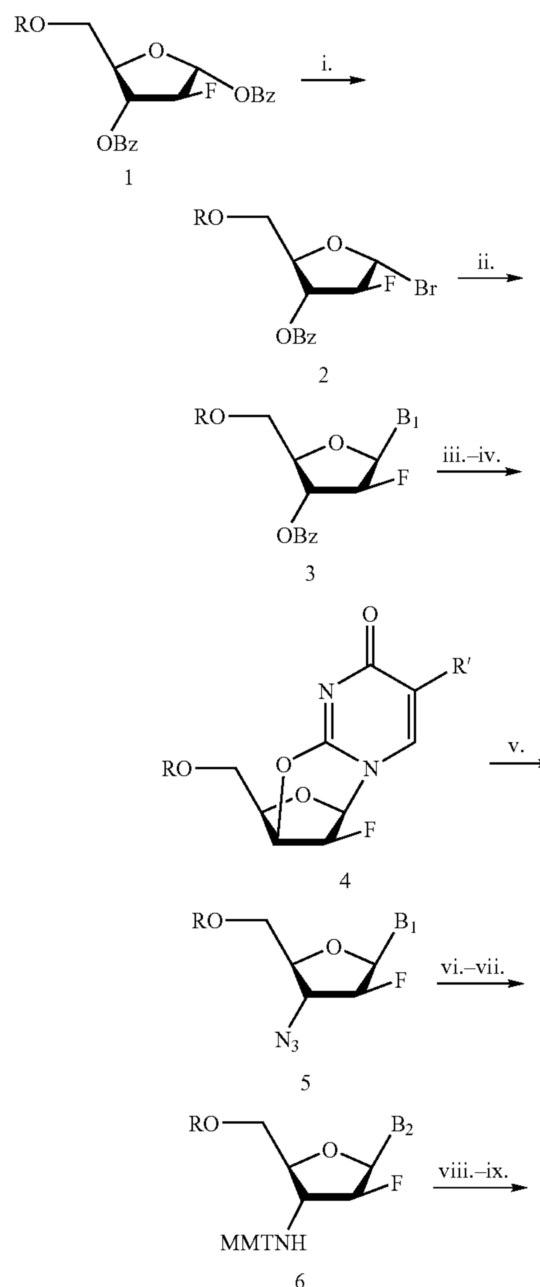
Scheme 4
