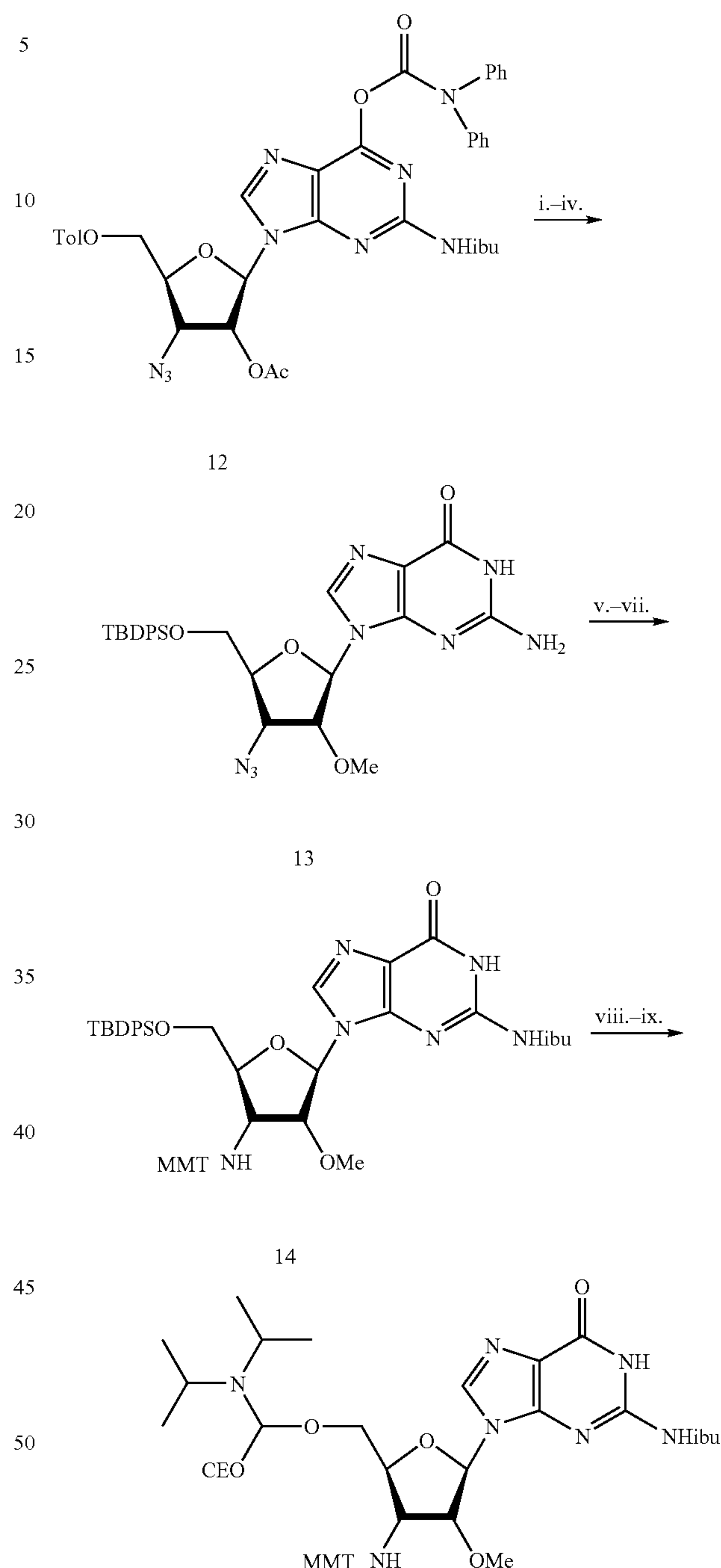
Scheme 3
