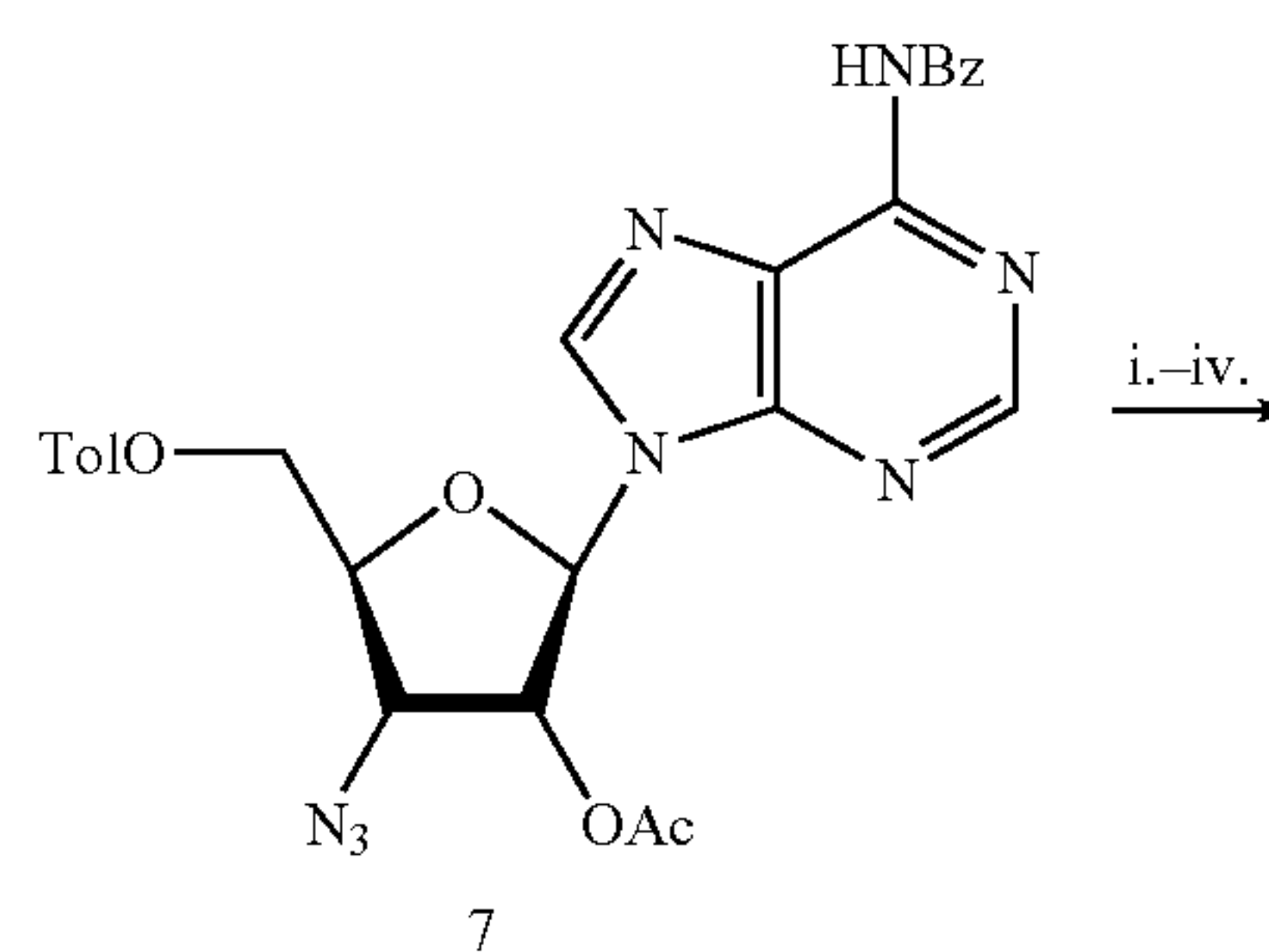
Scheme 2
