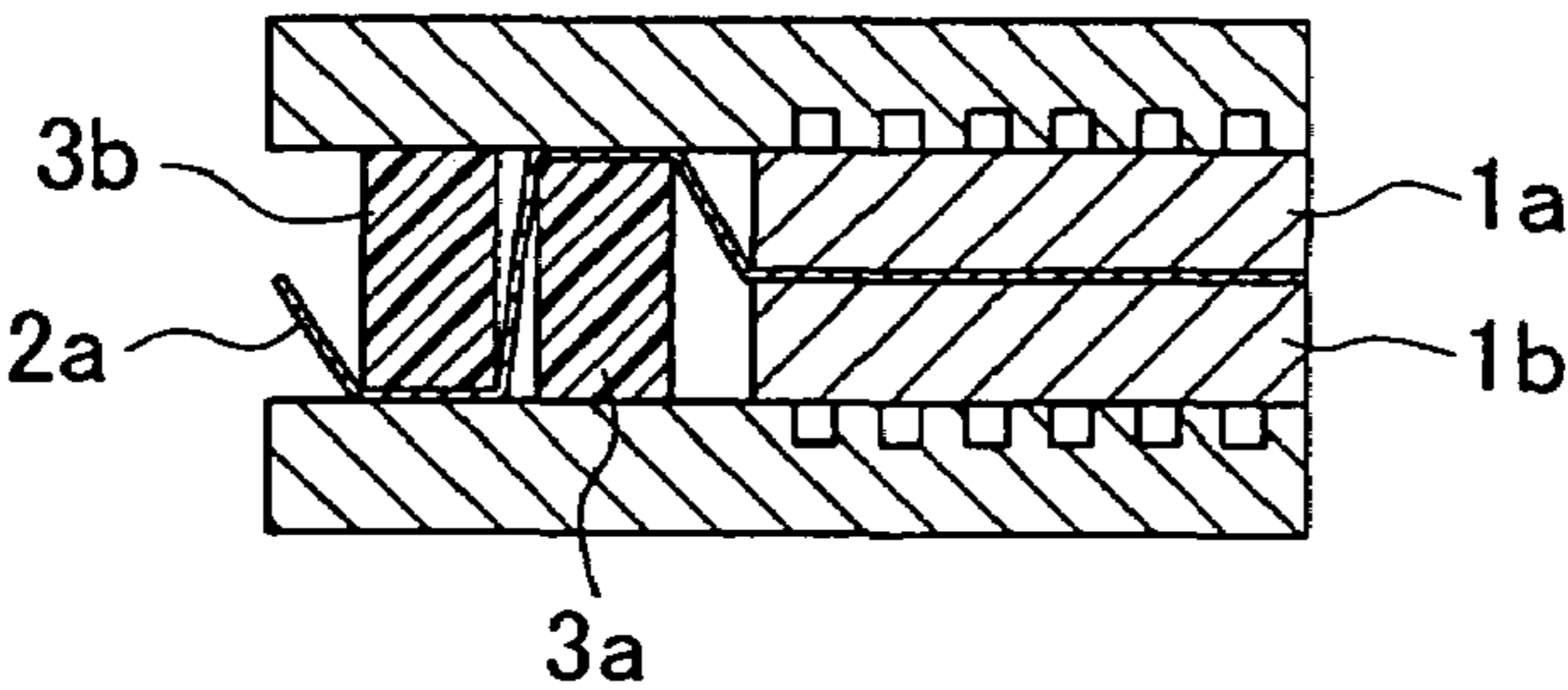
FIG. 19 (Prior Art)
