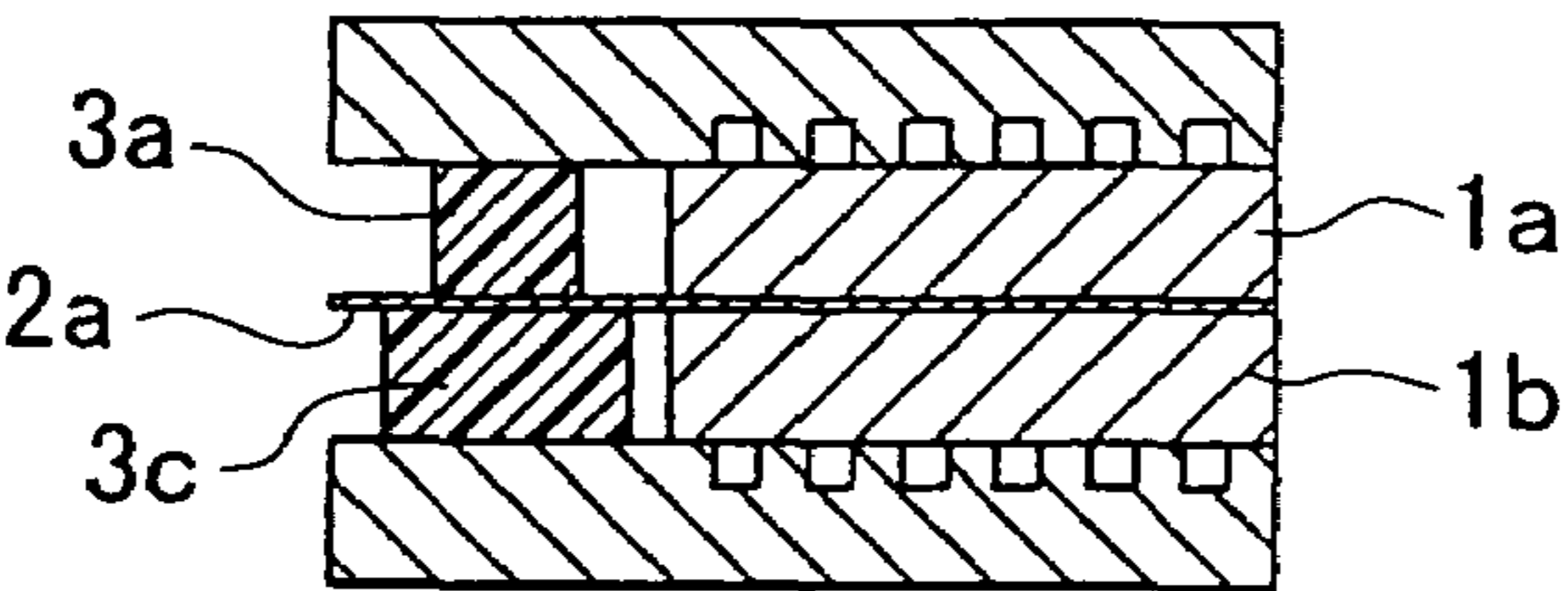
FIG. 20 (Prior Art)
