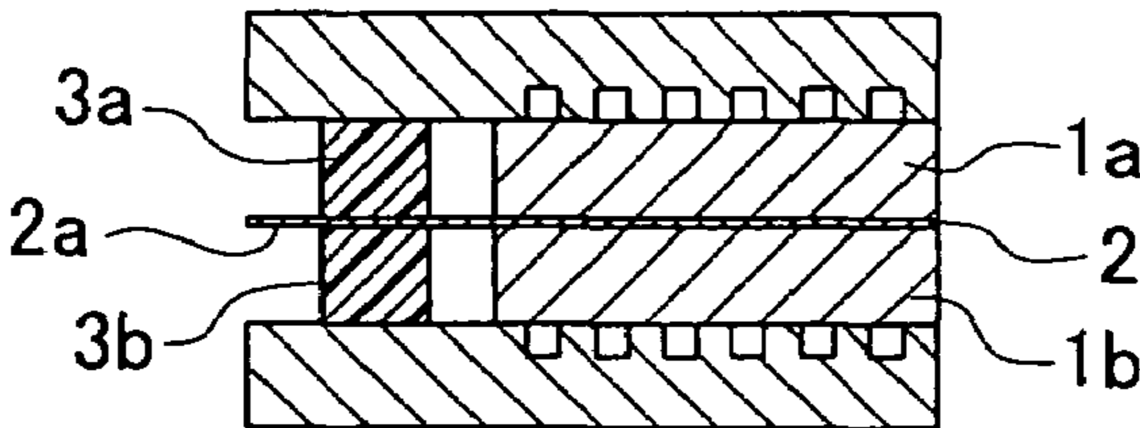
FIG. 17 (Prior Art)
