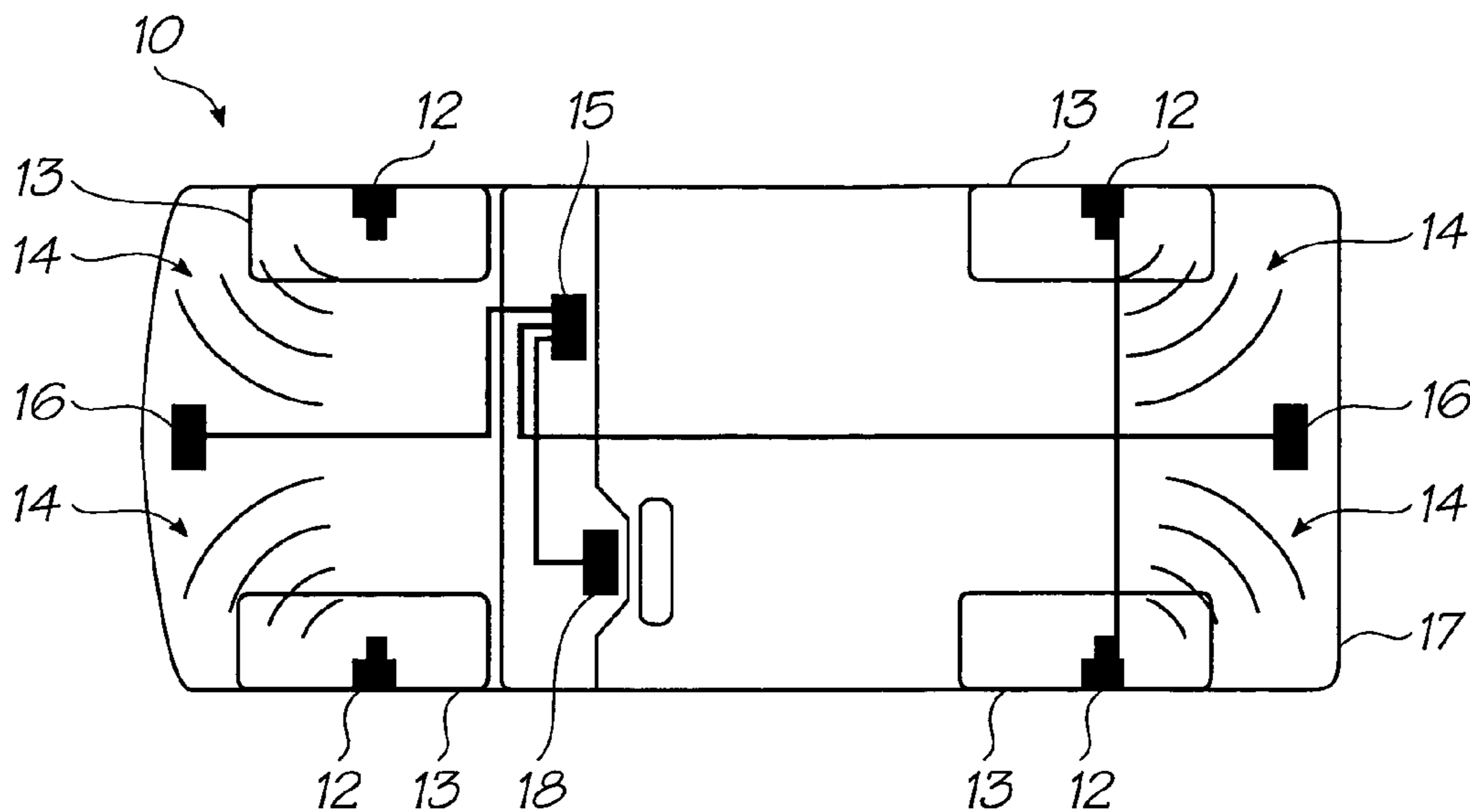
FIG. 1 (Prior Art)
