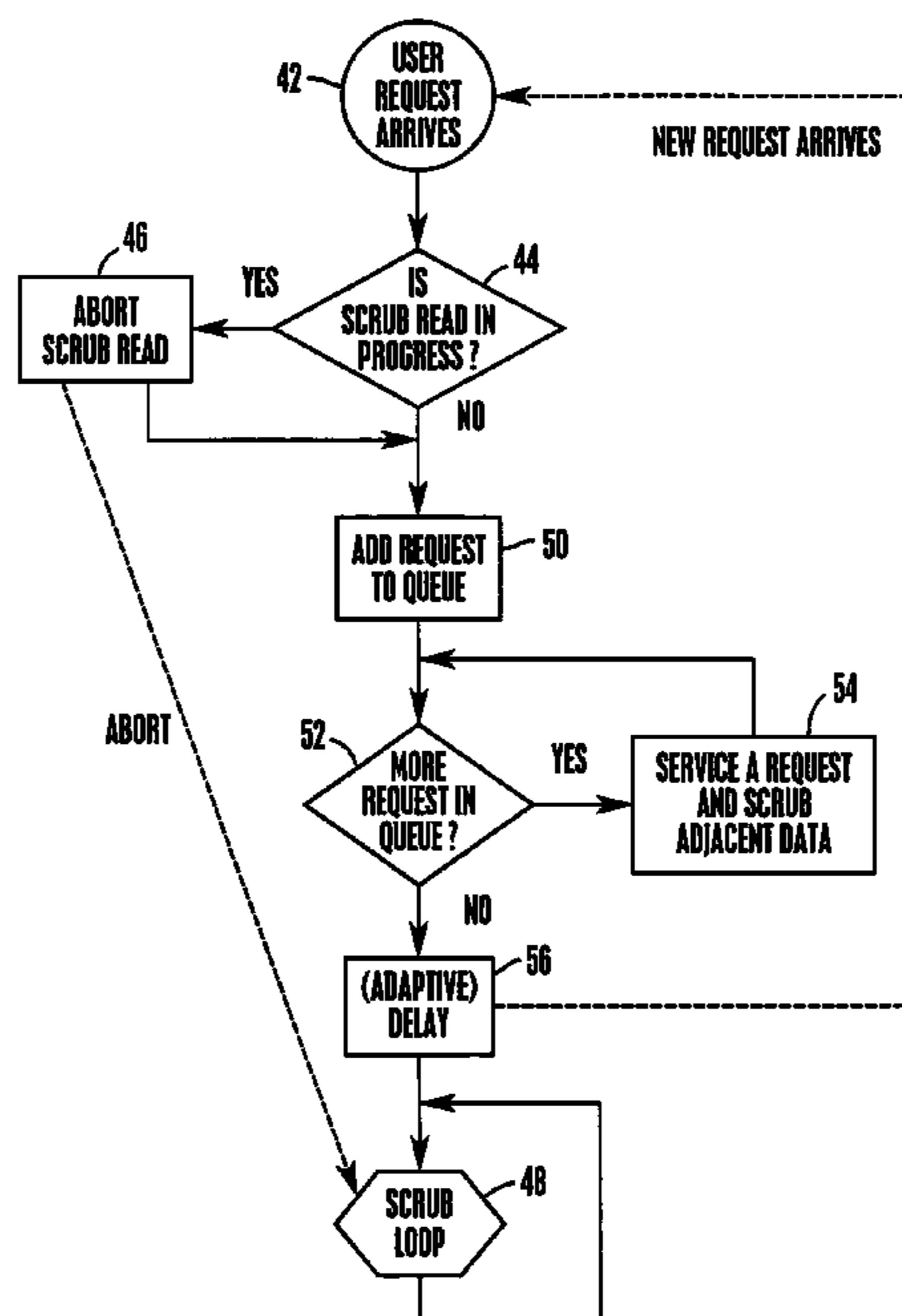
Interrupt of Scrub with Delay, opportunistic options
