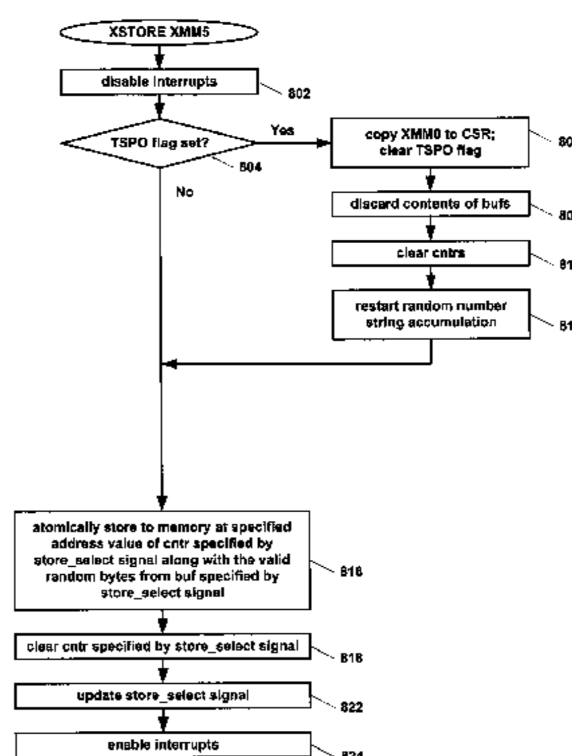
RNG Unit Operation (XSTORE XMM5 instruction)
