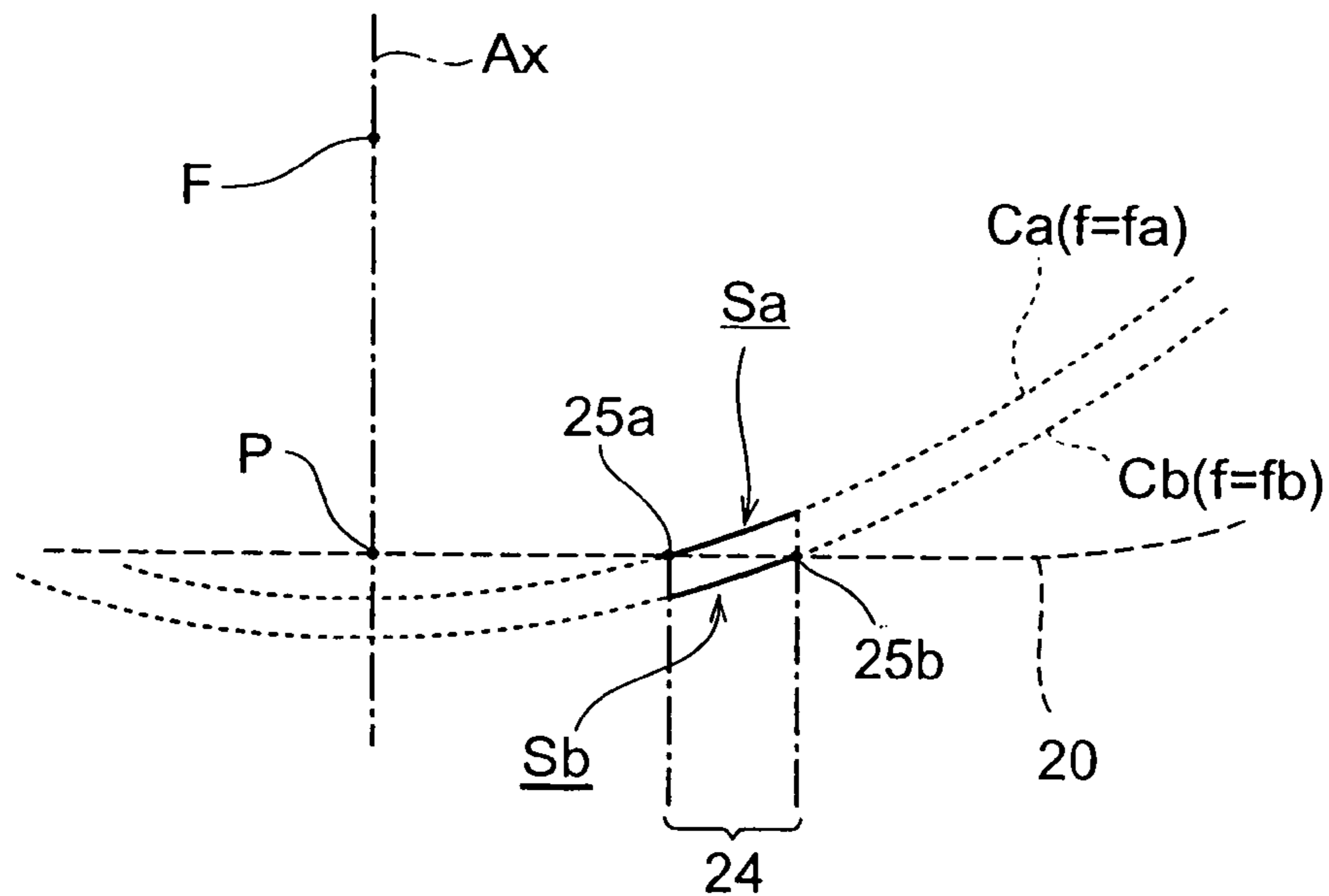
Fig. 7 PRIOR ART
