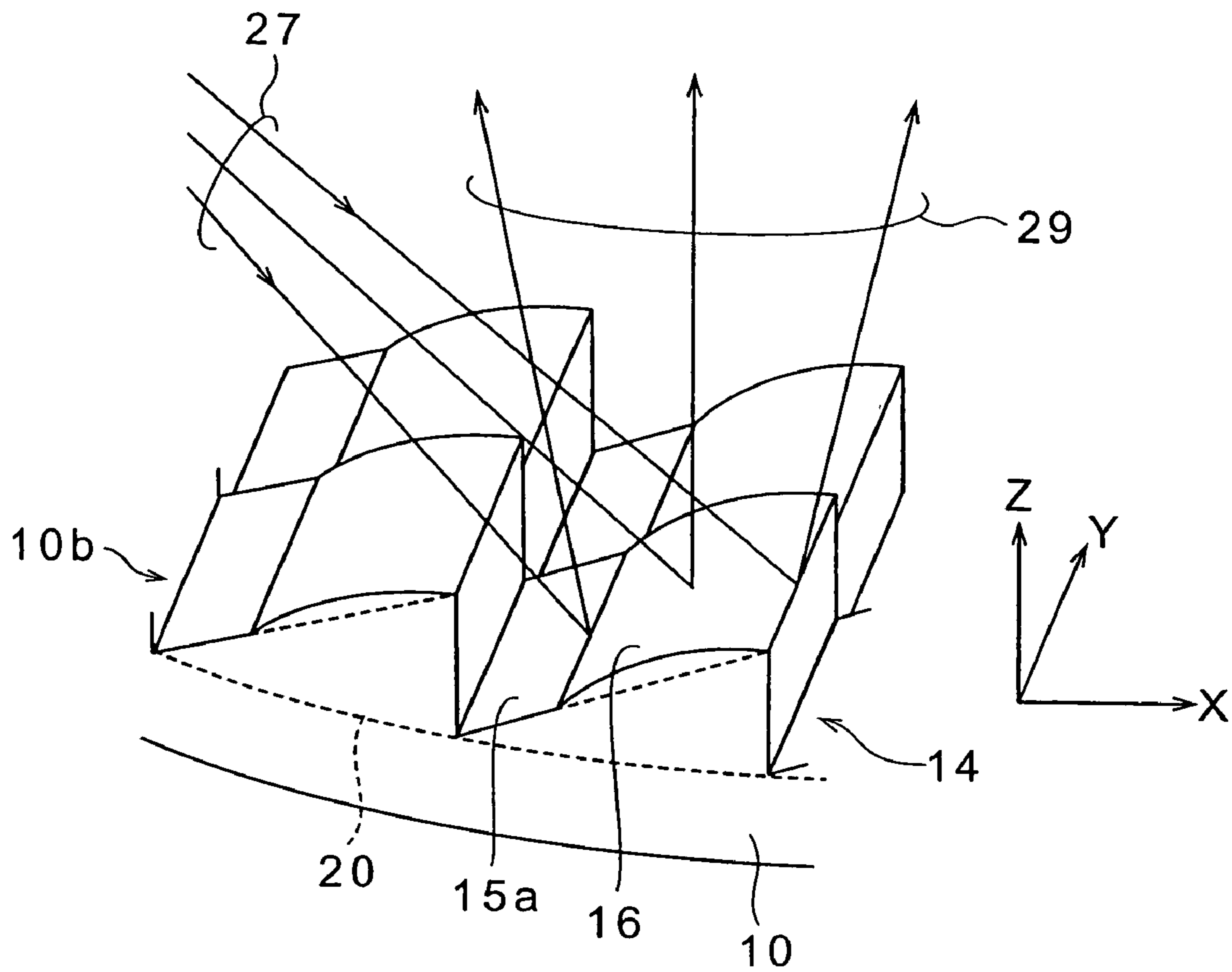
Fig.14 PRIOR ART
