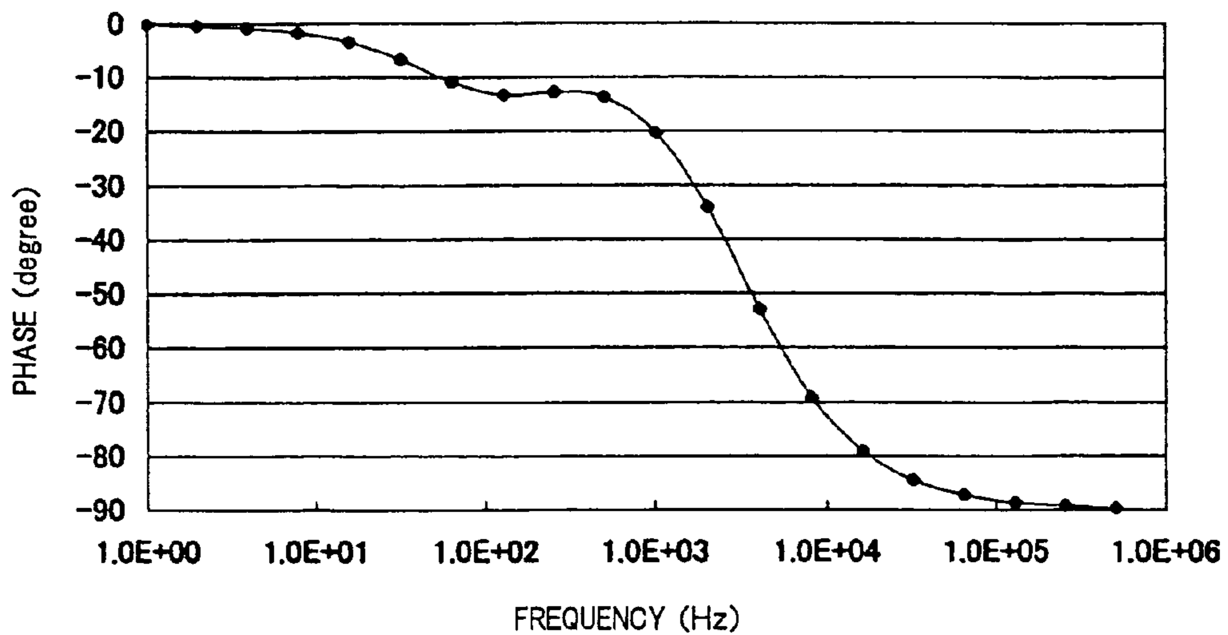
PHASE CHARACTERISTIC OF CONVENTIONAL EDFA
