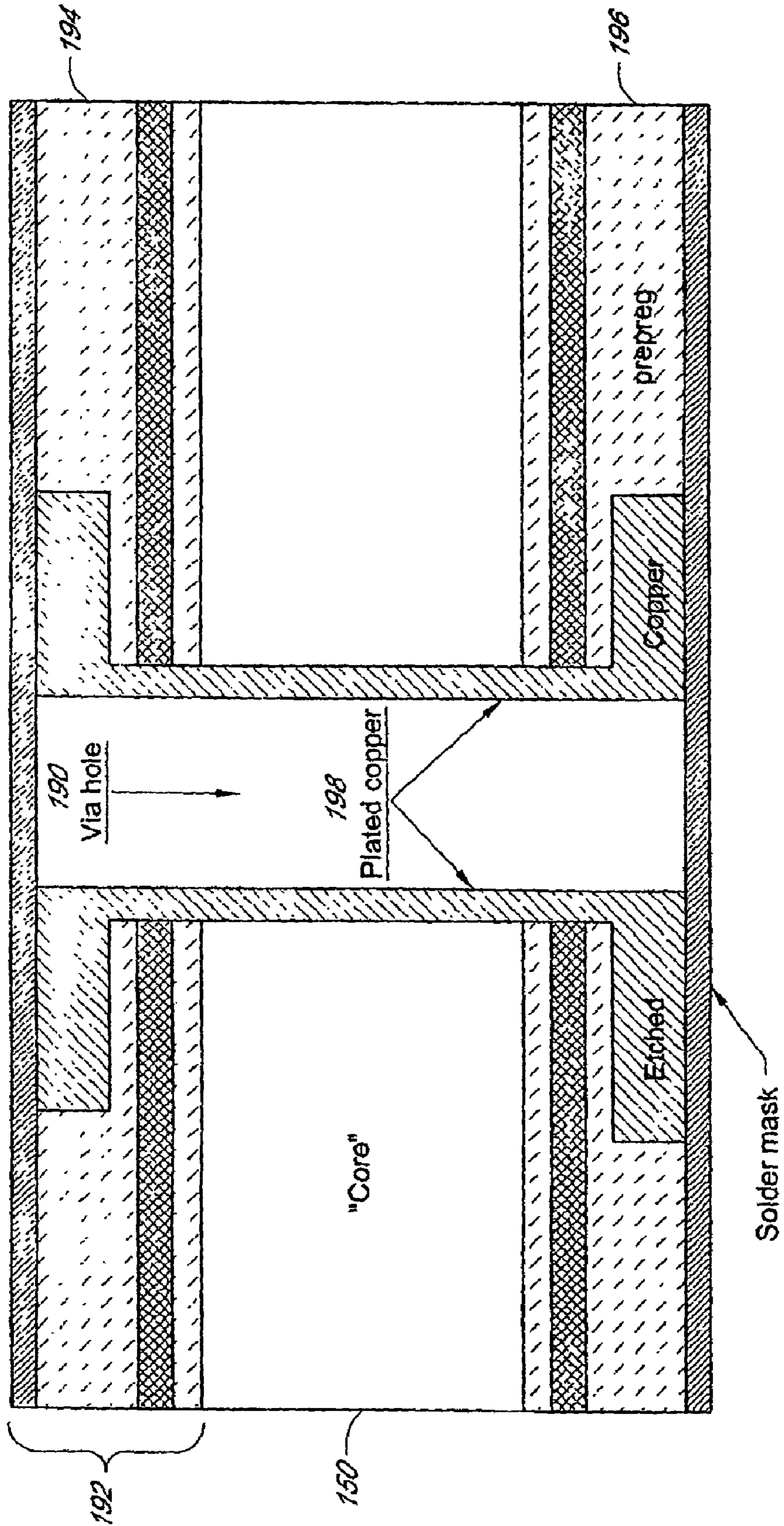
Cross section of via hole
