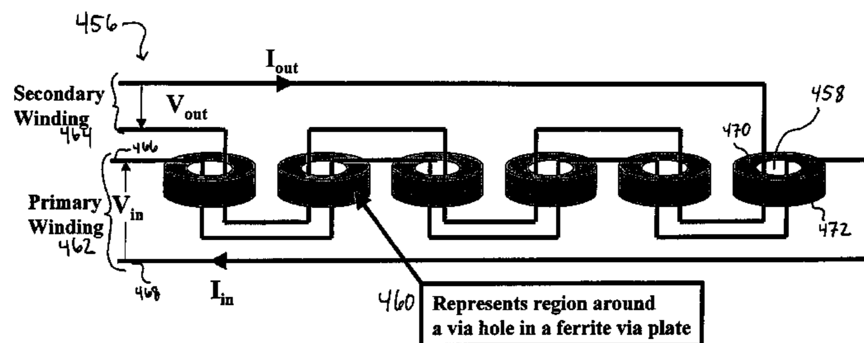
6 Cell Transformer turns ratio=1 to 1 (primary to secondary) V_{in} = V_{out} I_{in} = I_{out} Max current in Cell= I_{out}
