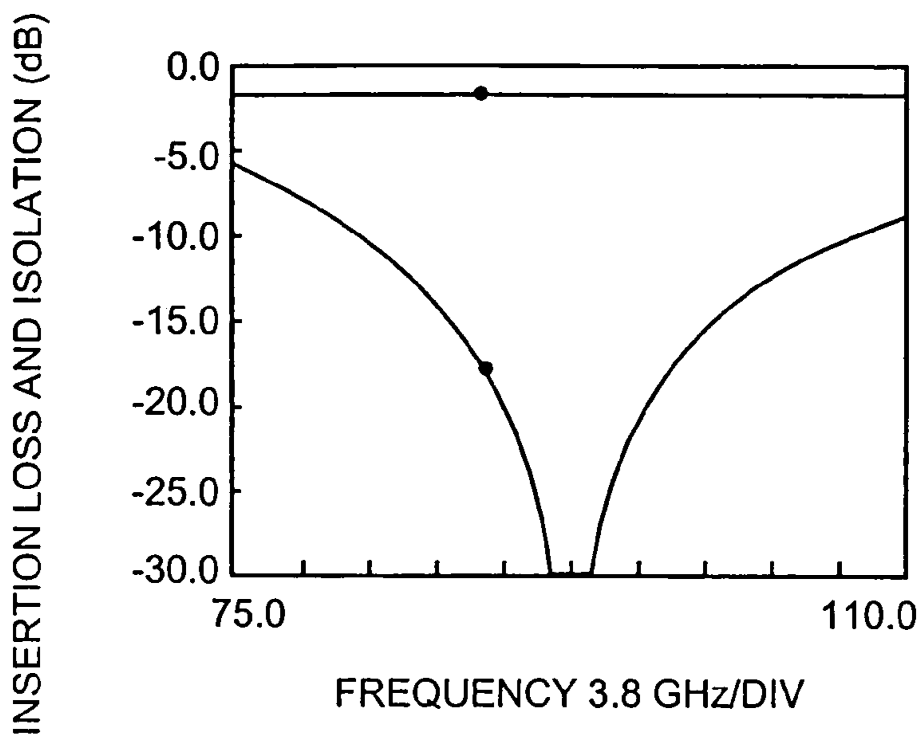
Fig.15 (Prior Art)
