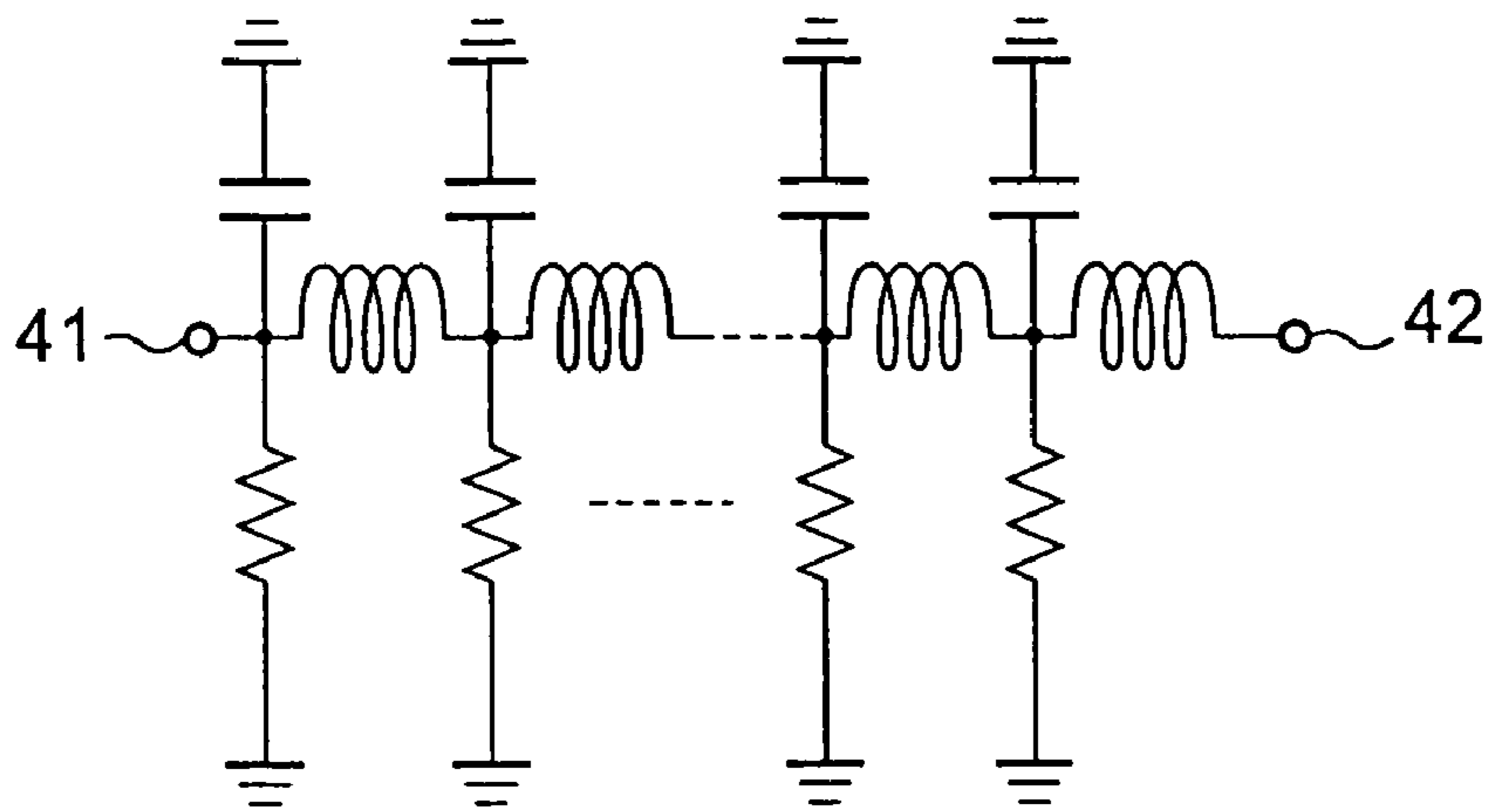
Fig.18 (Prior Art)
