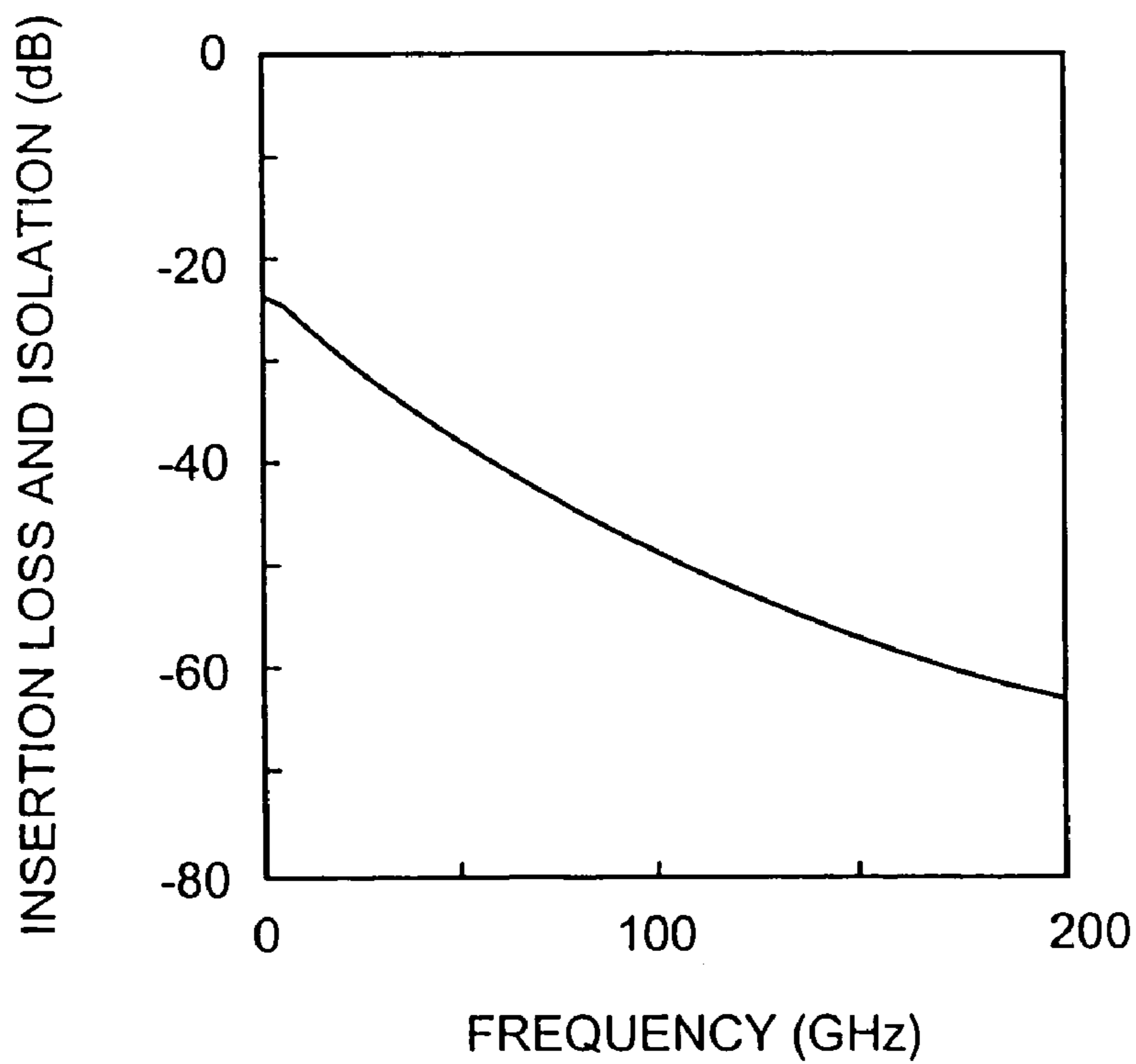
Fig.19 (Prior Art)
