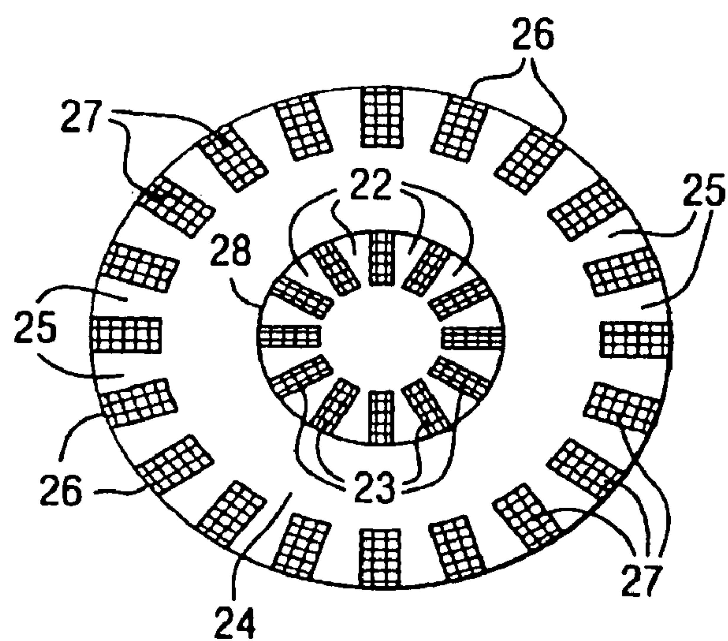
FIG. 2 Prior Art
