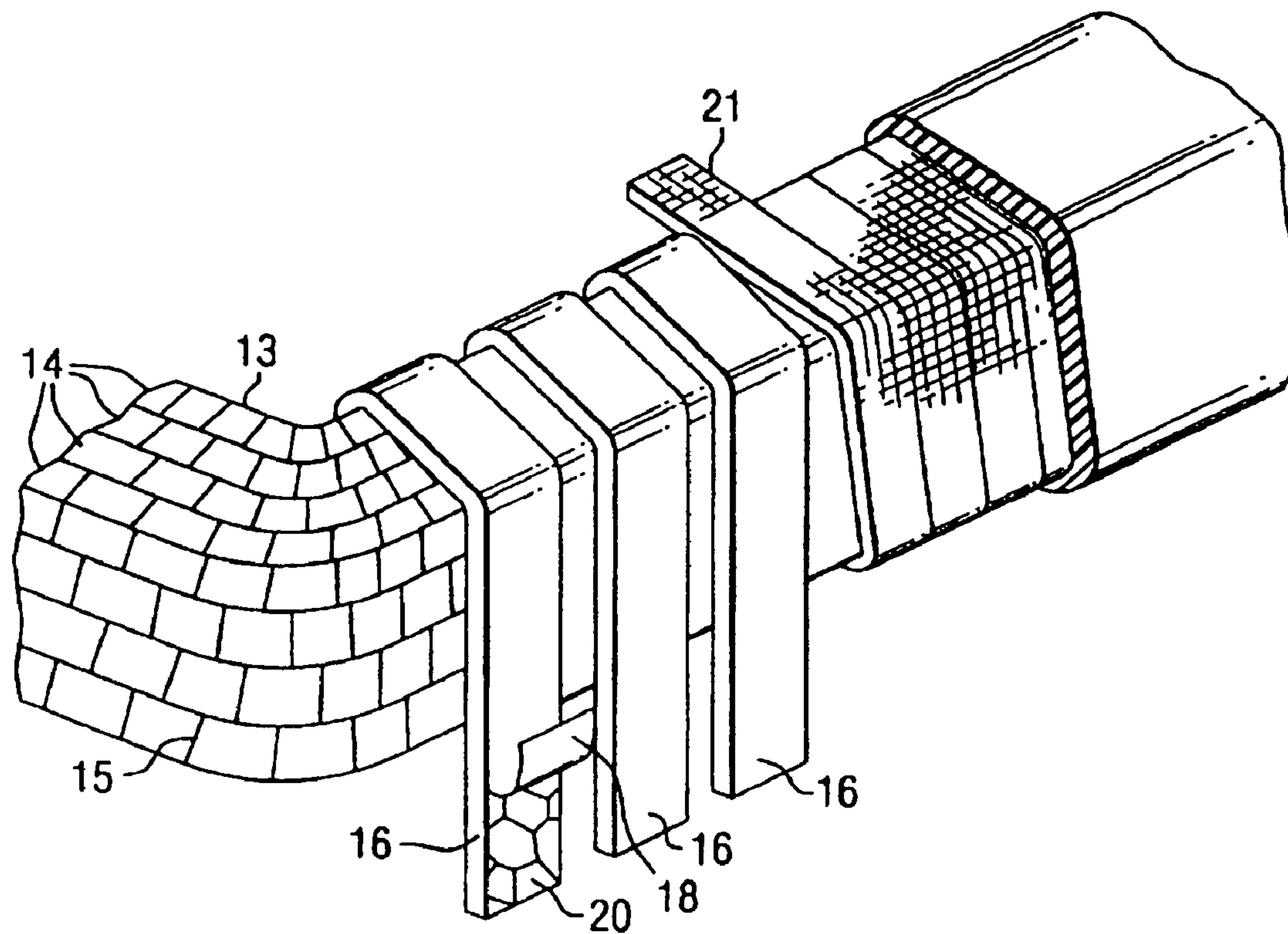
FIG. 1 Prior Art
