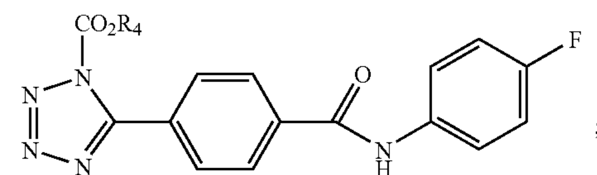
Formula CR
