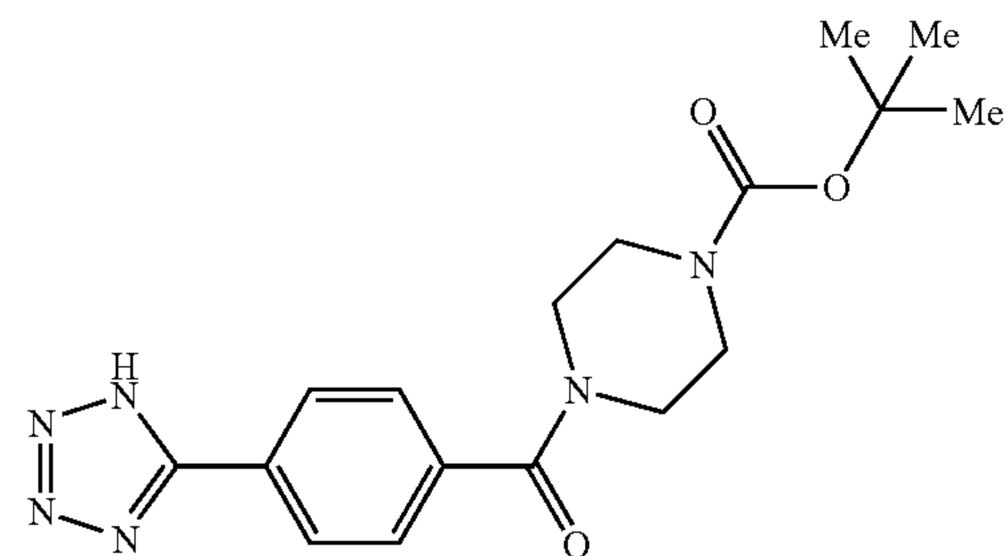
Compound HL
