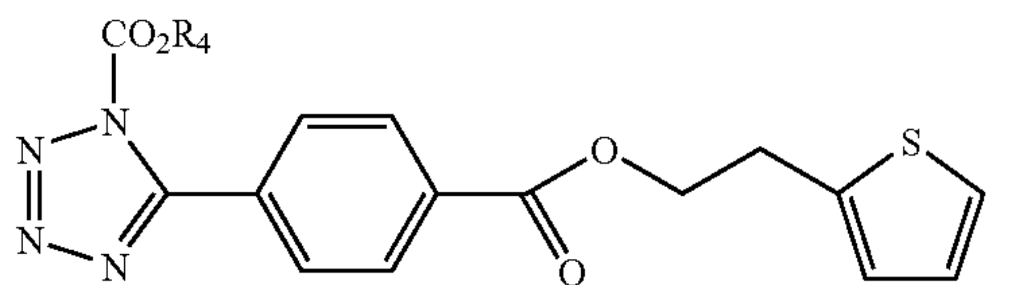
Formula CJ
