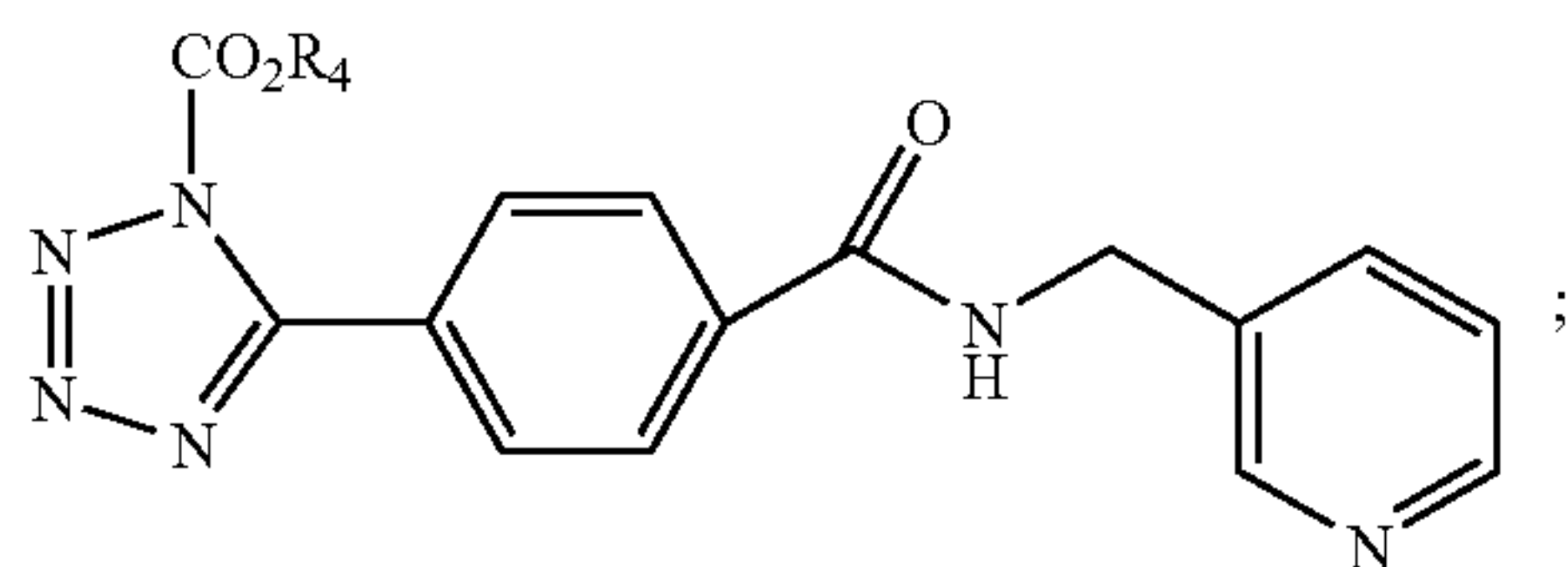
Formula BY
