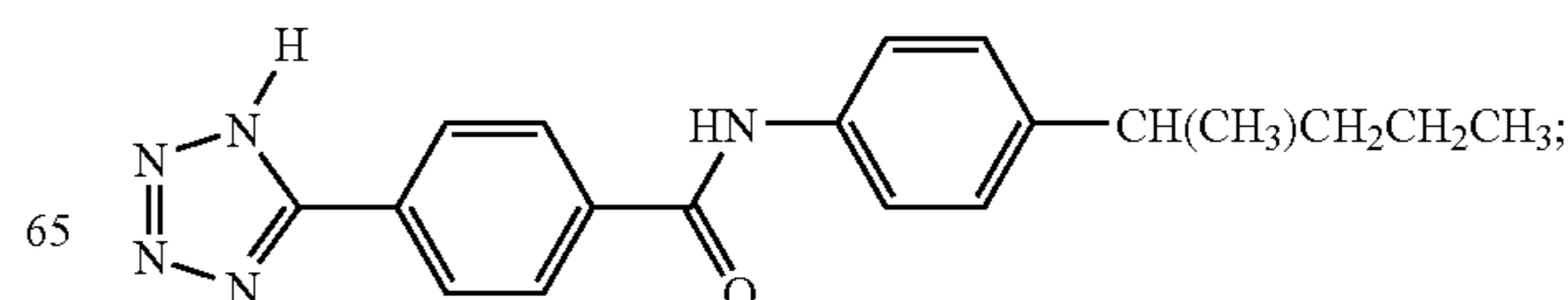
Compound EL
