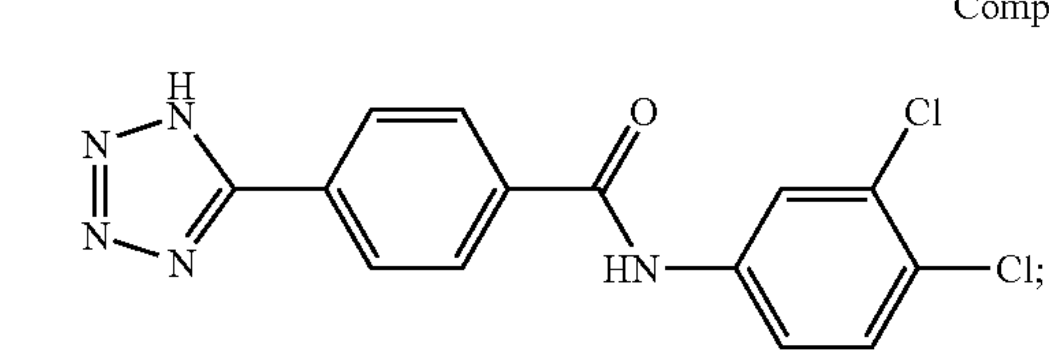
Compound JM
