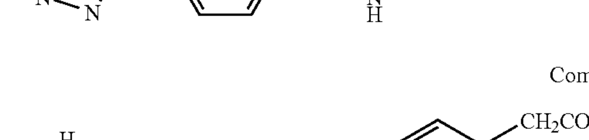
Compound IJ
