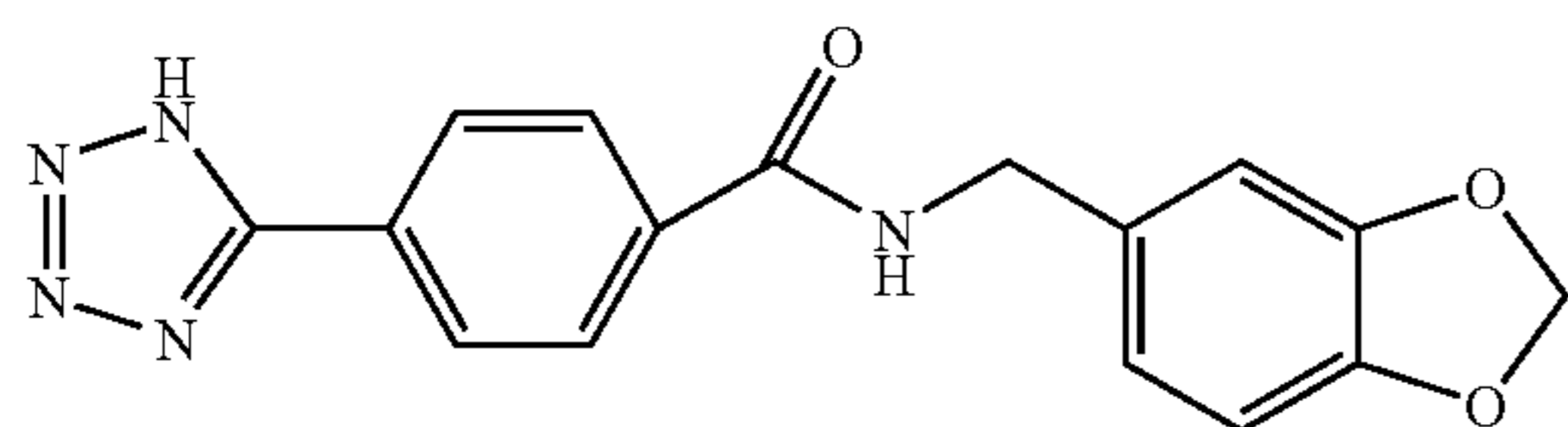
Compound HC
