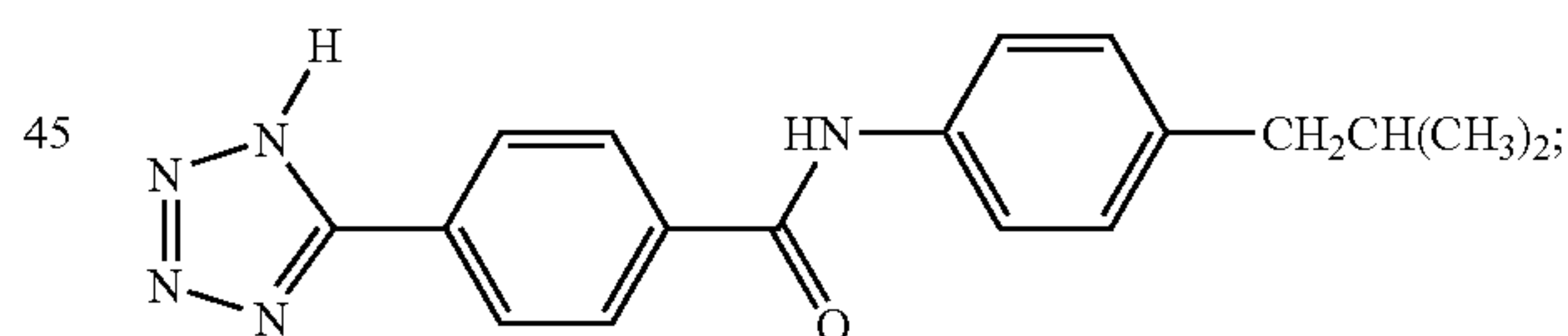
Compound EJ
