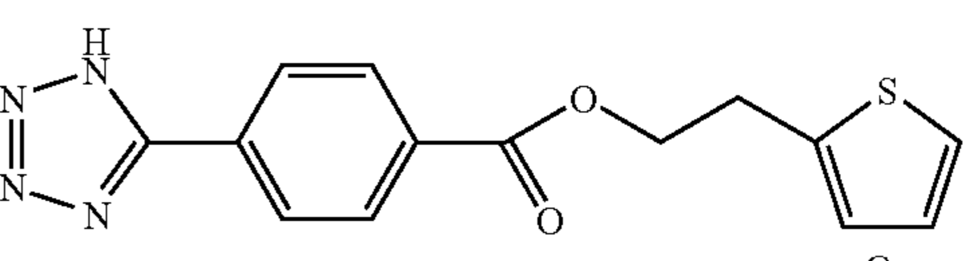
Compound HR
