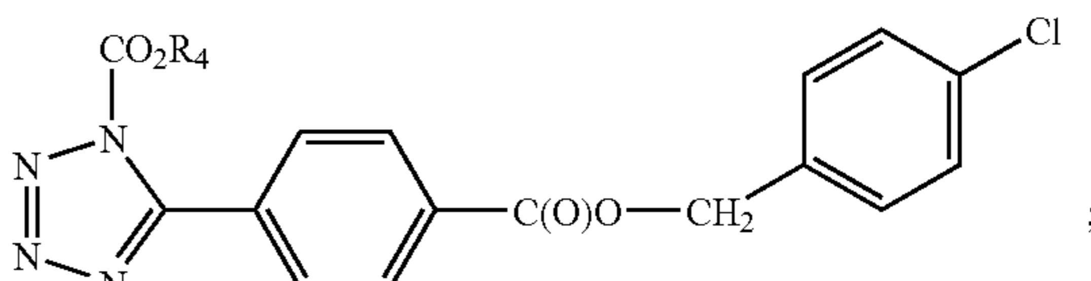
Formula BA
