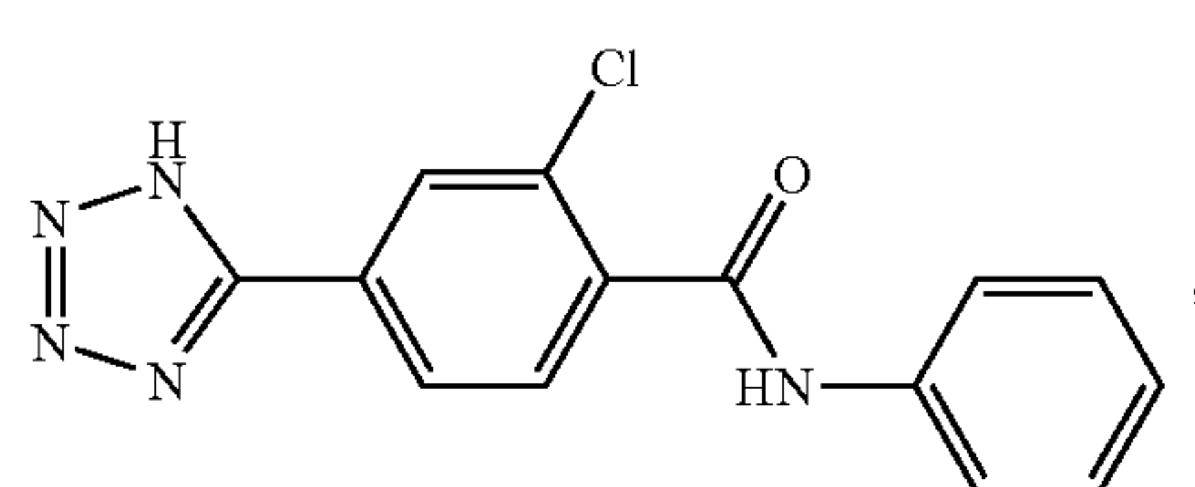
Compound JJ
