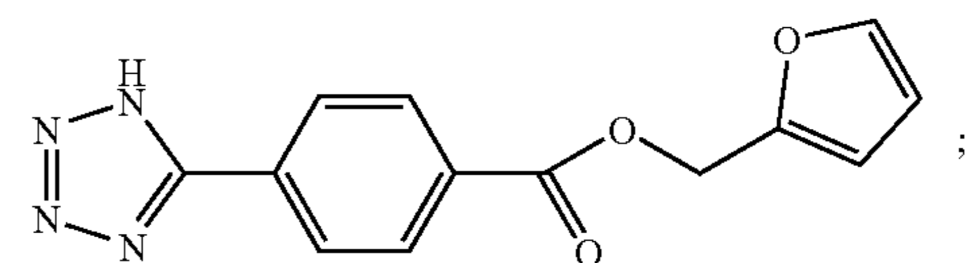
Compound HQ
