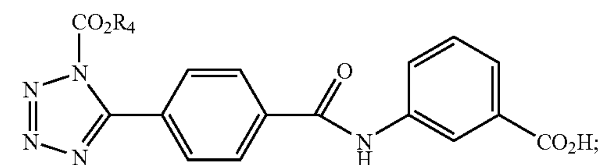
Formula CV
