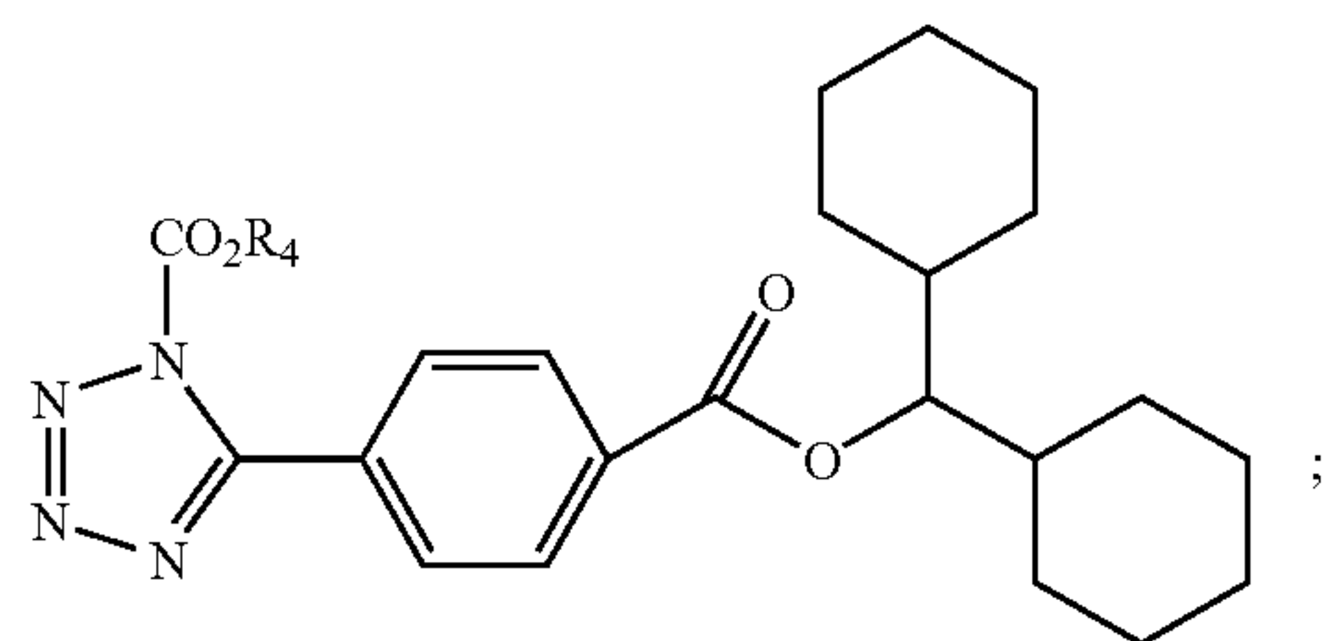
Formula BV
