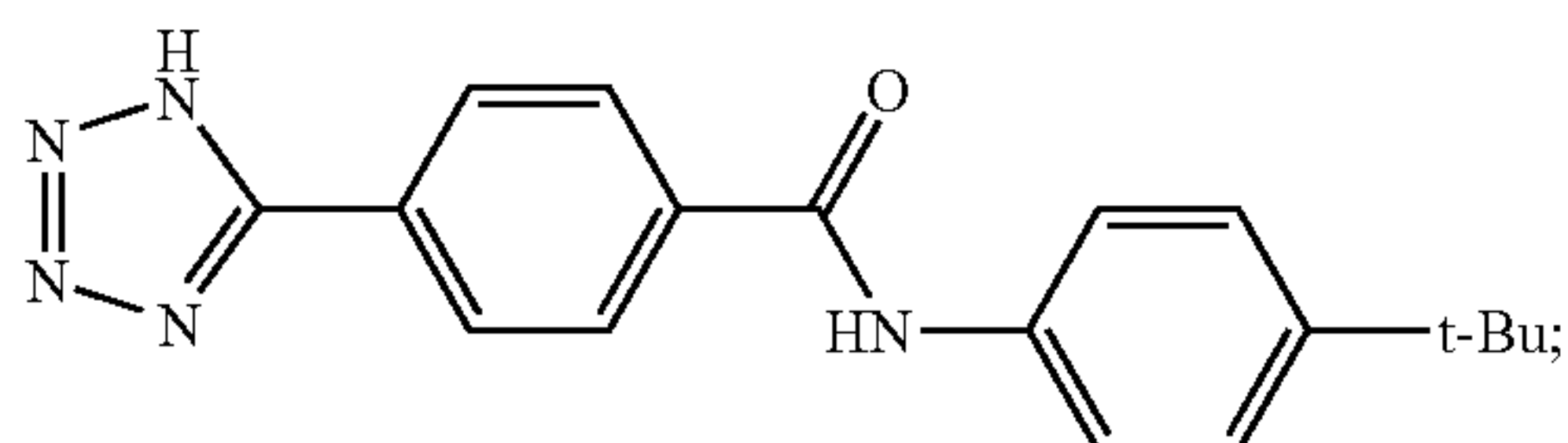
Compound JO
