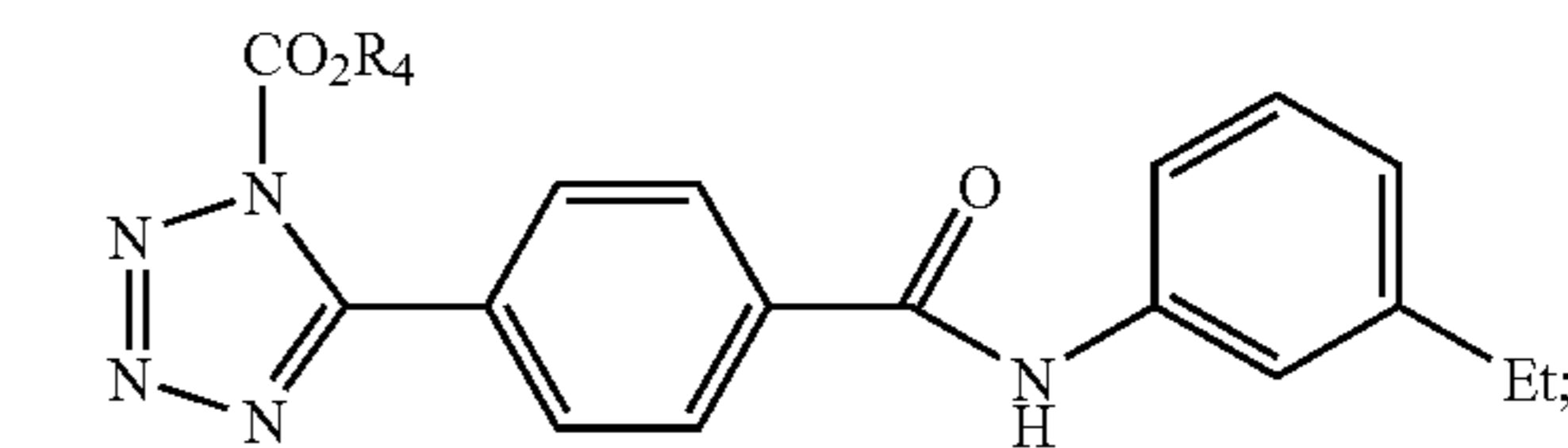
Formula CY
