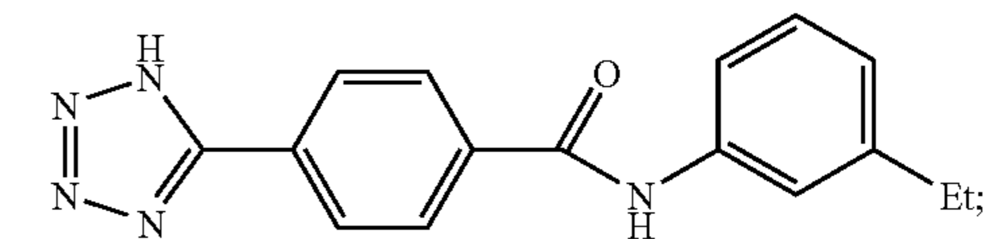
Compound IF
