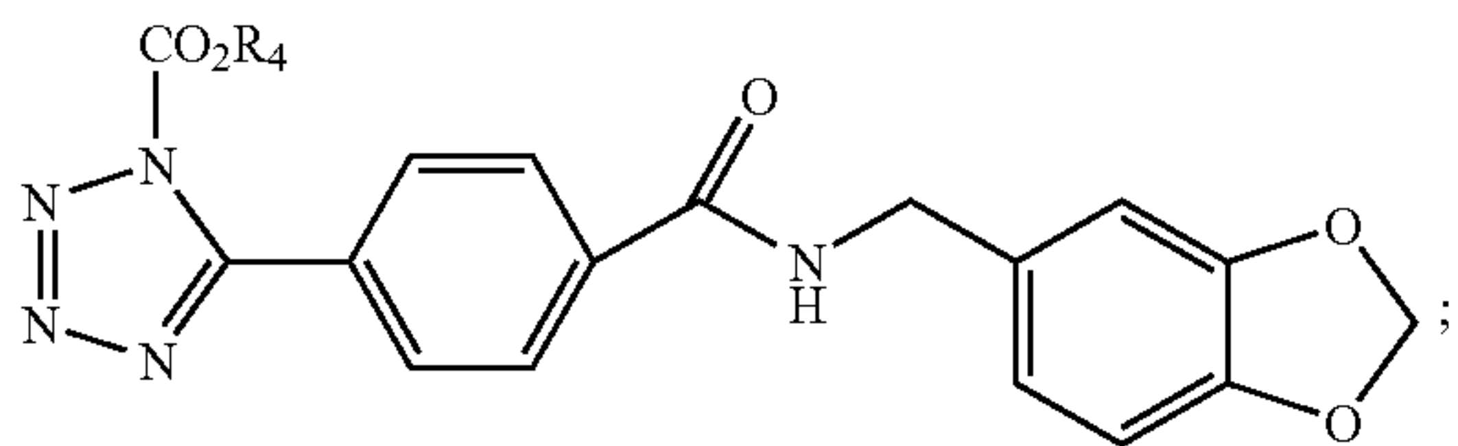
Formula BX
