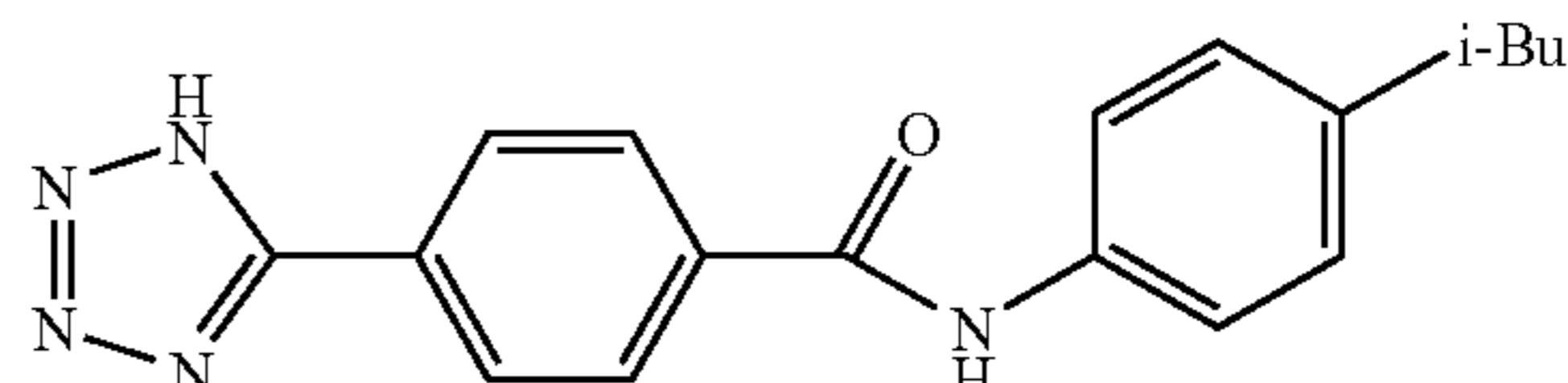
Compound IH
