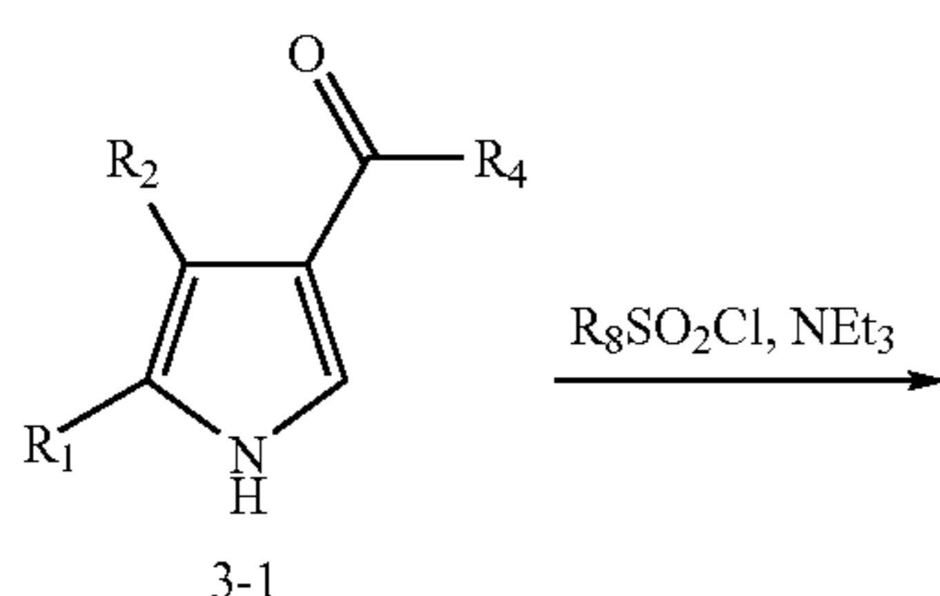
Scheme 3
