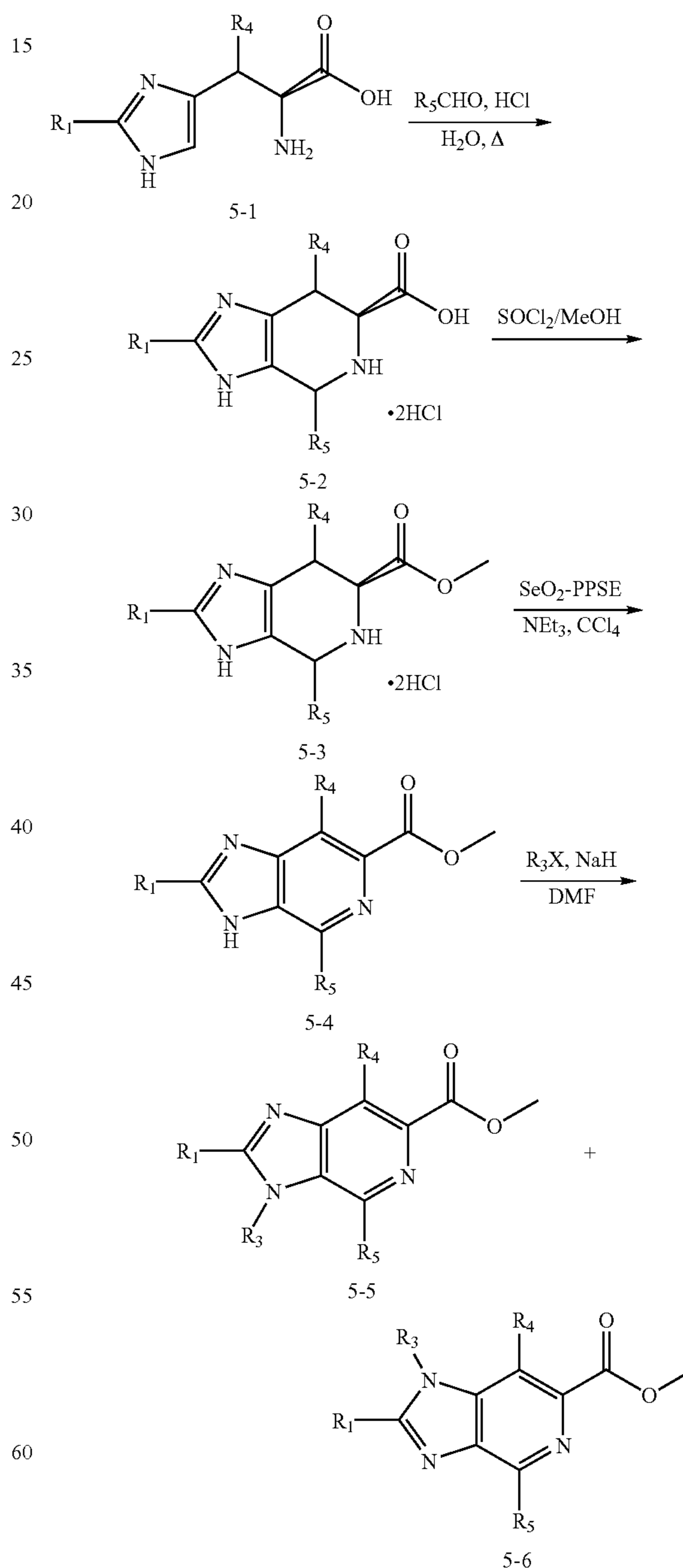
Scheme 5
