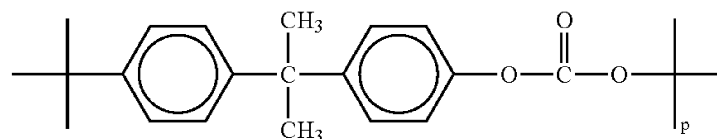
Lexan® 141: p~120, Tg~150° C. Makrolon® 5700: p~280, Tg~157° C.
